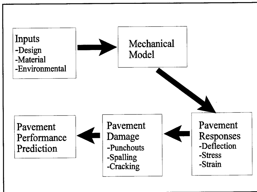
Figure 2.2 Typical Framework of Mechanically Based Design.
