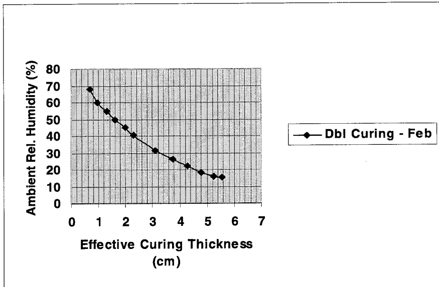
Figure 3.25 Standard for Curing Effectiveness Based on Field Data.
