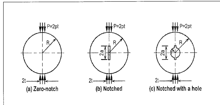
Figure 3.12 Split Cylinder Specimens.
