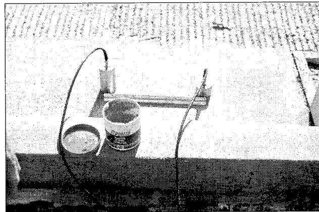
Figure 3.5 Pulse Velocity Test Configuration.
