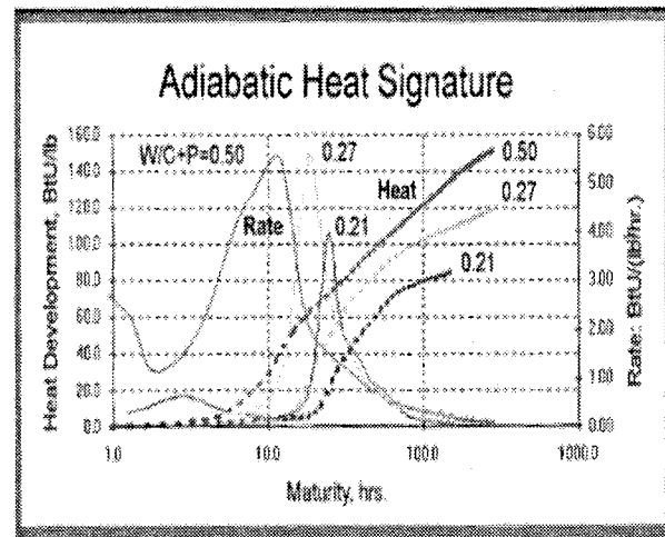
Figure 3.20 AHS Curve.
