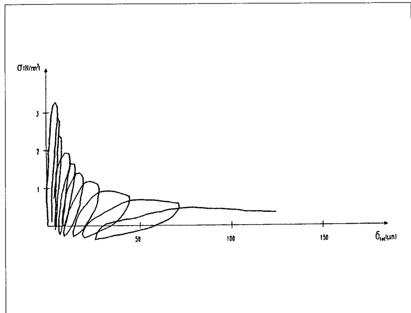
Figure 2.4 Reduction on Concrete Modulus Due to Cracking Damage.(Grzybowski 1989).
