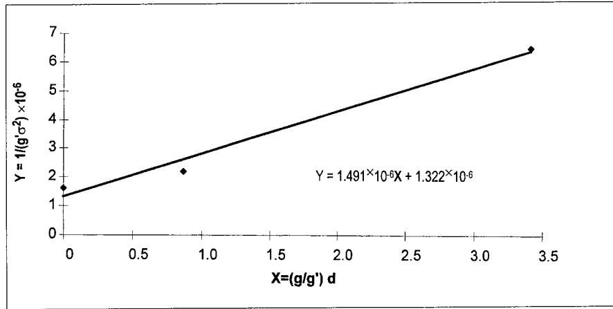
Figure 3.13 Fracture Test Results.
