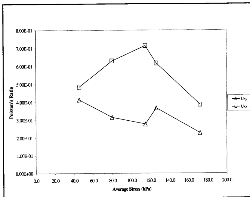
Figure 3.4 Poisson's Ratio Derived from Triaxial Test.
