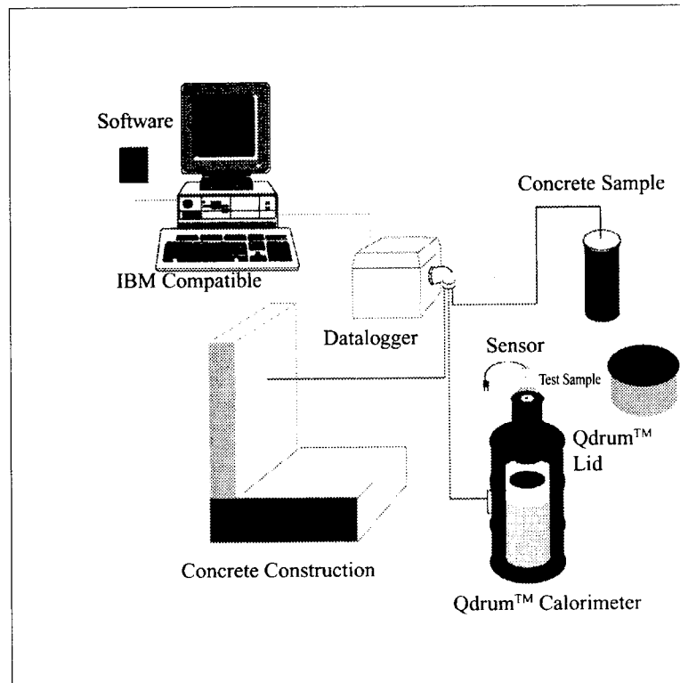
Figure 3.19 AHS System.
