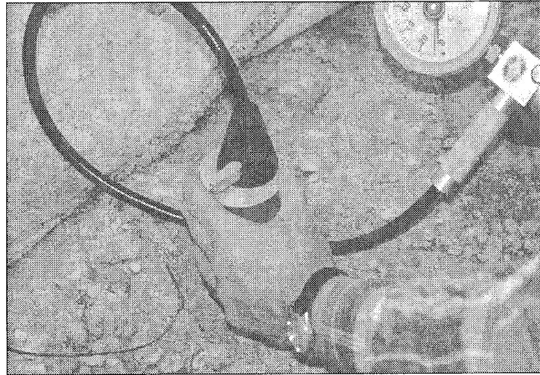
Figure 3.11 Break-Off Test Apparatus.
