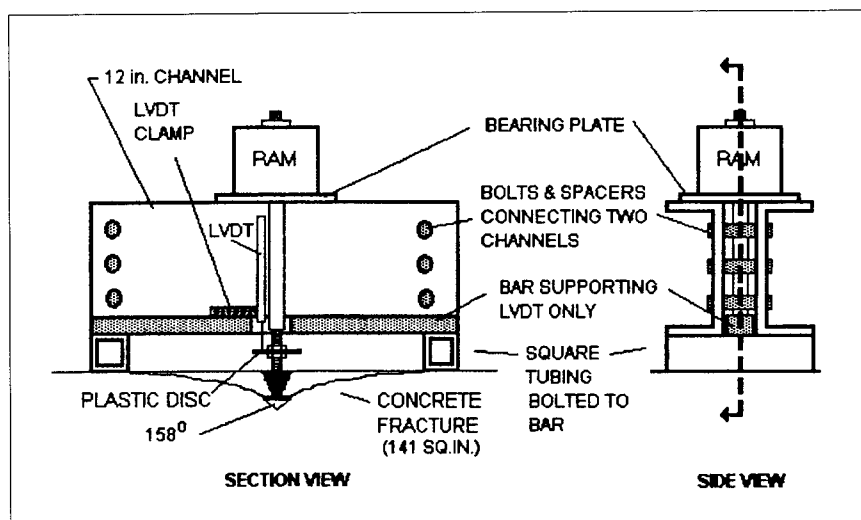
Figure 3.10 Pullout Loading Frame for Fracture Testing. (Dilly, 1994).
