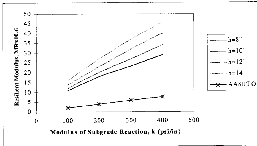
Figure 1.1 Correlation Between k-value and M_R .
