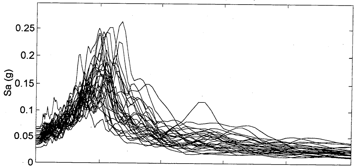
Alaskan Way Viaduct 2 Spectral Accelerations (M=8.0)
