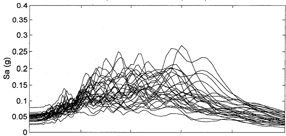
Nooksack River Spectral Accelerations (M=8.5)
