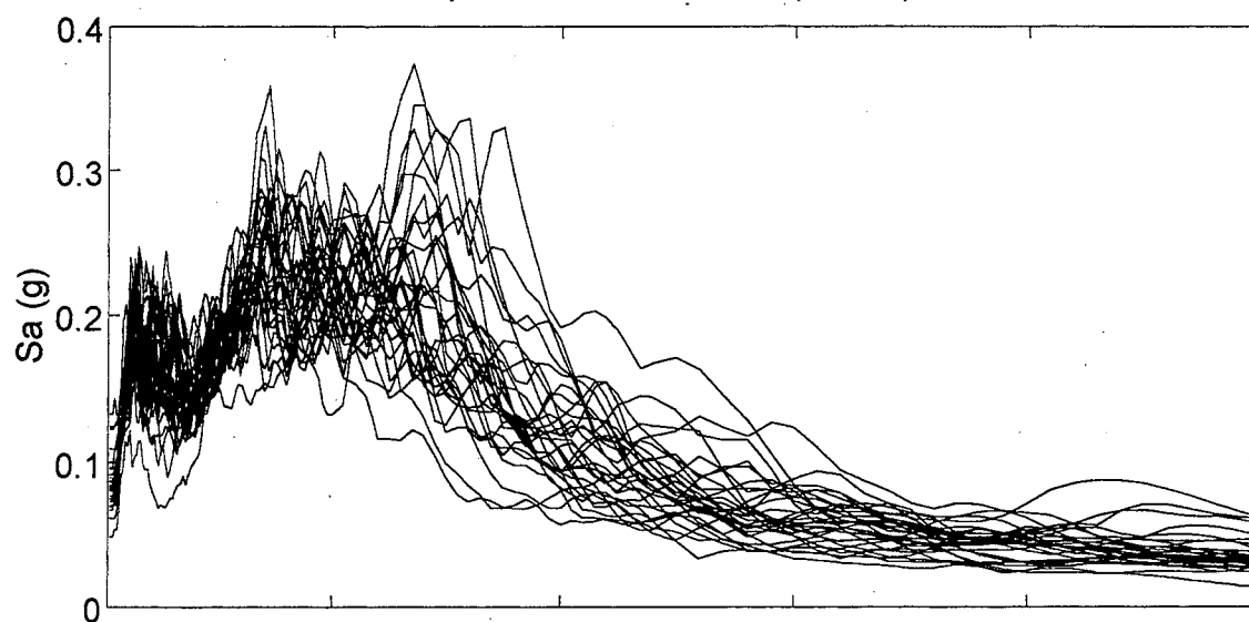
Alaskan Way Viaduct 2 Spectral Accelerations (M=8.5)
