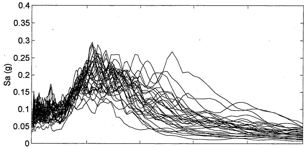
North Ferndale Spectral Accelerations (M=9.0)
