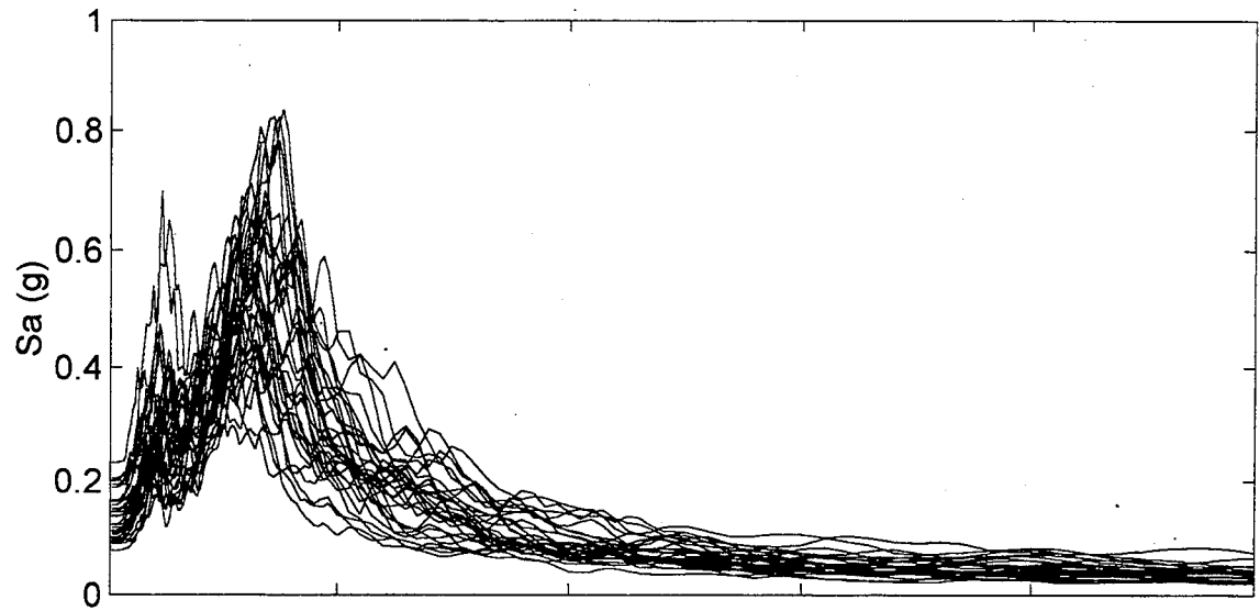
Andresen Road Spectral Accelerations (M=9.0)
