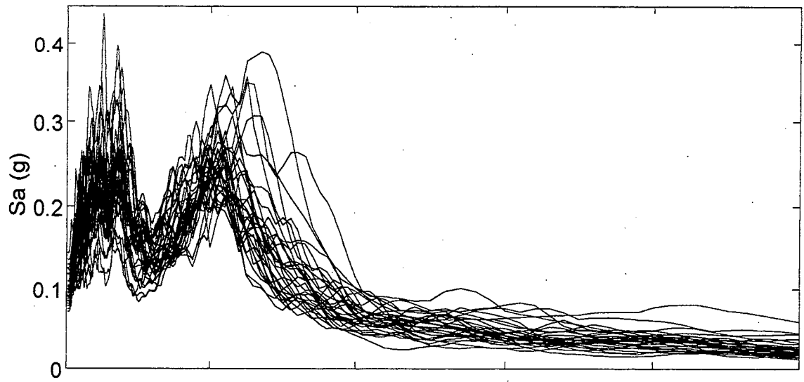
Capitol Boulevard Spectral Accelerations (M=8.0)
