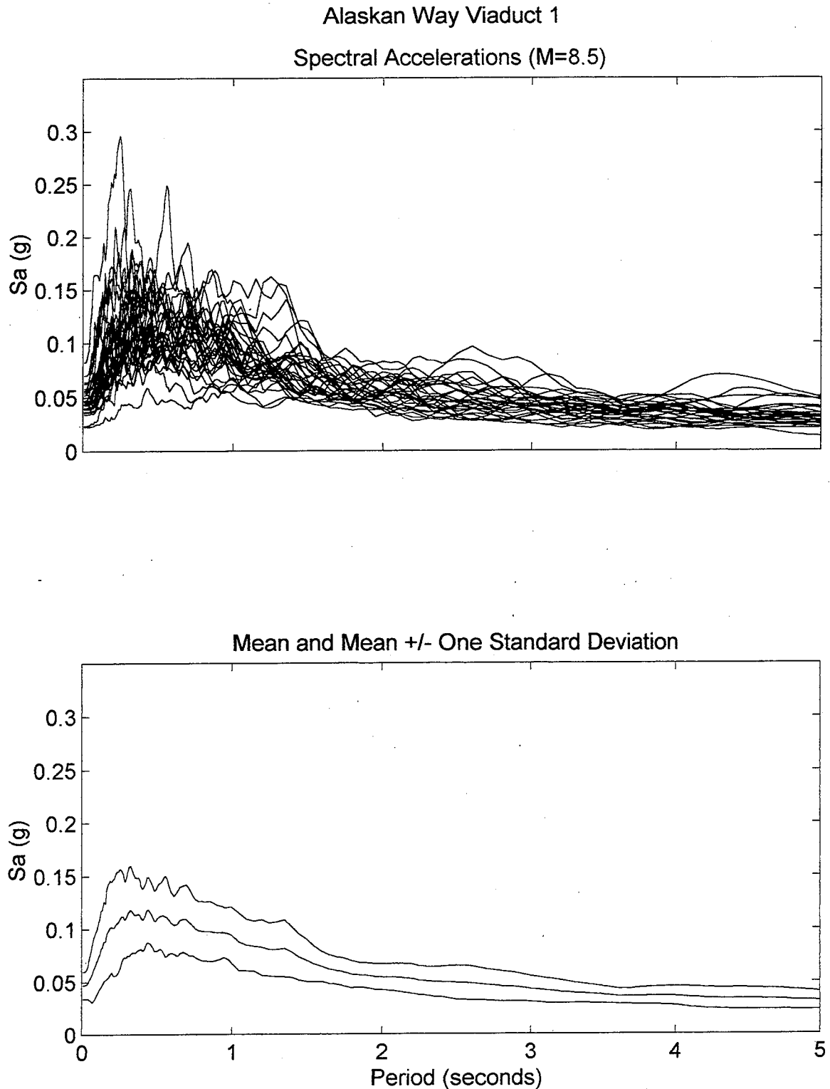
Figure 14. (a) Computed rock outcrop response spectra at Alaskan Way Viaduct site for 30 realizations of the M_w = 8.5 Cascadia subduction zone earthquake, and (b) corresponding mean and mean \pm one standard deviation rock outcrop response spectra.
