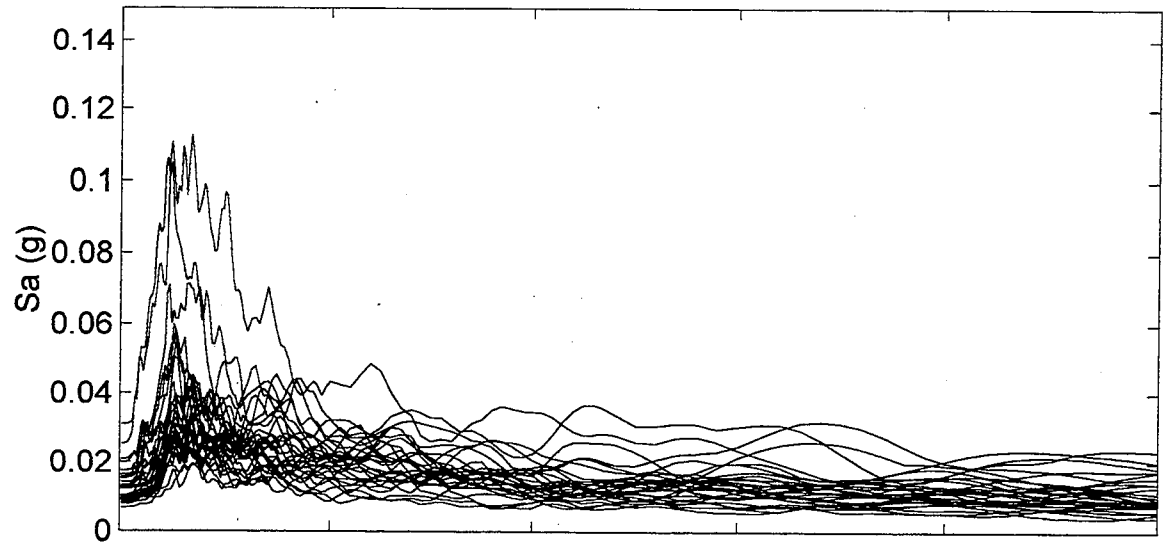
Yakima Spectral Accelerations (M=8.0)
