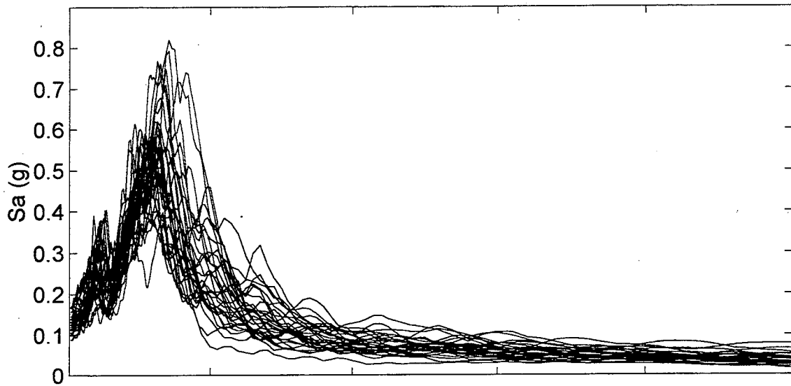
I-5/NE 99th Street Spectral Accelerations (M=8.5)
