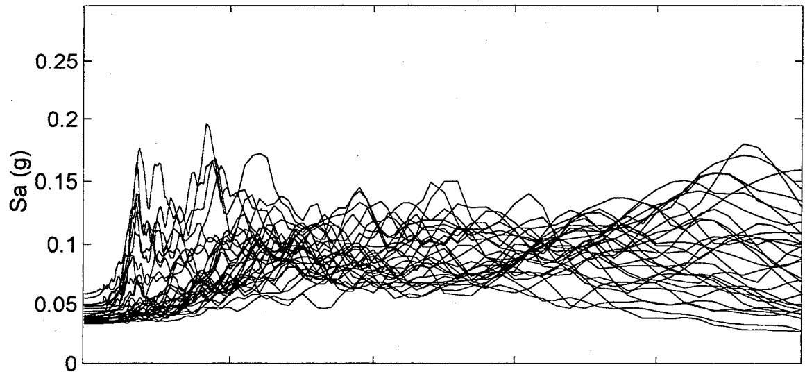
Bone River Spectral Accelerations (M=9.0)
