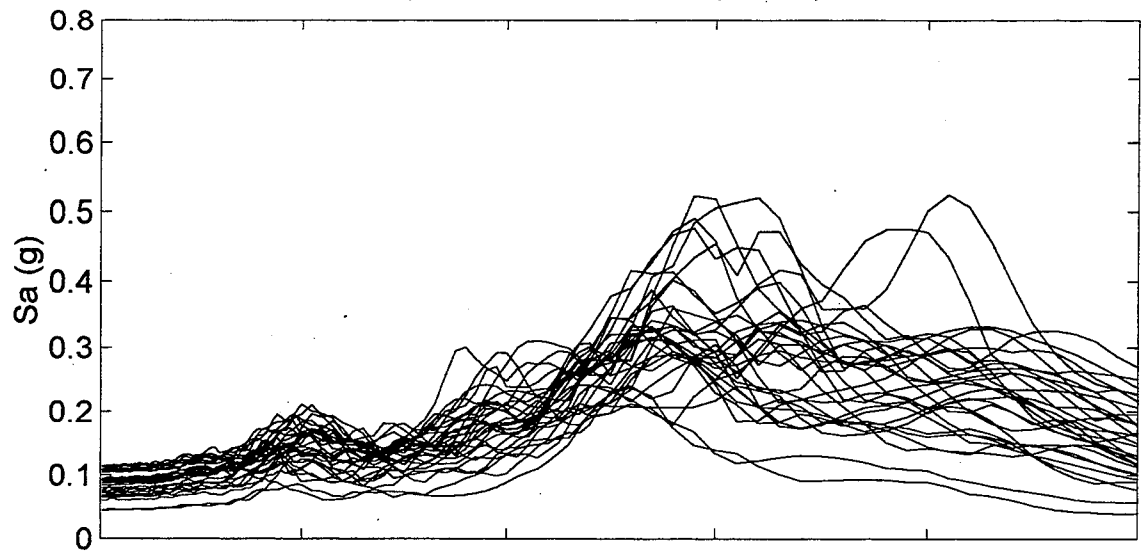
Mercer Slough 2 Spectral Accelerations (M=9.0)
