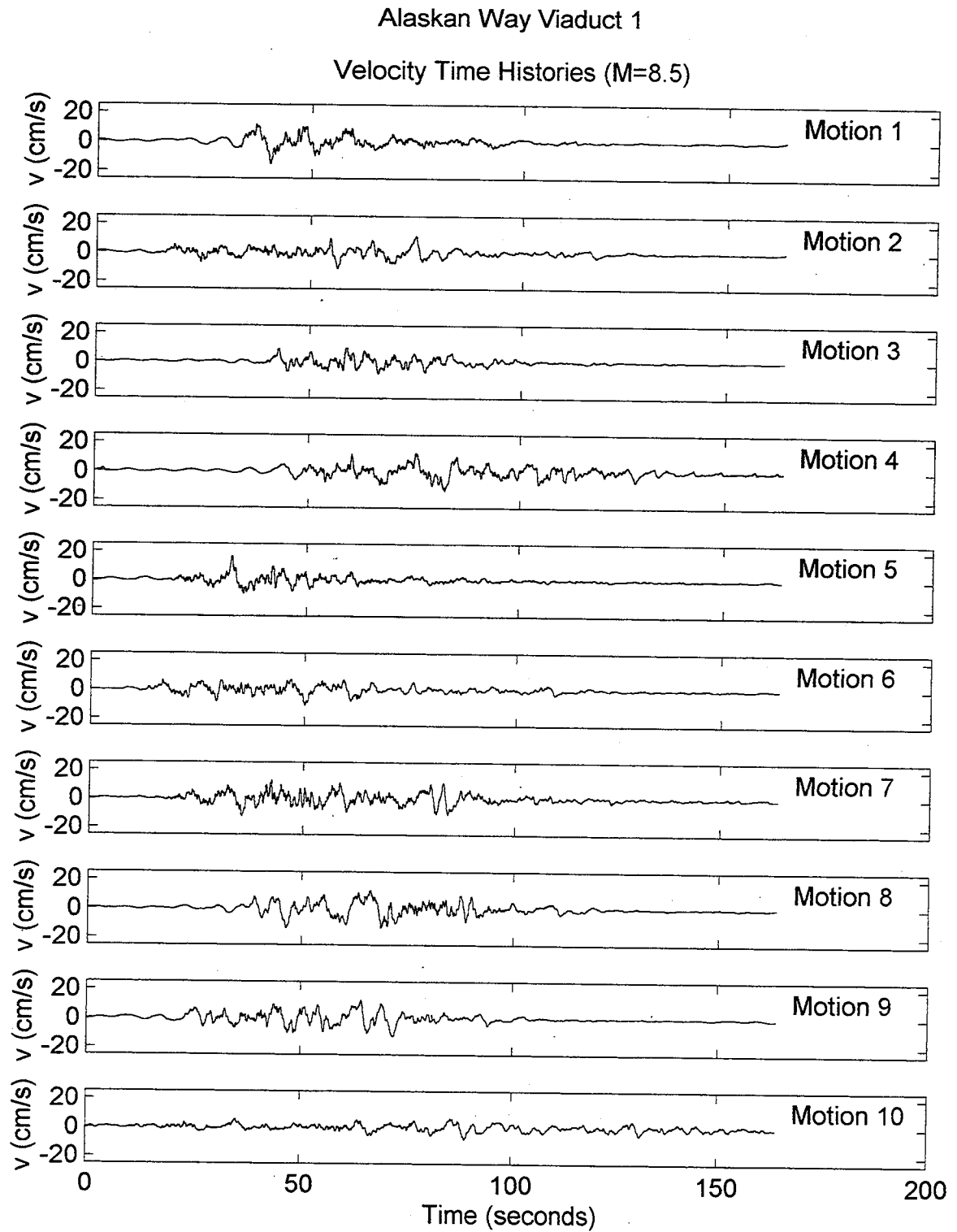
Figure 11. Computed time histories of rock outcrop velocity at Alaskan Way Viaduct site for M_w = 8.5 Cascadia subduction zone earthquake.
