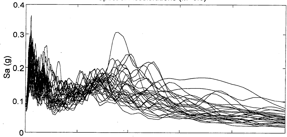
Black Diamond Road Spectral Accelerations (M=8.0)
