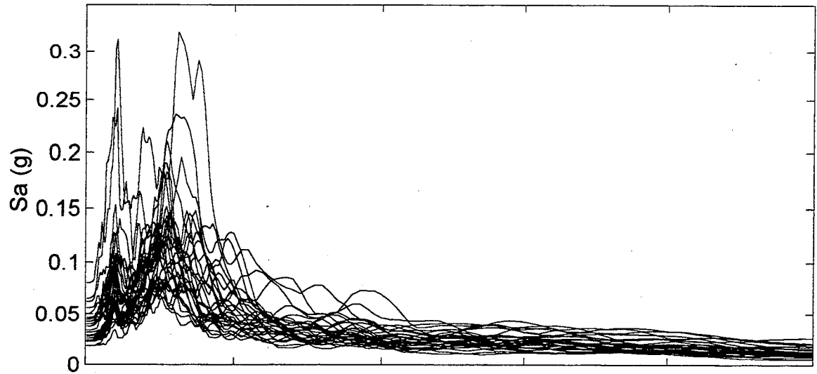
Coldwater Creek Spectral Accelerations (M=8.0)
