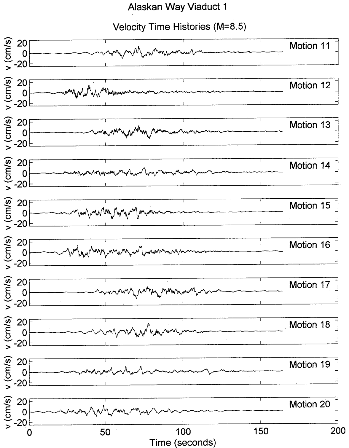
Figure 11. Computed time histories of rock outcrop velocity at Alaskan Way Viaduct site for M_w = 8.5 Cascadia subduction zone earthquake (continued).
