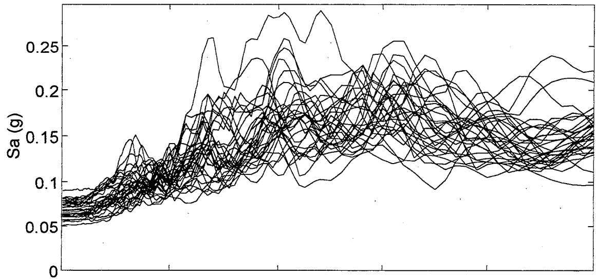
Mercer Slough 1 Spectral Accelerations (M=8.5)
