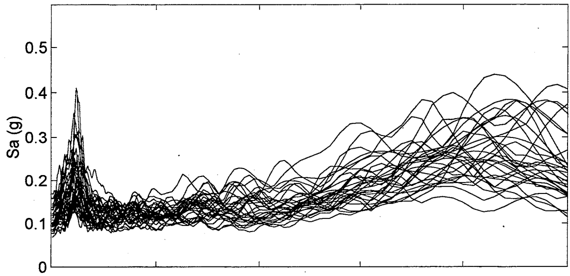
Bone River Spectral Accelerations (M=8.5)
