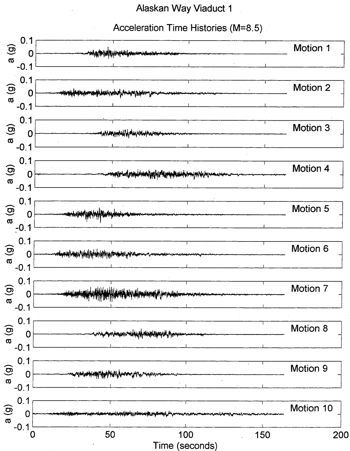
Figure 10. Computed time histories of rock outcrop acceleration at Alaskan Way Viaduct site for M_w = 8.5 Cascadia subduction zone earthquake.
