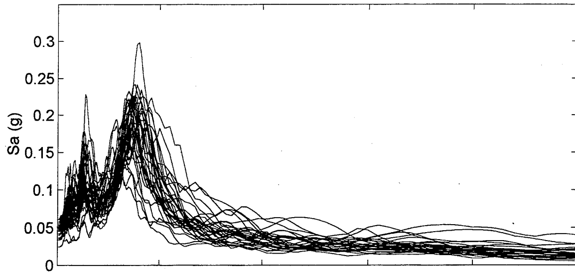
Coldwater Creek Spectral Accelerations (M=8.0)
