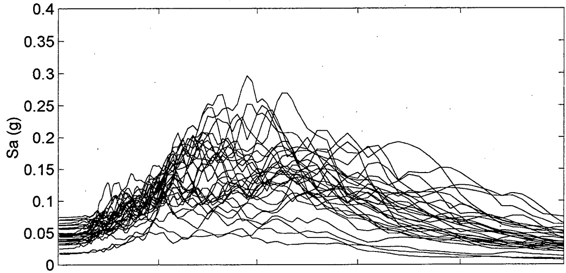
Nooksack River Spectral Accelerations (M=9.0)
