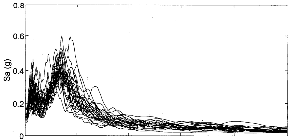
Andresen Road Spectral Accelerations (M=8.5)
