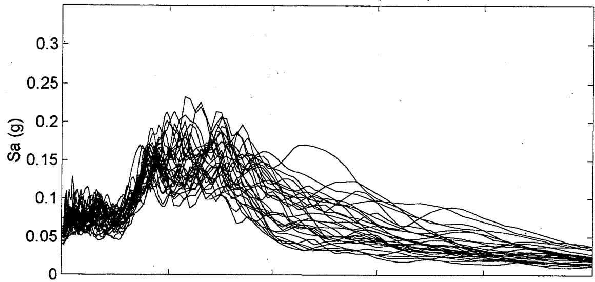
North Ferndale Spectral Accelerations (M=8.0)
