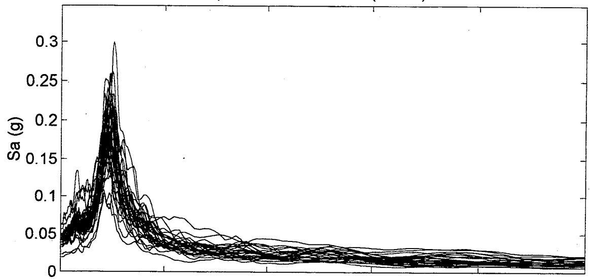
I-5/NE 99th Street Spectral Accelerations (M=8.0)
