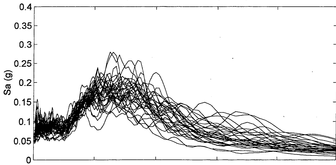
North Ferndale Spectral Accelerations (M=8.5)
