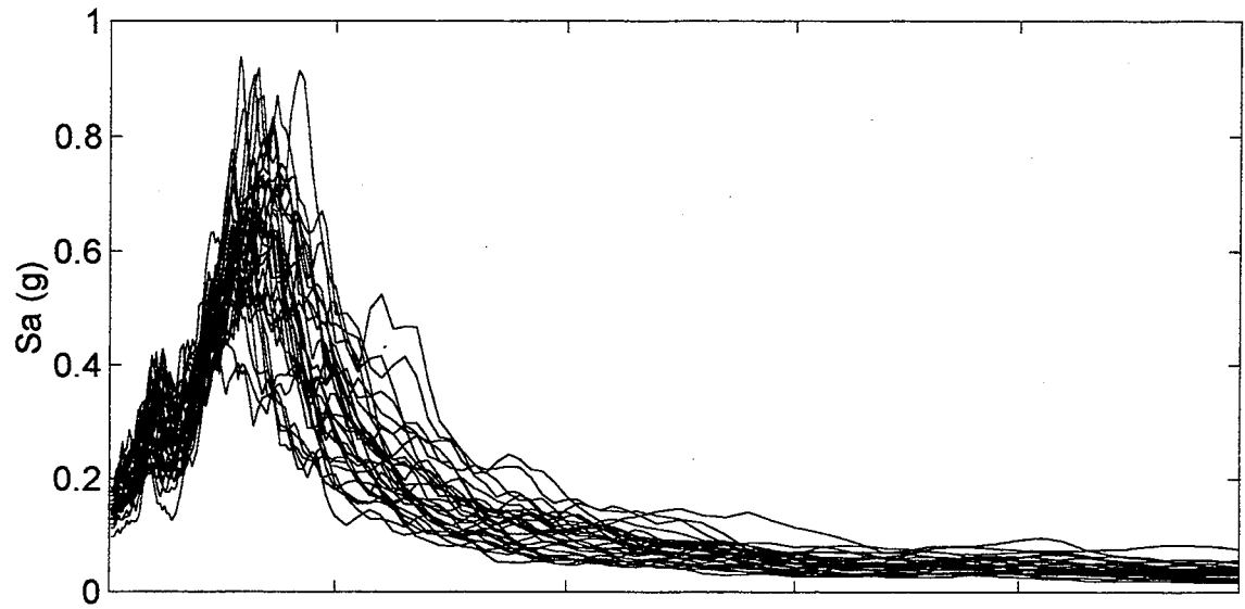
I-5/NE 99th Street Spectral Accelerations (M=9.0)
