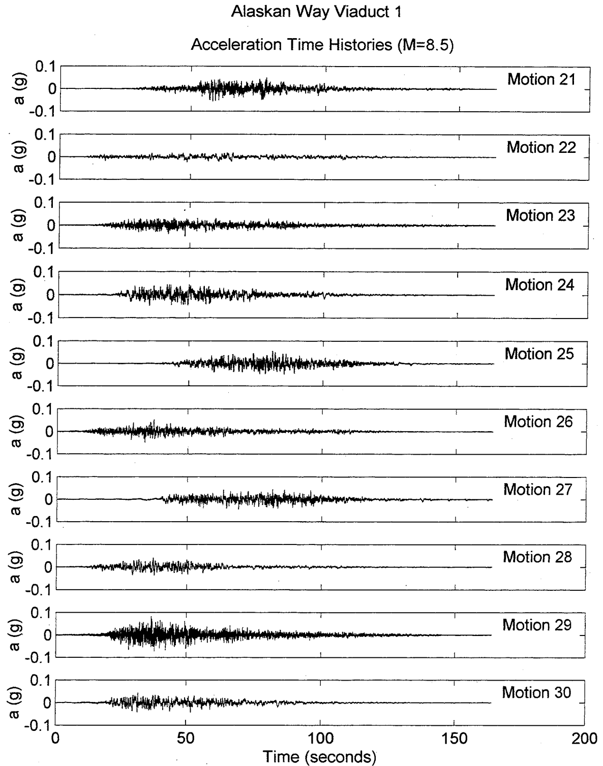
Figure 10. Computed time histories of rock outcrop acceleration at Alaskan Way Viaduct site for M_w = 8.5 Cascadia subduction zone earthquake (continued).
