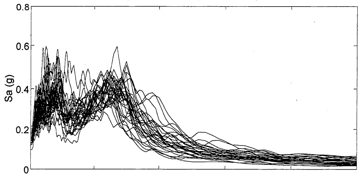
Capitol Boulevard Spectral Accelerations (M=9.0)
