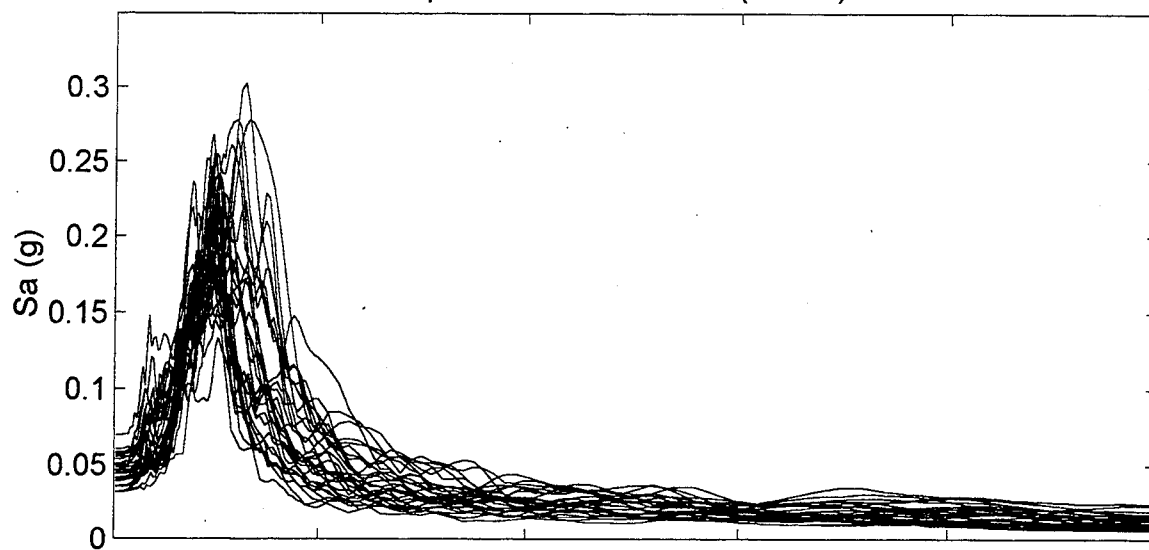
I-5/NE 99th Street Spectral Accelerations (M=8.0)
