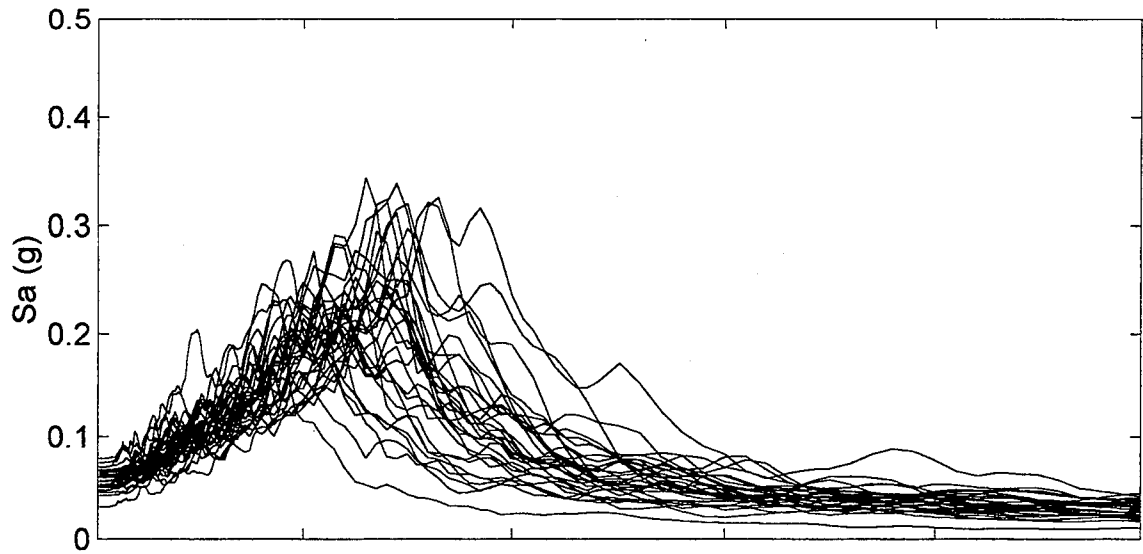
Alaskan Way Viaduct 2 Spectral Accelerations (M=9.0)
