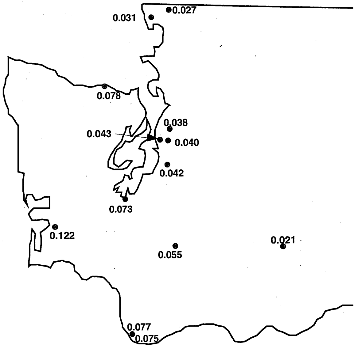
Figure 15. Computed median peak rock outcrop accelerations for M_w=9.0 earthquakes.
