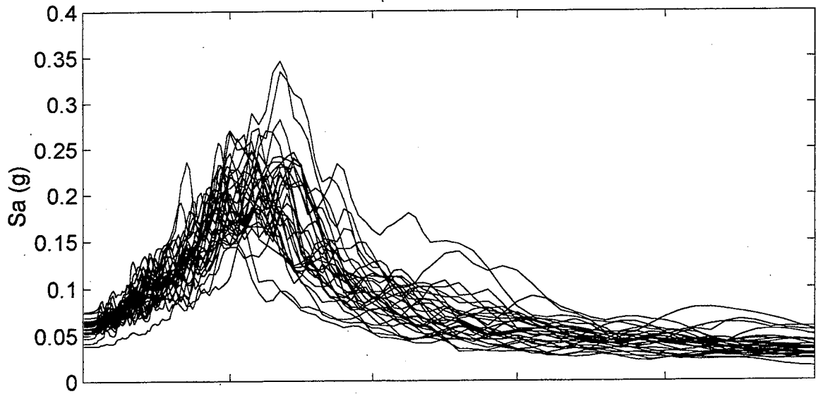
Alaskan Way Viaduct 2 Spectral Accelerations (M=8.5)
