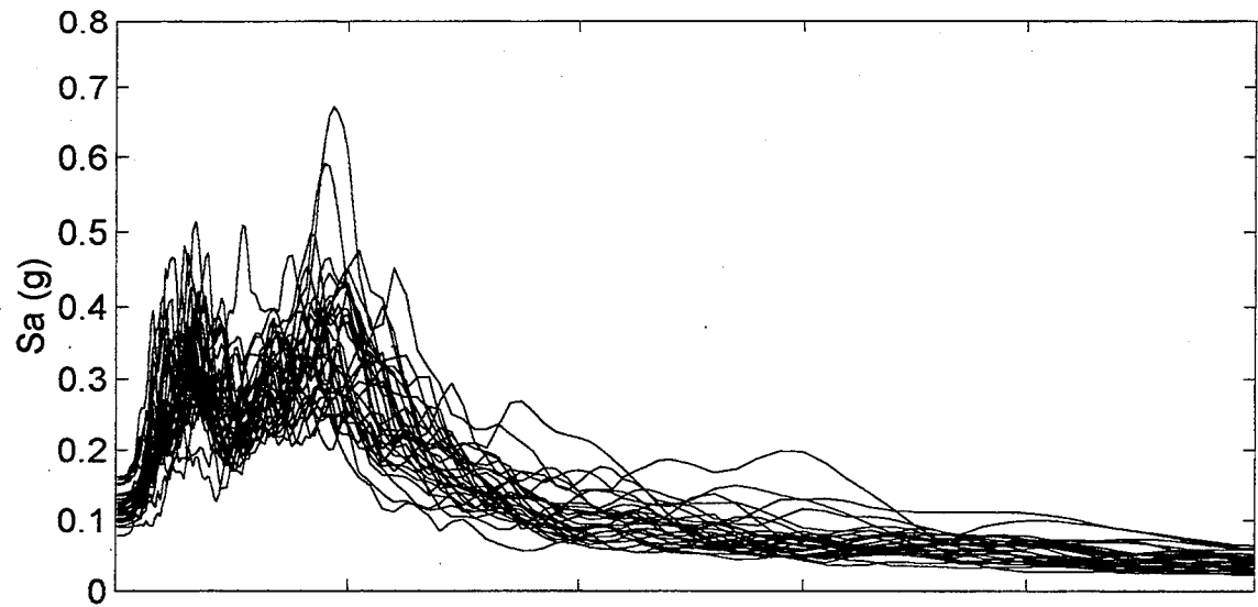
Capitol Boulevard Spectral Accelerations (M=8.5)
