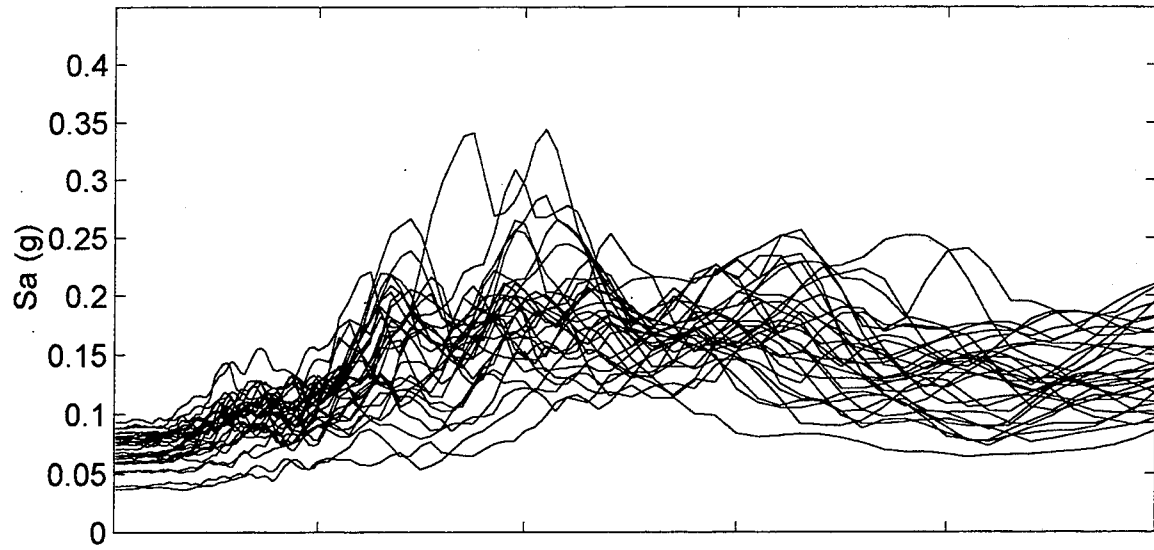
Mercer Slough 1 Spectral Accelerations (M=9.0)
