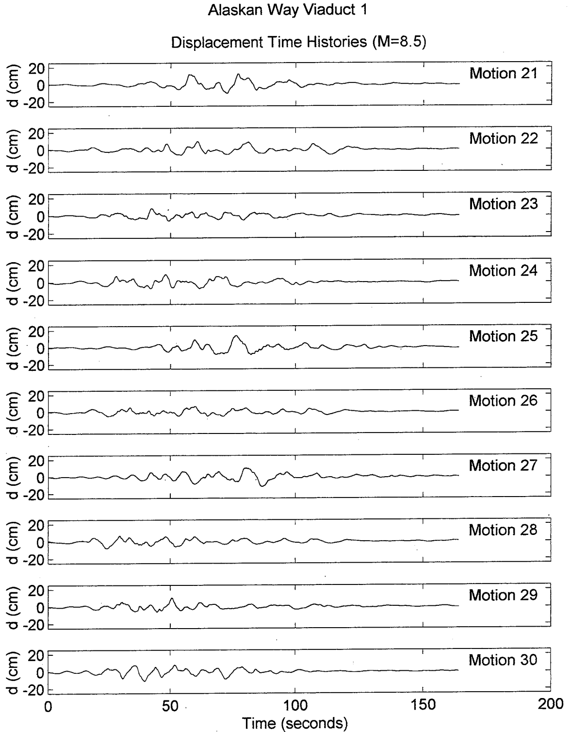
Figure 12. Computed time histories of rock outcrop displacement at Alaskan Way Viaduct site for M_w = 8.5 Cascadia subduction zone earthquake (continued).
