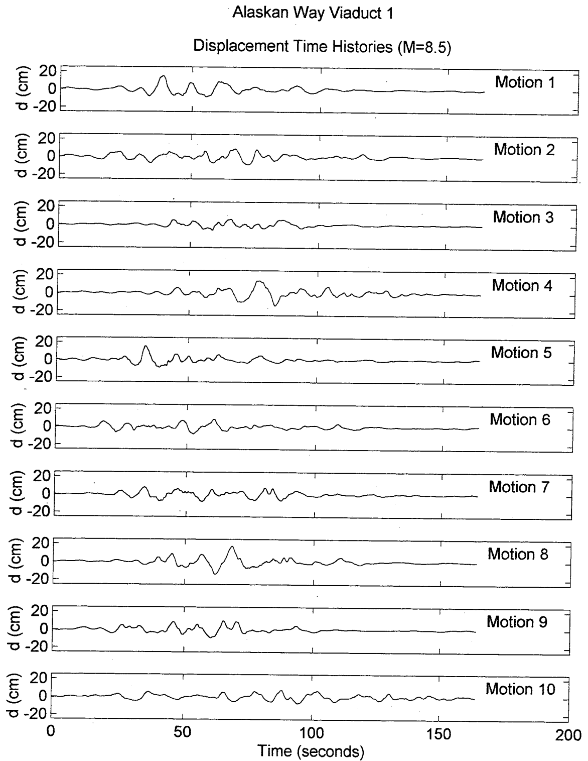
Figure 12. Computed time histories of rock outcrop displacement at Alaskan Way Viaduct site for M_w = 8.5 Cascadia subduction zone earthquake.
