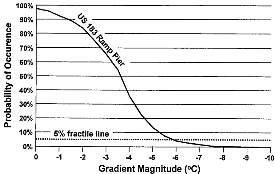
Figure 2.16: Probability of negative gradients in substructure.
