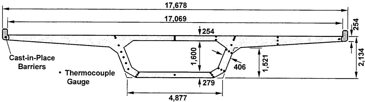
Figure 2.3: Cross-section and instrumentation for Span D6 of the US 183 Mainlane.
