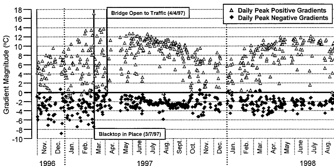
Figure 2.6: US 183 Ramp P daily maximum gradient data.
