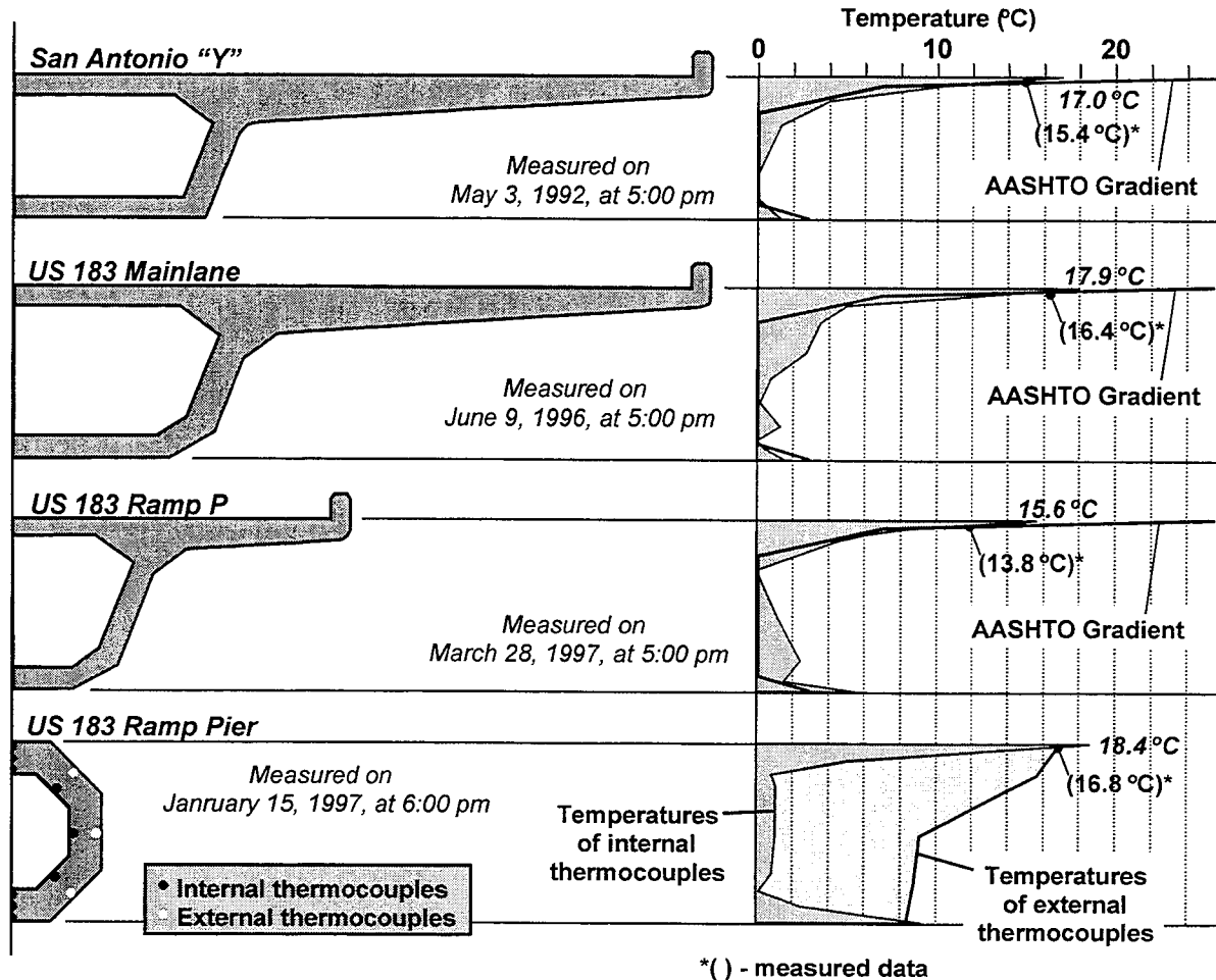
Figure 2.9: Maximum positive gradient shapes.
