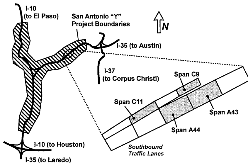
Figure 1.1: Project 0-1234 field instrumentation locations (San Antonio, TX).
