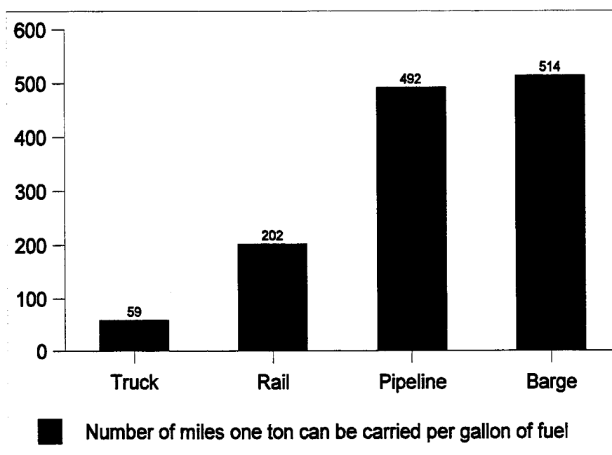
FIGURE 2.4 Relative Energy Efficiencies
