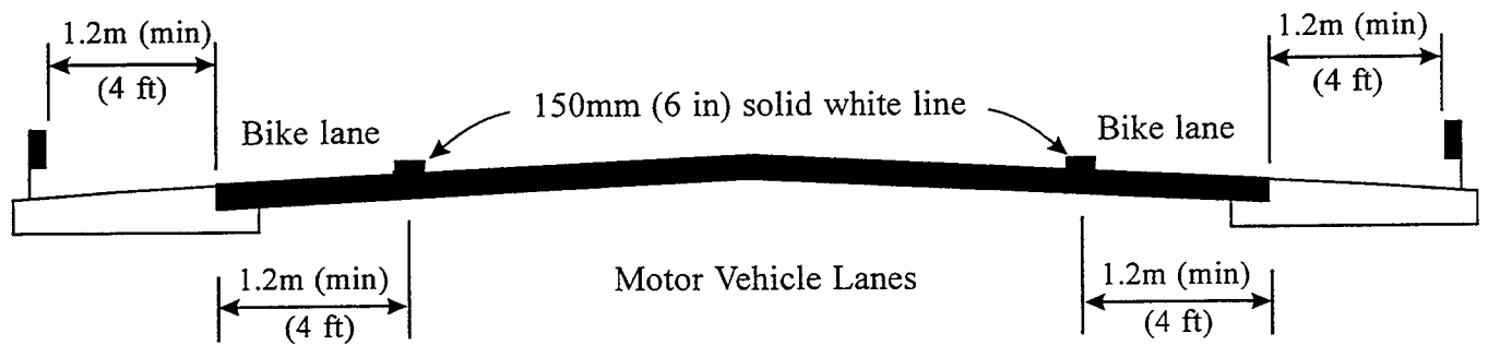
Figure 10. Examples of Bike Lanes on Rural Roadway
