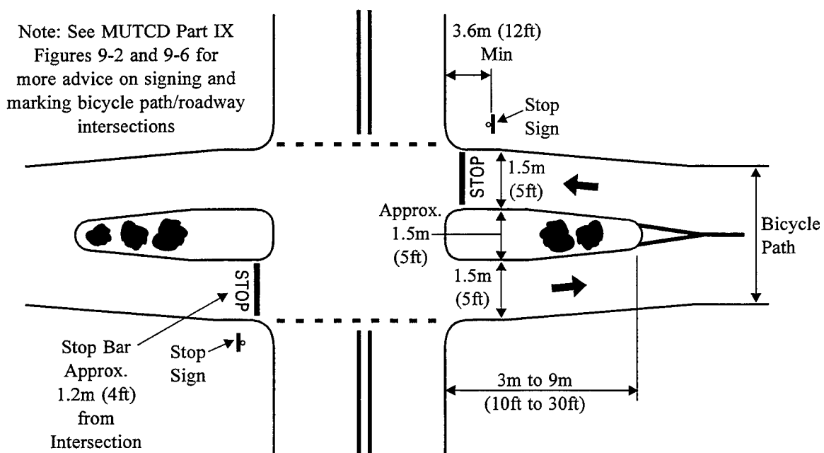
Figure 31. Reflectorized Post to Restrict Motor Vehicles from Bicycle Paths
