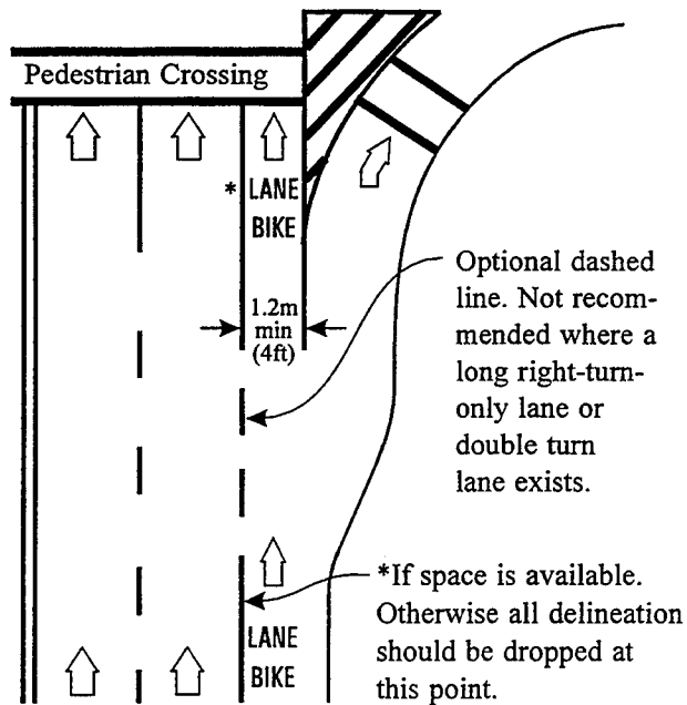
(1) Right-turn-only lane
