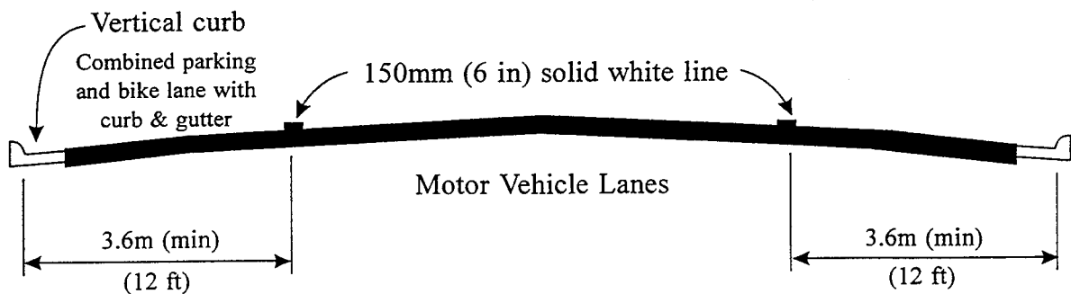
Figure 12. Example of Shared Bike and On-Street Parking Lanes
