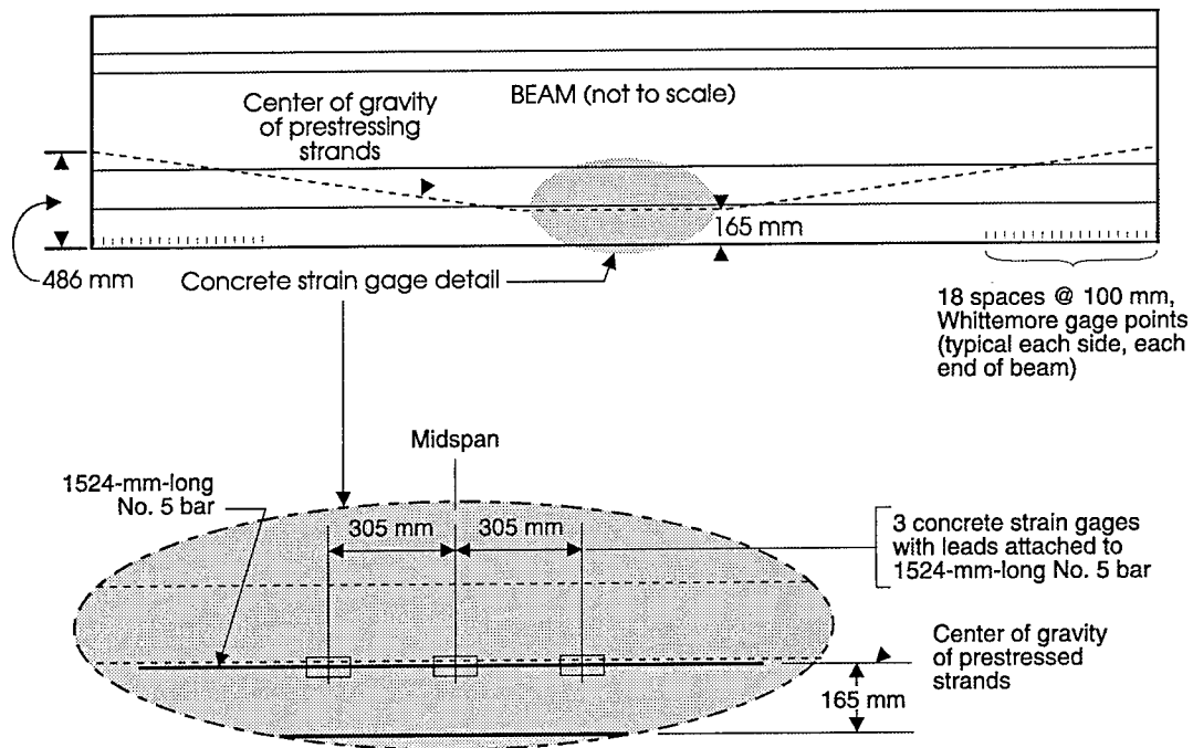
Figure 26. Location of Strain Gages
