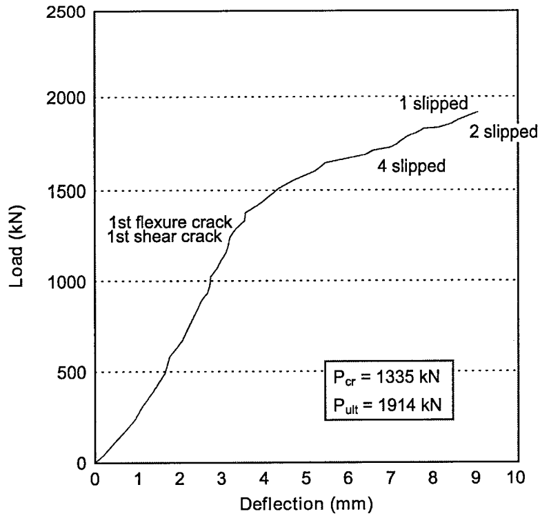
Figure 17. Load Versus Midspan Deflection for Test Beam 1, End A
