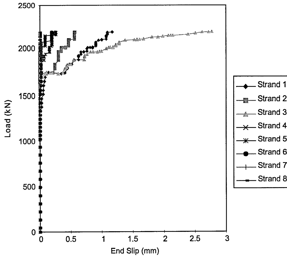
Figure 22. End Slip Versus Load for Test Beam 2, End A
