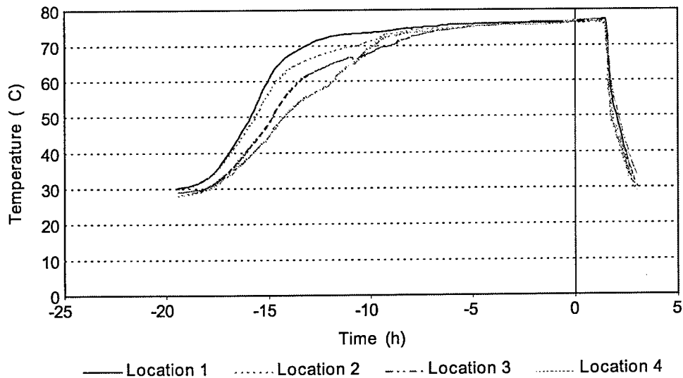
Figure 29. Temperature Versus Time for Beam 1
