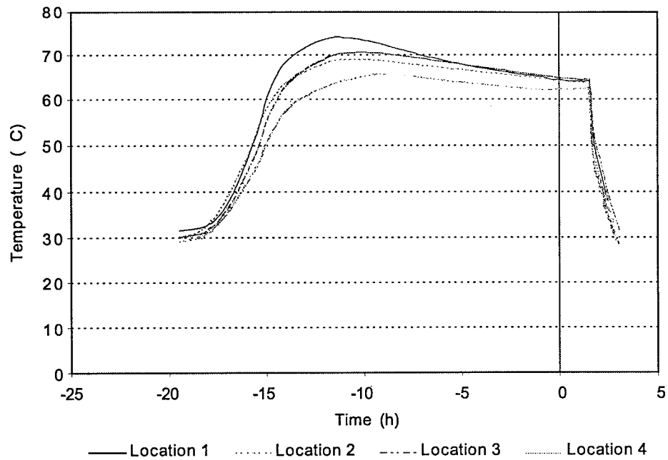
Figure 30. Temperature Versus Time for Beam 2
