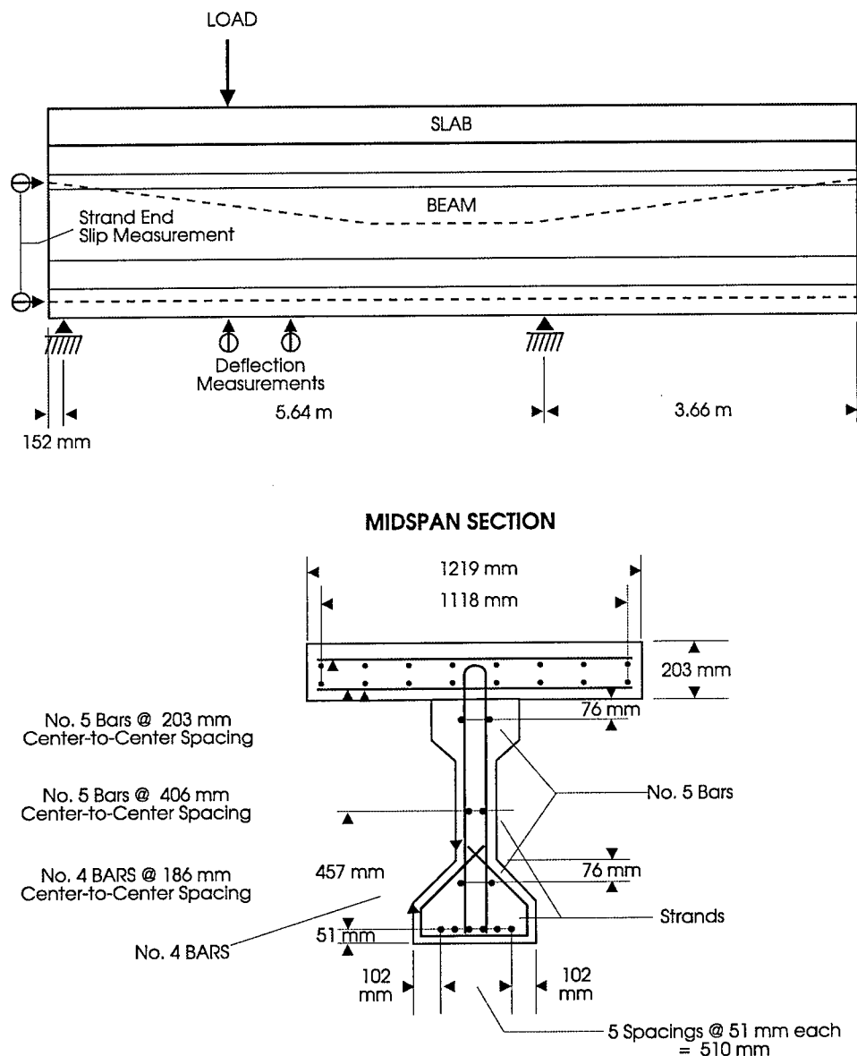
Figure 2. Test Beam and Laboratory Setup
