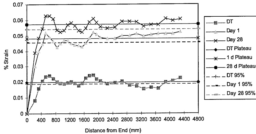
Figure 12. Concrete Surface Strain for Transfer Length Determination of Test Beam 2, End A
