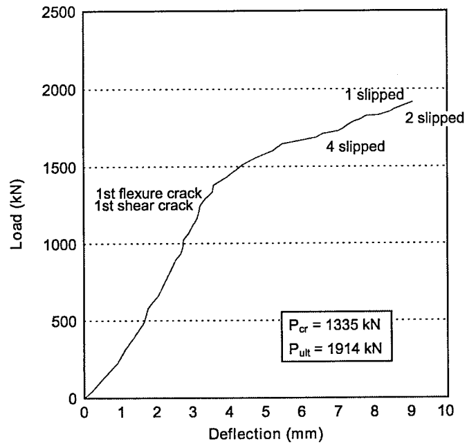
Figure 16. Load Versus Midspan Deflection for Test Beam 1, End B
