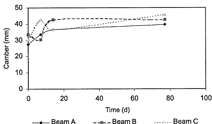
Figure 35. Midspan Camber Versus Time
