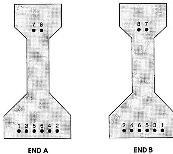
Figure 14. Strand Notation for End Slip
