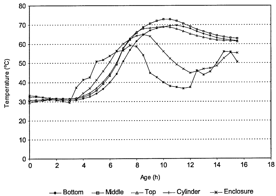
Figure 6. Temperature Development in Test Beam 2
