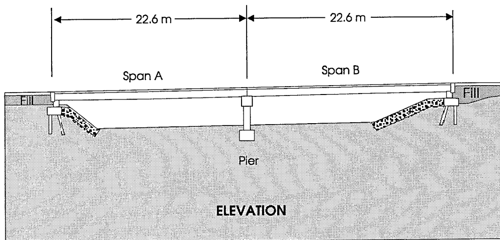
Figure 23. Elevation View of Bridge
