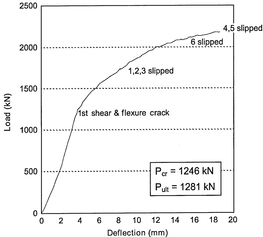
Figure 19. Load Versus Midspan Deflection for Test Beam 2, End A
