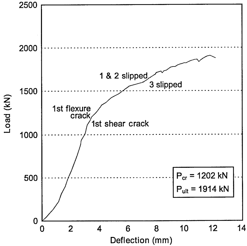
Figure 18. Load Versus Midspan Deflection for Test Beam 2, End B
