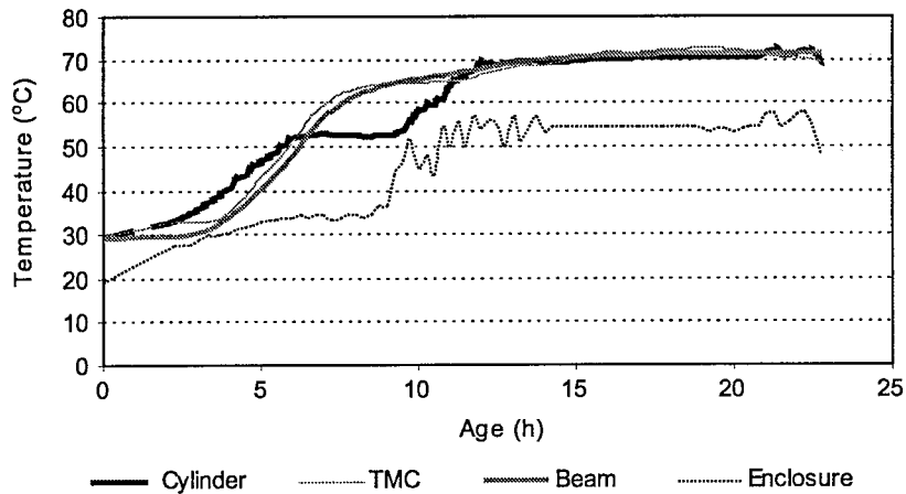
Figure 27. Temperature Development in Bridge Beam
