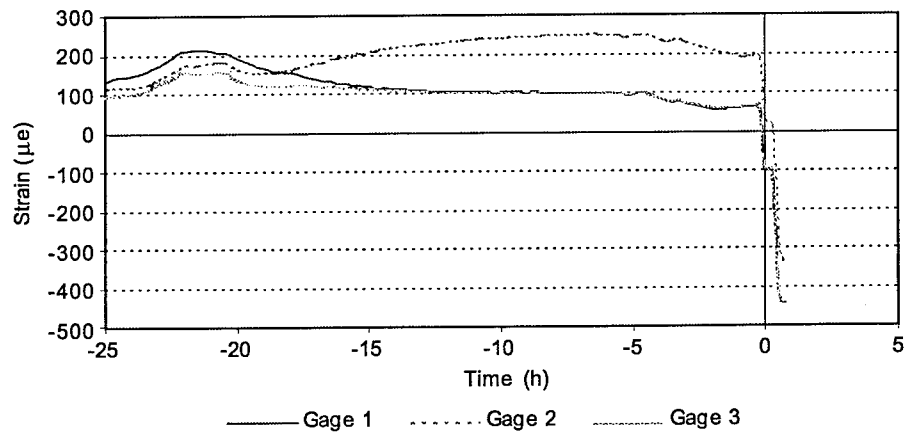
Figure 34. Strain Versus Time for Beam 3
