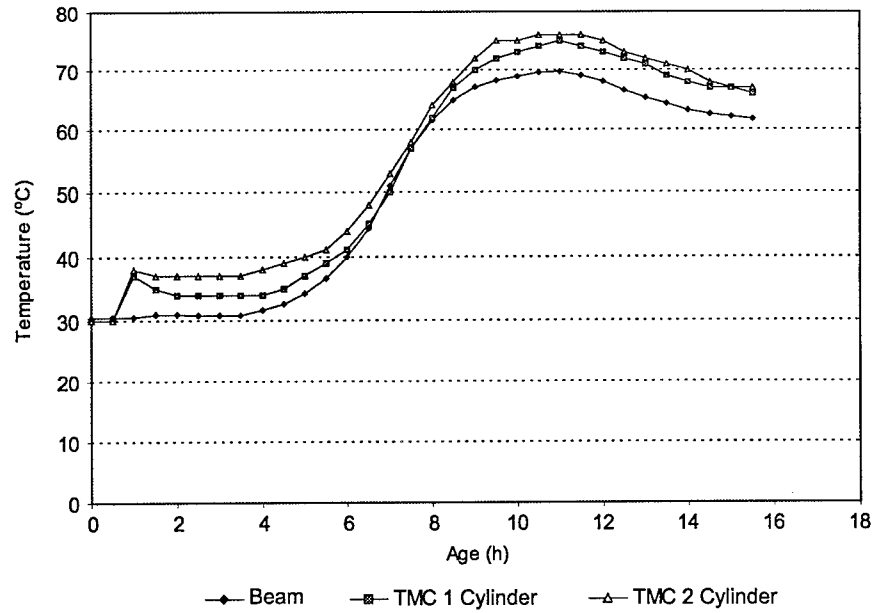
Figure 7. Temperature Development in TMC Cylinders
