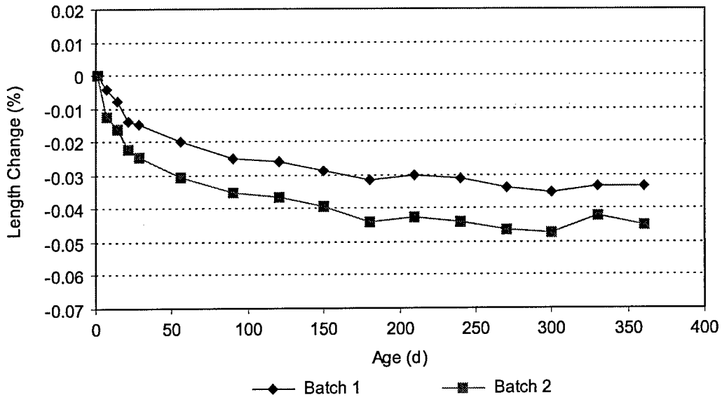
Figure 28. Length Change Data
