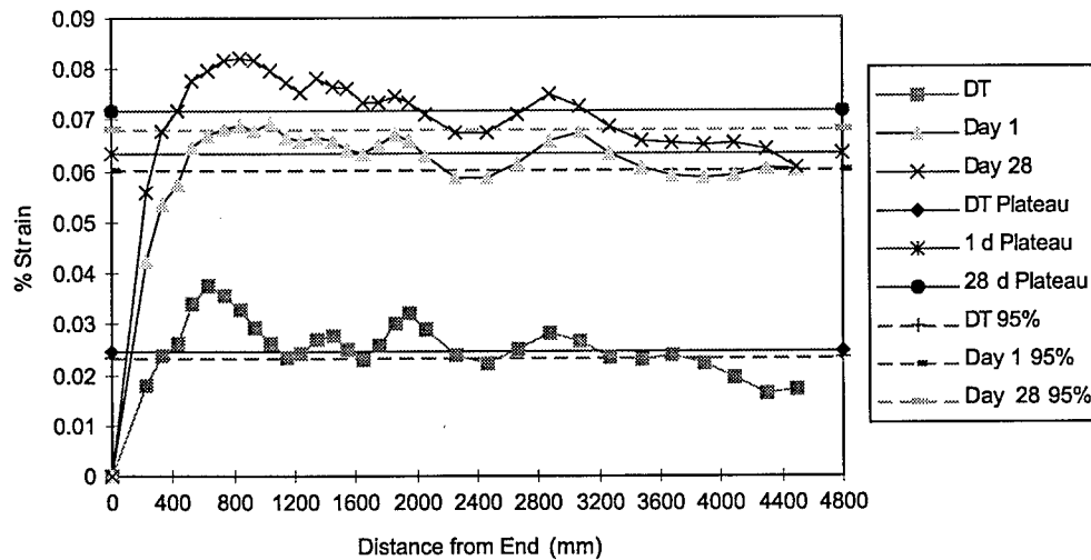
Figure 10. Concrete Surface Strain for Transfer length Determination of Test Beam 1, End A
