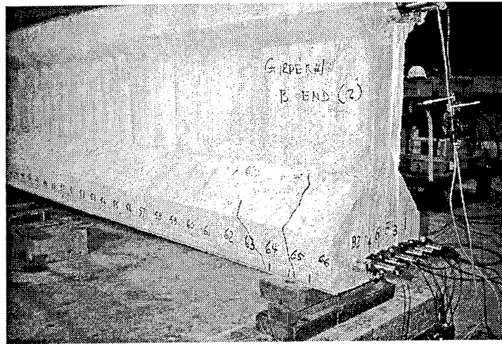
Figure 4. Measurement of End Slippage by LVDTs
