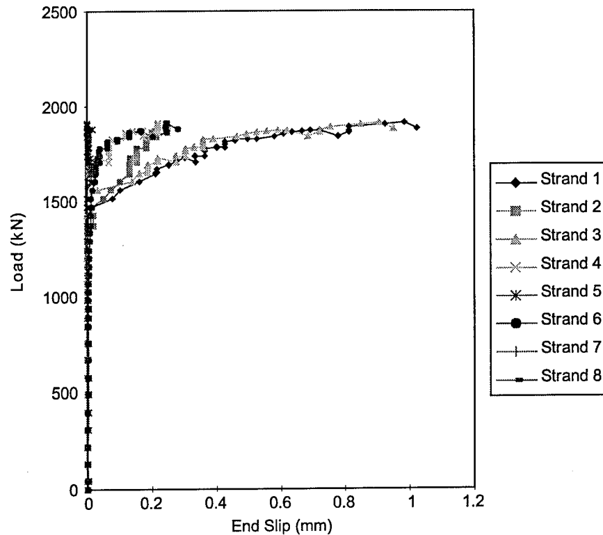
Figure 21. End Slip Versus Load for Test Beam 2, End B
