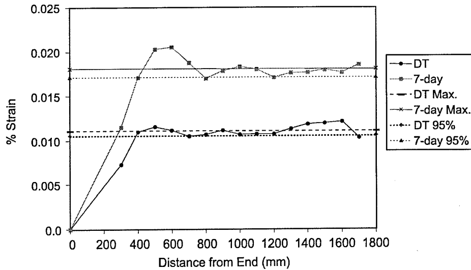
Figure 36. Concrete Surface Strain for Transfer length Determination of Beam 1
