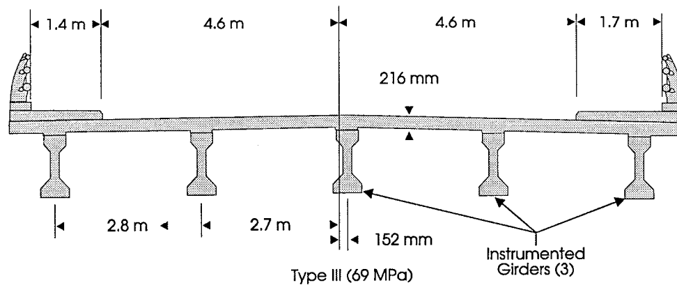
TRANSVERSE SECTION
