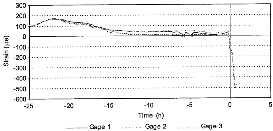
Figure 33. Strain Versus Time for Beam 2
