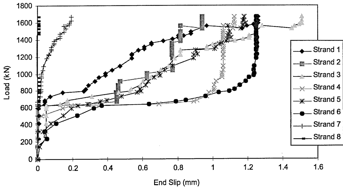
Figure 15. End Slip Versus Load for Test Beam 1, End B
