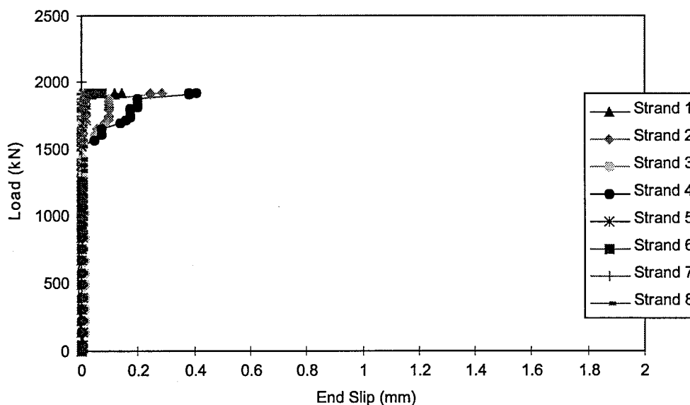
Figure 20. End Slip Versus Load for Test Beam 1, End A
