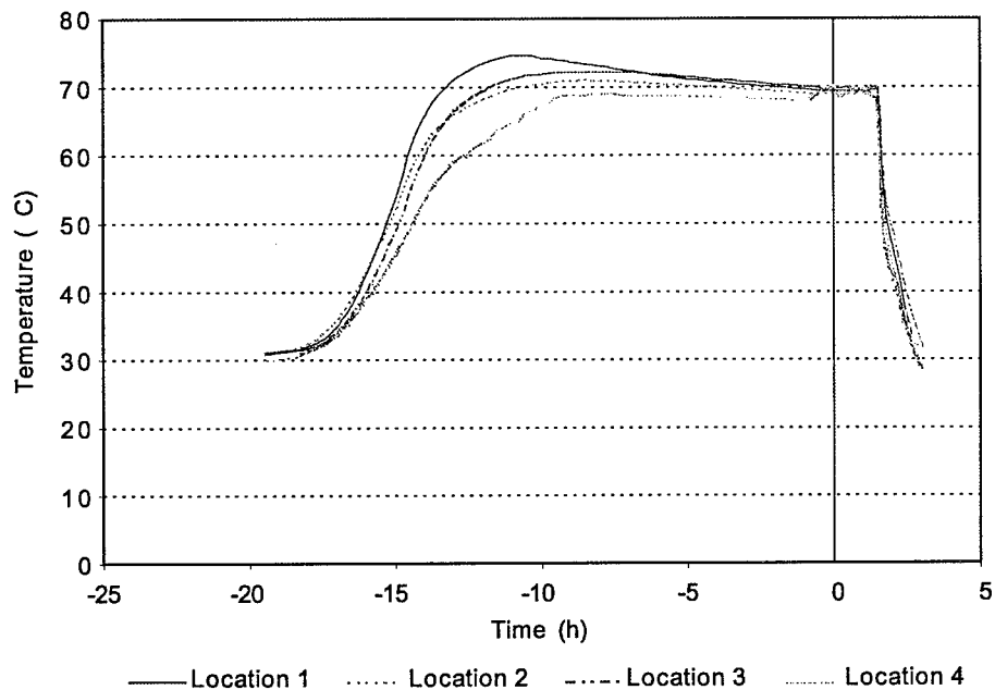
Figure 31. Temperature Versus Time for Beam 3
