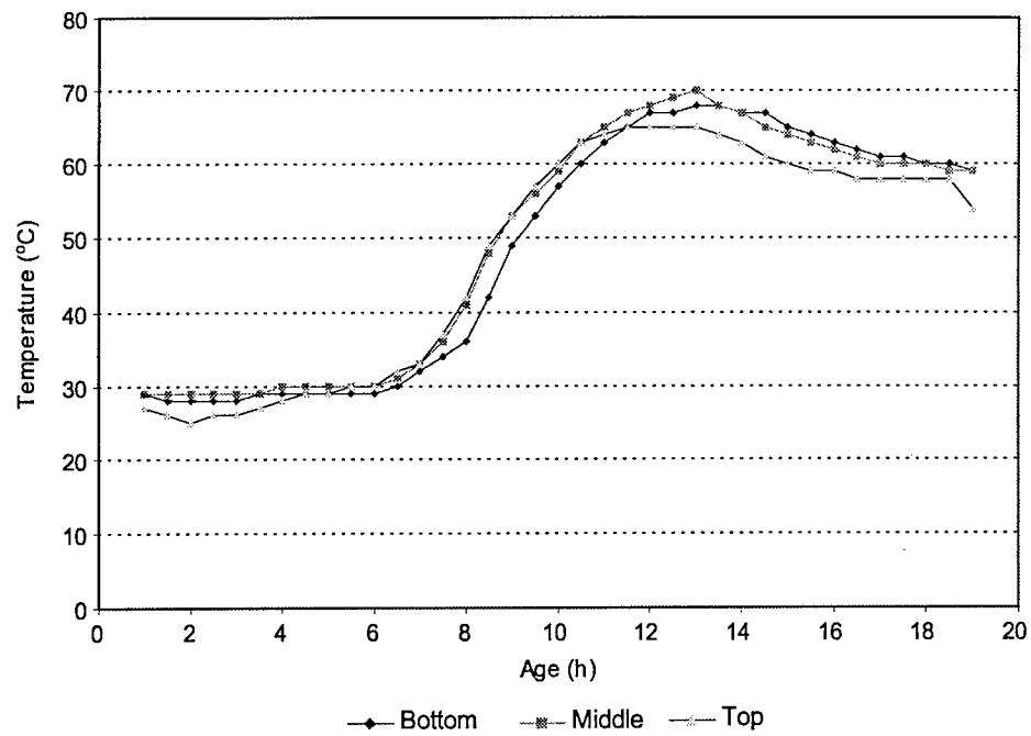
Figure 5. Temperature Development in Test Beam 1
