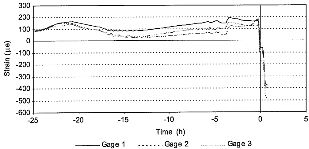
Figure 32. Strain Versus Time for Beam 1
