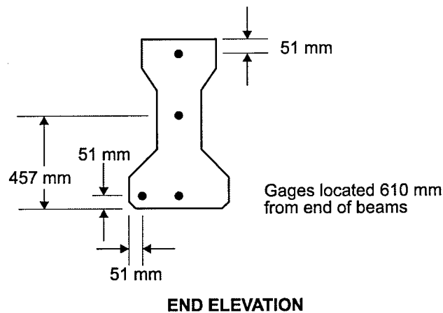
Figure 3. Location of Temperature Gages in Test Beams
