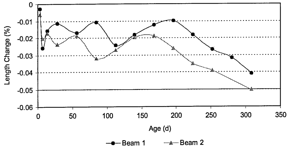
Figure 8. Length Change Data for Test Beams
