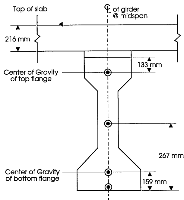
Figure 25. Locations of Thermocouples
