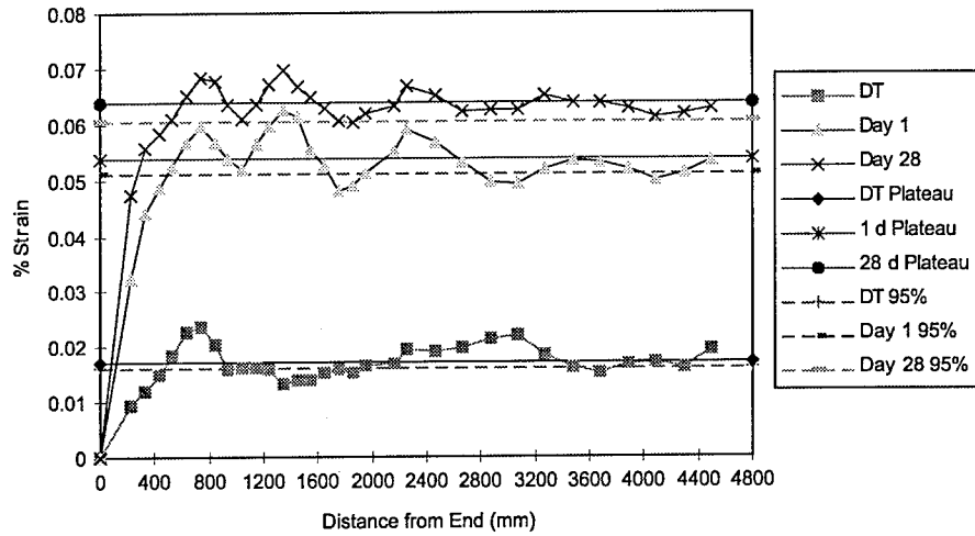
Figure 11. Concrete Surface Strain for Transfer length Determination of Test Beam 1, End B
