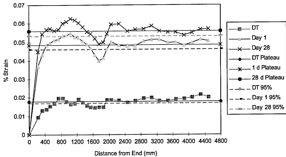
Figure 13. Concrete Surface Strain for Transfer Length Determination of Test Beam 2, End B
