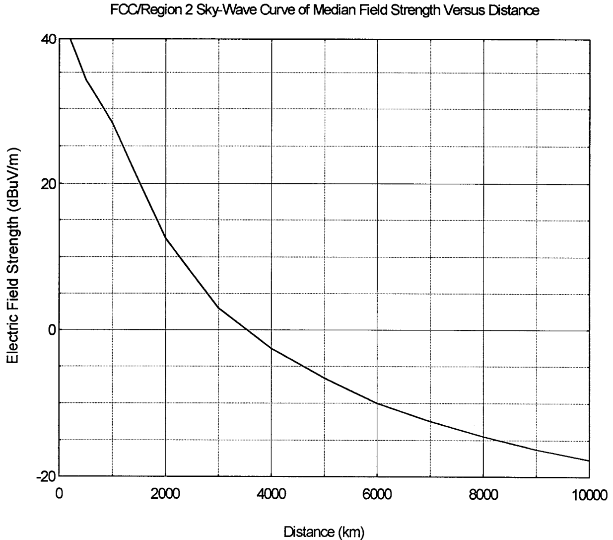
Figure 5. FCC/Region 2 sky-wave curve of median field strength versus distance.
