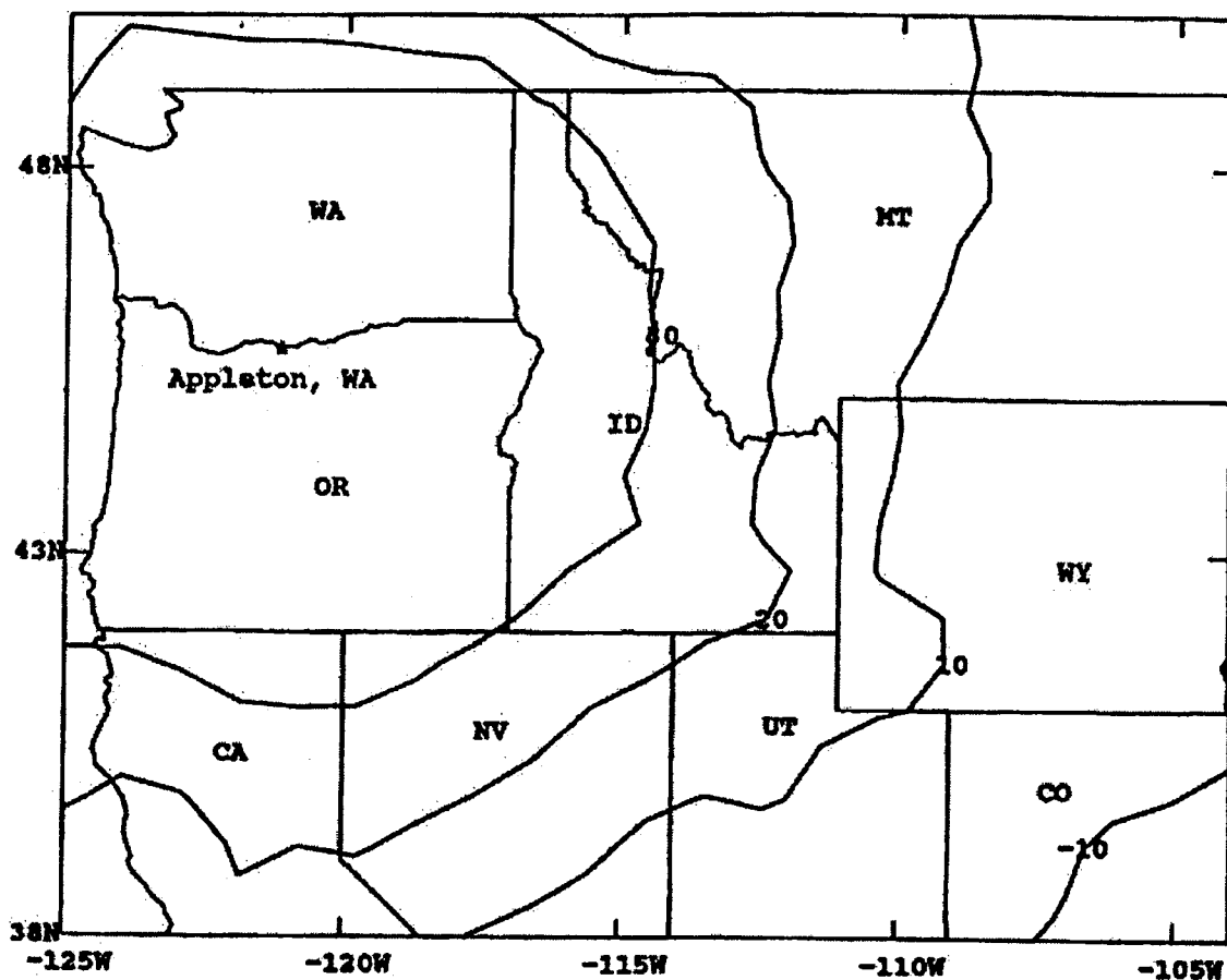
Figure 30. Contours of electric-field strength in dBuV/m from the Appleton, WA DGPS site at daytime ( f=300 kHz).
