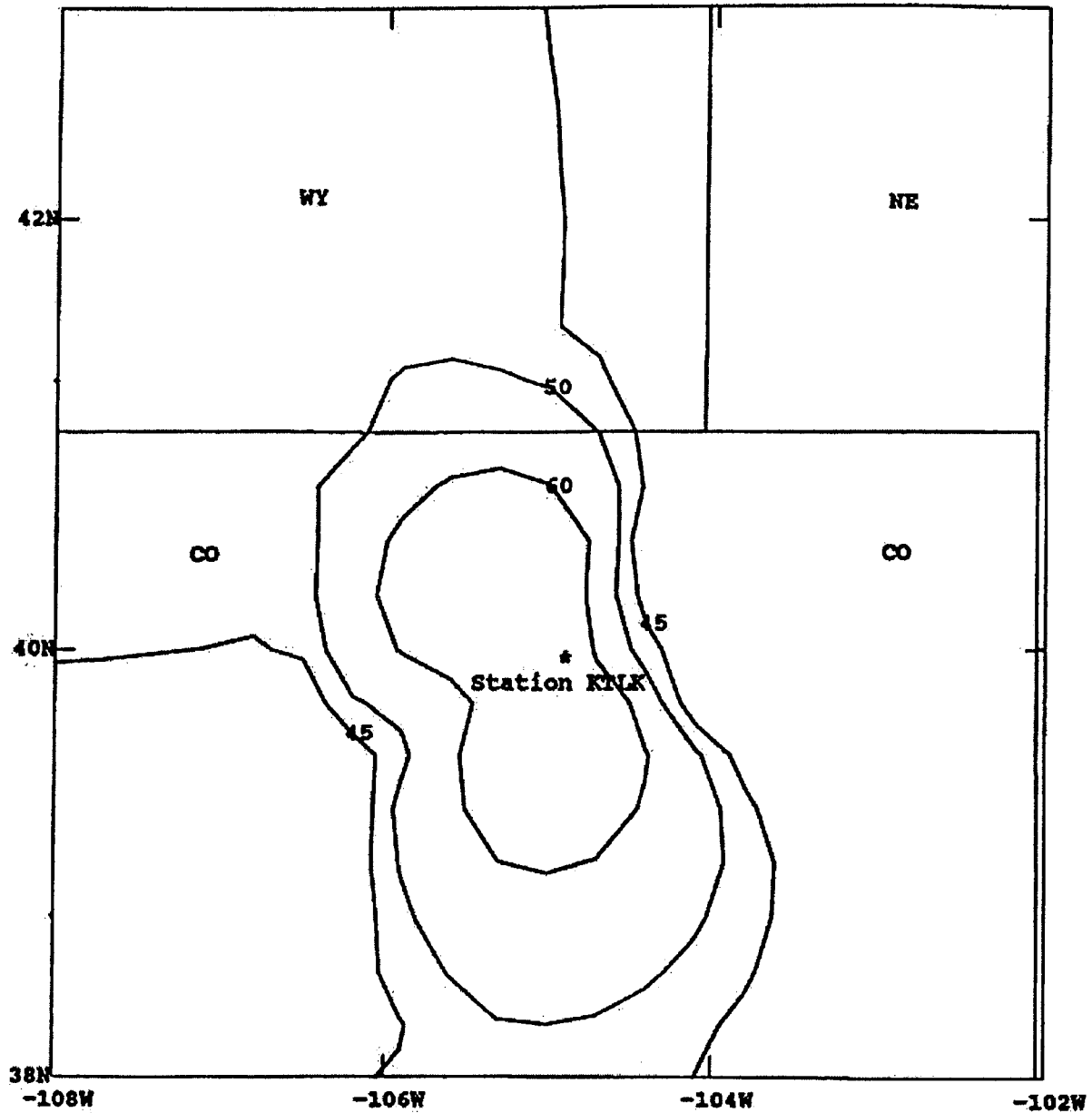
Figure 21. Predicted night coverage contours (dBuV/m) using the smooth-Earth mixed-path model.
