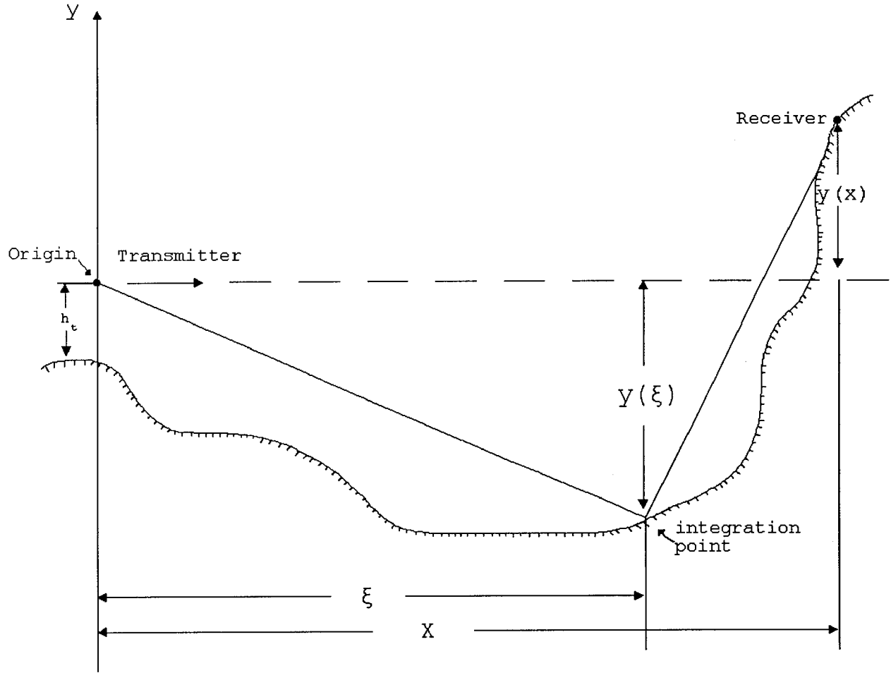
Figure 3. Geometry for integral equation irregular-Earth model along the great circle path.
