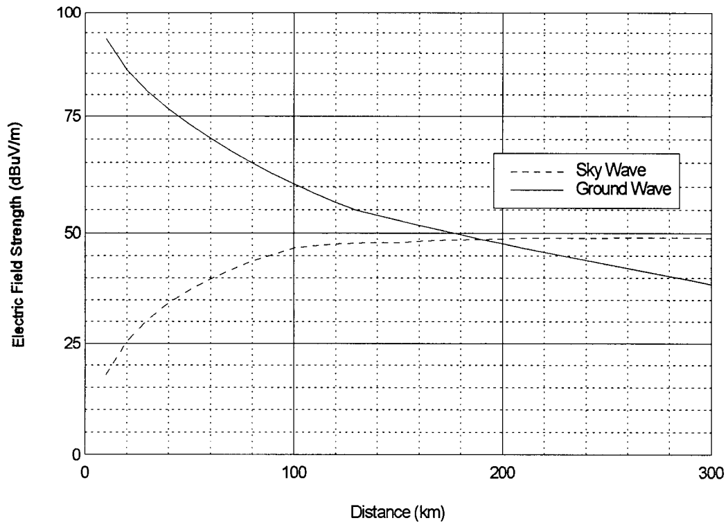
Figure 23. Electric field strength vs distance from station KTLK at nighttime on 330 degree radial using the smooth-Earth mixed-path model.
