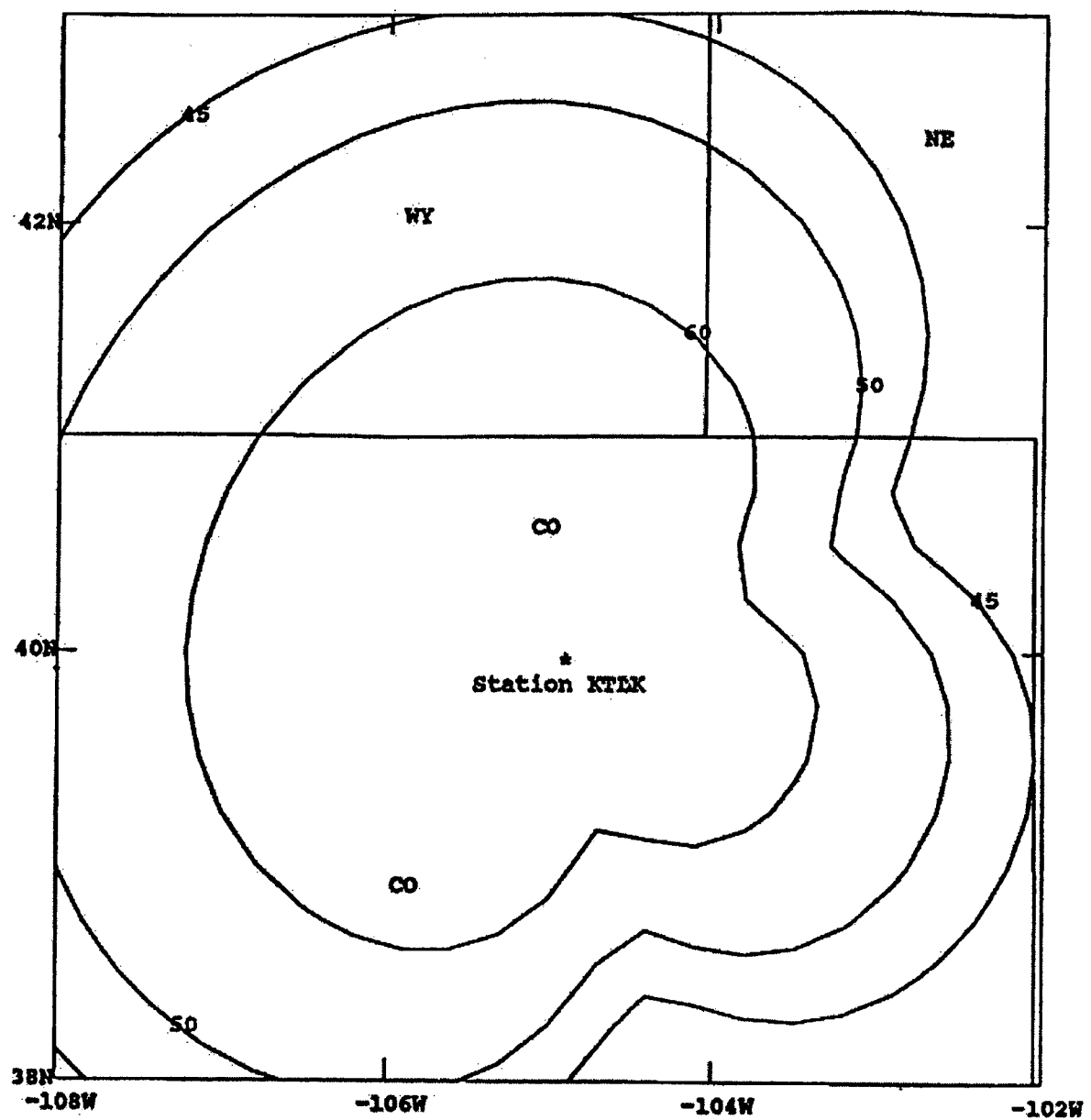
Figure 18. Predicted KTLK day coverage contours (dBuV/m) using the smooth-Earth model.
