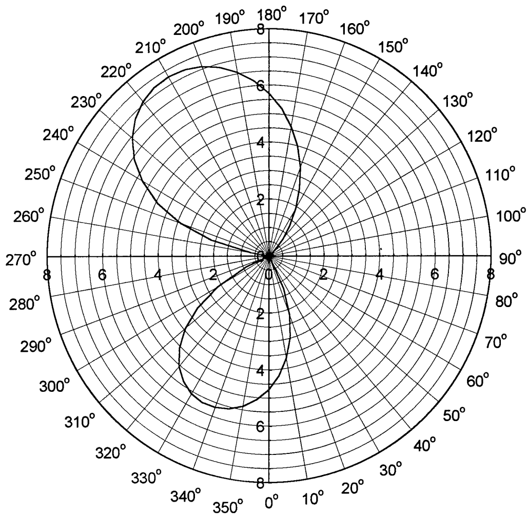
Figure 14. Equivalent gain antenna pattern for station KTLK nighttime antenna configuration versus azimuth angle for average ground conditions at 760 kHz.
