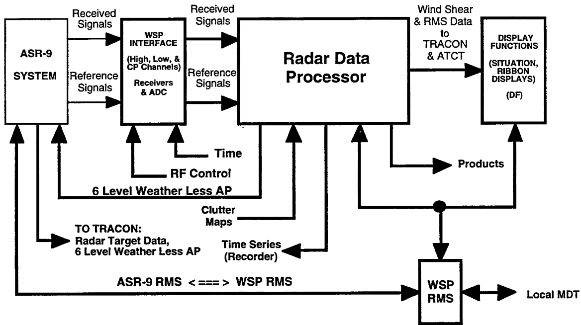
Figure 7. ASR-9 and WSP High Level Block Diagram.
