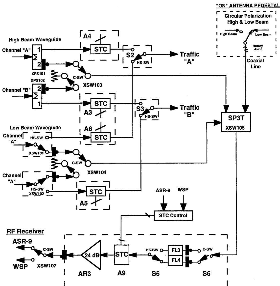
Figure 10. Simplified Waveguide Assembly Line Drawing.
