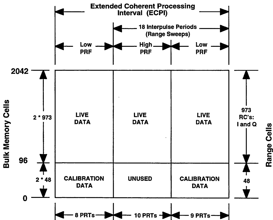
MODIFIED FOR WSP Bulk Memory Data Diagram TI 6310.28 (01 Dec. 90) pg 2-151
