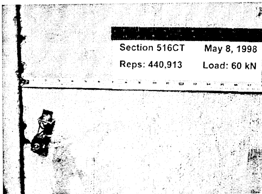
Figure 18b. Crack Activity Meter (CAM) overhead view.
