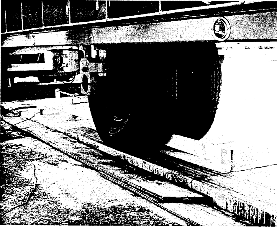
Figure 19. Road Surface Deflectometer.
