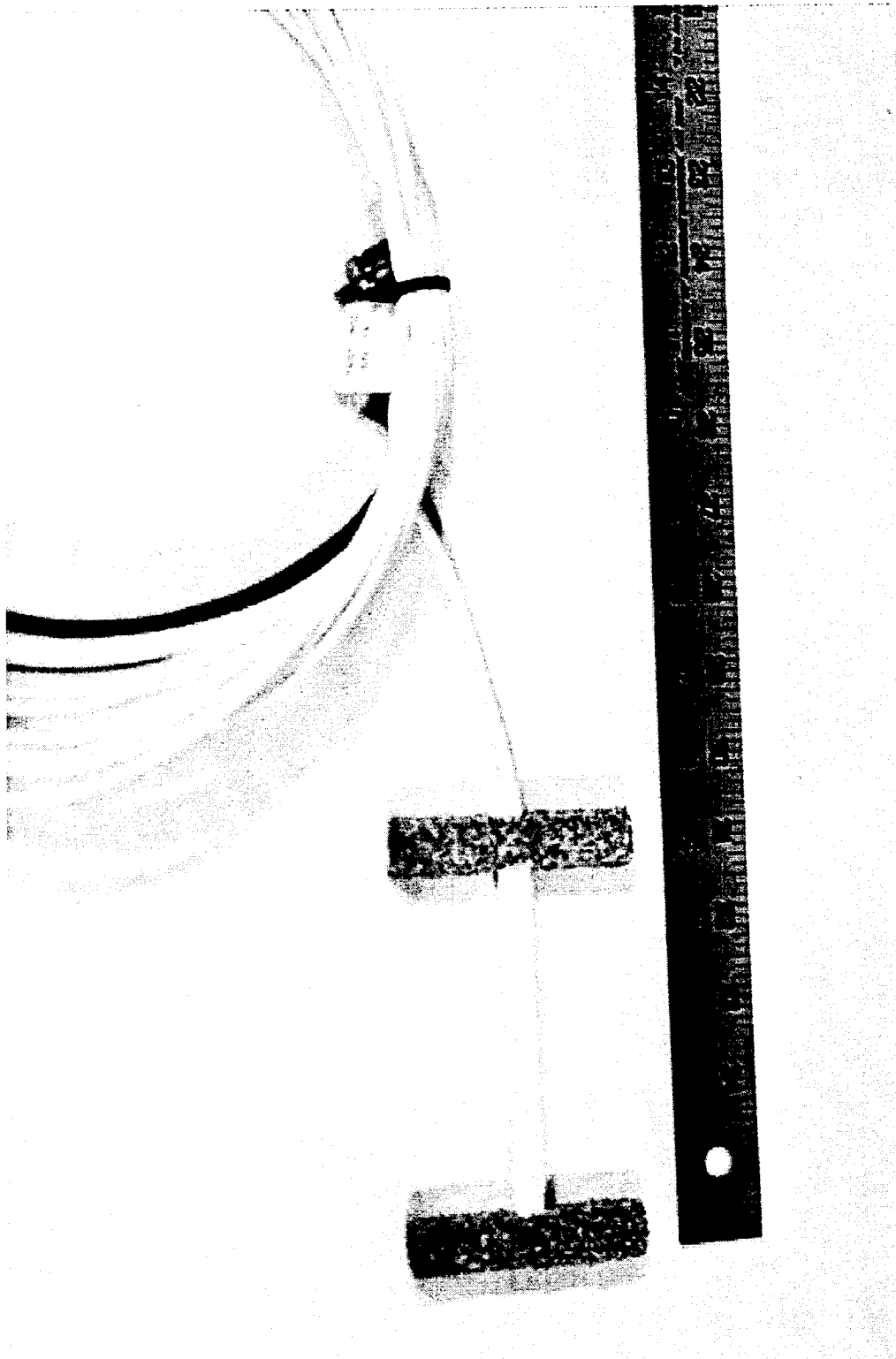
Figure 15. Dynatest PAST-2PCC strain gage.
