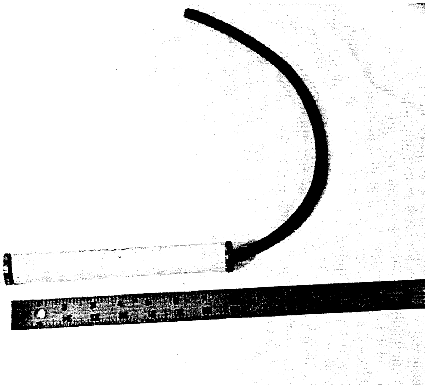
Figure 17. Carlson A-8 strain meter.
