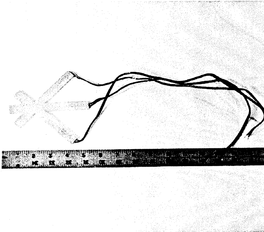
Figure 16. Tokyo Sokki PMR-60-6L strain gage.
