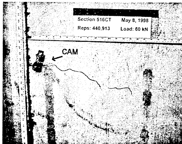
Figure 40a. Crack growth on 516CT at 440,913 repetitions. (Crack line has been enhanced for easier viewing.)
