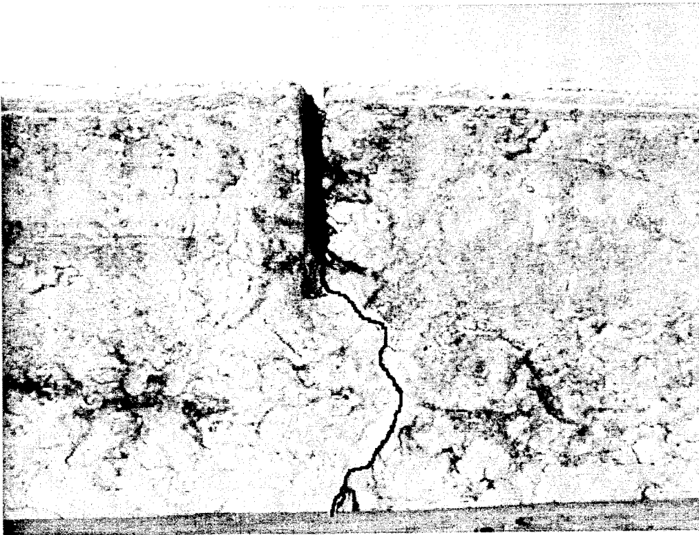
Figure 47b: Photo of Joint 2. Joint crack is enhanced for easier viewing.
