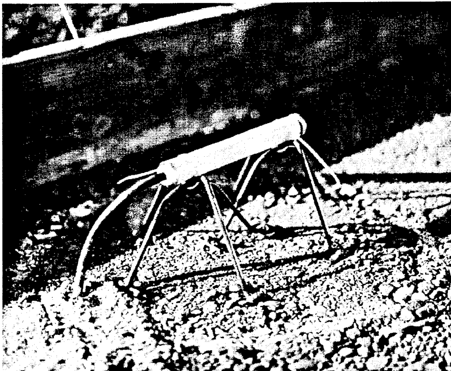
Figure 21a. Carlson A-8 strain meter on its cradle to maintain gage height and orientation during concrete placement.
