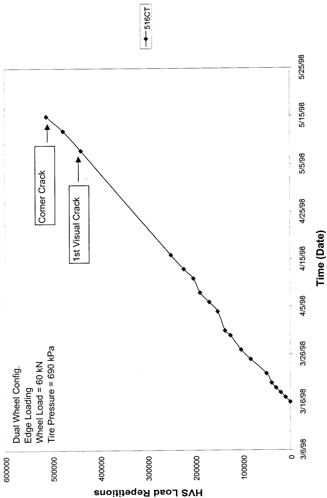
Figure 53. Richmond Field Station concrete test Section 516CT load repetitions versus time.
