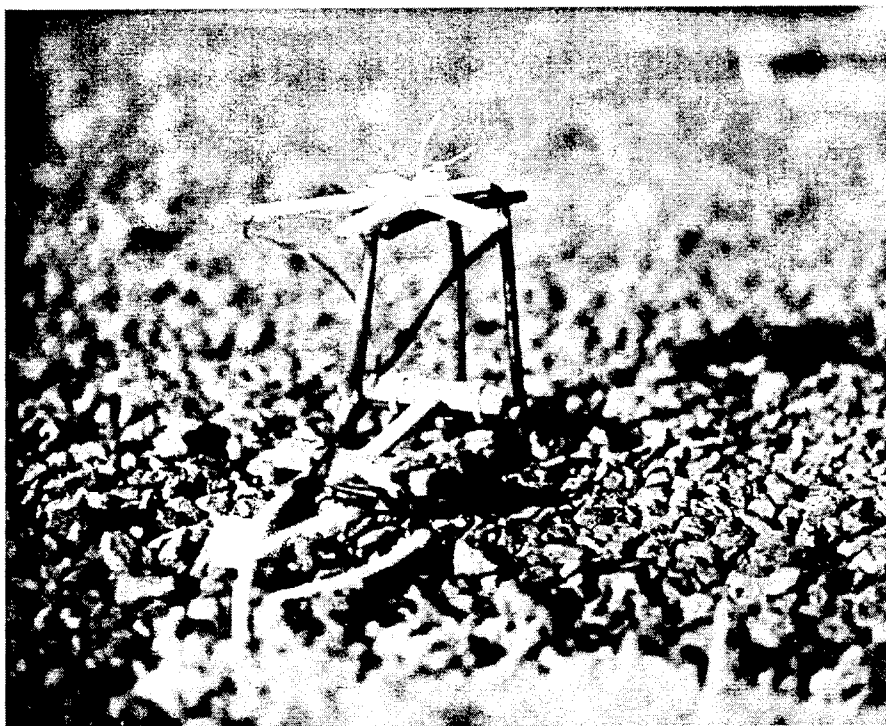
Figure 21b. Tokyo Sokki PMR-60-6L (top) and Dynatest PAST-2PCC (bottom) on cradle to maintain gage height and orientation during concrete placement.
