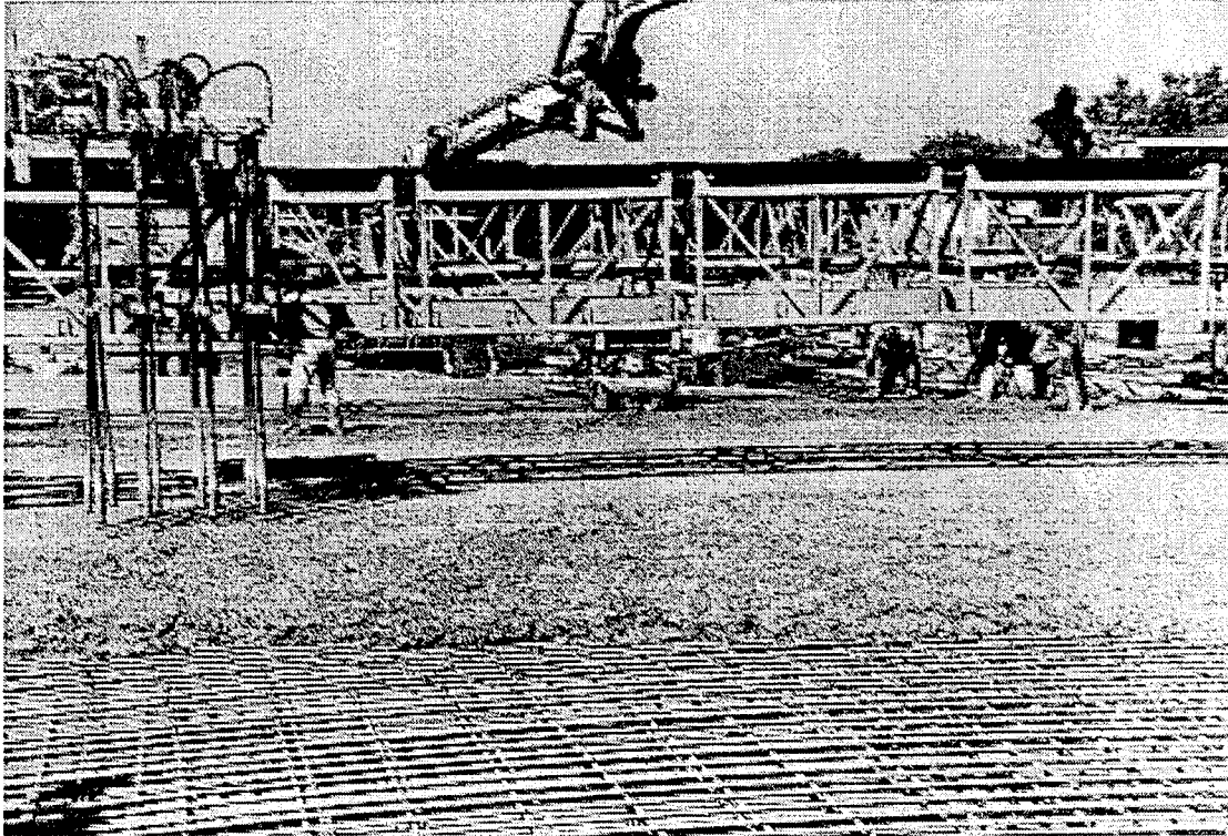
Figure 2. Four by four grid pattern device used on I-80 EB over NS RR in District 1.
