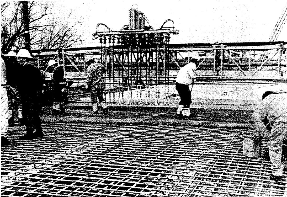
Figure 3. Two by eight grid pattern device with finishing carriage on same machine. This device was typically used for most subsequent grid vibration. Photo is actually from OR 66 bridge in District 3.
