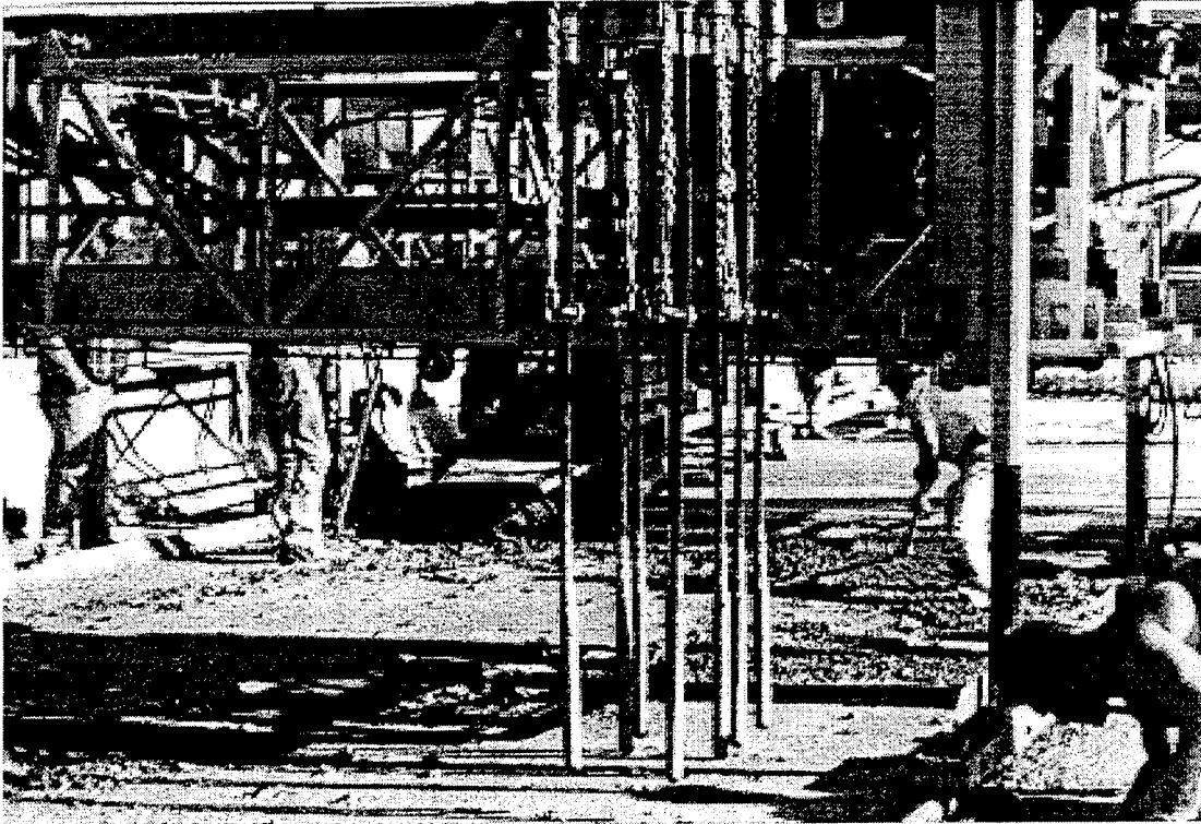
Figure 1. Two by four grid pattern vibration machine used for Stage I on I-57 southbound over EJ&E RR in District 1.
