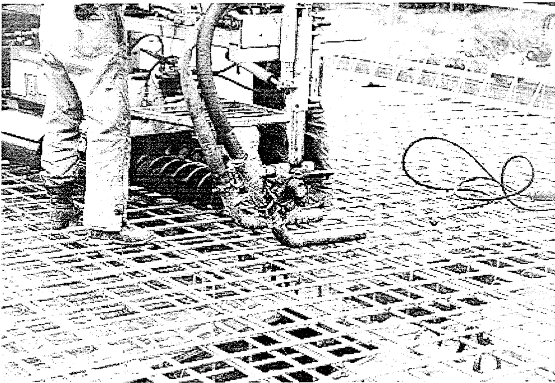
Figure 5. Drag-through vibration device used in Districts 5 & 6.
