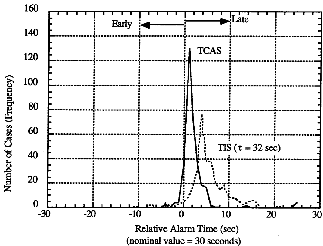
Figure 3. TIS and TCAS alarm times relative to nominal alarm time. TIS \tau set to 32 seconds.
