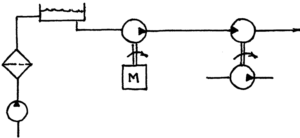
Figure 1. Open Circuit (a) and Non-return Open Circuit (b) Schematics.
