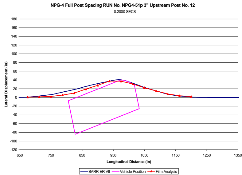
Figure 138. Sequential Figures from BARRIER VII Simulation of NPG-4
