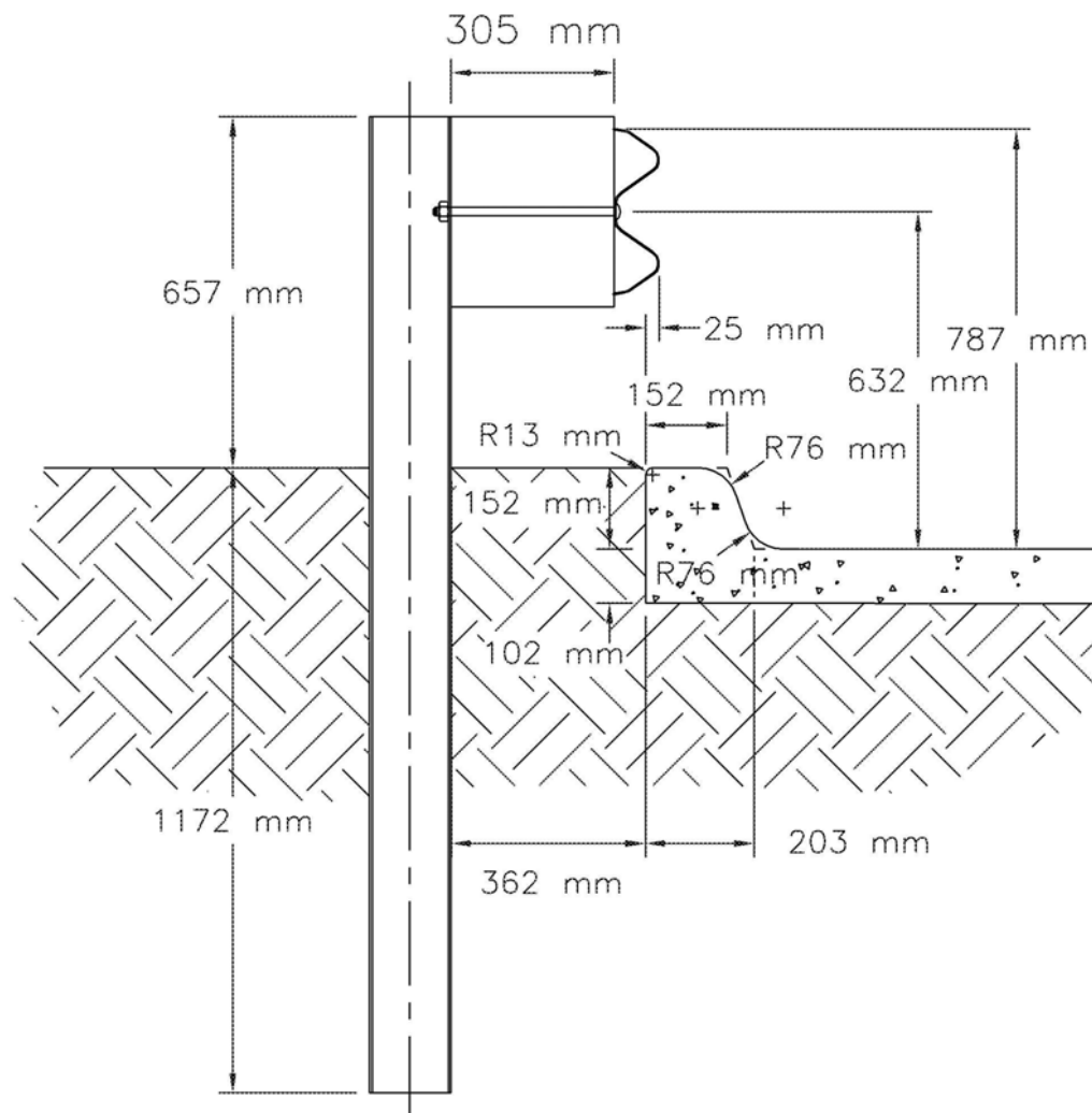
Figure H-2. Midwest Guardrail System Standard Post Spacing with Curb - System Profile (Metric)
