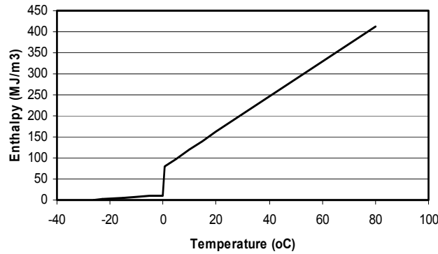
Figure 5-18 Enthalpy-Temperature Curve for Phase Change of Snow
