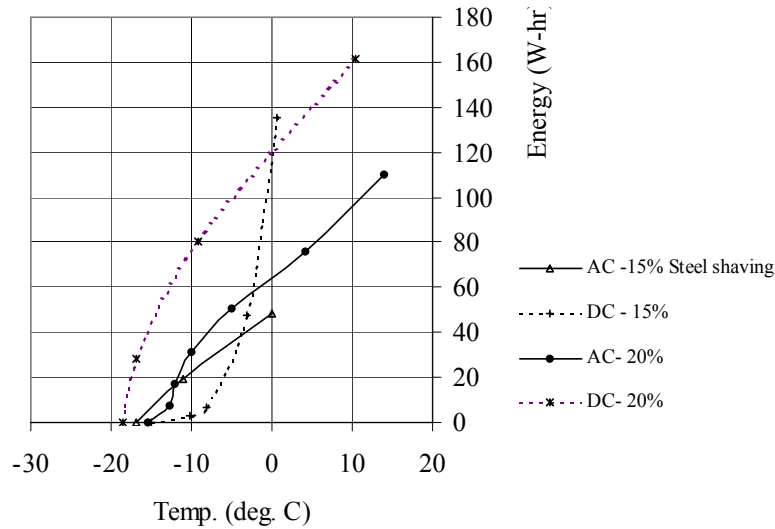
Figure 3-14 Power consumption – AC vs. DC
