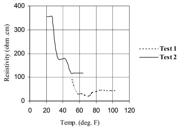
(b) Change of slab resistance with slab temperature
