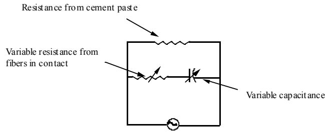
Figure. 3-12 A model for conduction of electricity through conductive concrete
