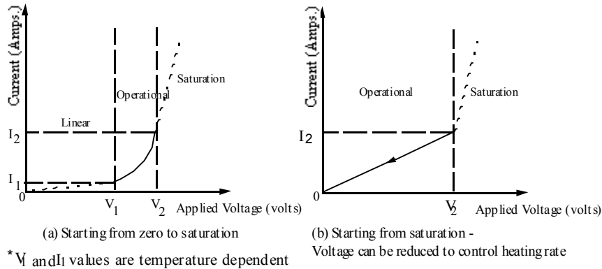
Figure. 3-12 A model for conduction of electricity through conductive concrete
