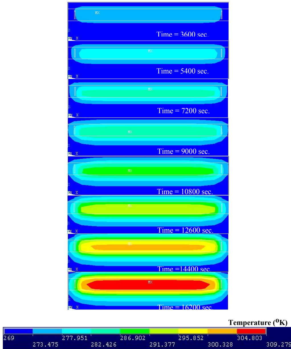
Figure 5-20 Electrical Resistance Heating of Conductive Concrete Overlay
