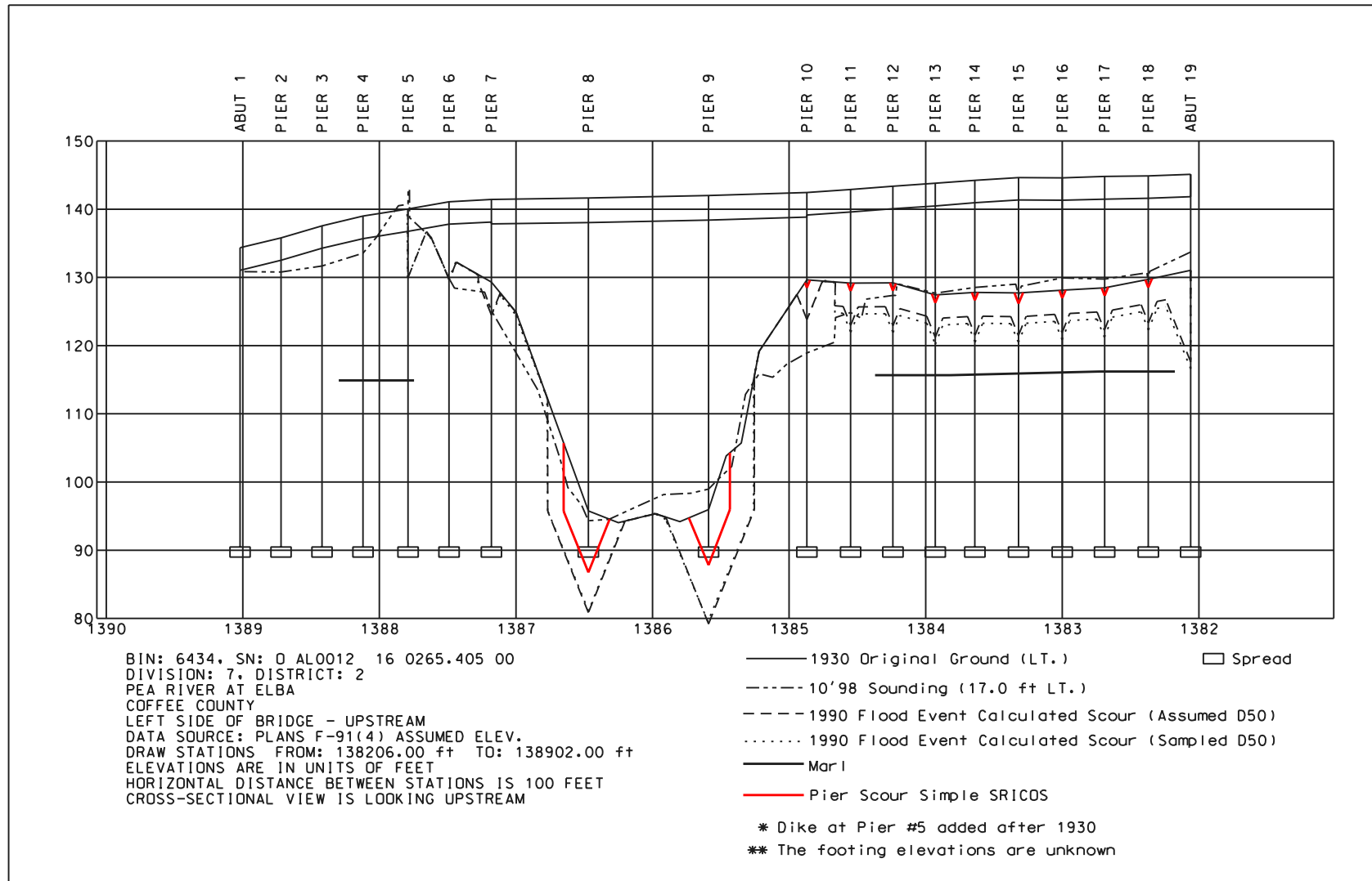
Figure 37. Scour calculations for Pea River at Elba
