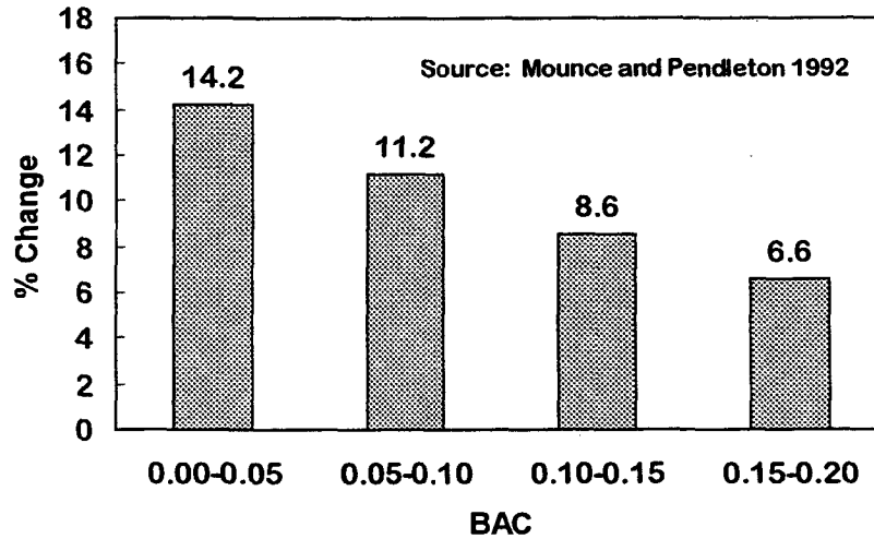
Figure 3-3: Percentage Change in Probability of Crash Responsibility with BAC for Fatal Multiple-Vehicle Crashes - Texas, 1988
