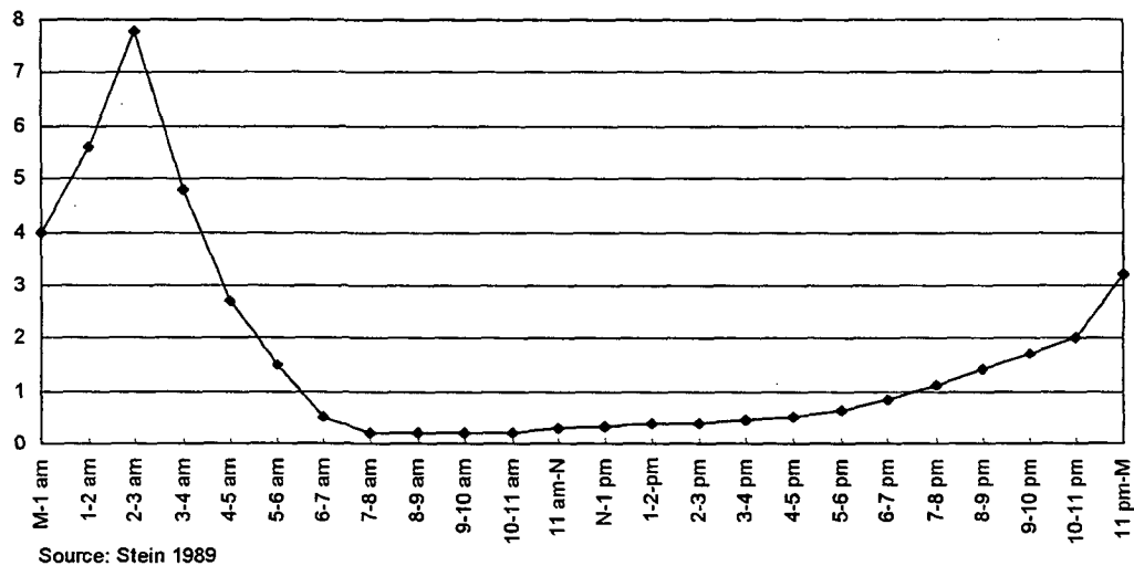
Figure 3-11: Estimated Percentage of Drunk Drivers On the Road Versus Time of Day
