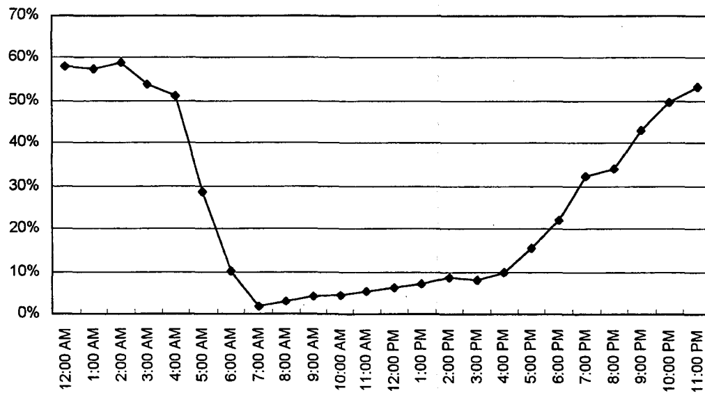
Figure 3-13: Time-of-Day Distribution of Fatally-Injured Involved Non-Occupants with a BAC \geq 0.10\% , FARS 1996
