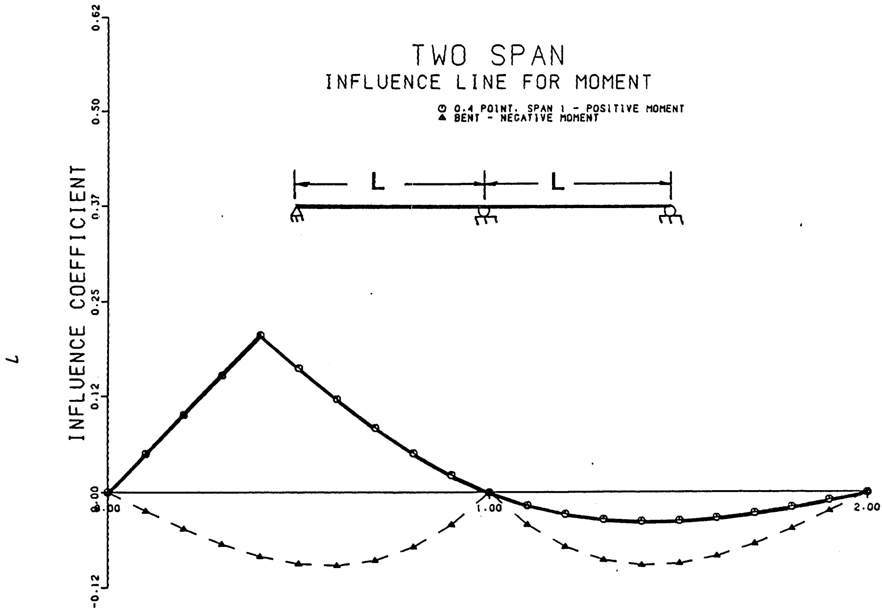
FIGURE 1-2. INFLUENCE LINE FOR A TWO-SPAN BRIDGE
