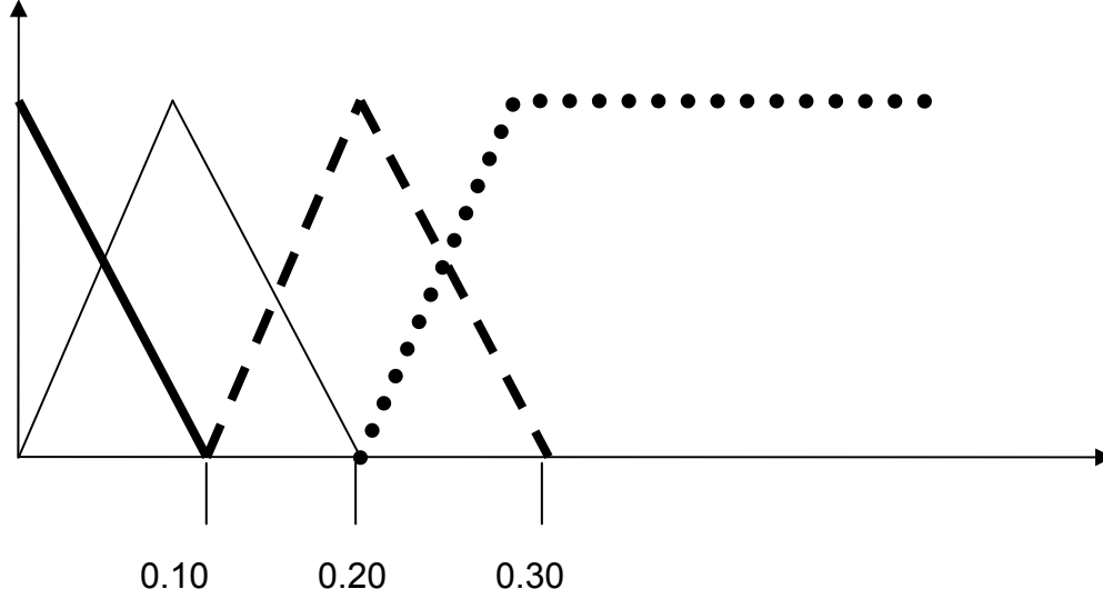
Figure 4.4: Fuzzification for fundamental consistency (regions from left to right are PC, MC, PI, and AI).
