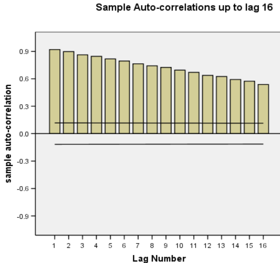
Figure E.2: Sample auto-correlation function for speed data
