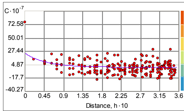
Figure 4.31: Semivariogram Fitting for AADT on Class 2 Segments
