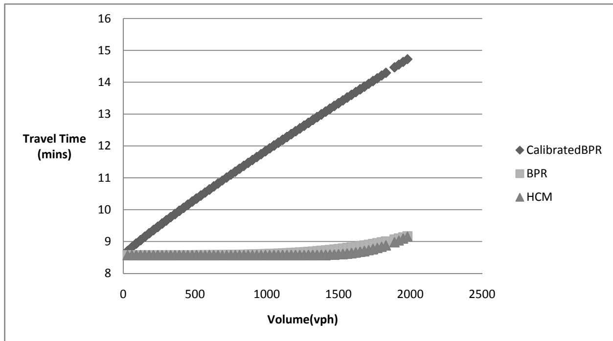
Figure D.4: Calibrated BPR, BPR, and HCM volume delay functions
