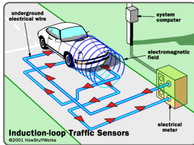
Figure A.6: Inductive loop detector technology
