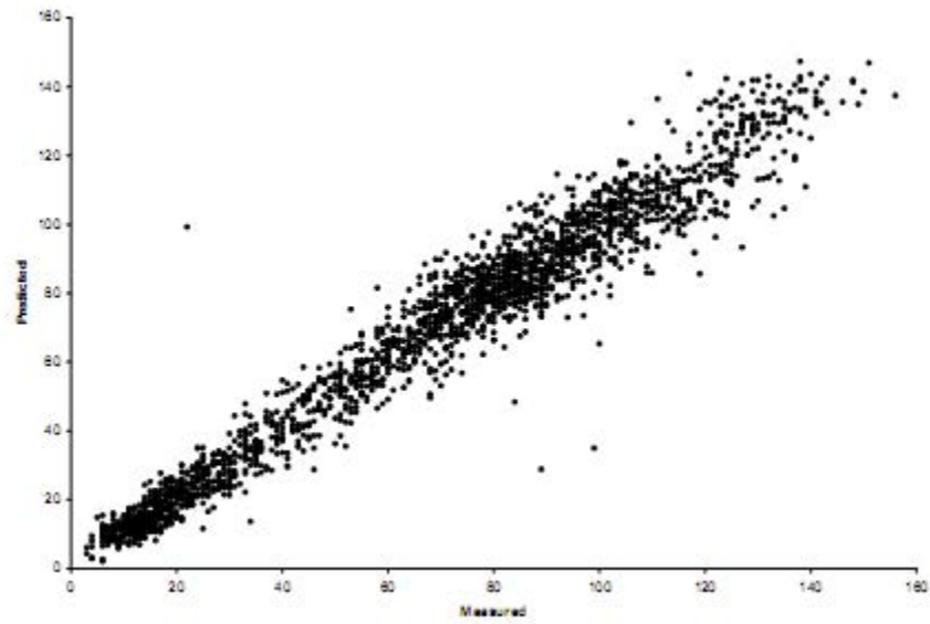
Figure 4.18: Plot of data estimated with LOCAL vs. observed data
