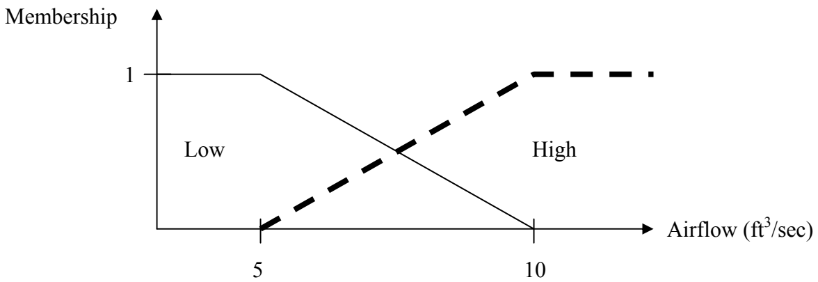
Figure 4.3: Defuzzification converting linguistic airflow to a numeric value
