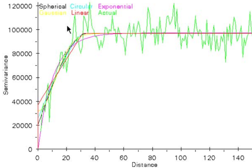
Figure 4.24: Several semivariance model specifications
