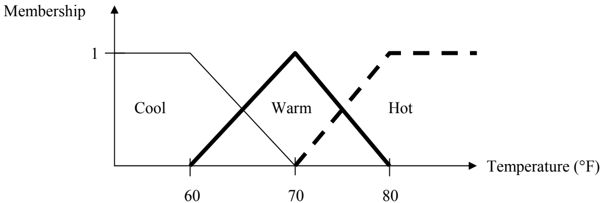
Figure 4.1: Fuzzification of indoor air temperature.
