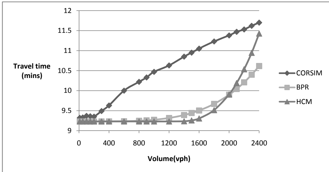
Figure D.5: Comparison of CORSIM, BPR and HCM Volume Delay Function
