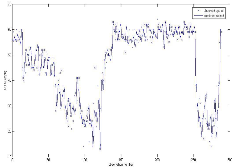
Figure E.4: Predicted and observed speeds
