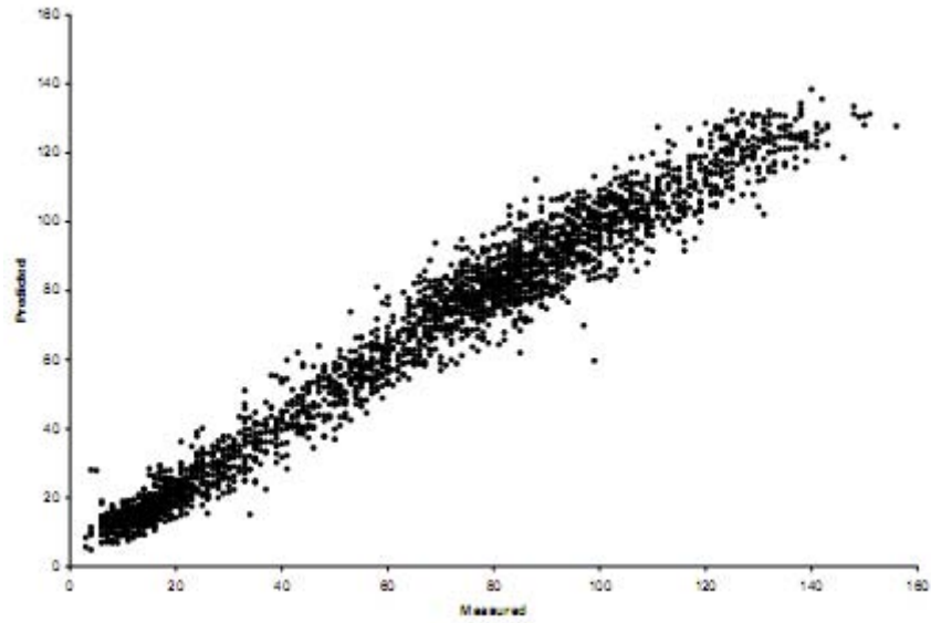
Figure 4.17: Plot of data estimated with MLR-AVG vs. observed data
