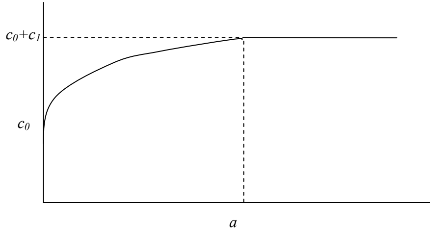
Figure 4.25: Illustration of Semivariogram
