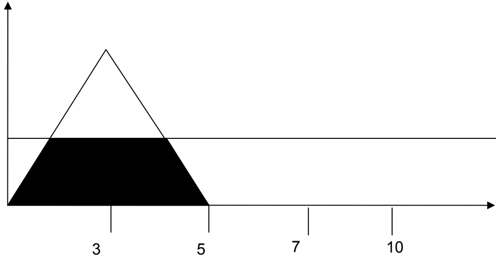
Figure 4.9: Area below the MC curve and the horizontal line \mu = \mu^*
