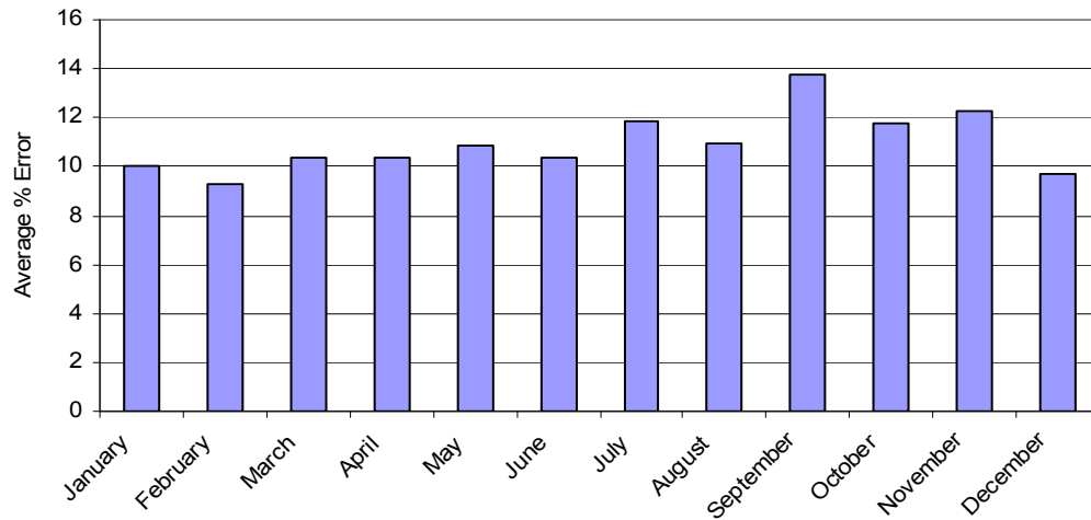
Figure C.3 Variation in AADT Estimation Errors by Month of Year
