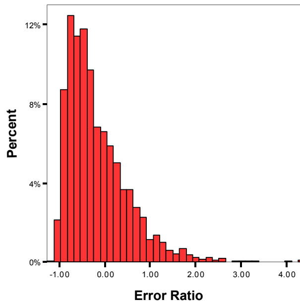
Figure 4.34: Histogram of Differences between Kriging Estimates and Observed Traffic Counts
