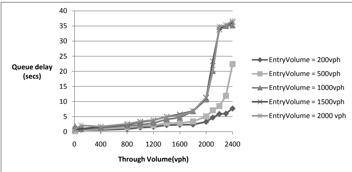
Figure D.6: Queuing delay for different entry volume at entry ramps
