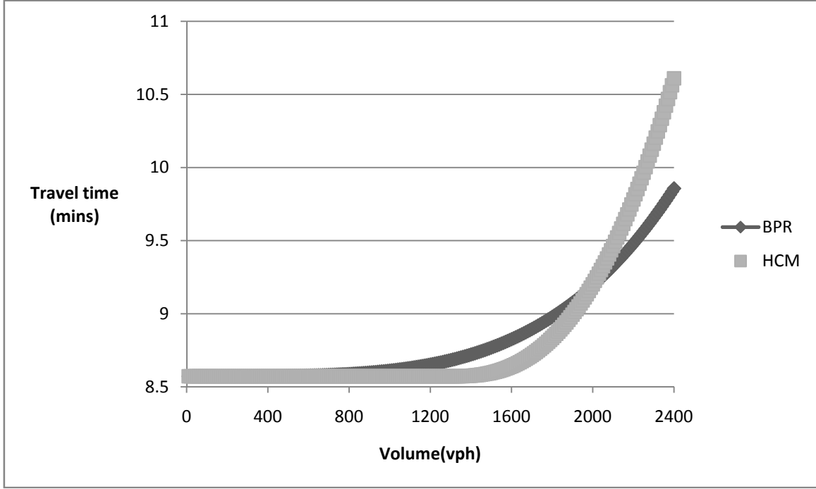
Figure D.1: BPR and HCM Volume Delay Function
