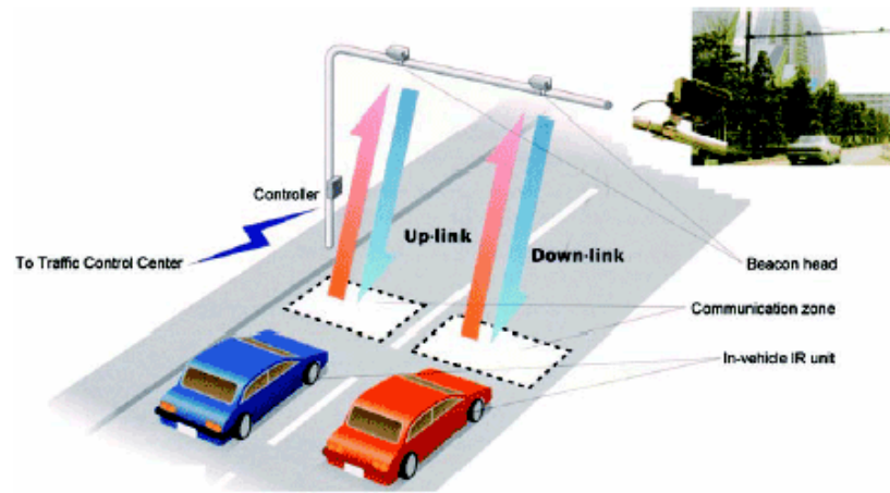
Figure A.4: Infrared technology
