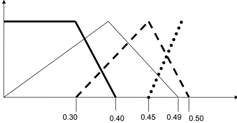
Figure 4.7: Fuzzification for historical consistency
