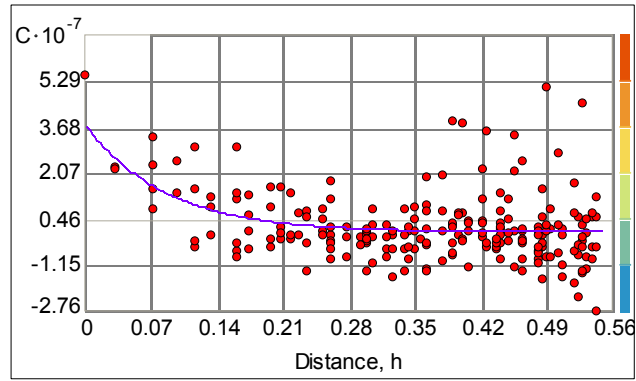
Figure 4.30: Semivariogram Fitting for AADT on Class 1 Segments
