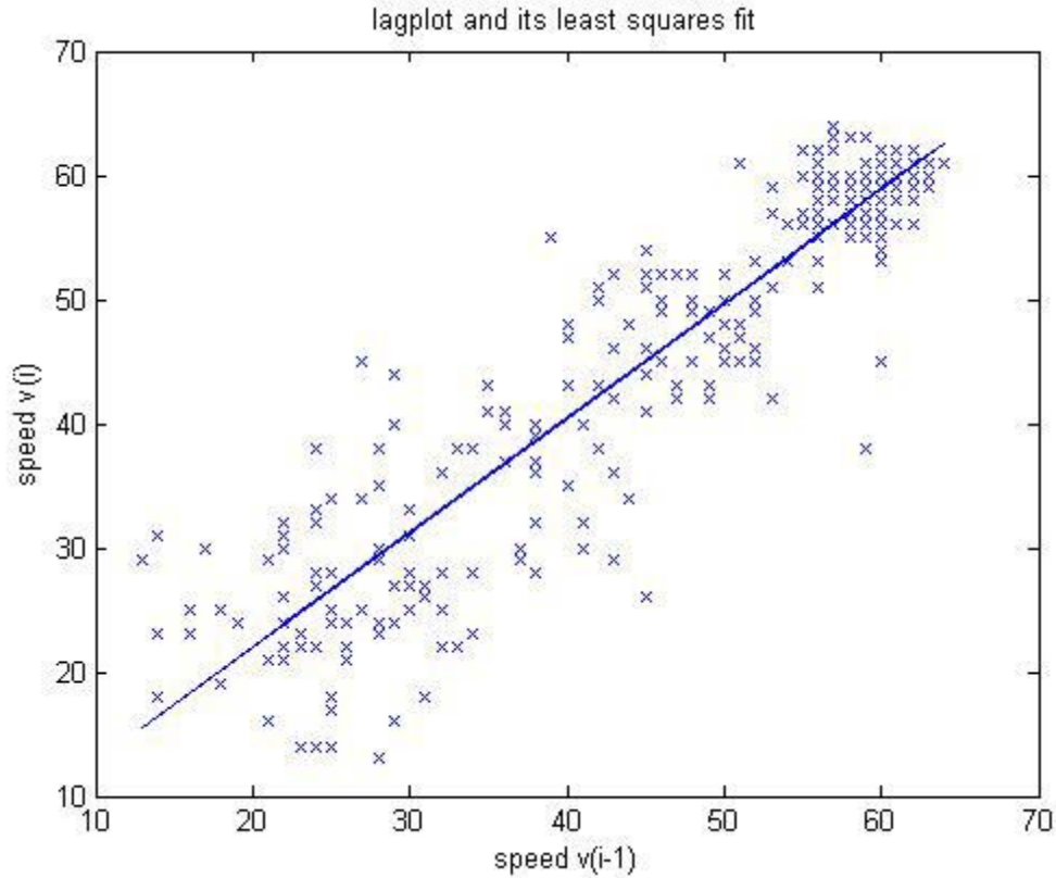
Figure E.3: Lagplot and the least squares line
