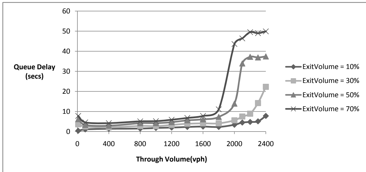
Figure D.7: Queuing delay for different exit ramp volumes
