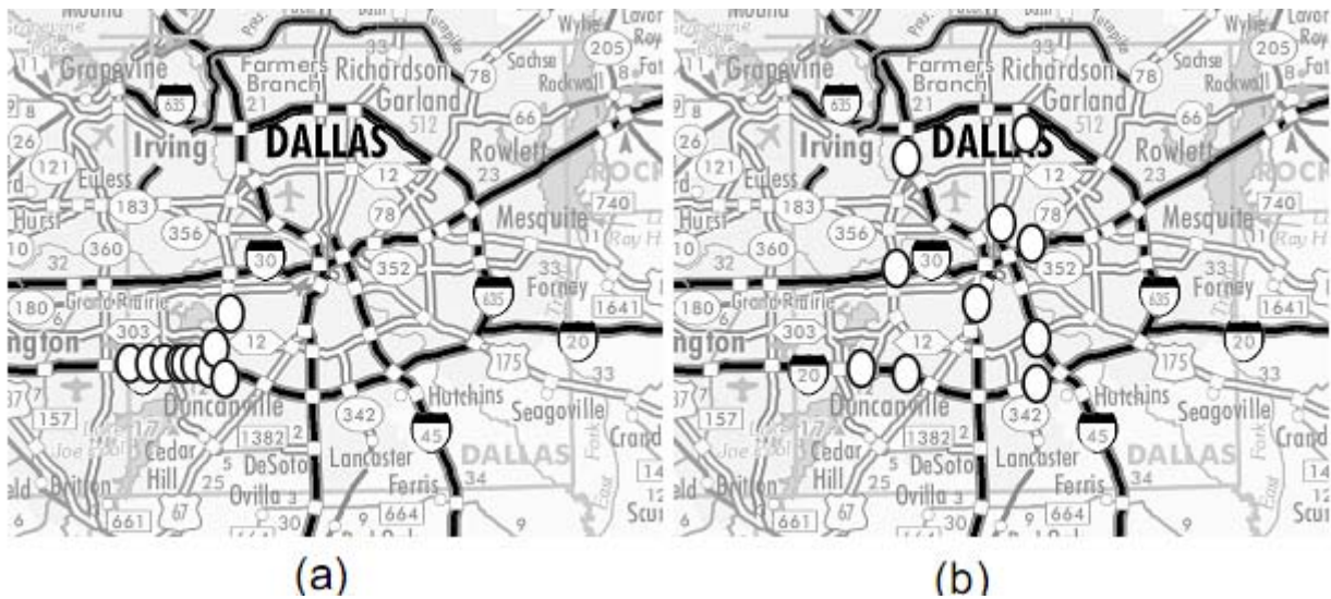
Figure 4.15: Detector locations for (a) local regression and (b) global regression
