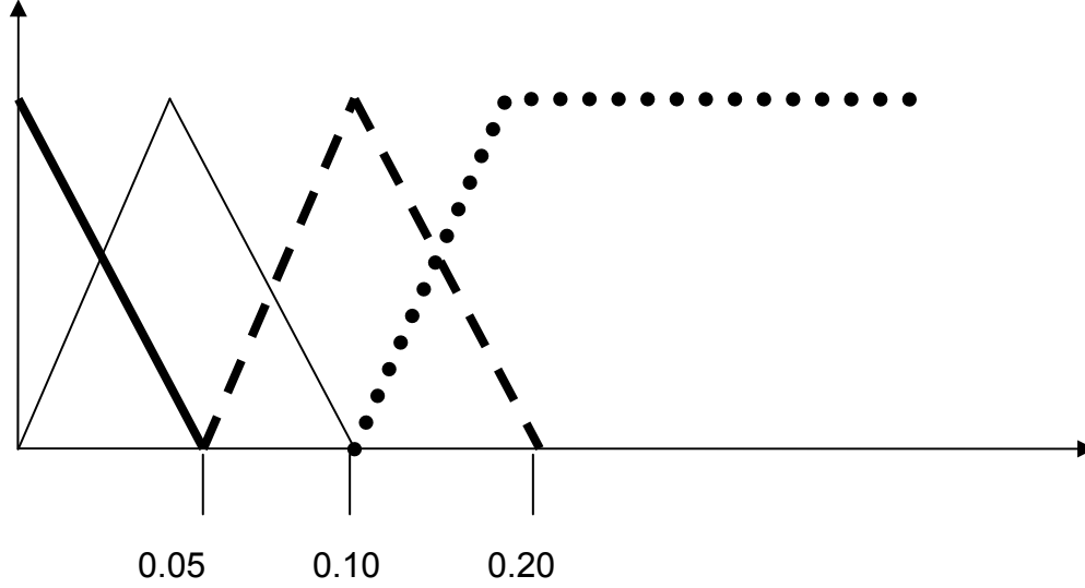
Figure 4.6: Fuzzification diagram for network consistency
