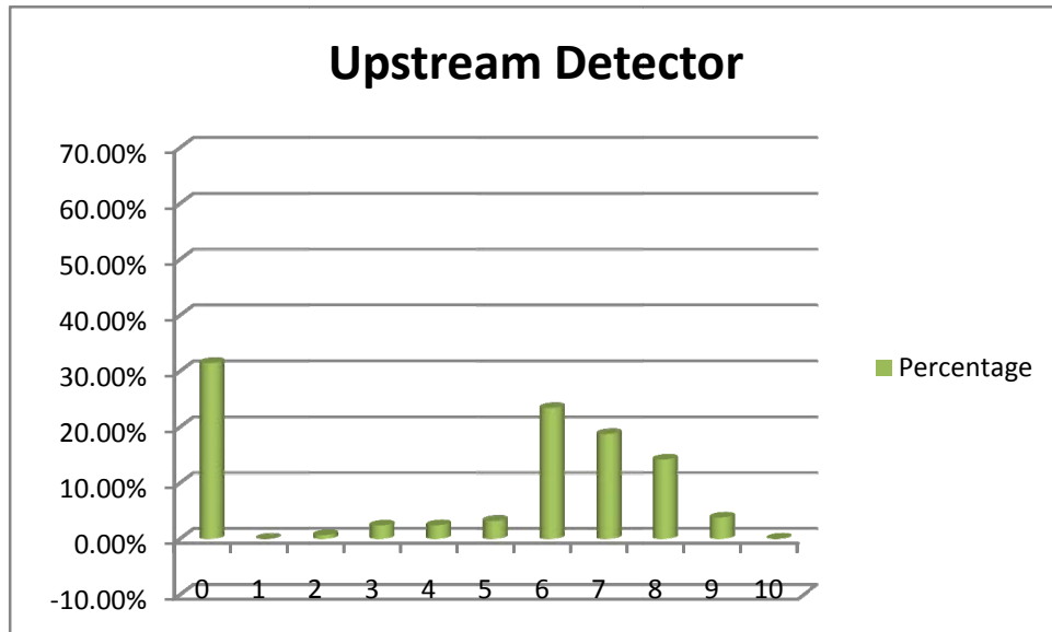
Figure 4.11: Upstream Detector Reliability Index Distribution
