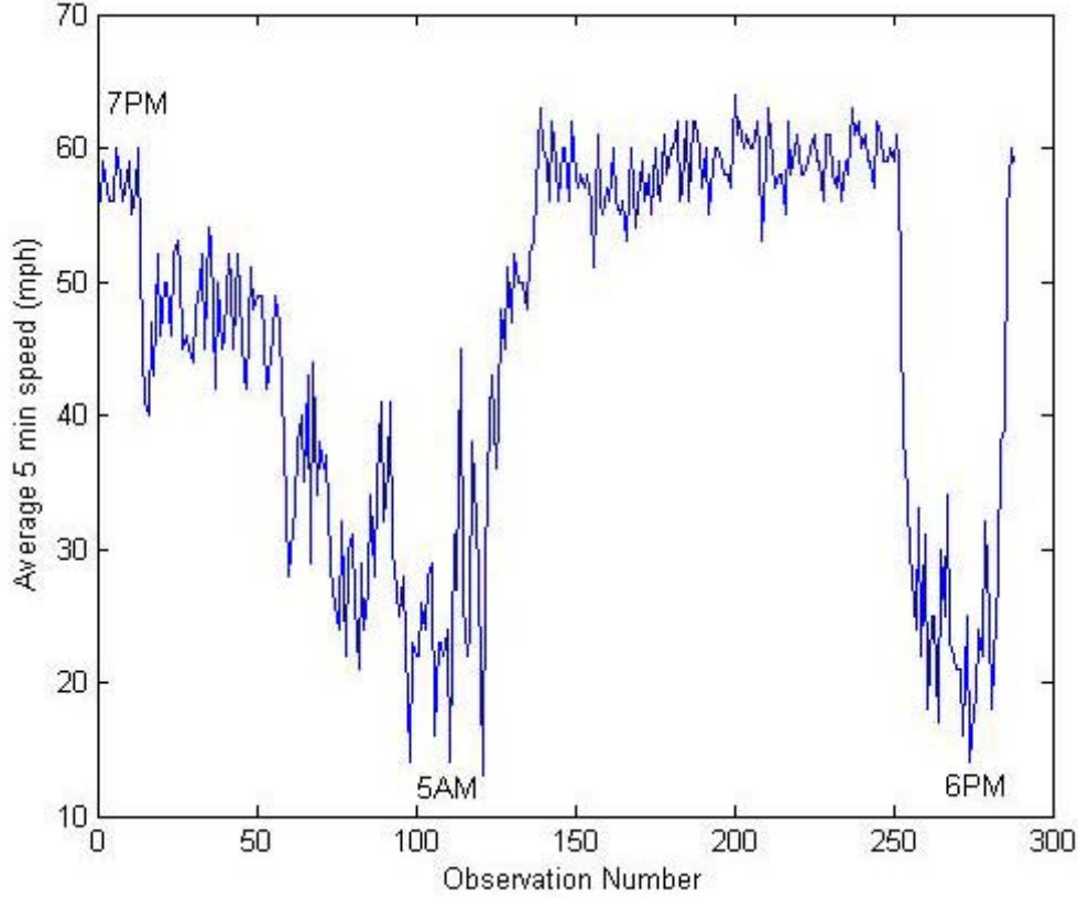
Figure E.1: Speed data for sensor with ID 10043 1084
