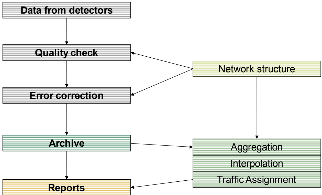
Figure 1.1: Prototype system schematic.
