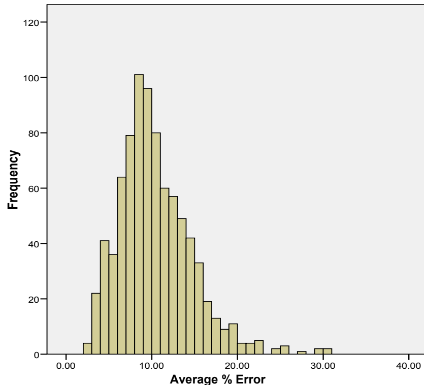
Figure C.1 Histogram of Errors in Predicting AADT from A Single Count Record
