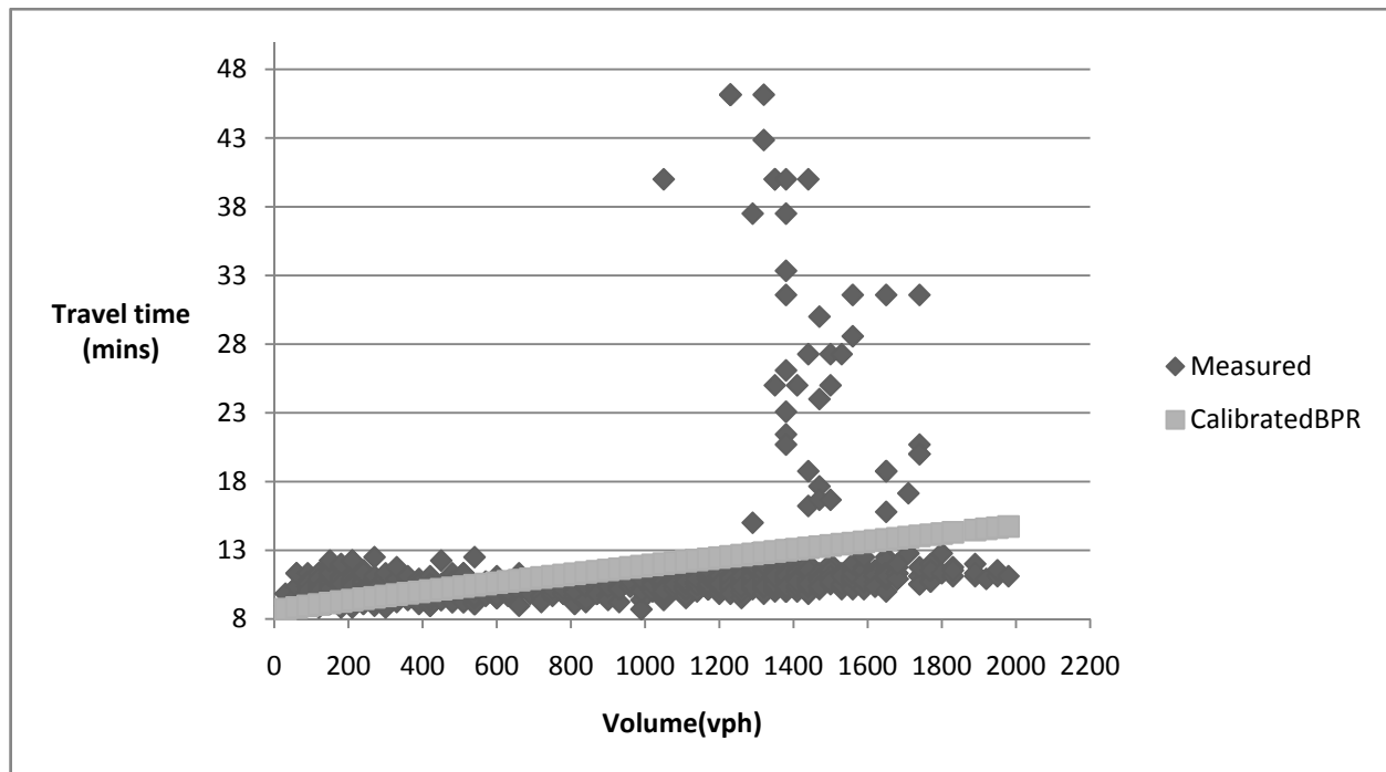
Figure D.3: Calibrated BPR and Measured travel time
