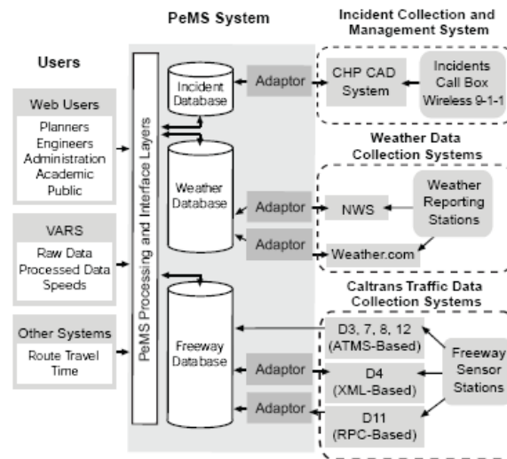
Figure 2.4: Schematic of Major PeMS Components (FHWA, 2005)
