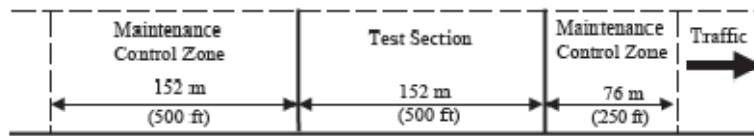
Figure 4.1: Layout of a Generic GPS Test Section
