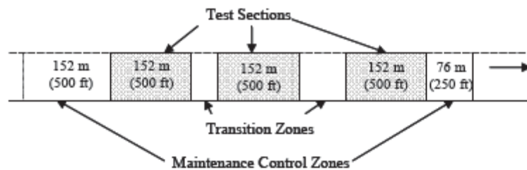
Figure 4.2: Layout of a Generic SPS Test Project
