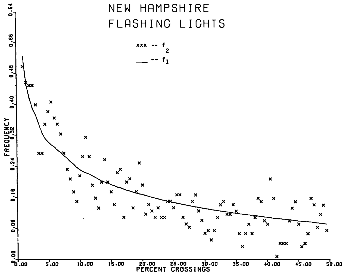
FIGURE E-7. NEW HAMPSHIRE FLASHING LIGHTS MODEL ( f_1 AND f_2 )
