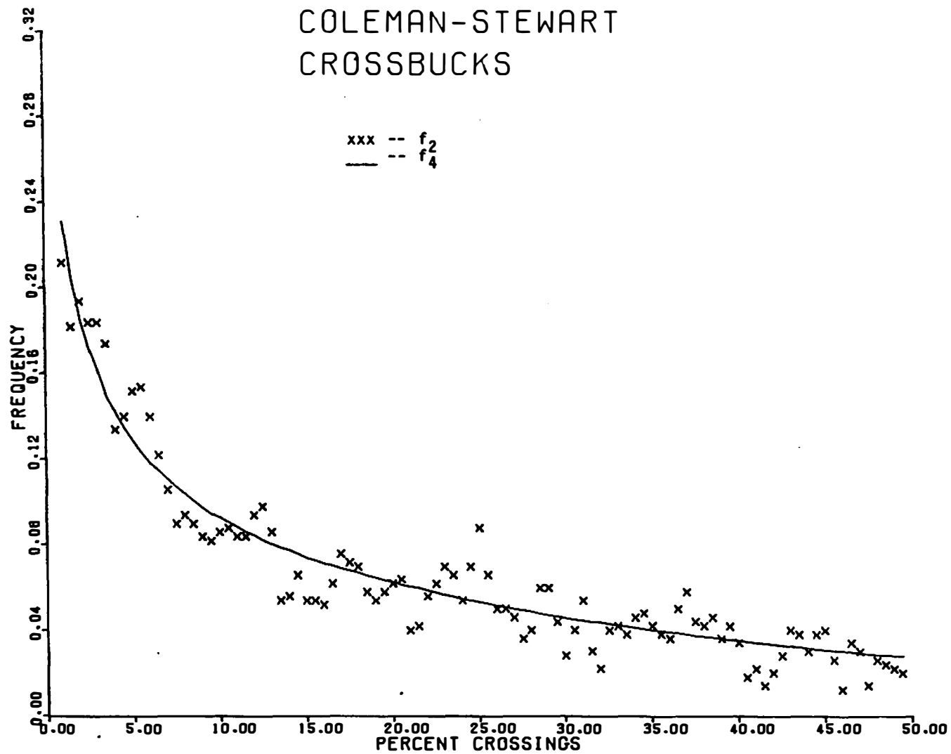
FIGURE E-3. COLEMAN-STEWART CROSSBUCKS MODEL ( f_2 AND f_4 ) (SEE SECTION 4.3)
