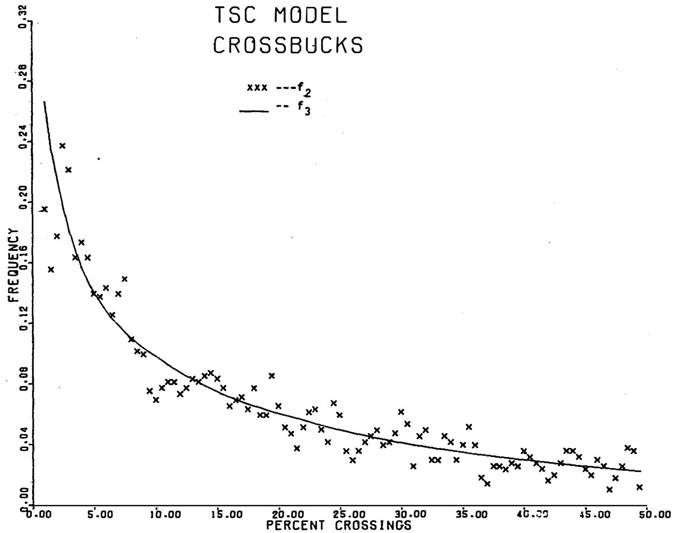
FIGURE E-2. TSC CROSSBUCKS MODEL ( f_2 AND f_3 ) (SEE SECTION 4.3)
