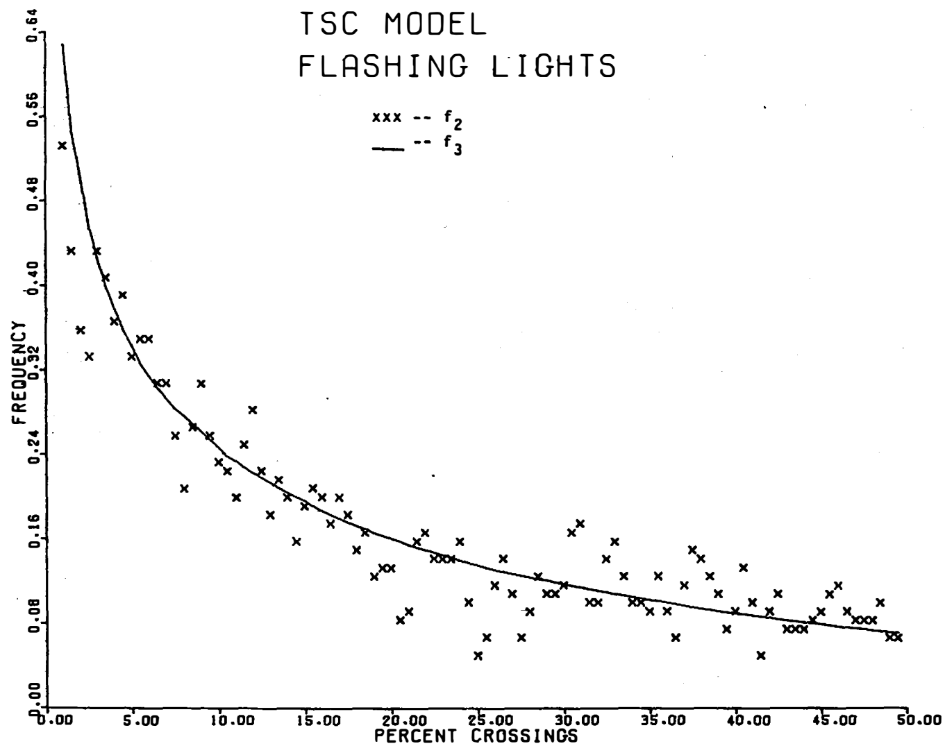
FIGURE E-4. TSC FLASHING LIGHTS MODEL ( f_2 AND f_3 )
