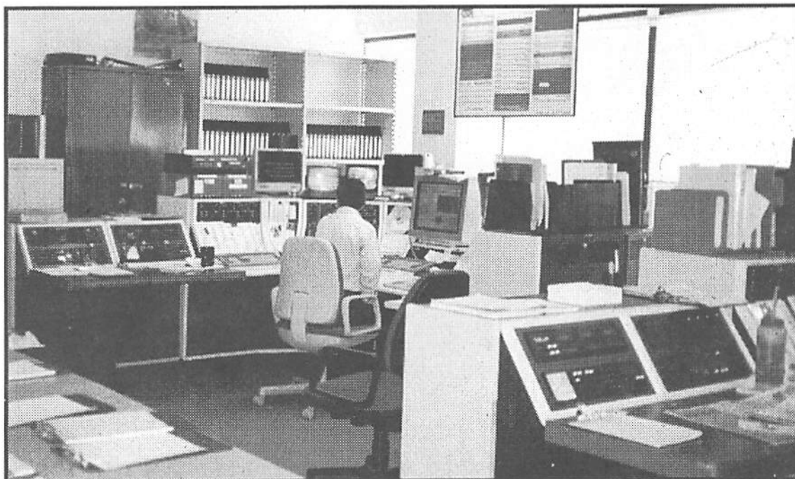
Figure 17. New Dispatcher Consoles
