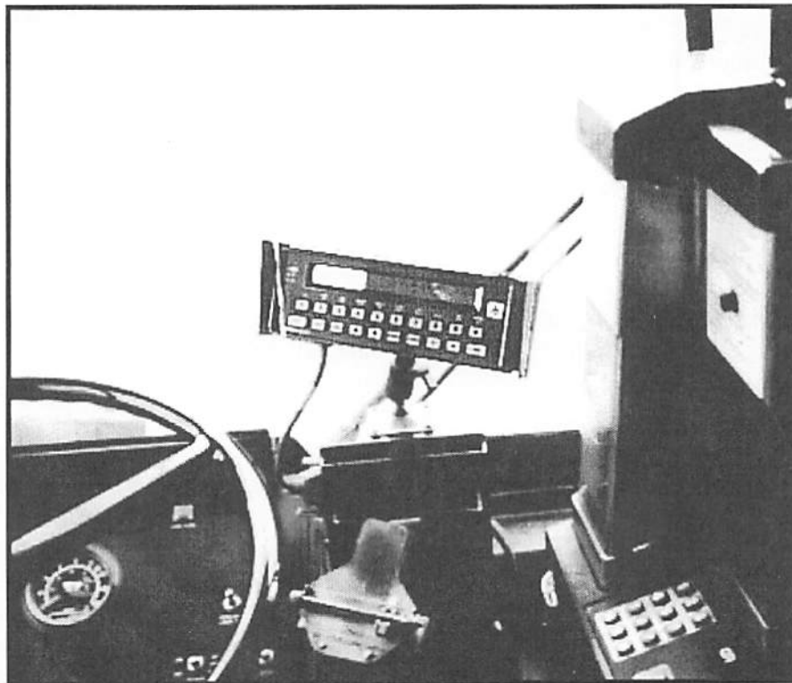
Figure 24. TCH Installed in Bus
