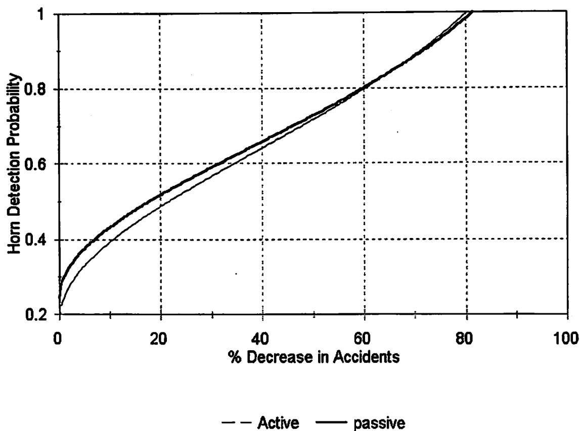
Figure 6. Percent Decrease in Accidents vs. Horn Detectability
