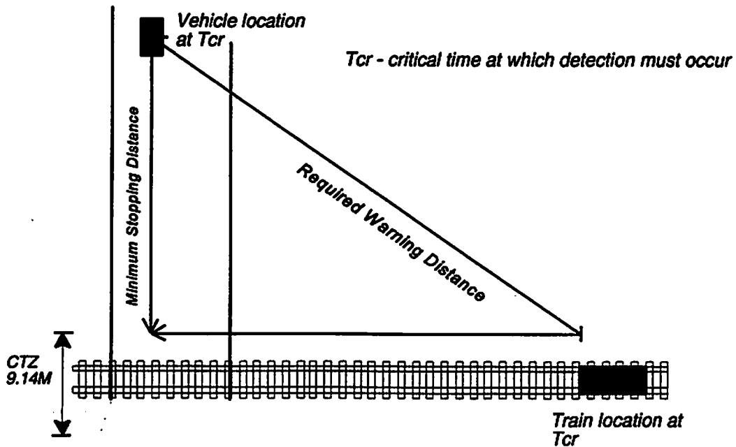
Figure 5. Required Warning Distance
