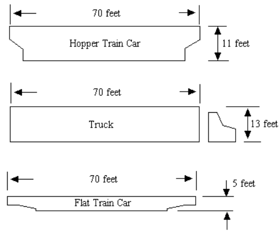
Figure 4. Vehicle Dimensions
