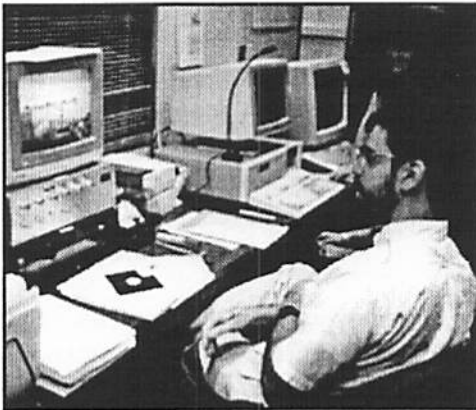
Computer-based training
