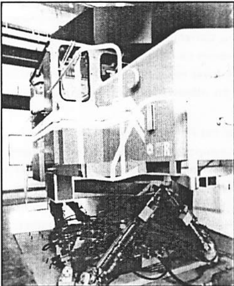
Research and Locomotive Evaluator/Simulator (RALES) Courtesy of IIT Research Institute, Chicago IL
