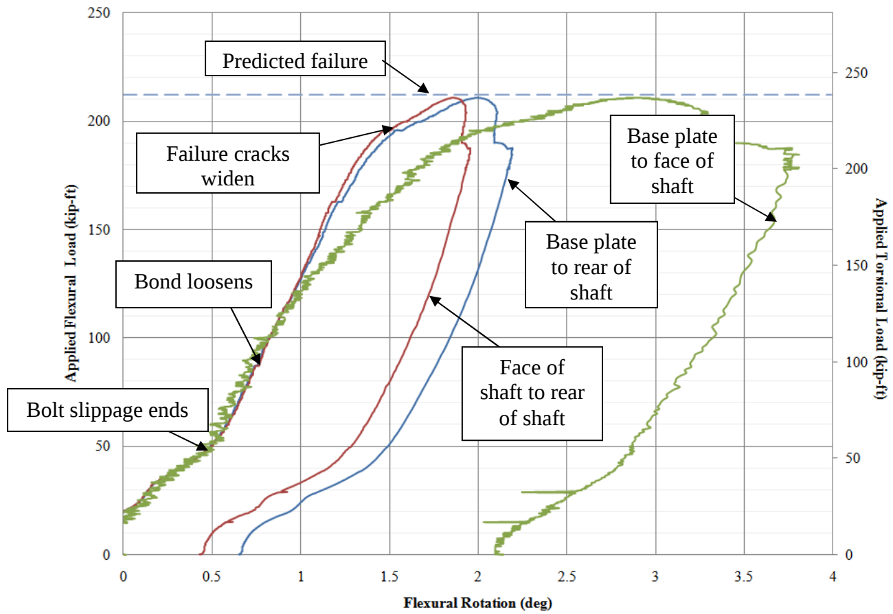
Figure C-4. Load and flexural rotation for torsion and flexure test
