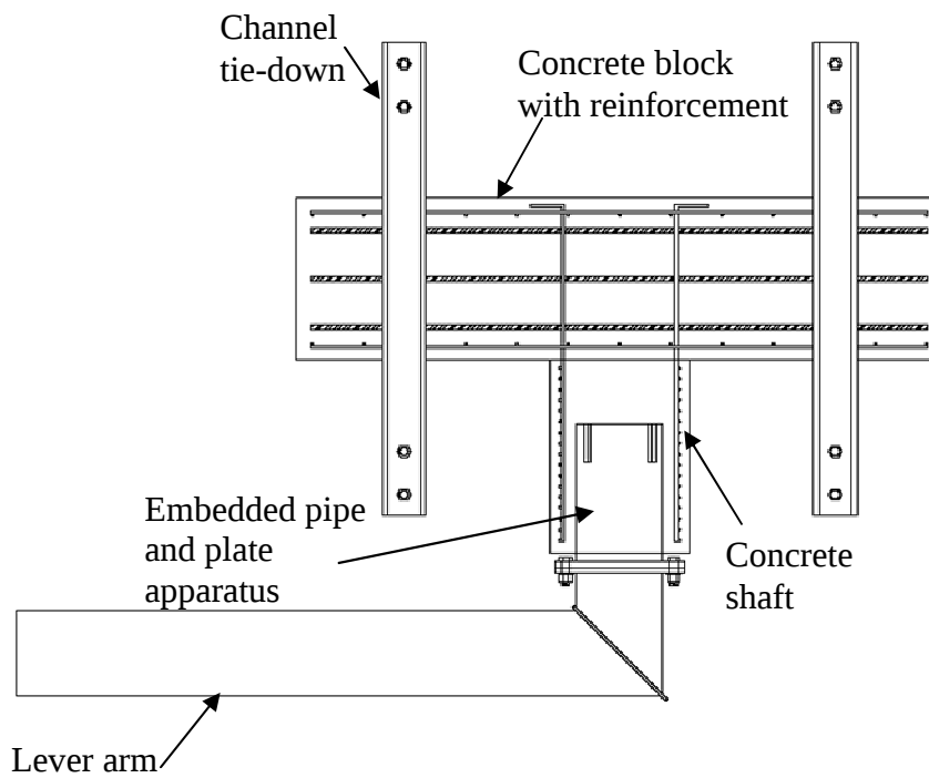
Figure 4-5. Top view of torsion test setup
