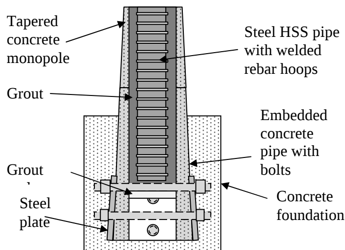
Figure 6-7. Embedded concrete pipe with bolts option with grouted splice to concrete monopole
