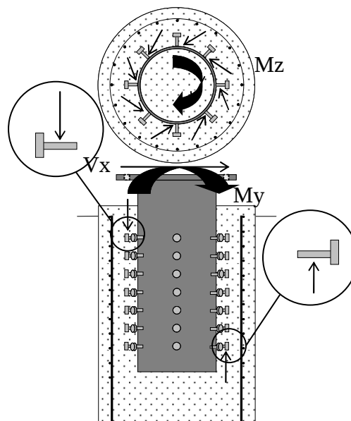
Figure 2-5. Alternate foundation: pipe with welded studs
