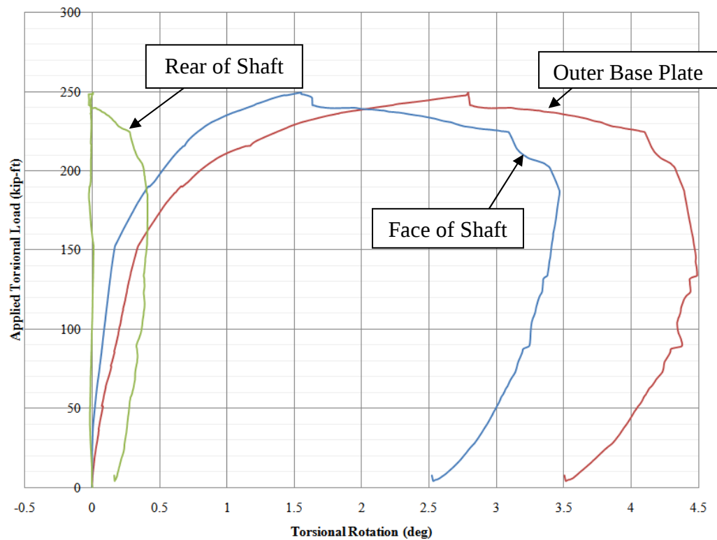
Figure 5-7. Torsional moment and rotation plot for torsion test
