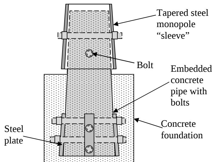
Figure 6-5. Embedded concrete pipe and plate option with slip base connection
