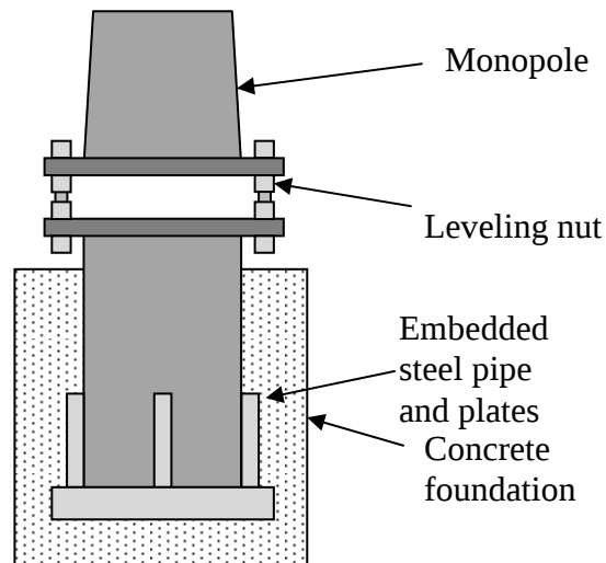
Figure 6-9. Embedded steel pipe and plates with bolted plate connection
