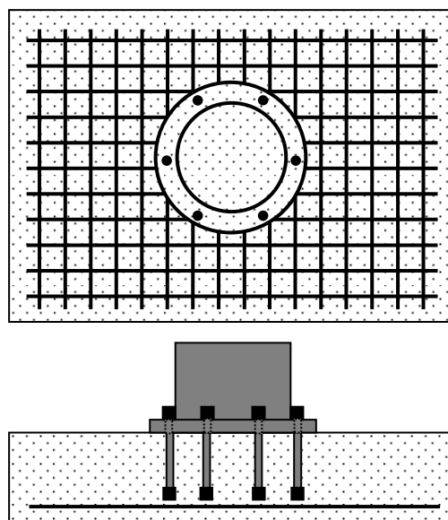
Figure 2-14. Mat foundation for wind turbines
