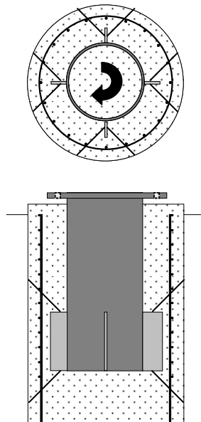
Figure 4-1. Predicted concrete breakout failure
