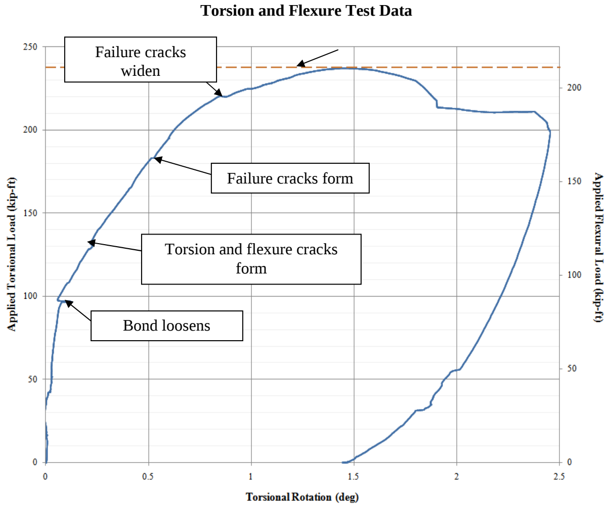
Figure C-3. Load and torsional rotation of base plate for torsion and flexure test
