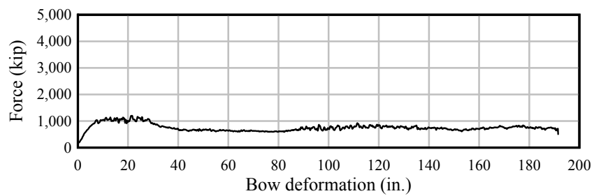
Figure D.4 Barge bow force-deformation data. 6-ft flat-faced pier surface at 5^\circ
