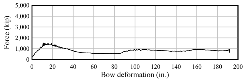
Figure D.20 Barge bow force-deformation data. 12-ft flat-faced pier surface at 5^\circ
