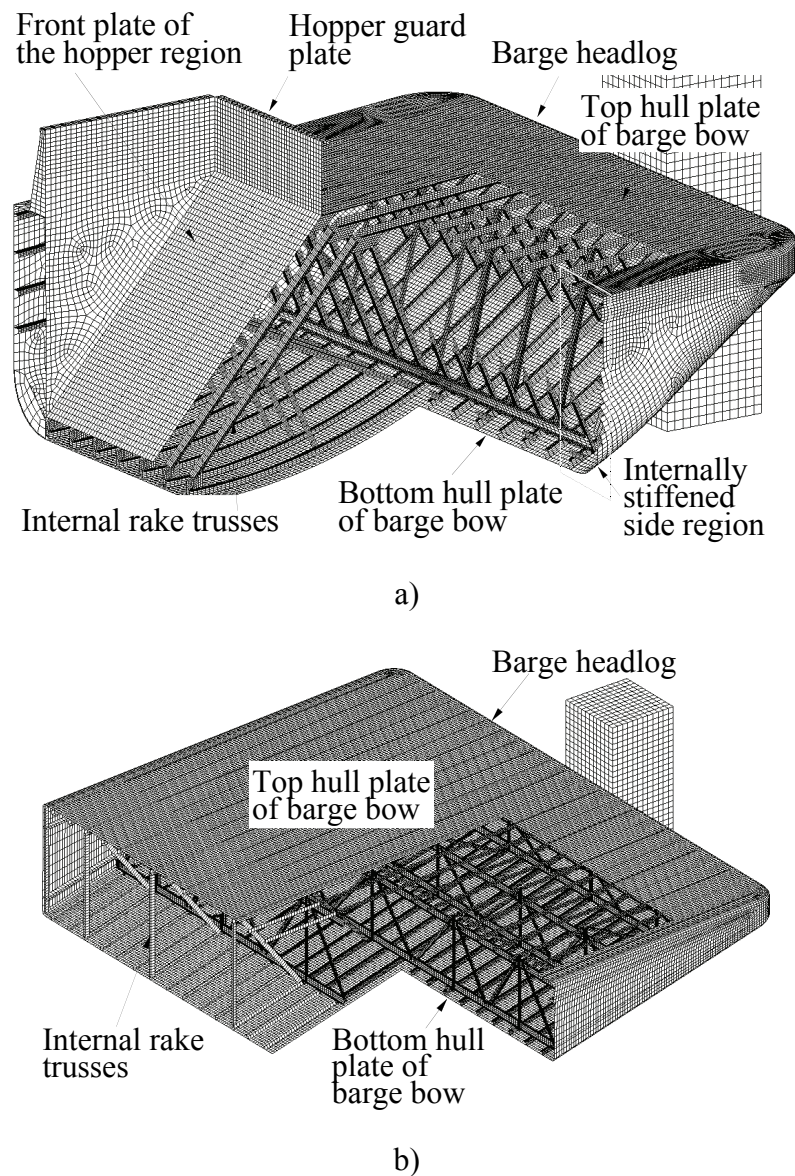
Figure 3.2 Barge bow internal structures (not to relative scale, Consolazio et al. 2009a). a) Jumbo hopper; b) Oversize tanker
