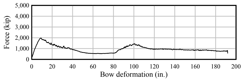
Figure D.27 Barge bow force-deformation data. 18-ft flat-faced pier surface at 2^\circ
