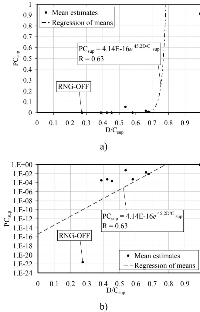
Figure 8.7 Exponential regression curve fit to mean-valued PC_{sup} estimates with inclusion of the RNG-OFF data point. a) Linear plot; b) Semi-log plot
