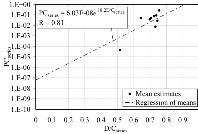
Figure 8.5 Exponential regression curve fit to mean-valued PC_{series} estimates. a) Linear plot; b) Semi-log plot
