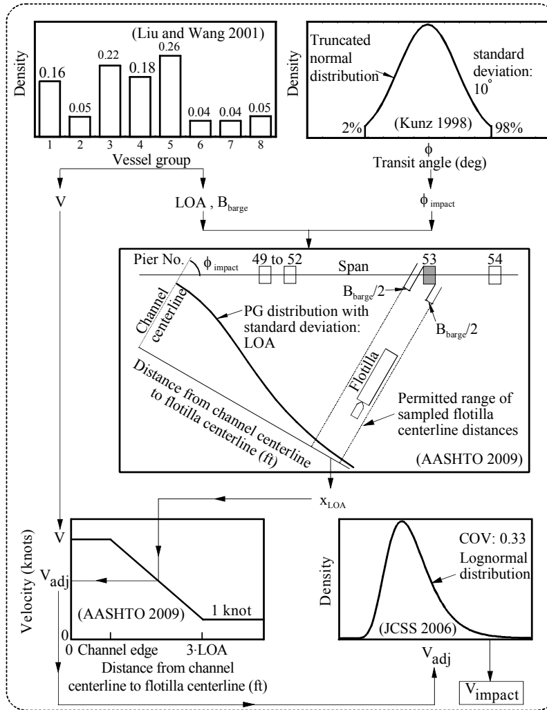
Figure 6.6 Impact velocity ( V_{\text{impact}} ) flowchart
