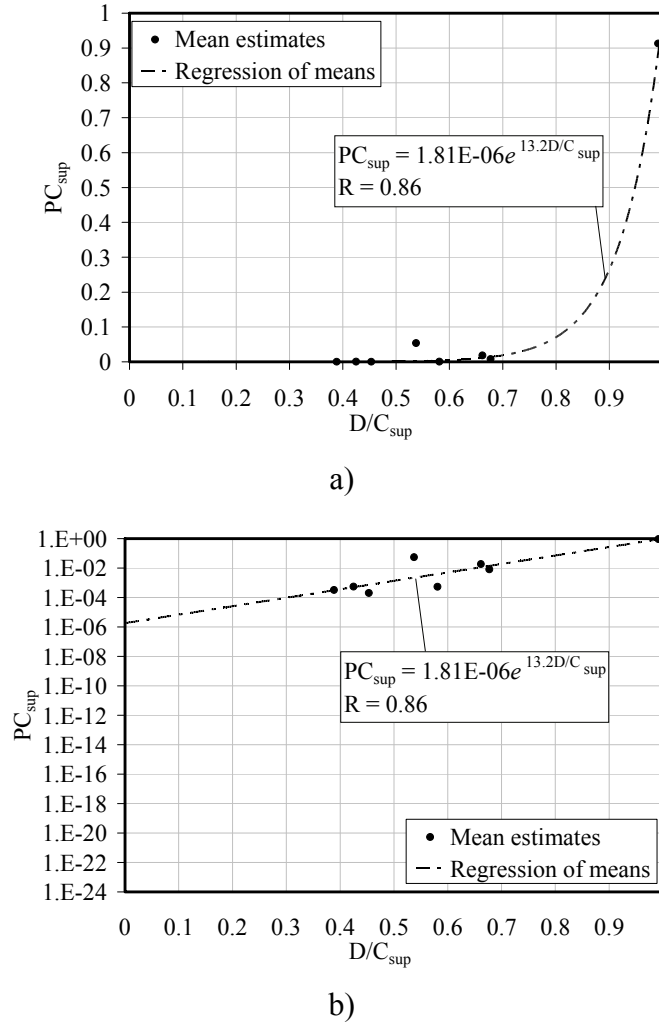
Figure 8.8 Exponential regression curve fit to mean-valued PC_{sup} estimates excluding the RNG-OFF data point. a) Linear plot; b) Semi-log plot
