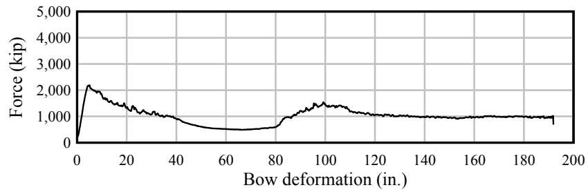
Figure D.26 Barge bow force-deformation data. 18-ft flat-faced pier surface at 1^\circ
