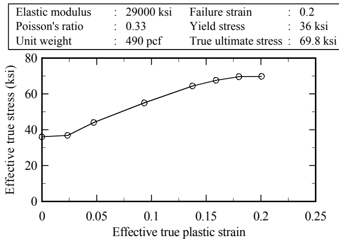
Figure 9.4 Material parameters for A36 structural steel
