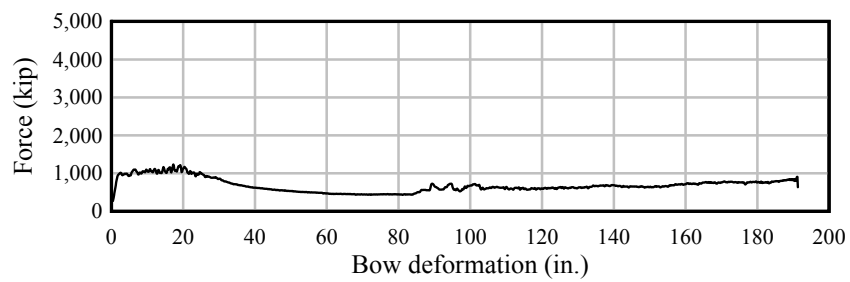
Figure D.2 Barge bow force-deformation data. 6-ft flat-faced pier surface at 1^\circ
