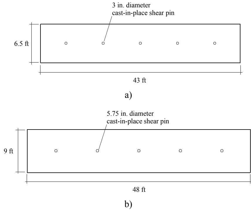
Figure 4.12 Original versus strengthened substructure-superstructure interface for NSG-OFF case. a) Plan view of original pier cap beam; b) Plan view of strengthened pier cap beam
