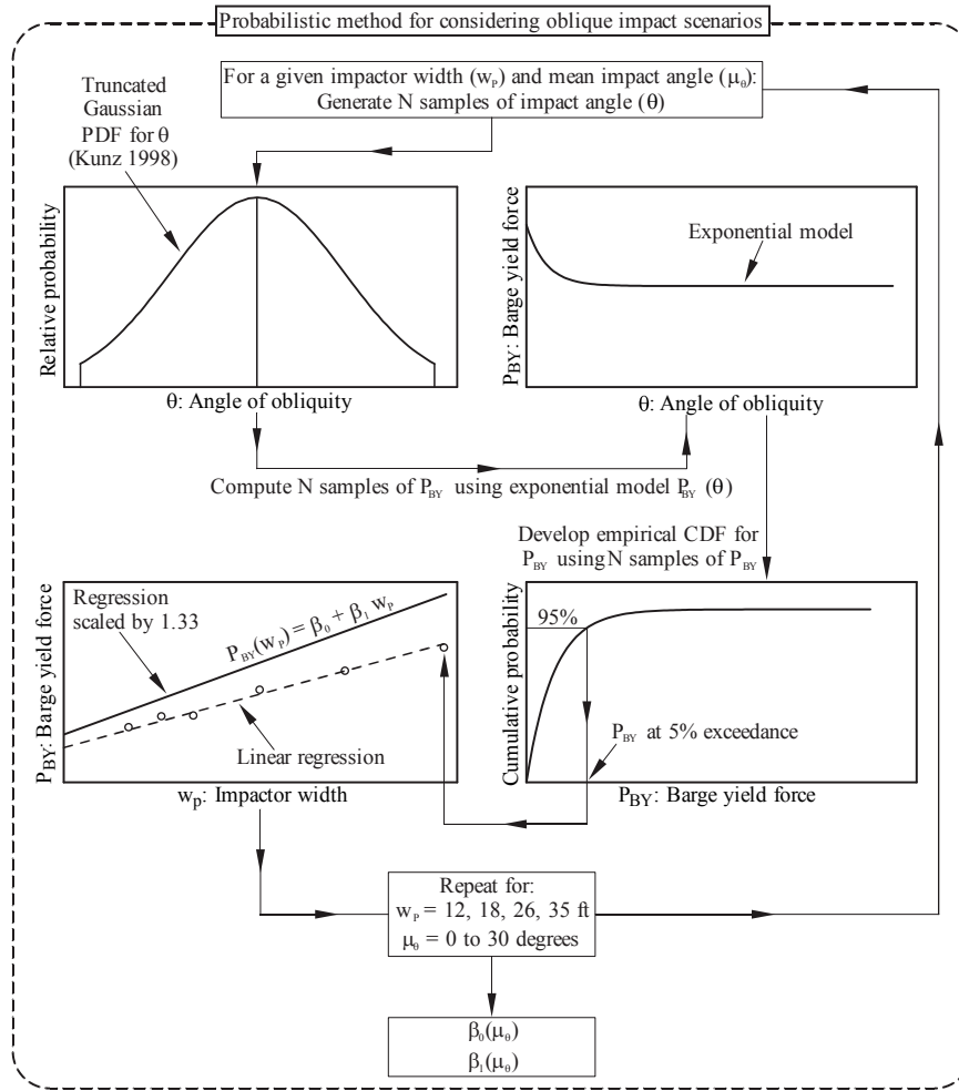
Figure 9.12 Monte Carlo simulation to account for the probability of oblique barge impact
