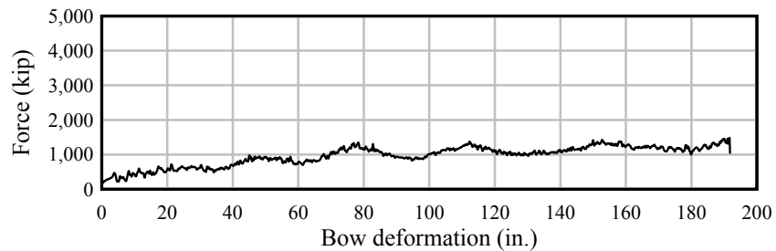
Figure D.16 Barge bow force-deformation data. 9-ft flat-faced pier surface at 45°
