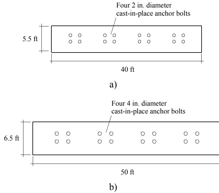
Figure A.7 Original versus strengthened substructure-superstructure interface for Gandy Bridge Pier 75W case. a) Plan view of original pier cap beam; b) Plan view of strengthened pier cap beam
