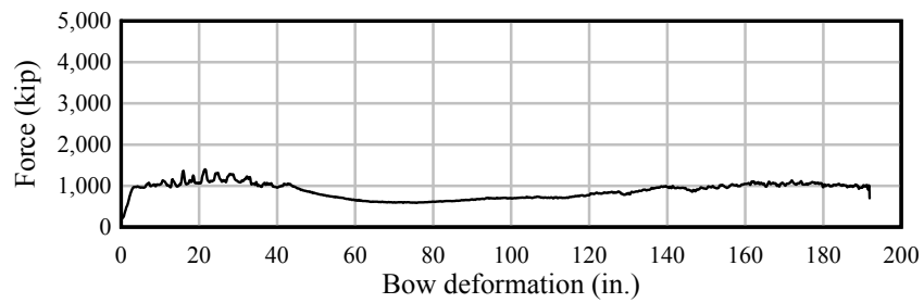
Figure D.3 Barge bow force-deformation data. 6-ft flat-faced pier surface at 2^\circ
