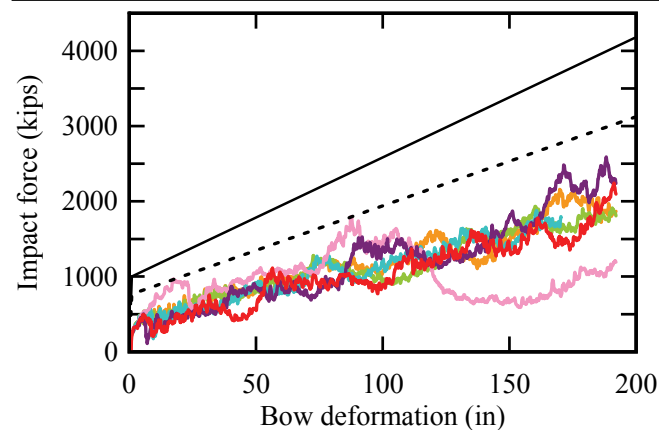
Figure 3.8 Pointed crush simulations. a) Schematic; b) Simulated force-deformation data, initial slope; c) Simulated force-deformation data, full dataset
