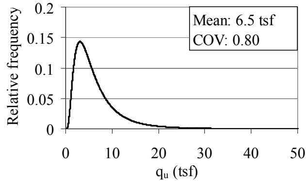
Figure B.17 Limestone unconfined compressive strength ( q_u ) frequency plot for John Ringling Causeway Bridge
