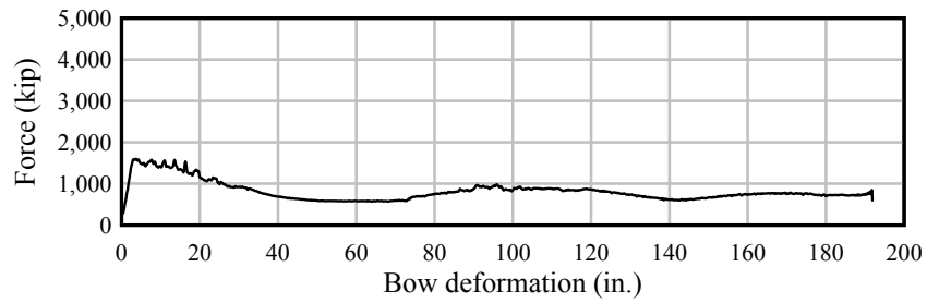
Figure D.18 Barge bow force-deformation data. 12-ft flat-faced pier surface at 1^\circ
