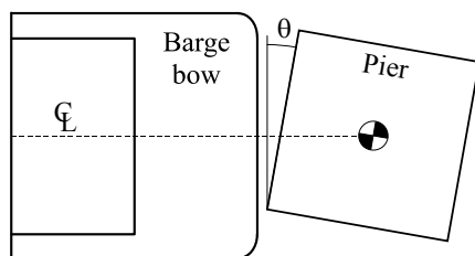
e) 26-ft pier surface
