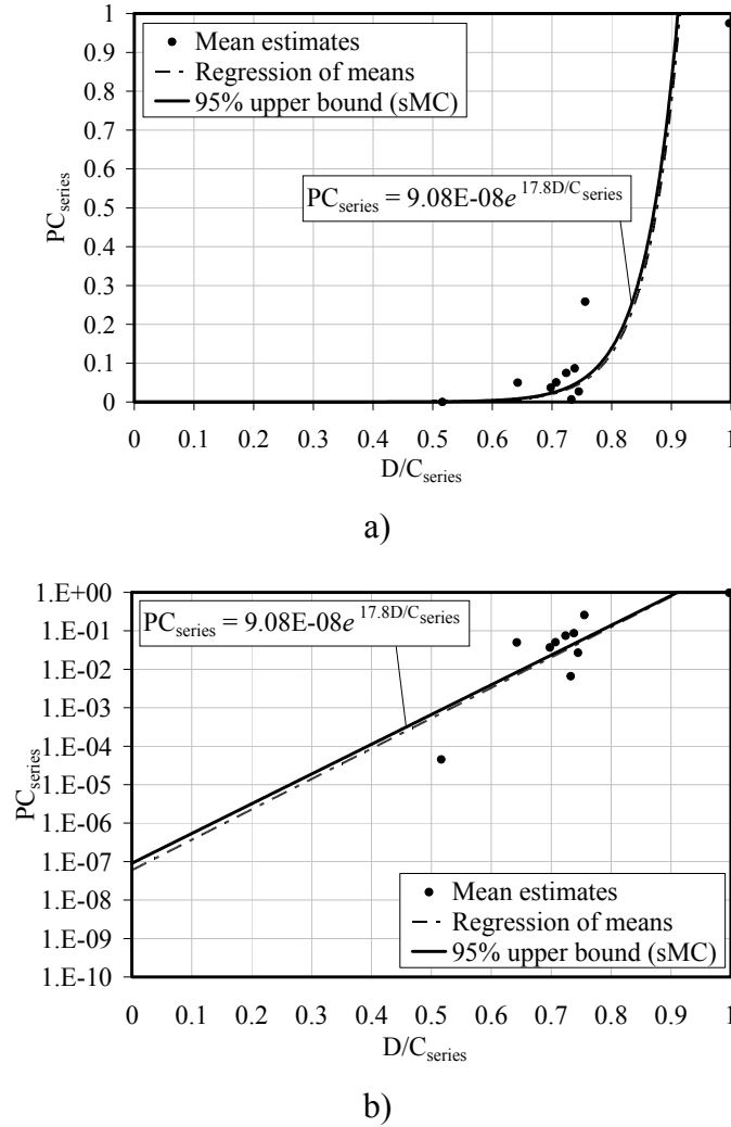
Figure 8.6 Proposed probability of collapse expression for the FDOT series limit state. a) Linear plot; b) Semi-log plot
