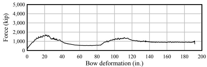
Figure D.28 Barge bow force-deformation data. 18-ft flat-faced pier surface at 5^\circ
