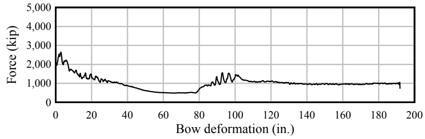
Figure D.25 Barge bow force-deformation data. 18-ft flat-faced pier surface at 0^\circ
