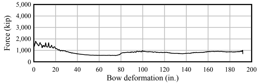
Figure D.17 Barge bow force-deformation data. 12-ft flat-faced pier surface at 0^\circ
