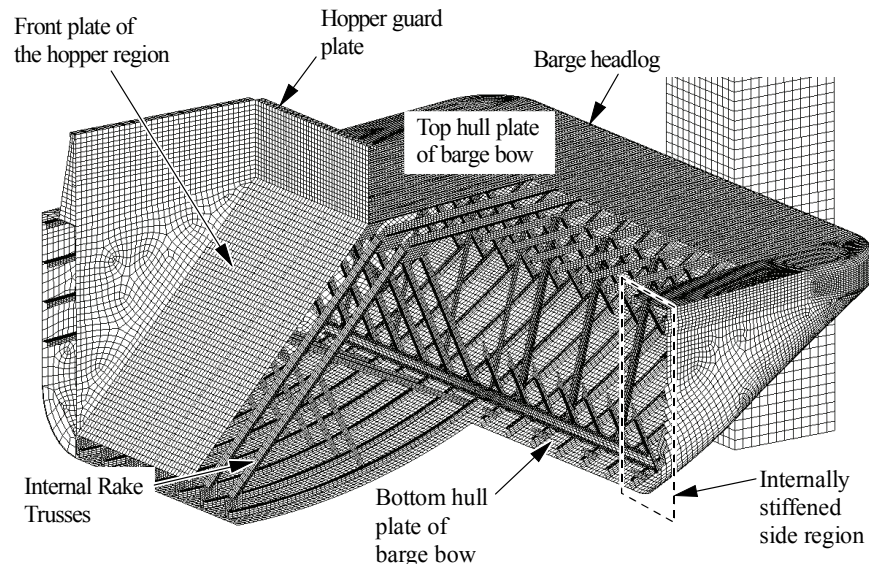
Figure 9.2 Jumbo hopper barge model.
