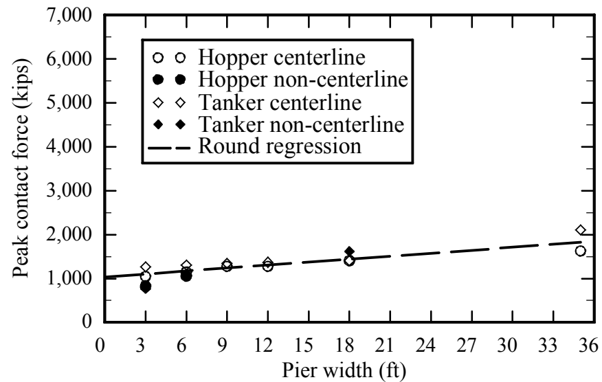
Figure 3.5 Barge peak contact force versus impactor width regression curves (after Consolazio et al. 2009a). a) Flat data; b) Round data
