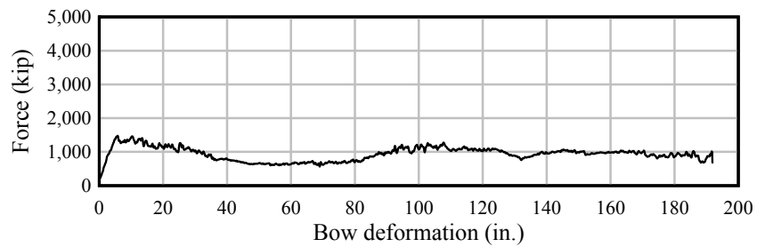
Figure D.19 Barge bow force-deformation data. 12-ft flat-faced pier surface at 2^\circ
