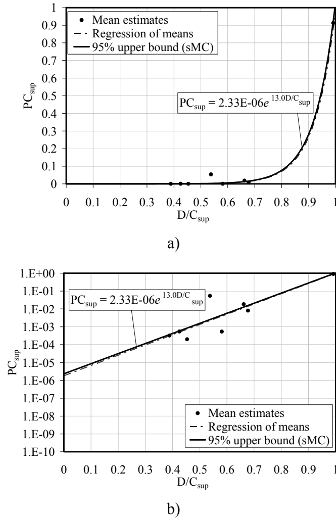
Figure 8.9 Proposed probability of collapse expression for the AASHTO superstructure collapse limit state. a) Linear plot; b) Semi-log plot
