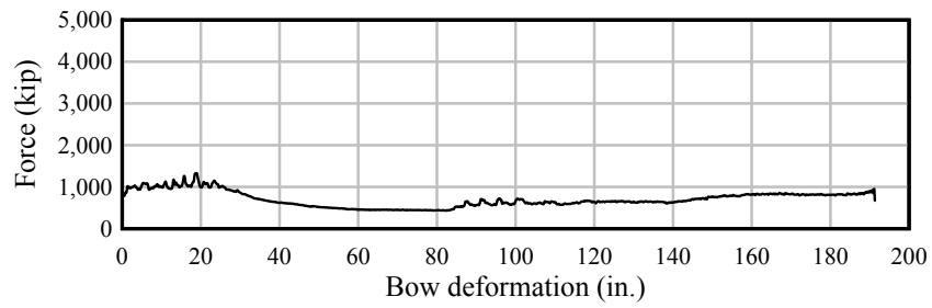
Figure D.1 Barge bow force-deformation data. 6-ft flat-faced pier surface at 0^\circ
