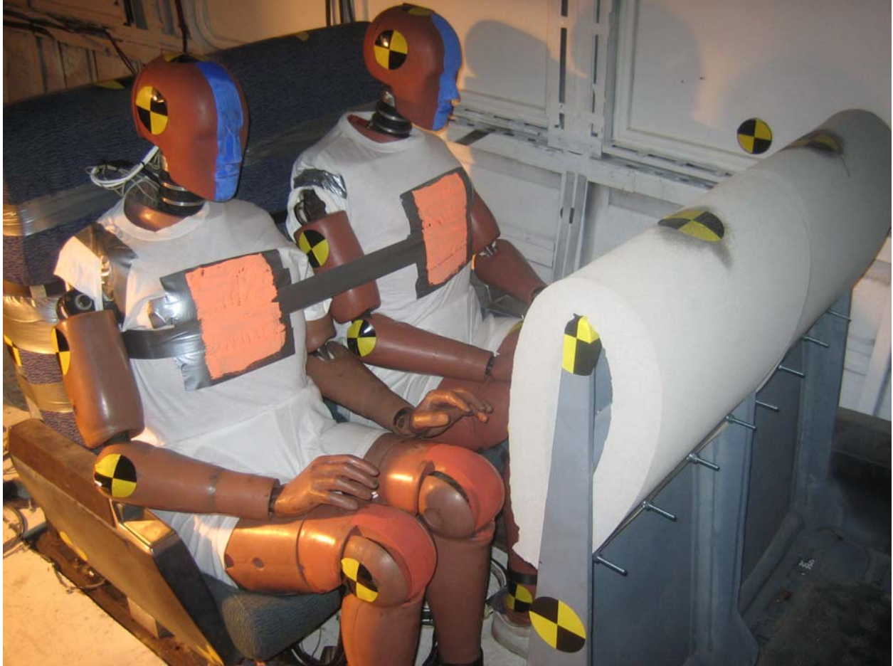
Figure 27. Pretest Photograph of Experiment 2.1
