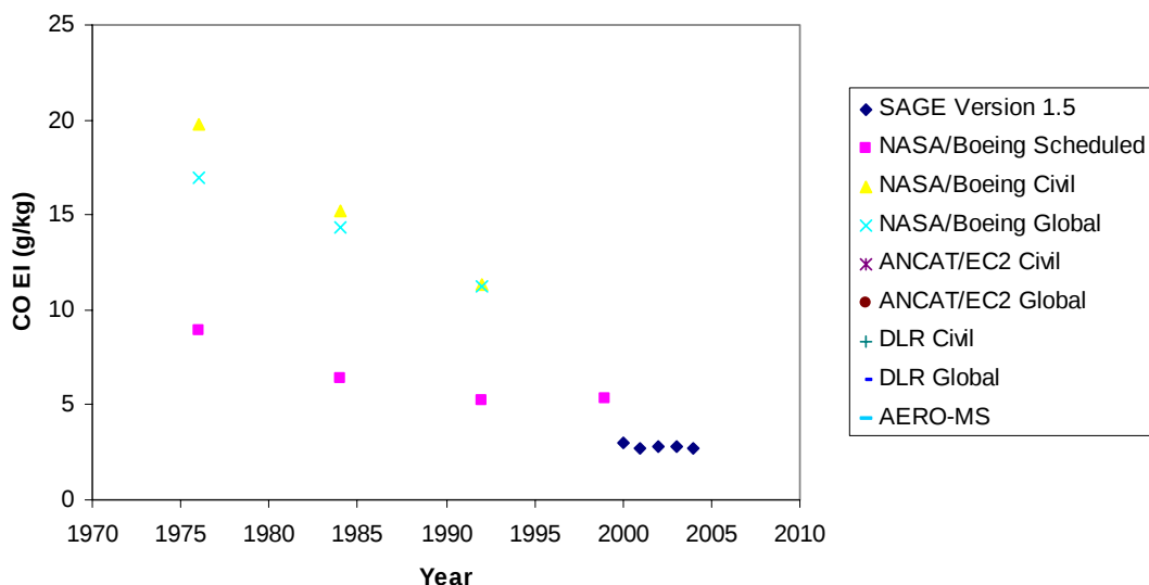
Figure 25. Comparison of SAGE Global Average CO EI Values with Past Studies
