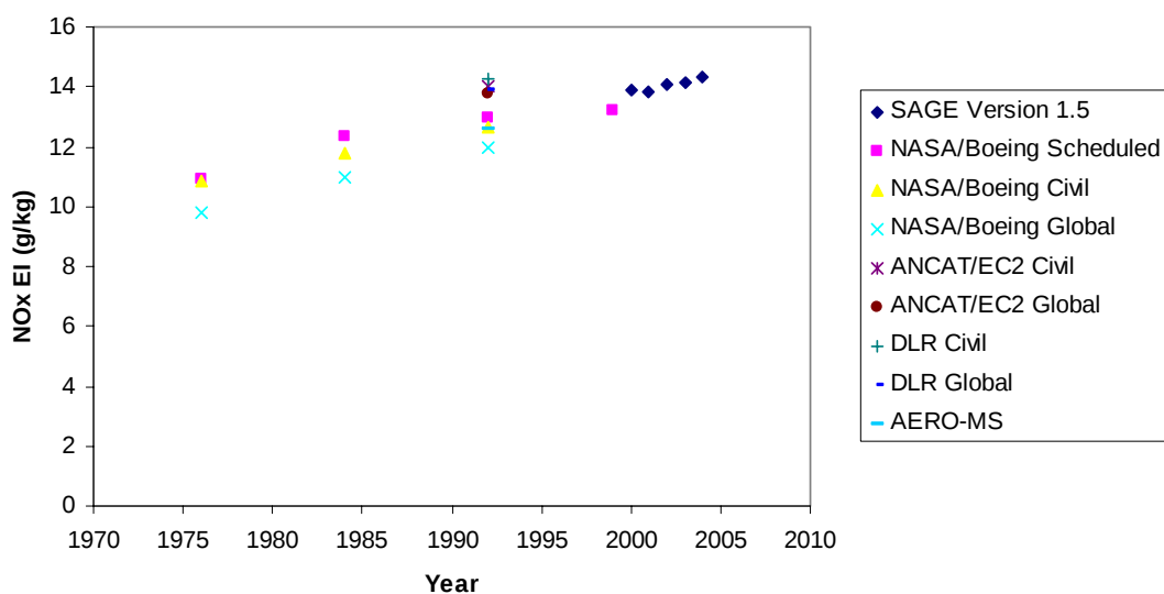
Figure 24. Comparison of SAGE Global Average NO x EI Values with Past Studies
