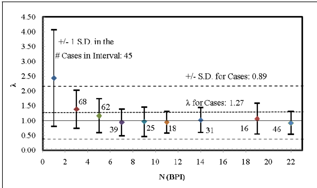
Figure 6.2: All EOID and BOR qualified 175 \lambda values plotted to blow count in 2 BPI intervals
