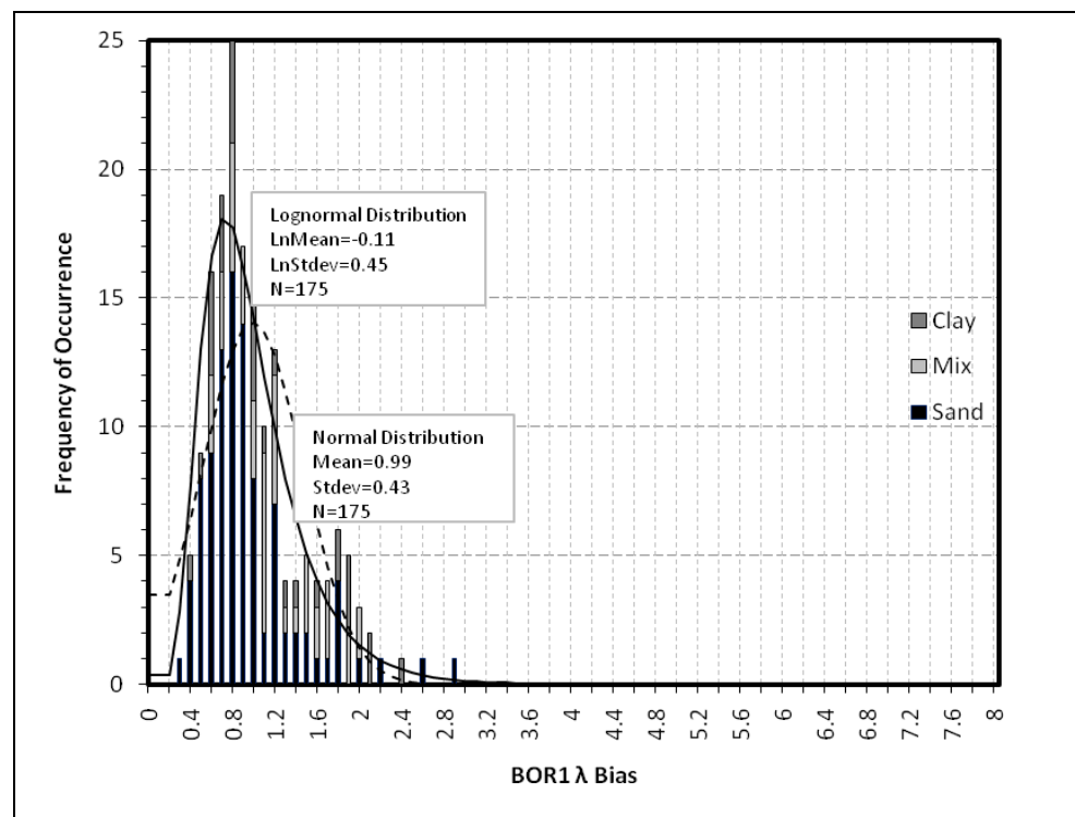
Figure 5.4: BOR \lambda histogram
