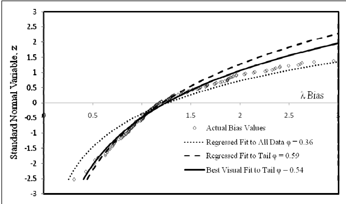
Figure 7.1: Scenario A Monte Carlo reliability method CDF fits at EOID
