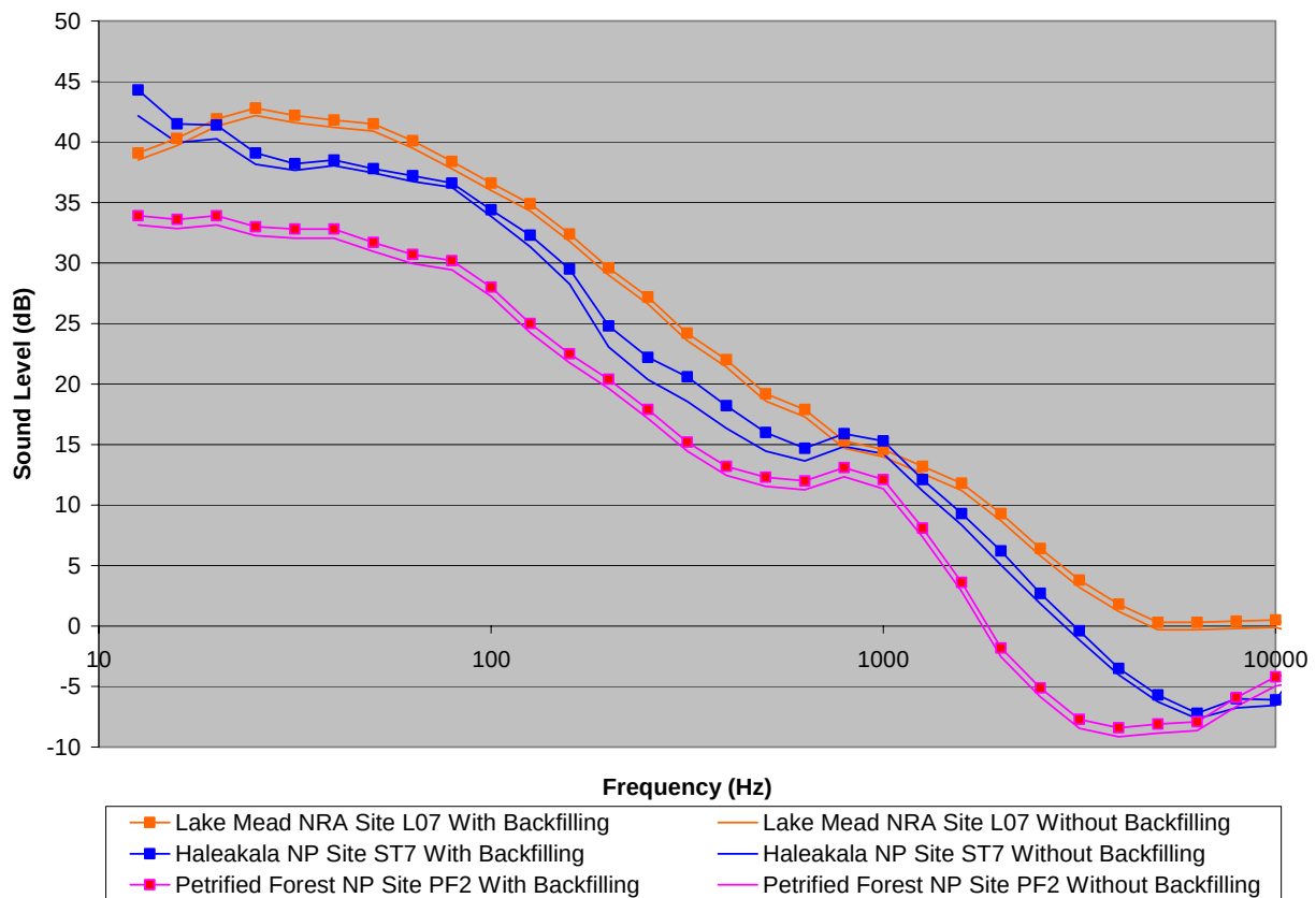
Figure 23. Comparison of natural ambient spectra with and without high-wind backfilling
