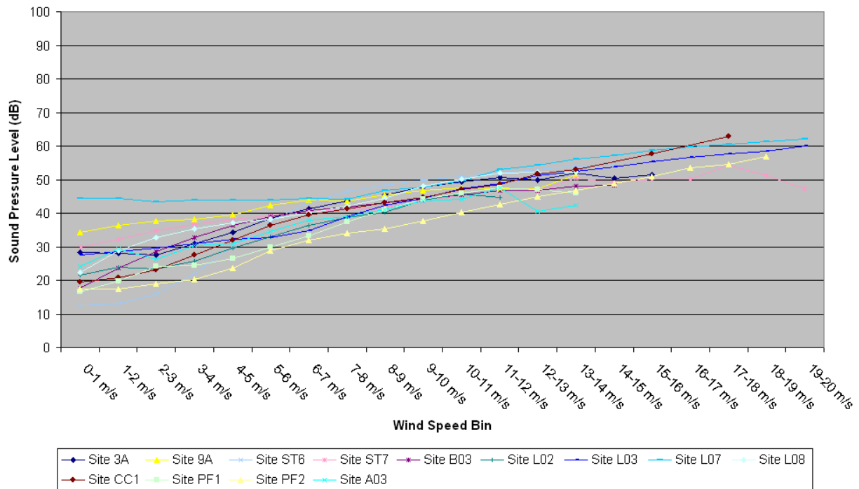
Figure 83. 1,000 Hz L_{eq} in 1-m/s wind speed bins by site.
