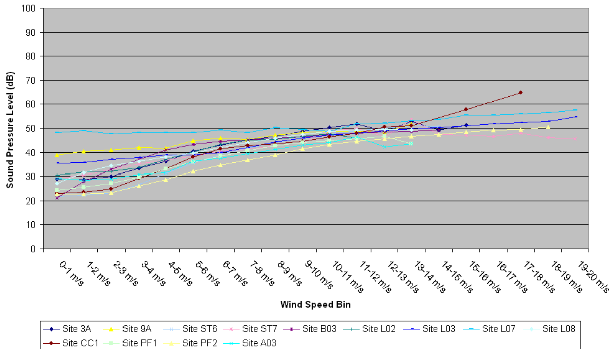
Figure 82. 500 Hz L_{eq} in 1-m/s wind speed bins by site.
