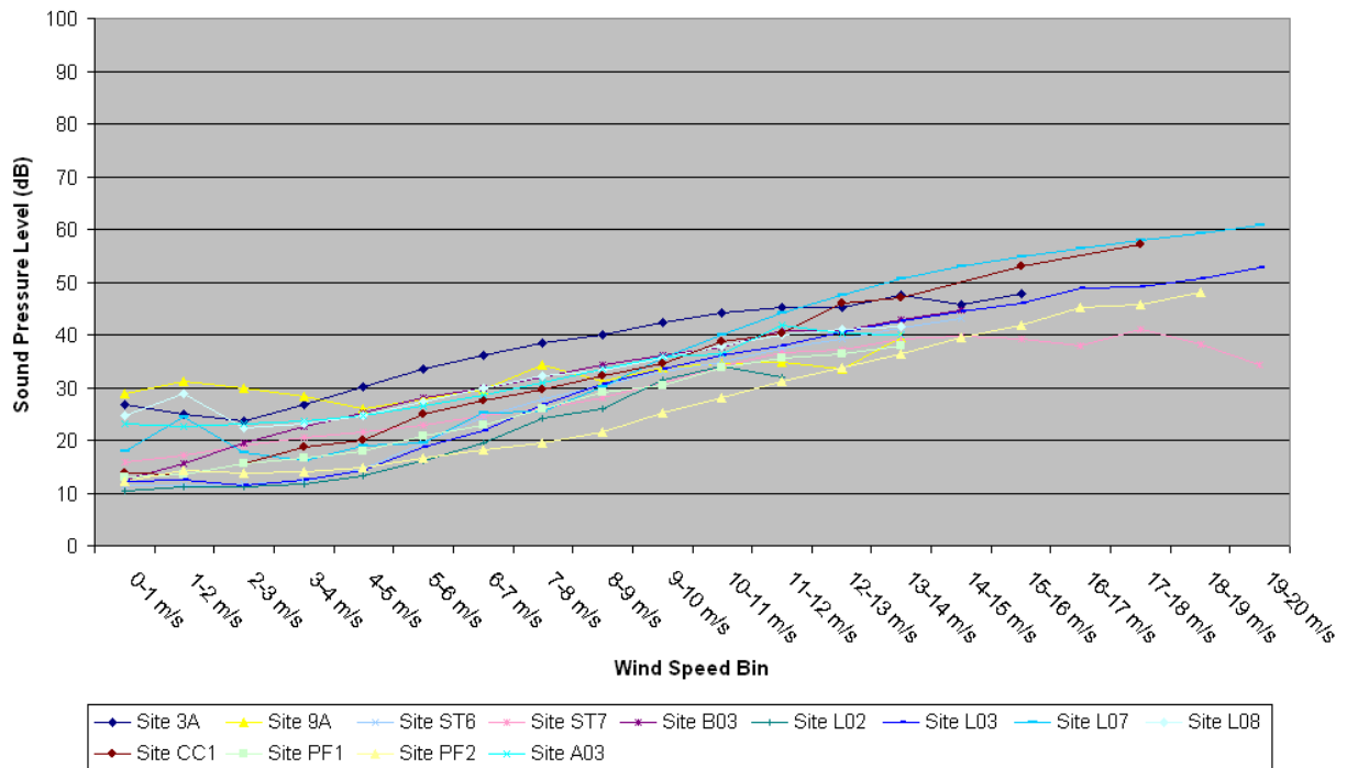
Figure 85. 10,000 Hz L_{eq} in 1-m/s wind speed bins by site.
