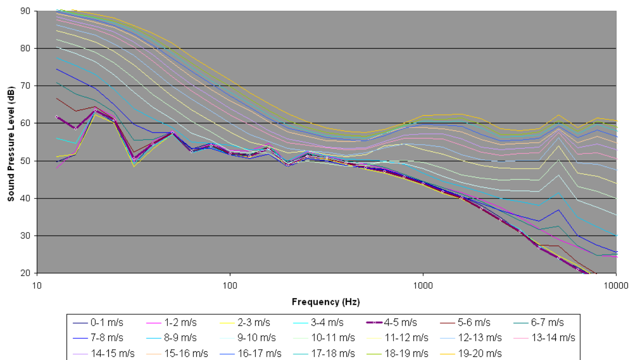
Figure 15. L_{eq} spectra for Lake Mead Site L07 in 1-m/s wind speed bins.
