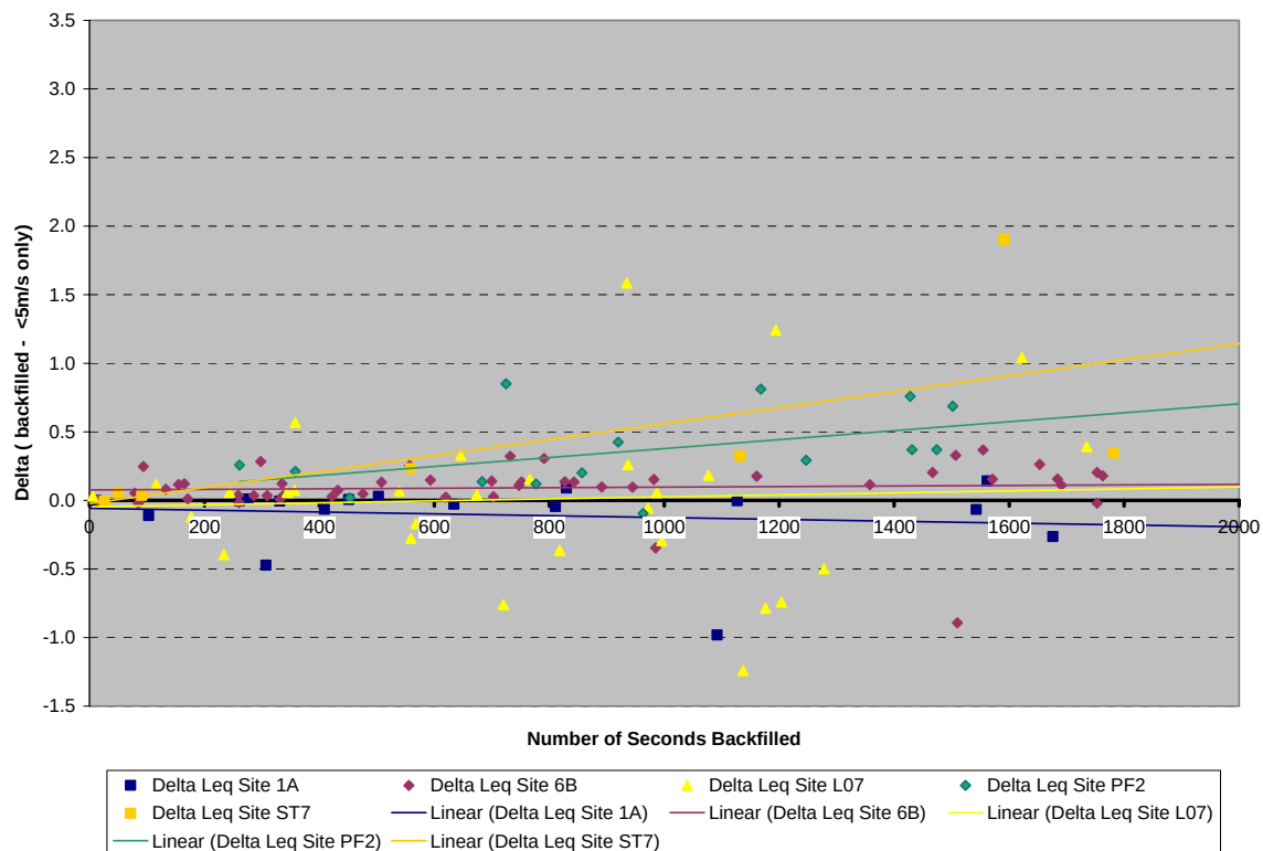
Figure 19. Comparison of L_{Aeq} computed with and without backfilled data
