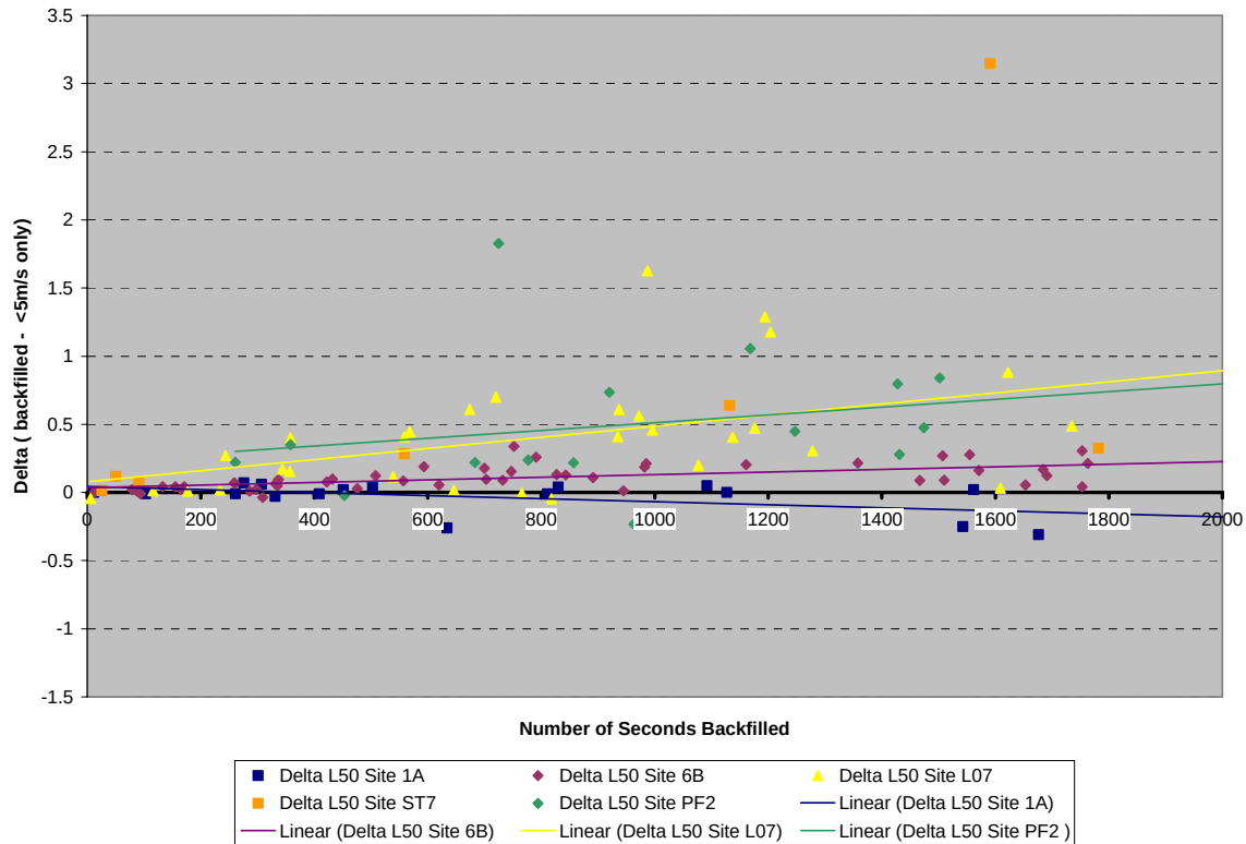
Figure 18. Comparison of L_{50} computed with and without backfilled data
