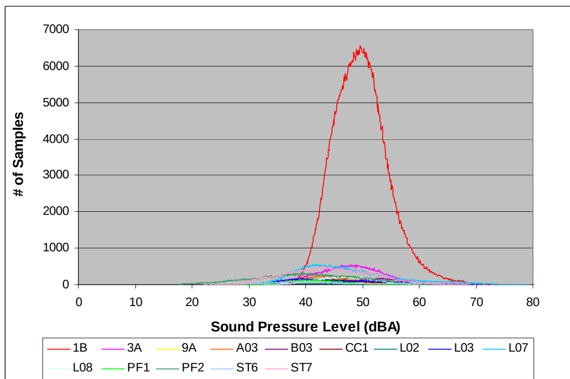
Figure 5. Sound pressure level distribution by site for high wind speeds (> 5 m/s)
