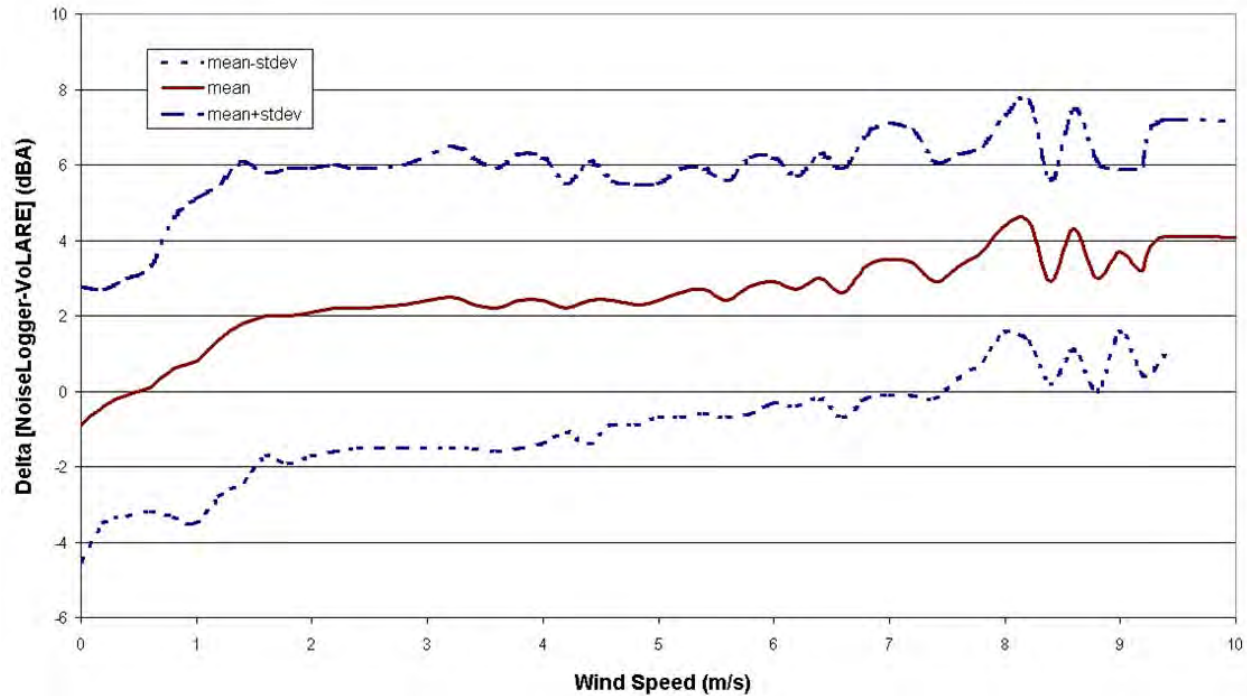
Figure 65. Average deltas between NoiseLogger™ and VoLARE data versus wind speed for 3 parks: Hawaii Volcanoes, Haleakala and Badlands.
