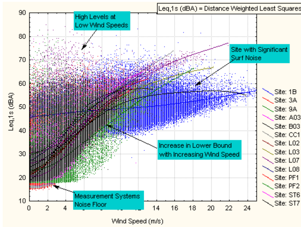
Figure 6. Scatter plot of high-wind dataset by site.
