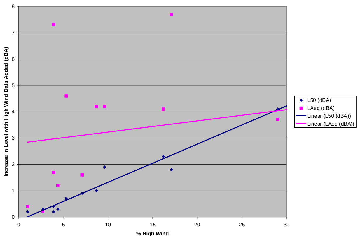
Figure 17. Increase in sound level as a function of % high-wind data added
