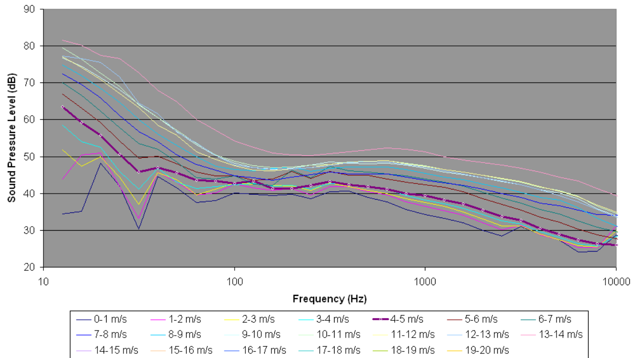
Figure 67. L_{eq} Spectra for Hawaii Volcanoes Site 9A in 1-m/s wind speed bins.
