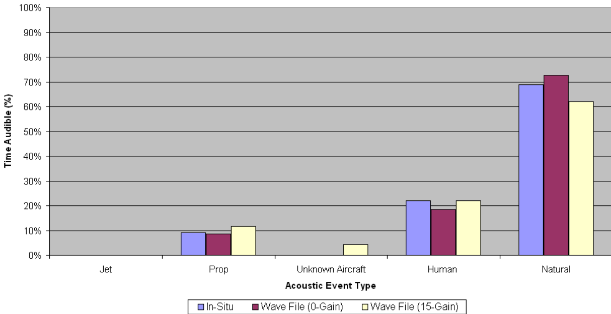
Figure 25. Comparison of in situ and off-site (using audio wave files) observer logging.
