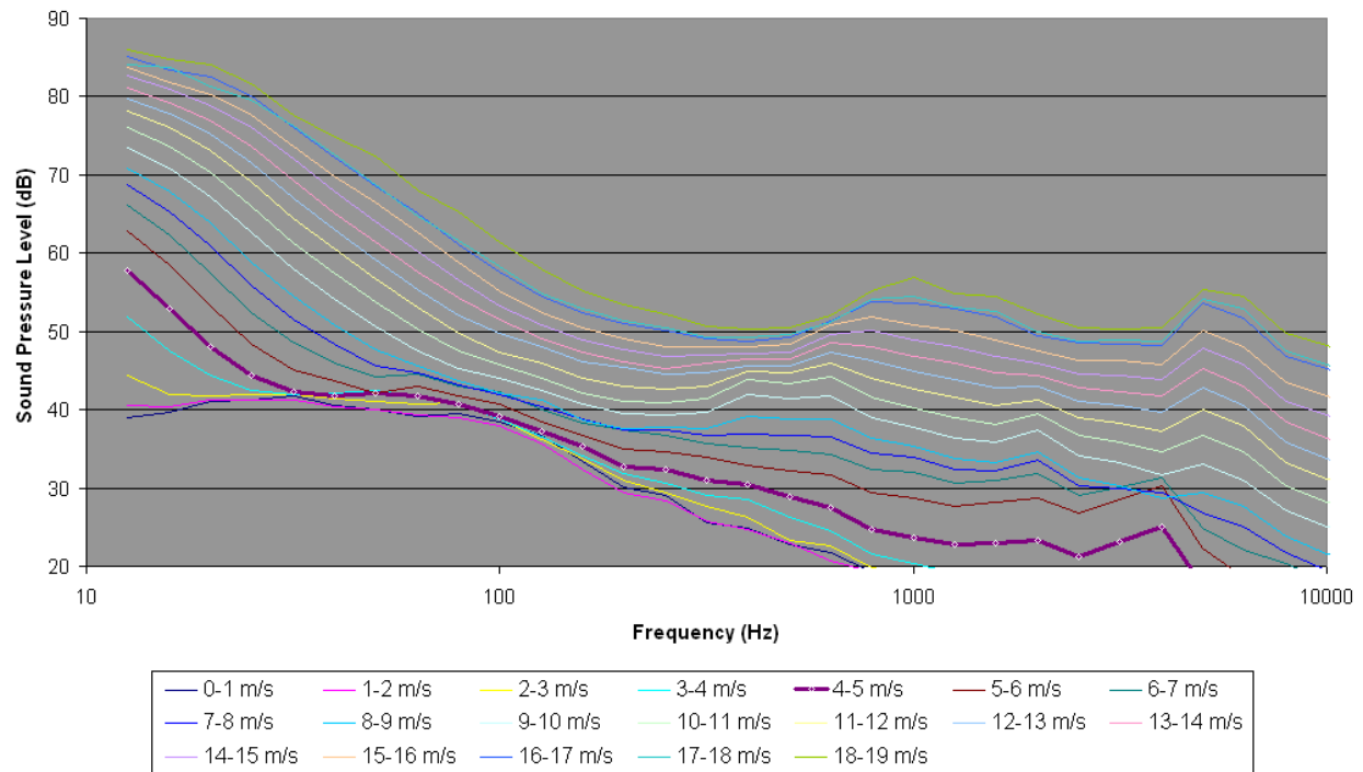
Figure 77. L_{eq} Spectra for Petrified Forest Site PF2 in 1-m/s wind speed bins.
