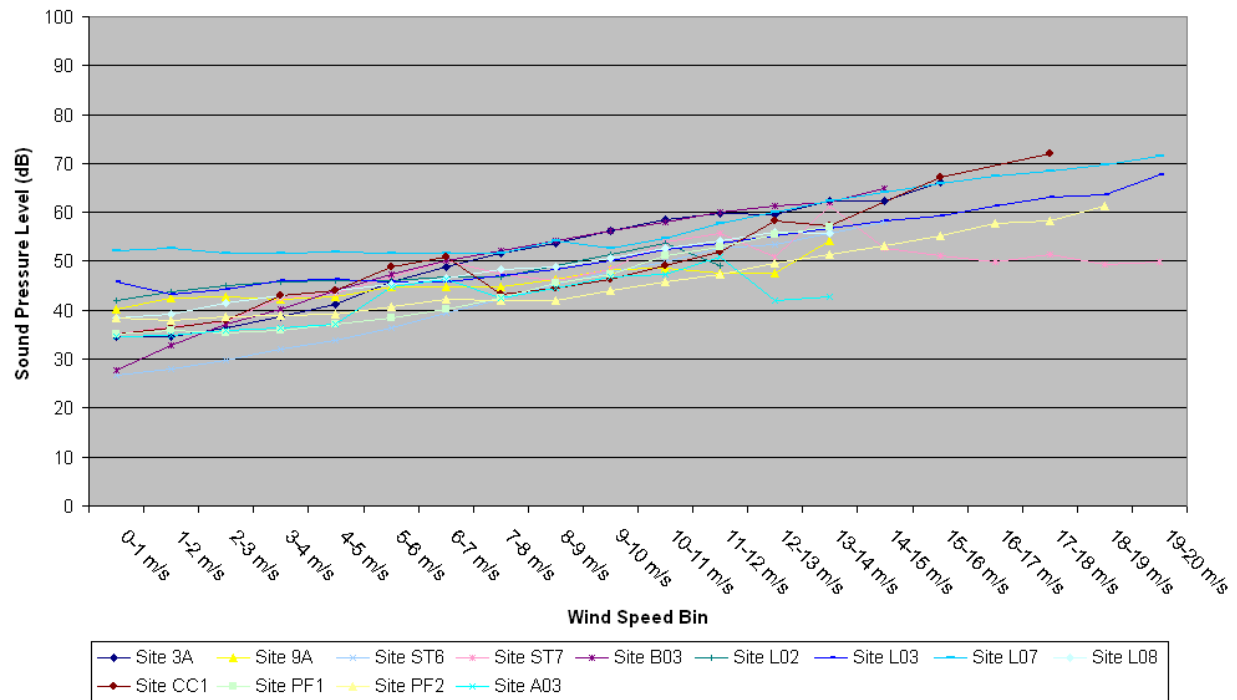
Figure 81. 100 Hz L_{eq} in 1-m/s wind speed bins by site.
