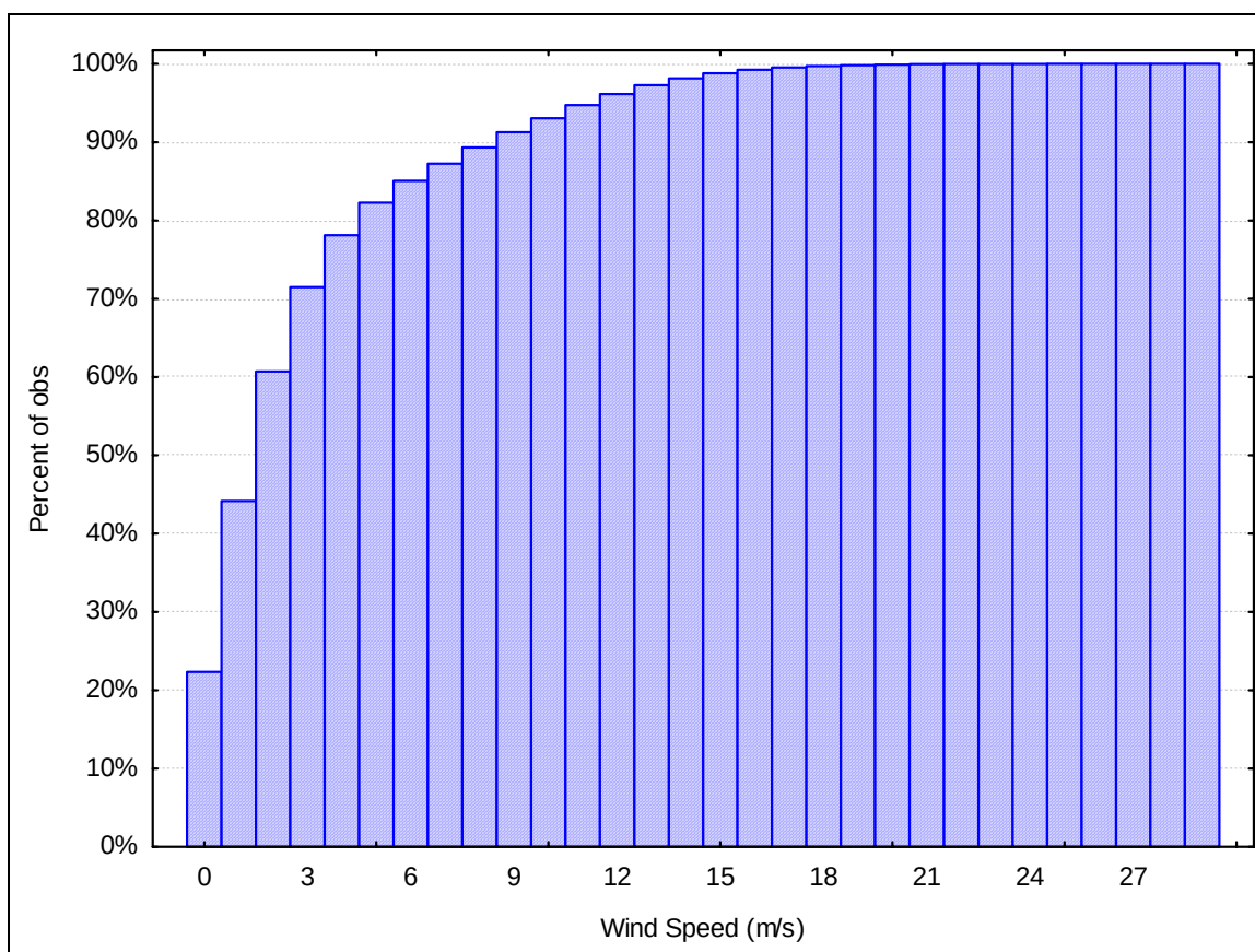
Figure 2. Cumulative wind-speed distribution of high-wind dataset.
