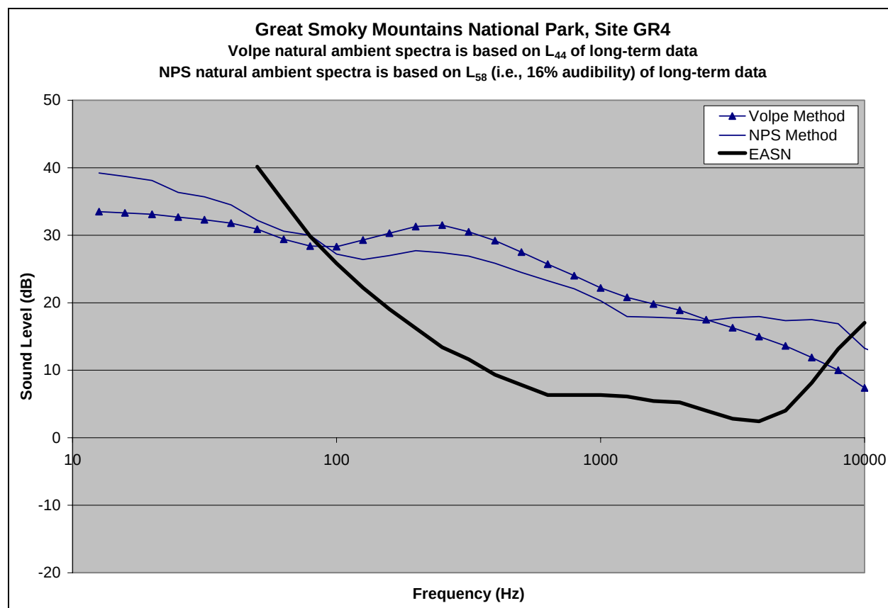
Figure 34. Great Smoky Mountains NP, Site GR4: Comparison of natural ambient spectra computed using Volpe and NPS methods
