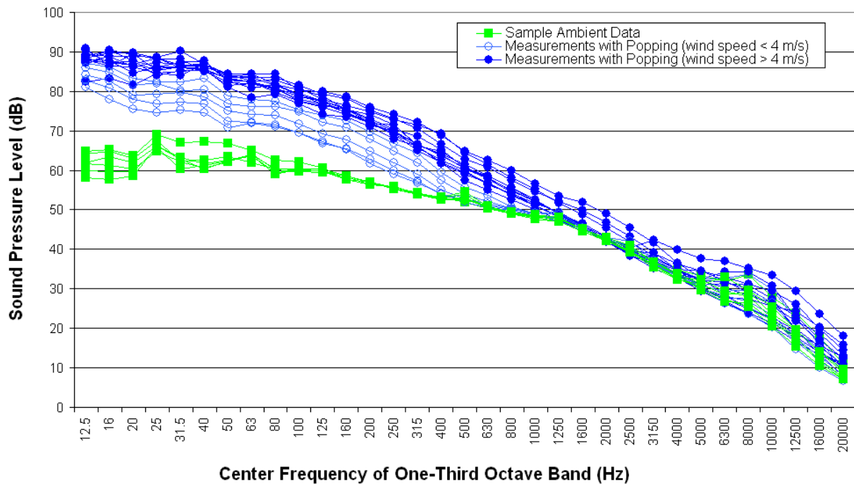
Figure 10. One-third octave band spectra for sample ambient data and measurements with popping.
