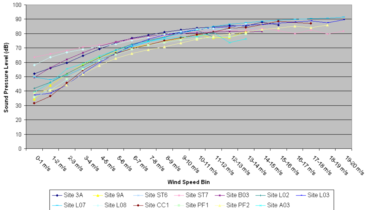
Figure 79. 12.5 Hz L_{eq,1s} in 1-m/s wind speed bins by site.
