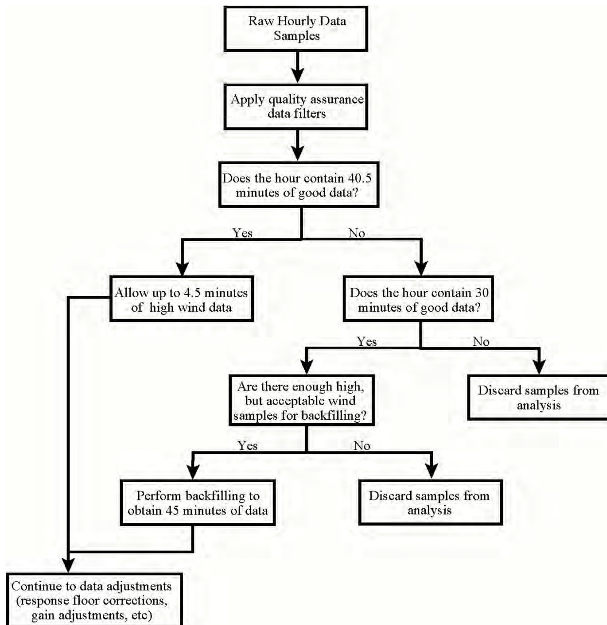
Figure 24. Recommended procedure for the processing of high-wind data.
