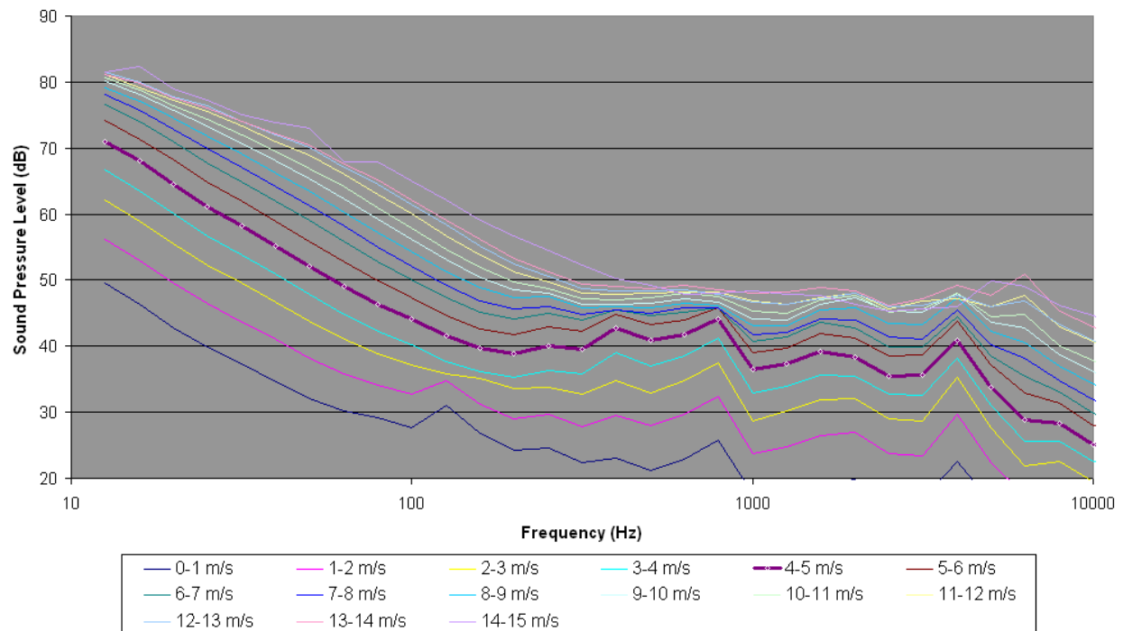
Figure 70. L_{eq} Spectra for Badlands Site B03 in 1-m/s wind speed bins.
