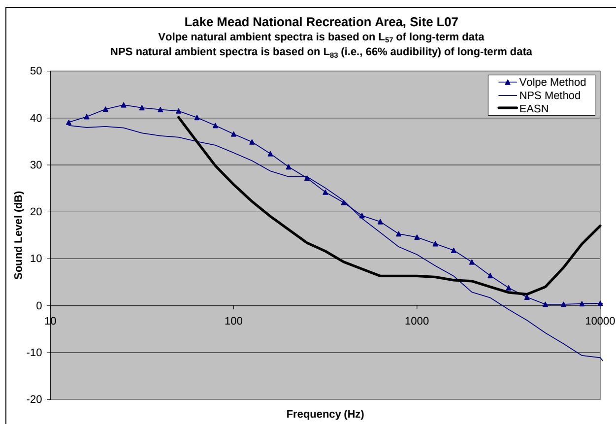
Figure 33. Lake Mead NRA, Site L07: Comparison of natural ambient spectra computed using Volpe and NPS methods
