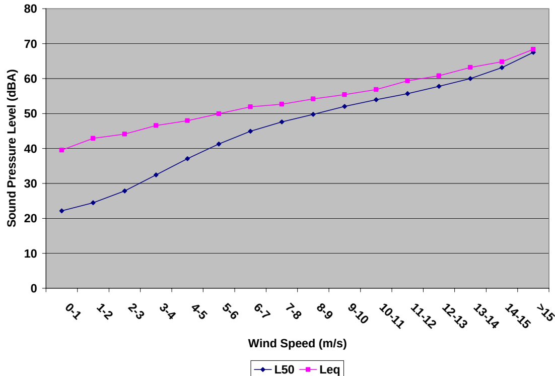
Figure 9. Computed L_{50} and L_{Aeq} for wind speeds in 1 m/s bins.
