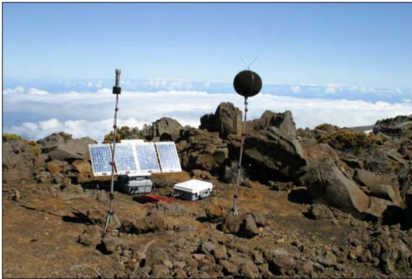
Figure 44. Haleakala National Park Site ST7 - Kalahaku Overlook (13 days – March 1, 2003 to March 13, 2003)
