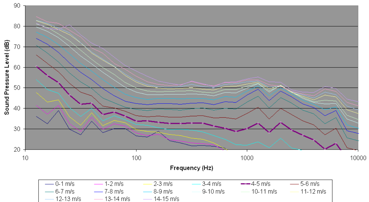
Figure 68. L_{eq} Spectra for Haleakala Site ST6 in 1-m/s wind speed bins.
