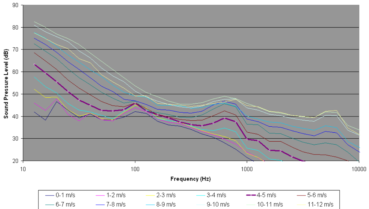
Figure 71. L_{eq} Spectra for Lake Mead Site L02 in 1-m/s wind speed bins.
