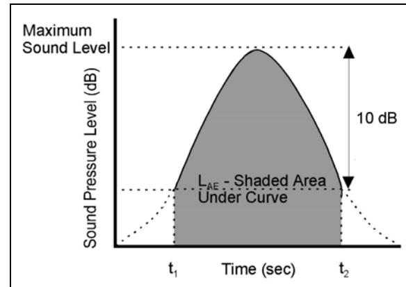
Figure 86. Graphical representation of L_{AE} .
