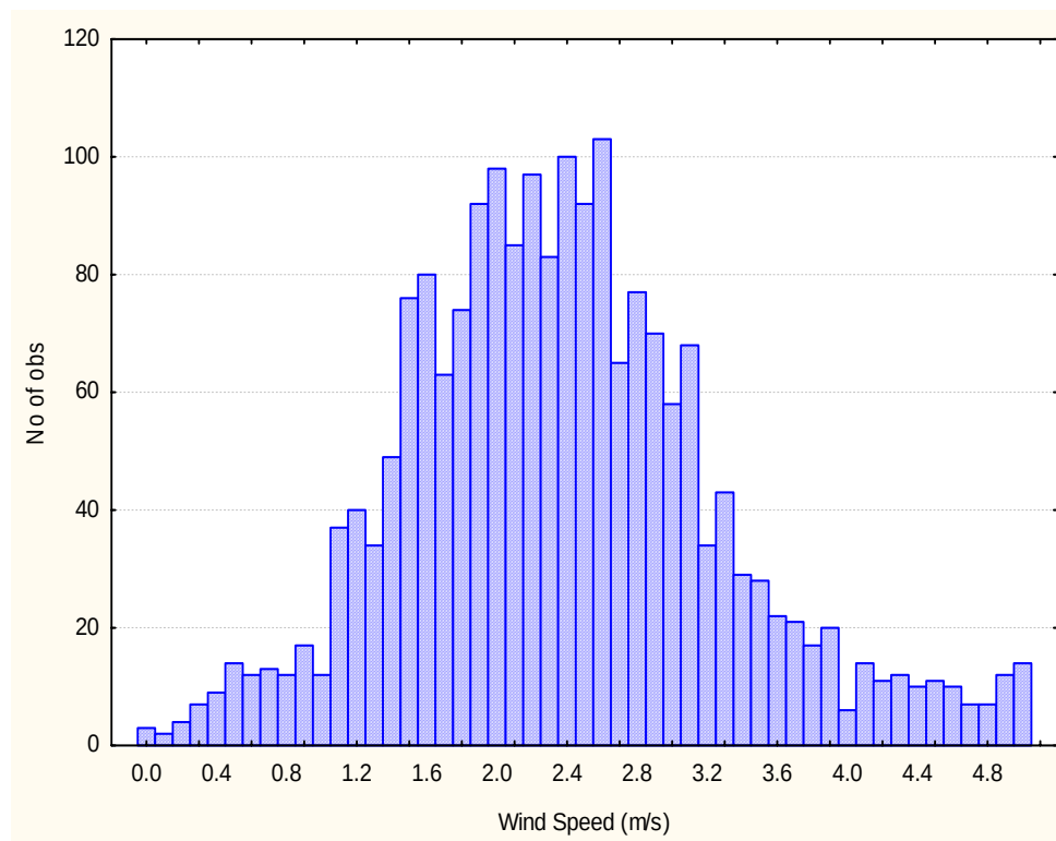
Figure 21. Wind Speed Distribution for 9/19, 1300 hour at Site PF2
