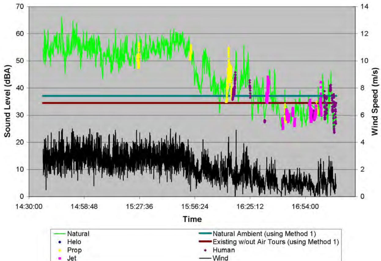
Figure 30. Time history of measured sound levels correlated with observer logging at Great Smoky Mountains National Park Site GR4.
