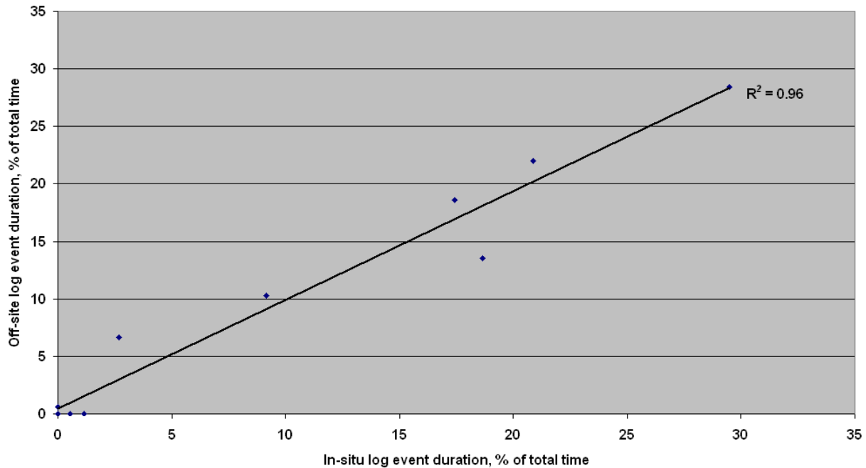
Figure 27. Audibility duration for observer logged events for Sites A02 and GR4 (Event durations are derived from a combination of logs from three days for A02 and four days for GR4).*
