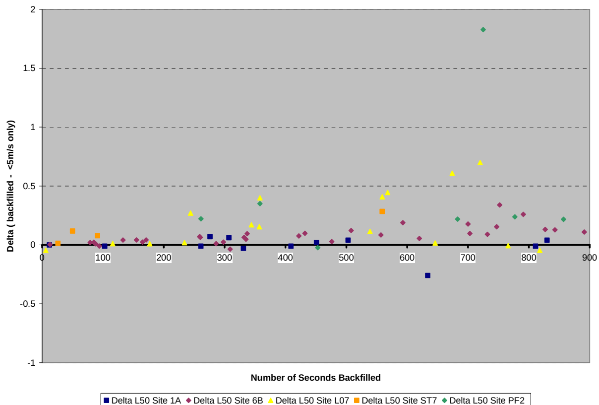
Figure 22. Change in L_{50} due to backfilling using the final procedure
