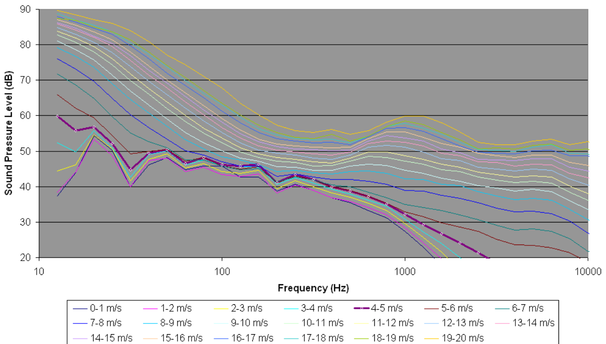
Figure 72. L_{eq} Spectra for Lake Mead Site L03 in 1-m/s wind speed bins.
