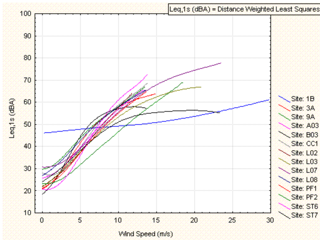
Figure 7. Distance-weighted least-squares line fits by site.
