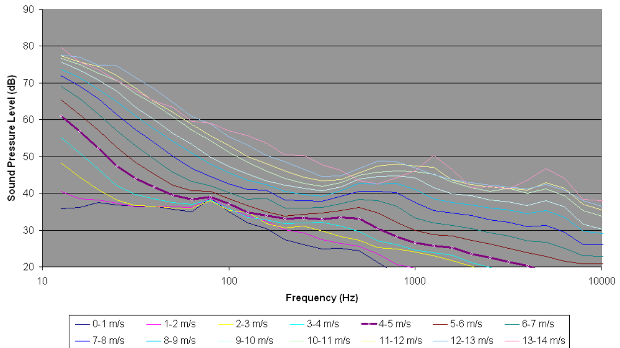
Figure 76. L_{eq} Spectra for Petrified Forest Site PF1 in 1-m/s wind speed bins.
