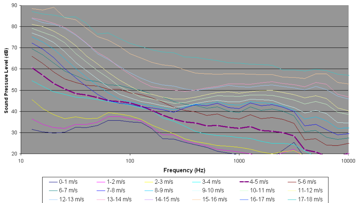
Figure 16. L_{eq} spectra for Canyon de Chelly Site CC1 in 1-m/s wind speed bins.
