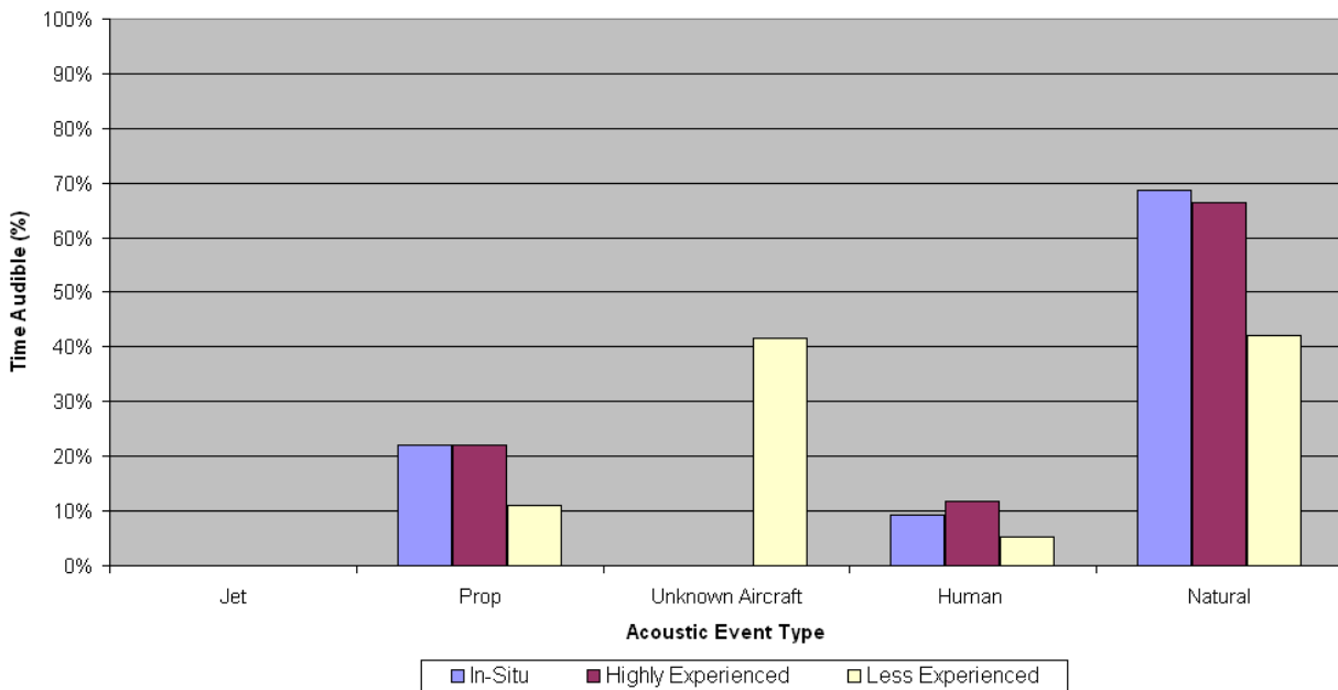
Figure 26. Comparison of in situ and off-site (using audio wave files) observer logging for different levels of observer experience.
