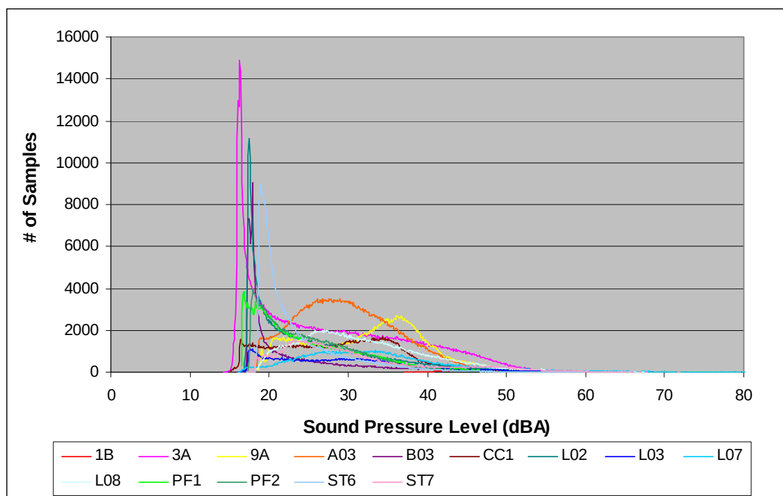
Figure 4. Sound pressure level distribution by site for low wind speeds (< 5 m/s).
