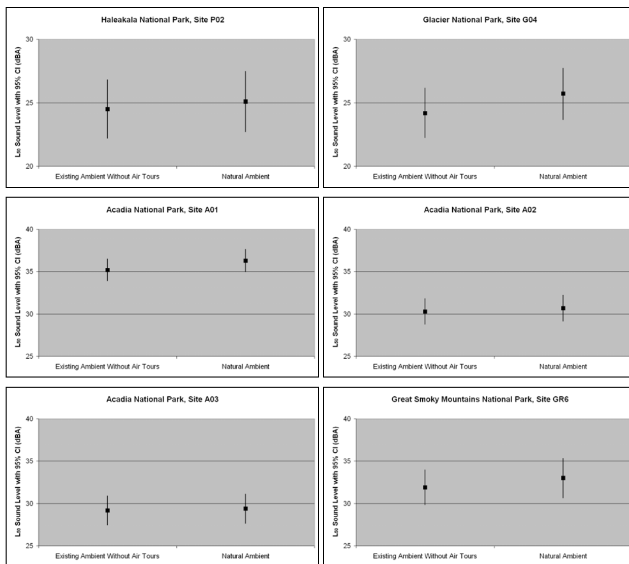
Figure 32. Comparison of 95% confidence intervals for sites where natural ambient is greater than existing ambient without air tours.
