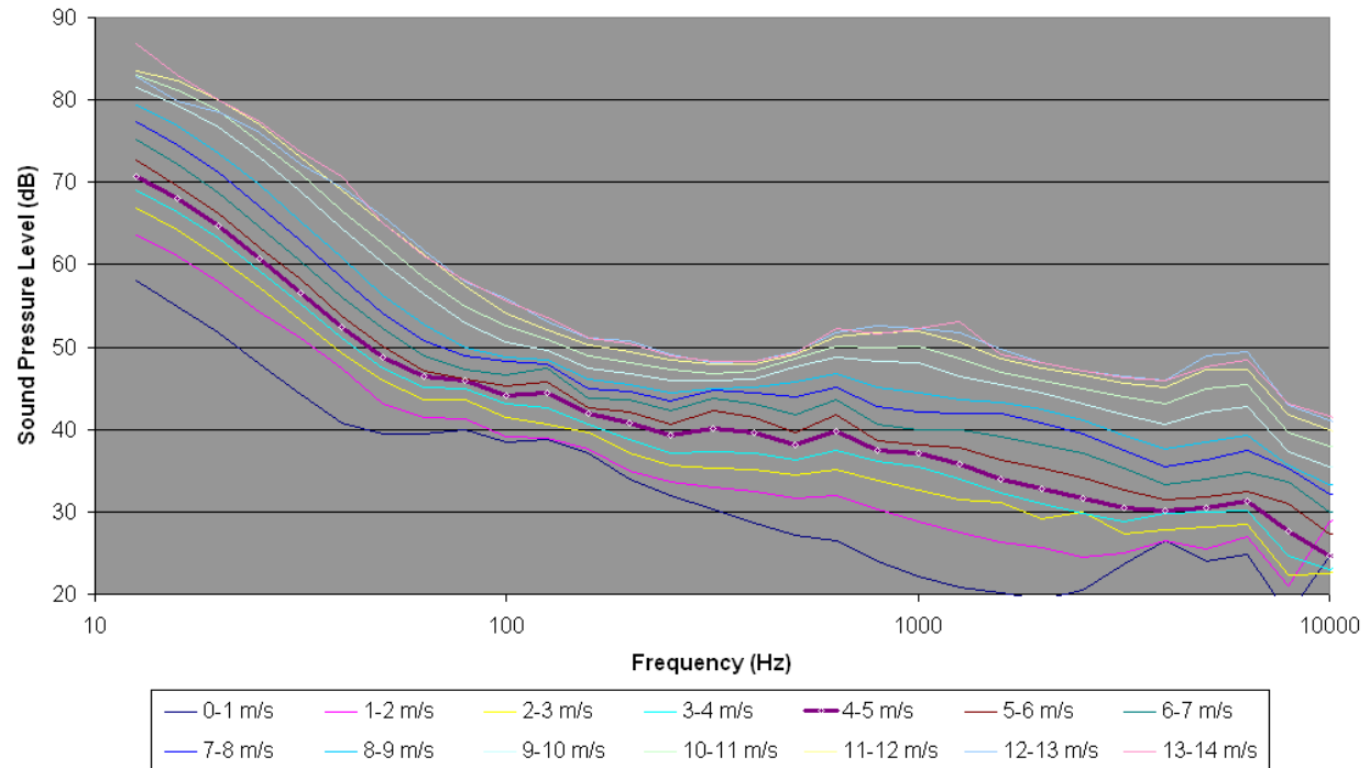
Figure 74. L_{eq} Spectra for Lake Mead Site L08 in 1-m/s wind speed bins.
