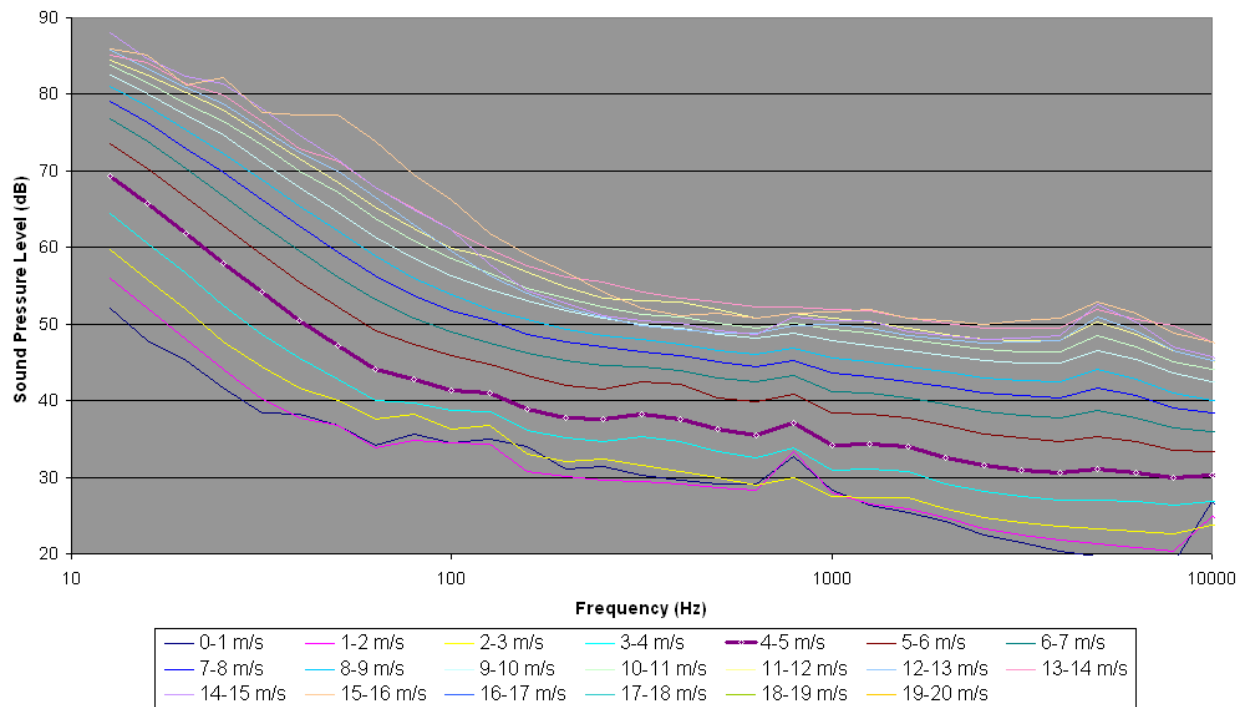
Figure 66. L_{eq} Spectra for Hawaii Volcanoes Site 3A in 1-m/s wind speed bins.
