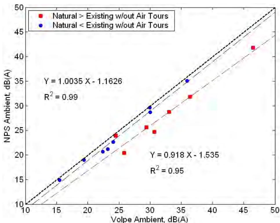
Figure 31. Correlation between ambient computation methods.
