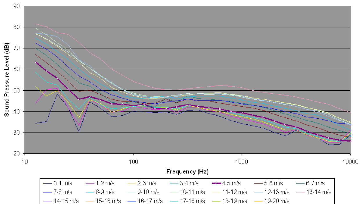
Figure 13. L_{eq} spectra for Hawaii Volcanoes Site 9A in 1-m/s wind speed bins.
