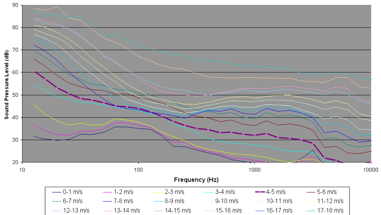
Figure 75. L_{eq} Spectra for Canyon de Chelly Site CC1 in 1-m/s wind speed bins.
