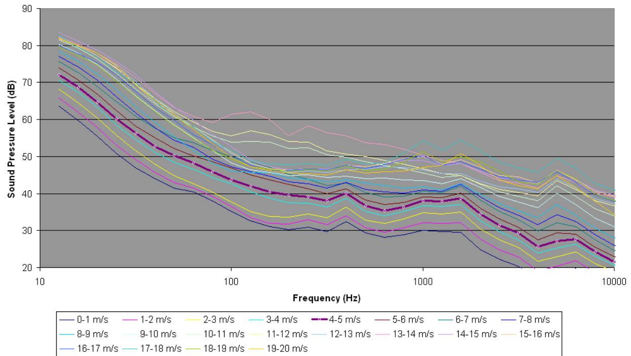
Figure 69. L_{eq} Spectra for Haleakala Site ST7 in 1-m/s wind speed bins.
