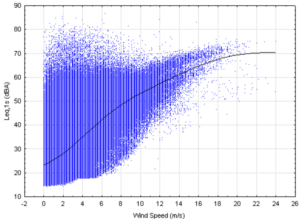
Figure 8 Cumulative wind-speed distribution of high-wind test dataset
