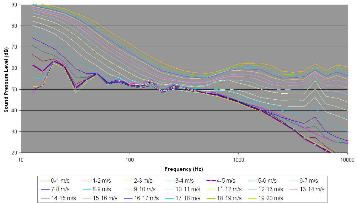
Figure 73. L_{eq} Spectra for Lake Mead Site L07 in 1-m/s wind speed bins.
