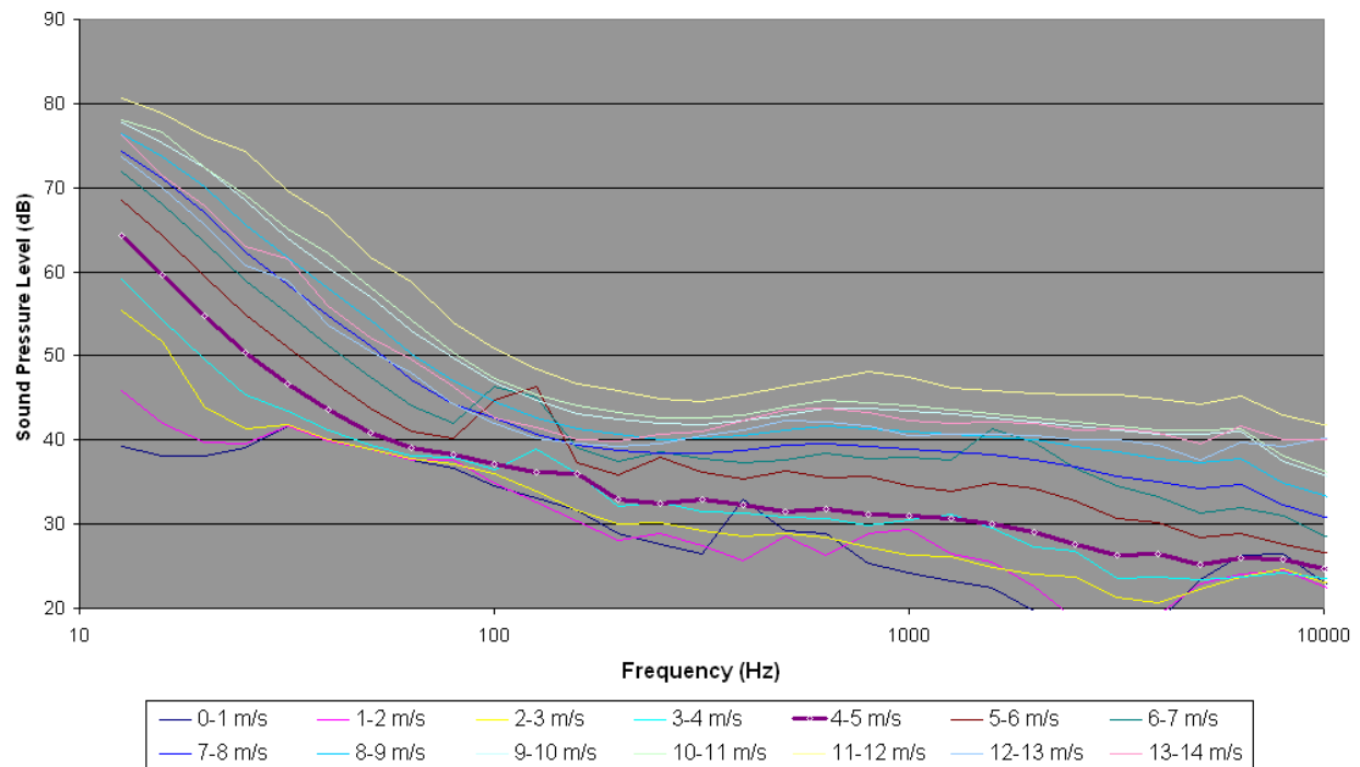
Figure 78. L_{eq} Spectra for Acadia Site A03 in 1-m/s wind speed bins.
