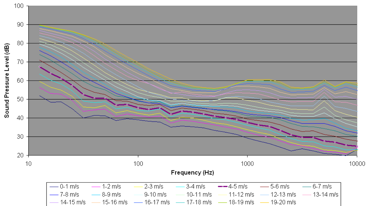
Figure 12. L_{eq} Spectra for all sites in 1-m/s wind speed bins.
