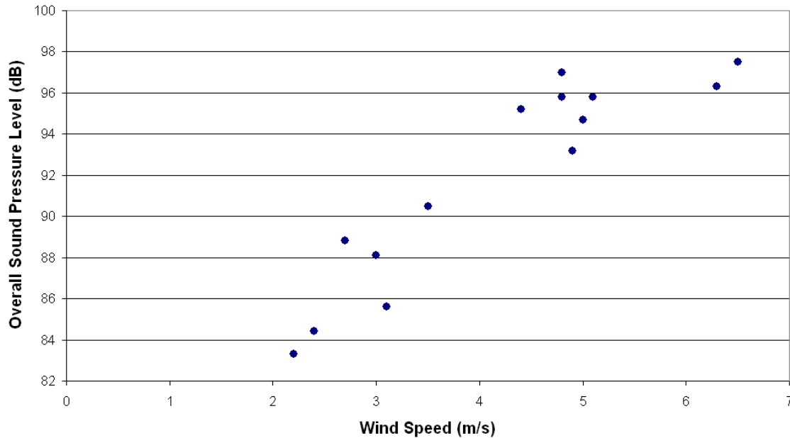
Figure 11. Relationship between wind speed and sound pressure level of popping sounds.
