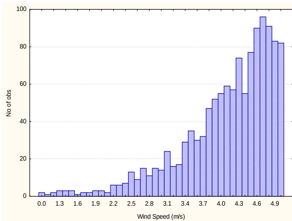
Figure 20. Wind Speed Distribution for 9/13, 1300 hour at Site PF2
