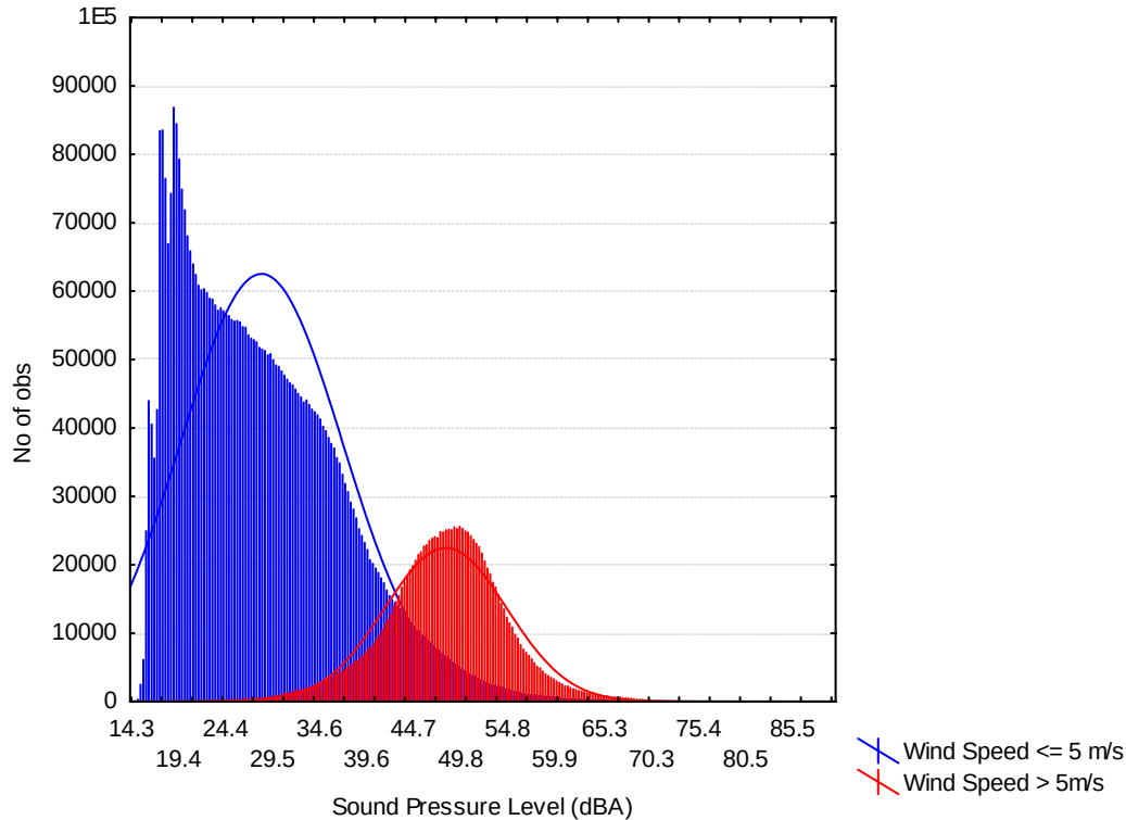
Figure 3. Distribution of sound pressure levels in high-wind dataset.
