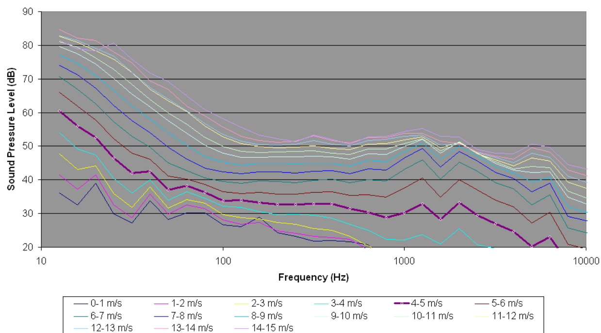
Figure 14. L_{eq} spectra for Haleakala Site ST6 in 1-m/s wind speed bins.
