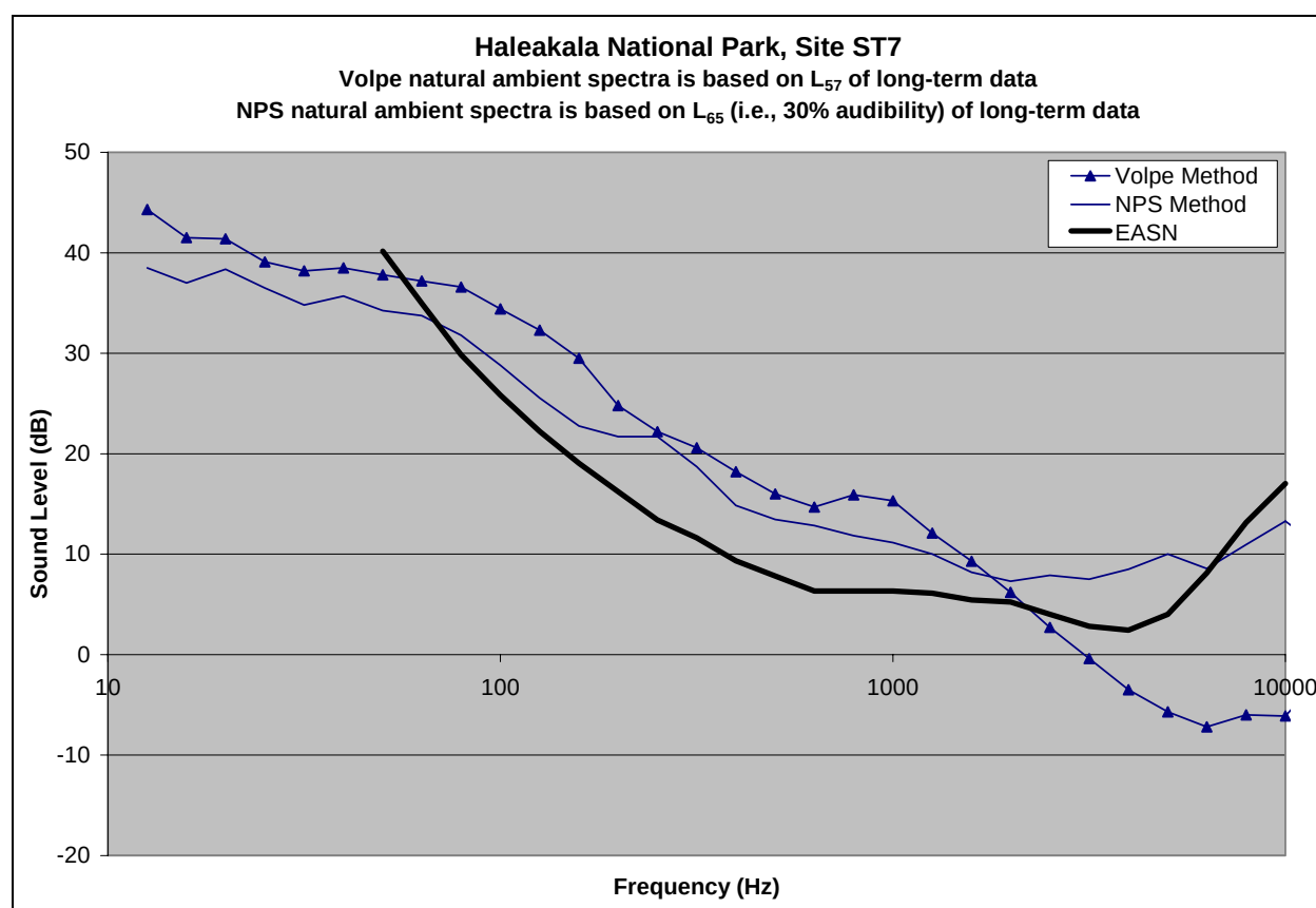
Figure 35. Haleakala NP, Site ST7: Comparison of natural ambient spectra computed using Volpe and NPS methods
