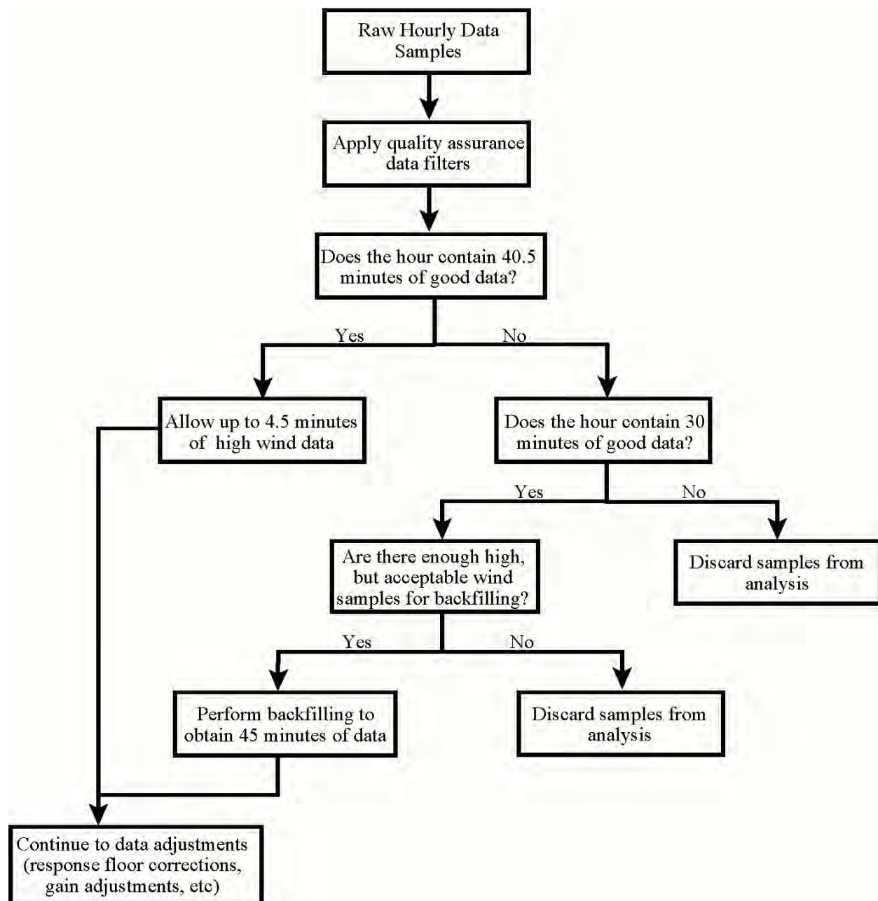
Figure 1. Recommended method for the processing of high-wind data.
