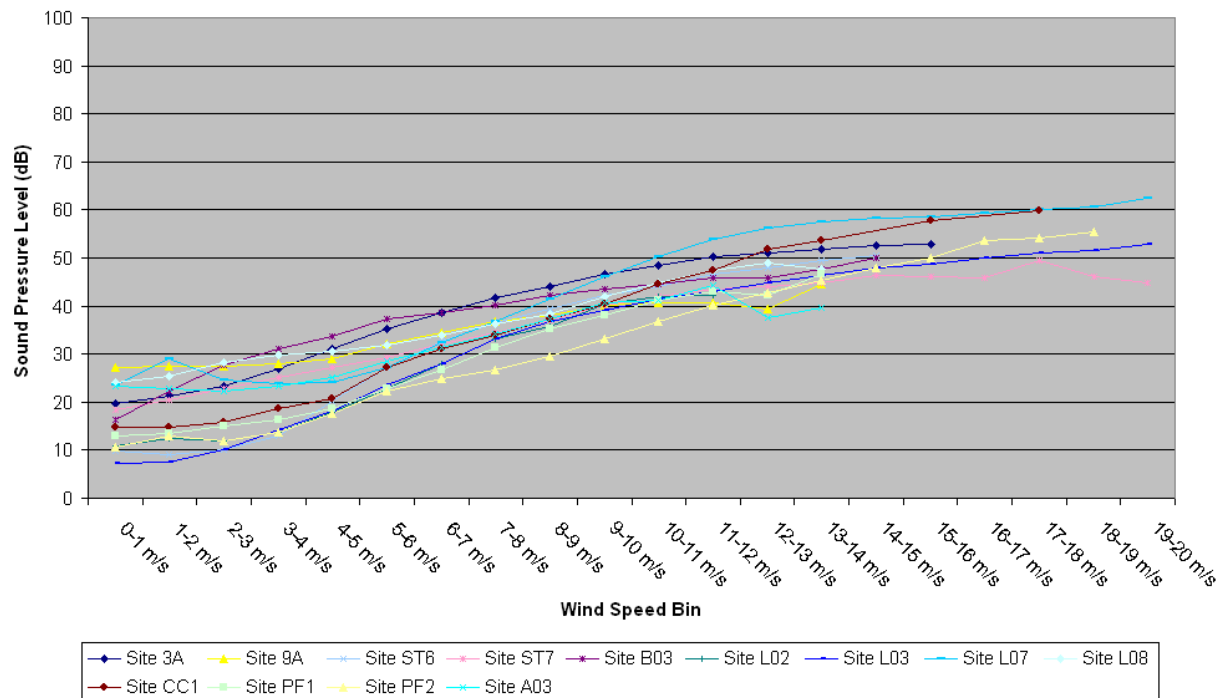
Figure 84. 5,000 Hz L_{eq} in 1-m/s wind speed bins by site.
