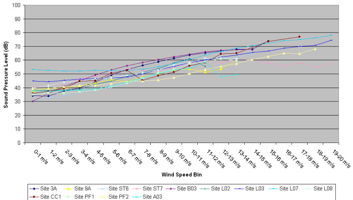
Figure 80. 50 Hz L_{eq,1s} in 1-m/s wind speed bins by site.
