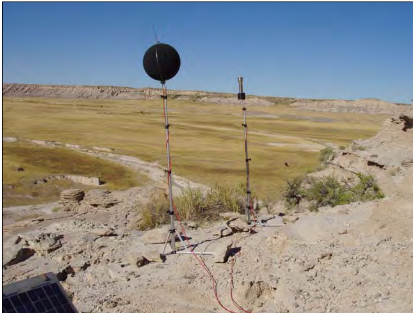
Figure 46. Badlands National Park Site B03 - Cedar Butte (12 days – September 14, 2003 to September 25, 2003)
