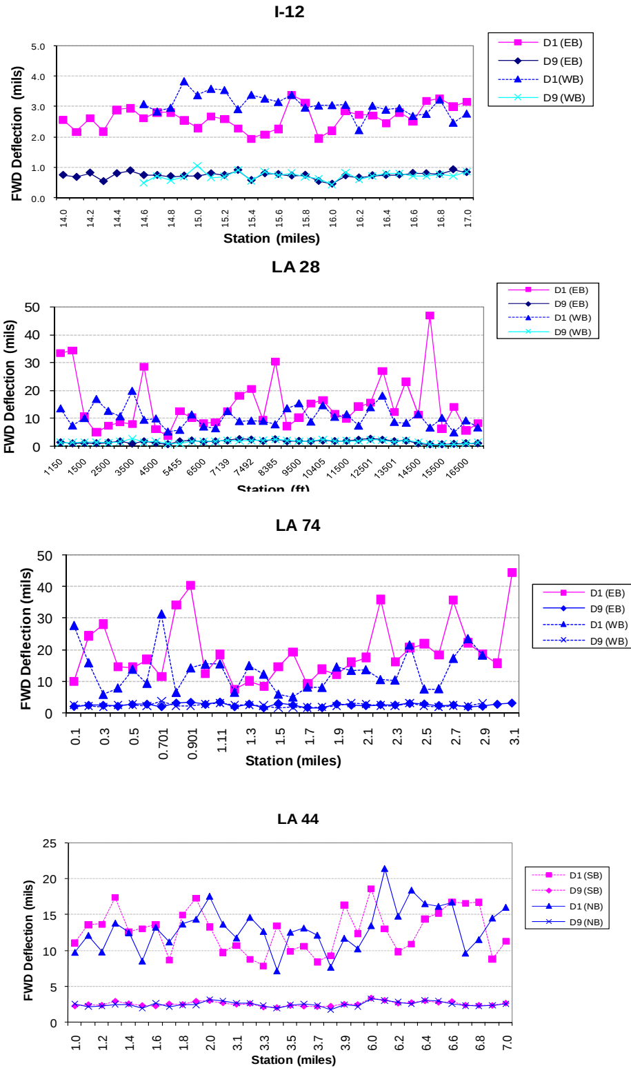
Figure 6 Comparison of Phase-I FWD deflections
