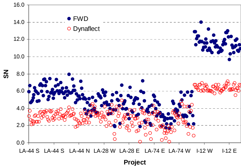
(a) SN_{eff} obtained from FWD and Dynaflect
