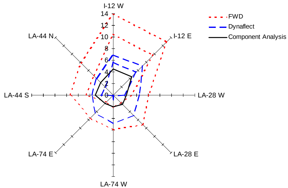
(b) SN_{eff} ranges from FWD, Dynaflect and condition survey
