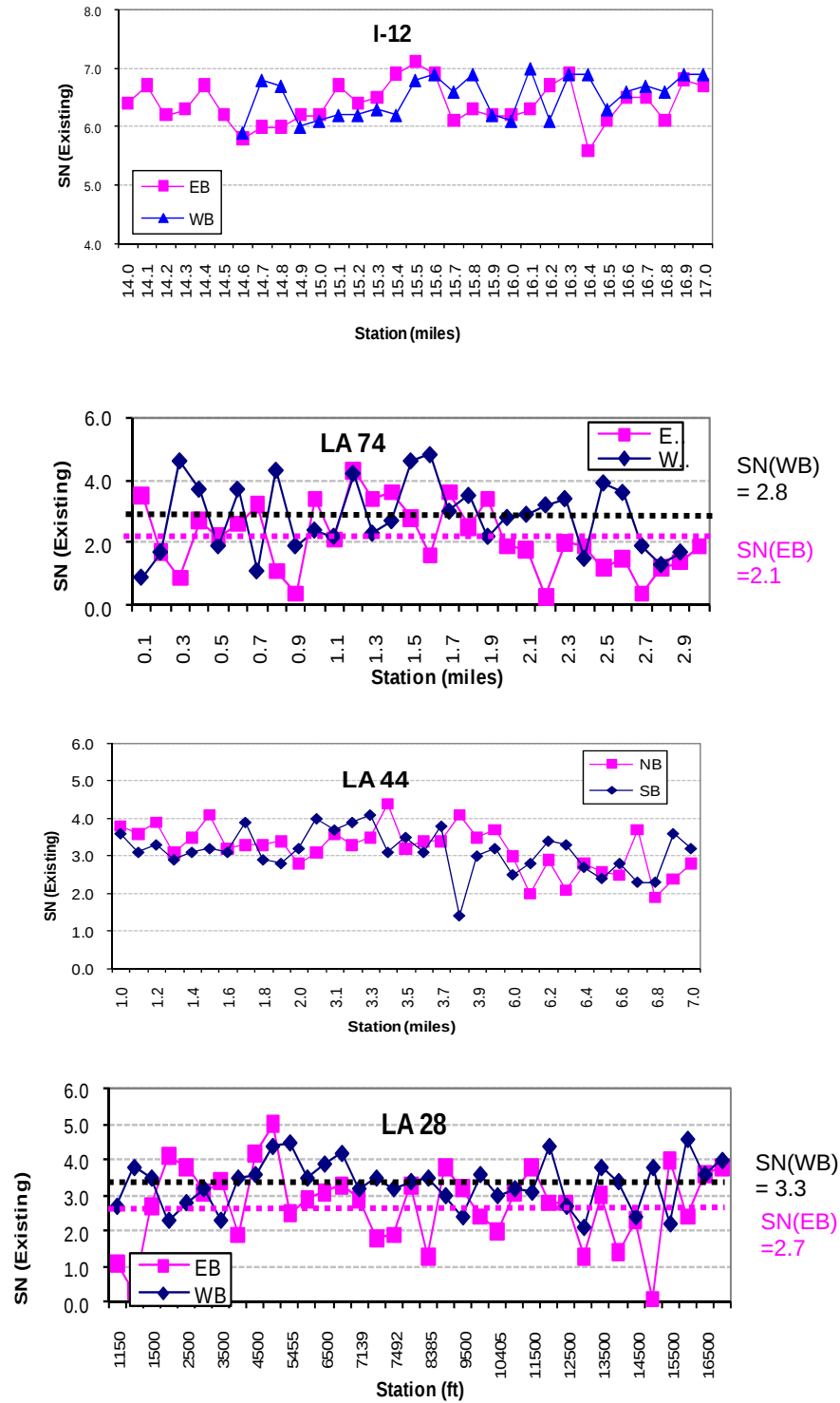
Figure 7 Dynalect estimated SN values of Phase-I projects
