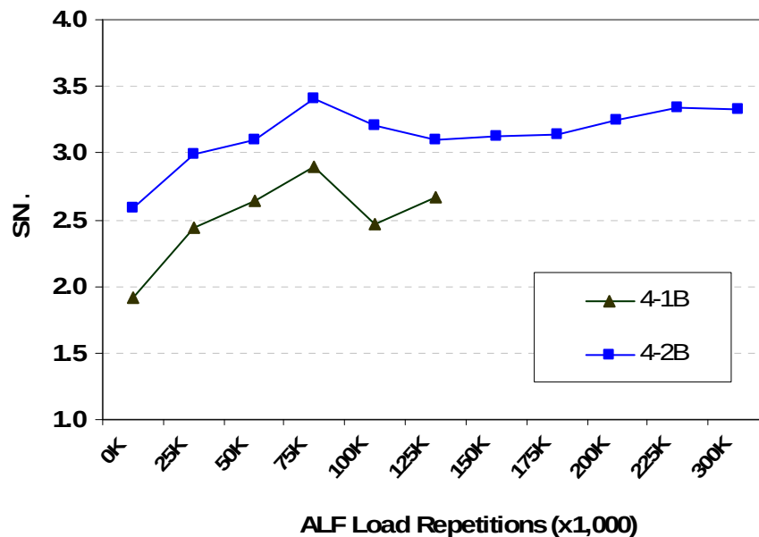
Figure 61 Dynaffect structural number results
