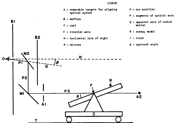
Figure A-1. Schematic diagram of apparatus.
