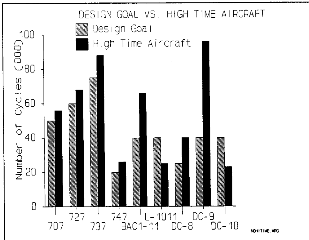
Figure 3. Comparison of design age with actual age of highest time aircraft in fleet.
