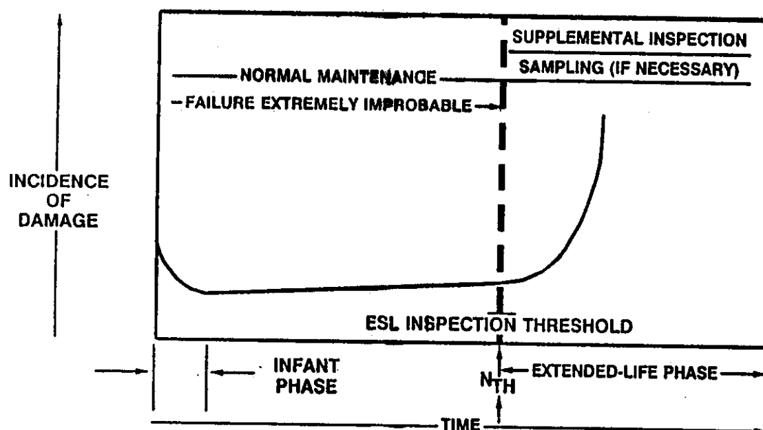
Figure 1. When in the life of an aircraft does damage occur?
