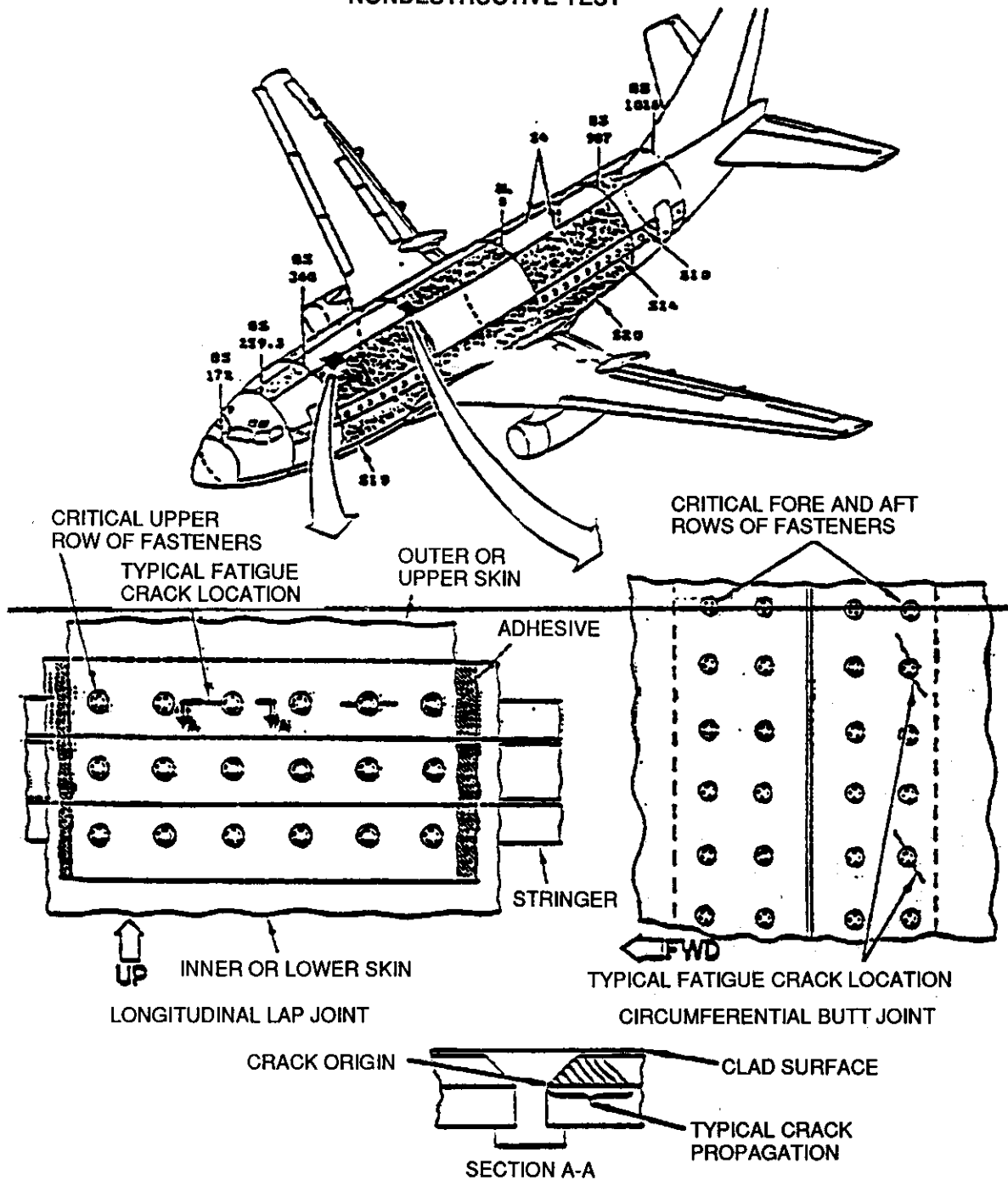
Figure 6. Typical fuselage skin joint configuration and crack orientation .
