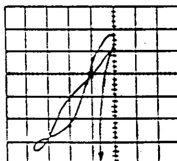
(B) EDDY CURRENT RESPONSE FROM CORROSION USING 20 KHz, 1/2-IN.-DIAMETER PROBE
