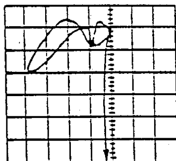
(C) EDDY CURRENT RESPONSE FROM CORROSION USING 50-KHz, 1/4-IN.-DIAMETER PROBE
