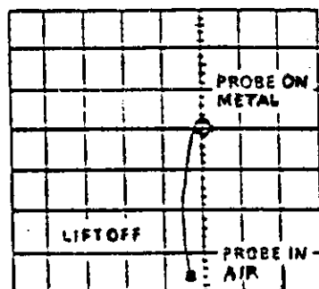
(A) EDDY CURRENT RESPONSE NO CORROSION
