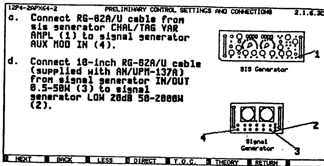
Figure 1. IMIS Prototype
