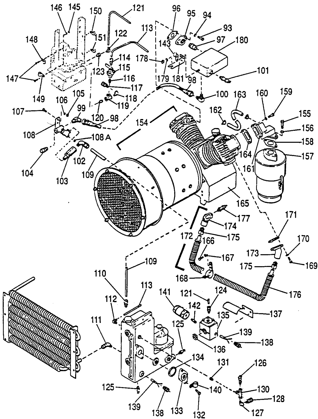
AIR COMPRESSOR EXPLODED VIEW
