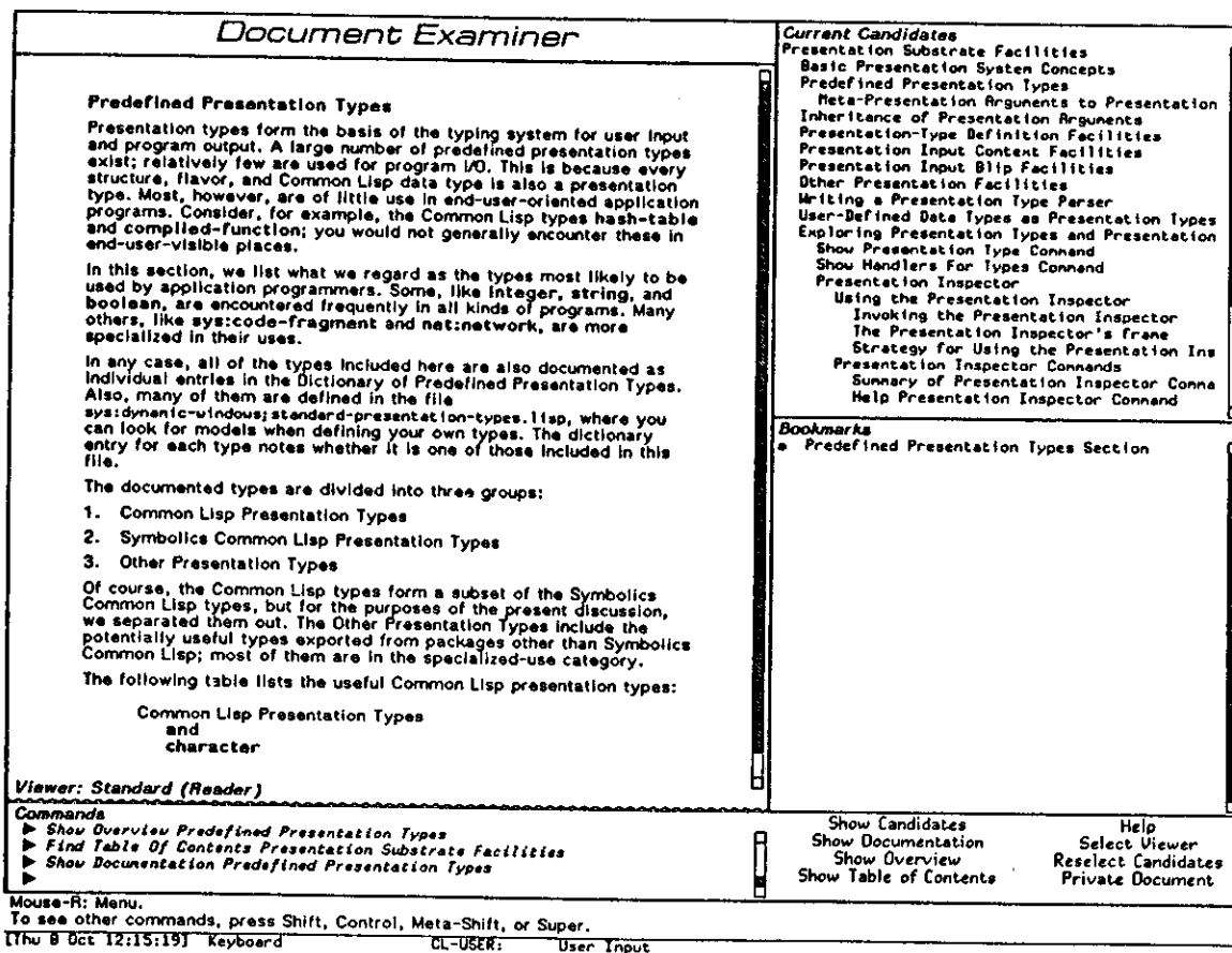
Figure 2. Document Examiner
