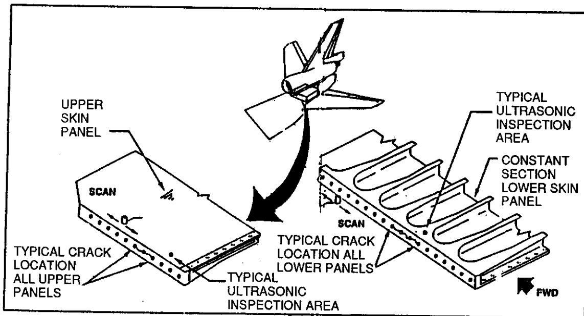
Figure 9. Typical crack environment for ultrasonic inspection.
