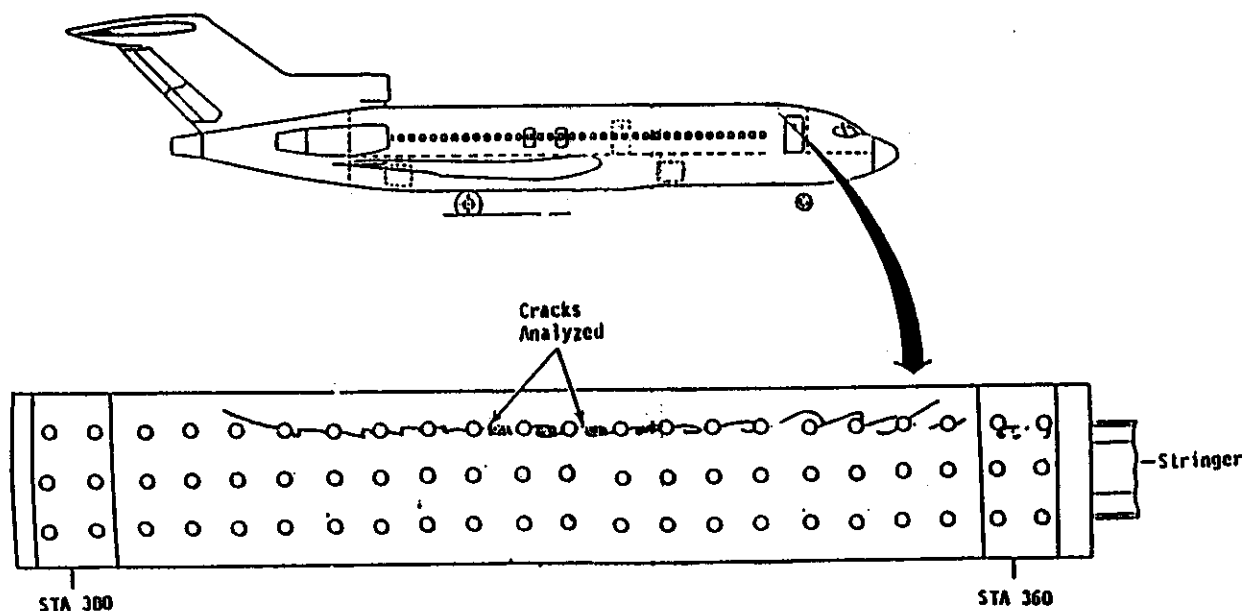
Figure 4. Example of multiple crack elongation.
