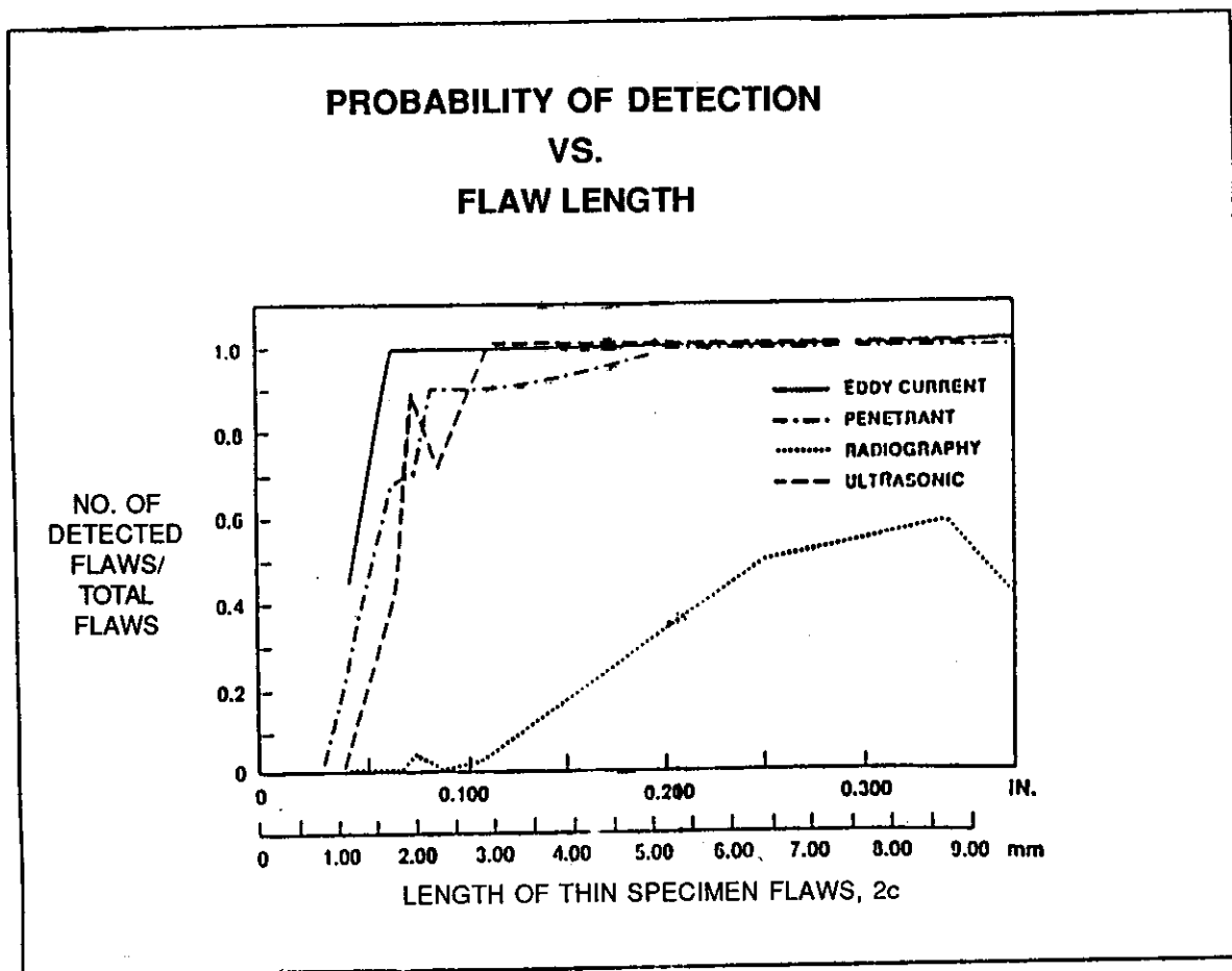
Figure 5. Detection probability curves for four NDI procedures.
