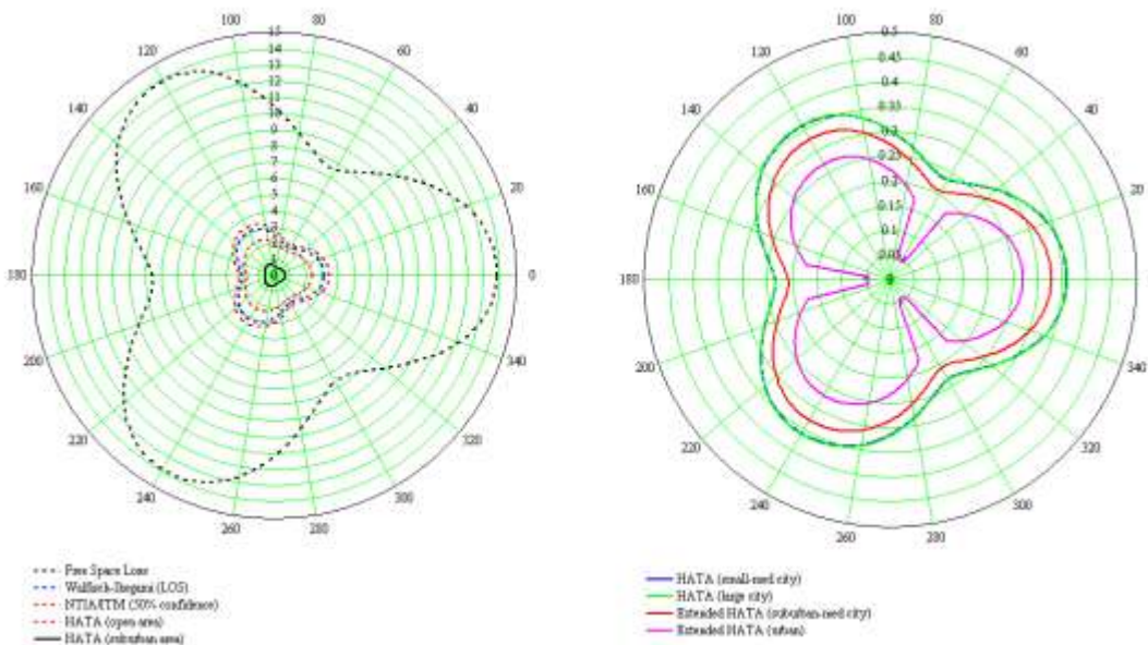
Figure 6-13. Separation Distance Contours for Receiver #16 and Interference Threshold = -68 dBm (1 dB C/N 0 degradation)
