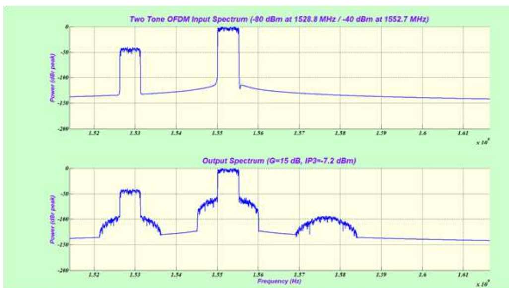
Figure 6-38. .Maxim MAX2741 Input (top) and Output (bottom) Power Spectra based Upon Simulations [2]
