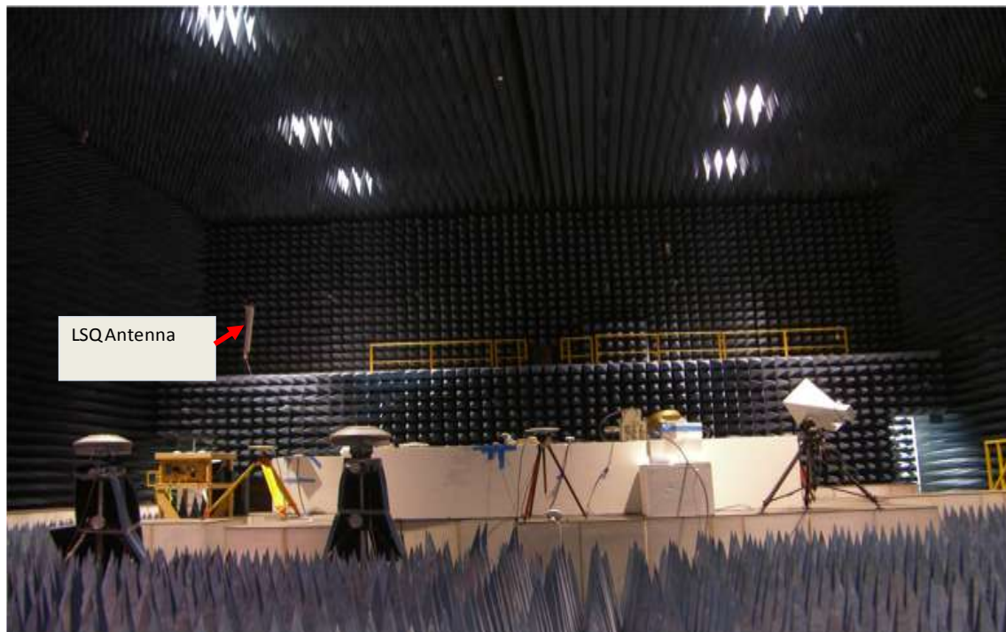
Figure 5-24. Chamber View Looking toward LSQ Antenna
