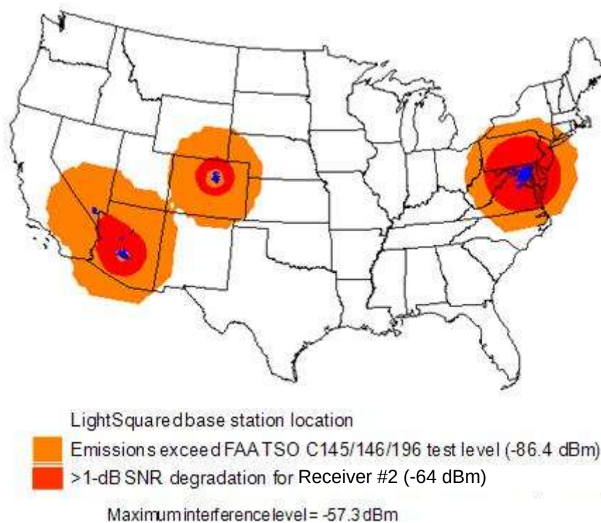
Figure 6-25. Initial LightSquared Deployment Aircraft at 20,000'
