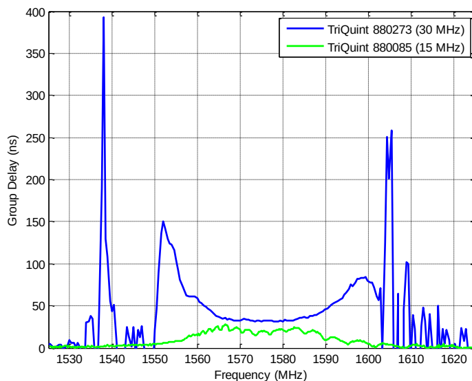
Figure 8-10. Group Delay of Two Representative BAW Filters
