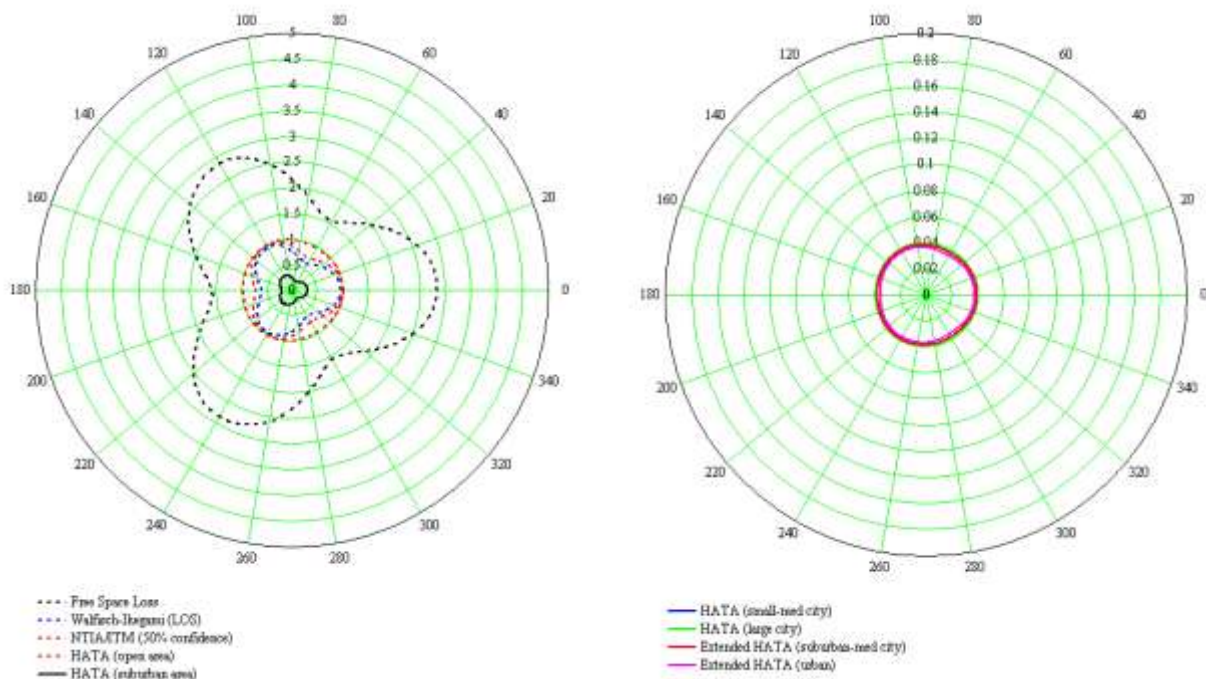
Figure 6-12. Separation Distance Contours for Receiver #15 and Interference Threshold = -54 dBm (1 dB C/N 0 degradation)
