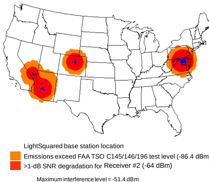
Figure 6-24. Initial LightSquared Deployment Aircraft at 10,000'
