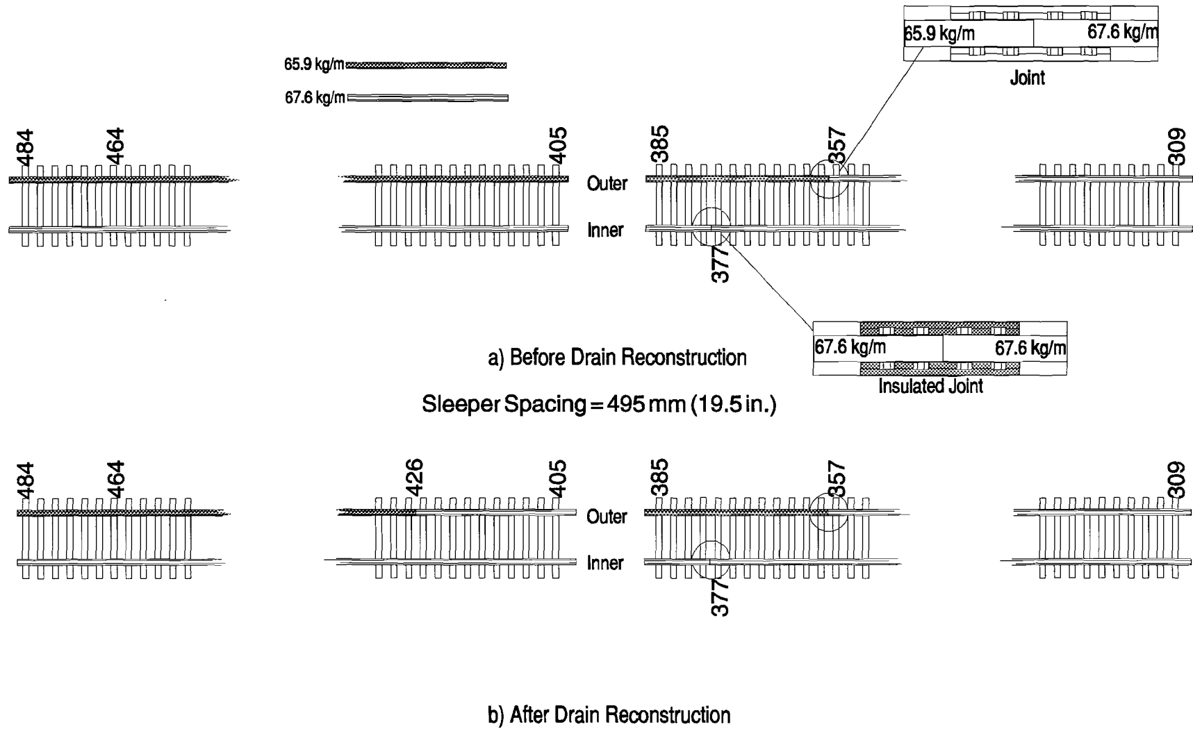
Figure 5: Tie Numbering and Joint Positions
