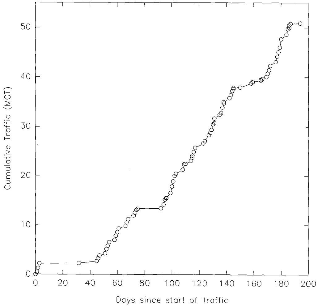
Figure 114: Cumulative Traffic
