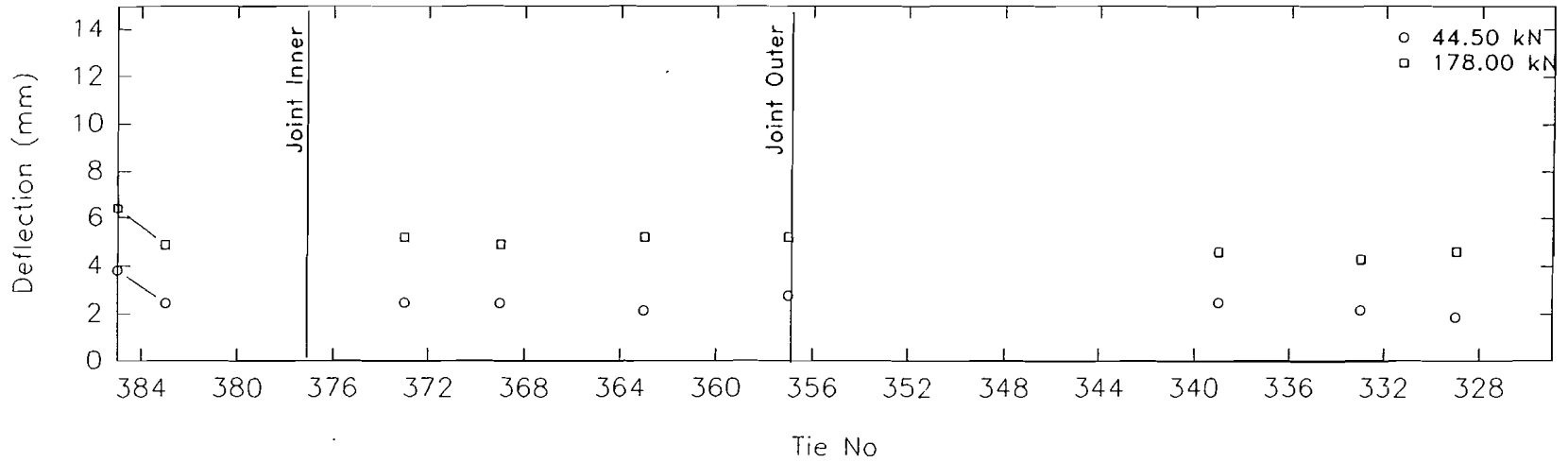
Figure 59: Running Deflection 17 June 1991
