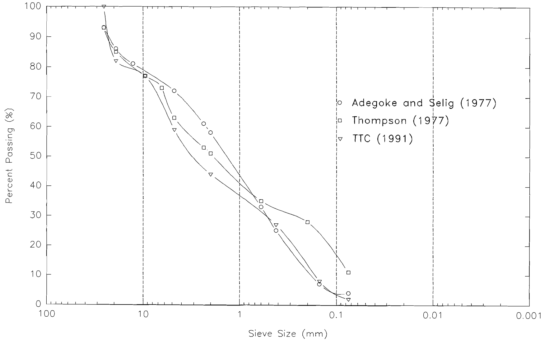
Figure 8: Subballast Gradations
