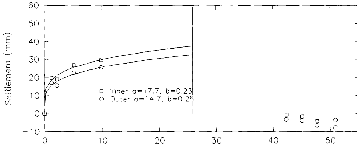
Figure 82: Settlements of Subsections
