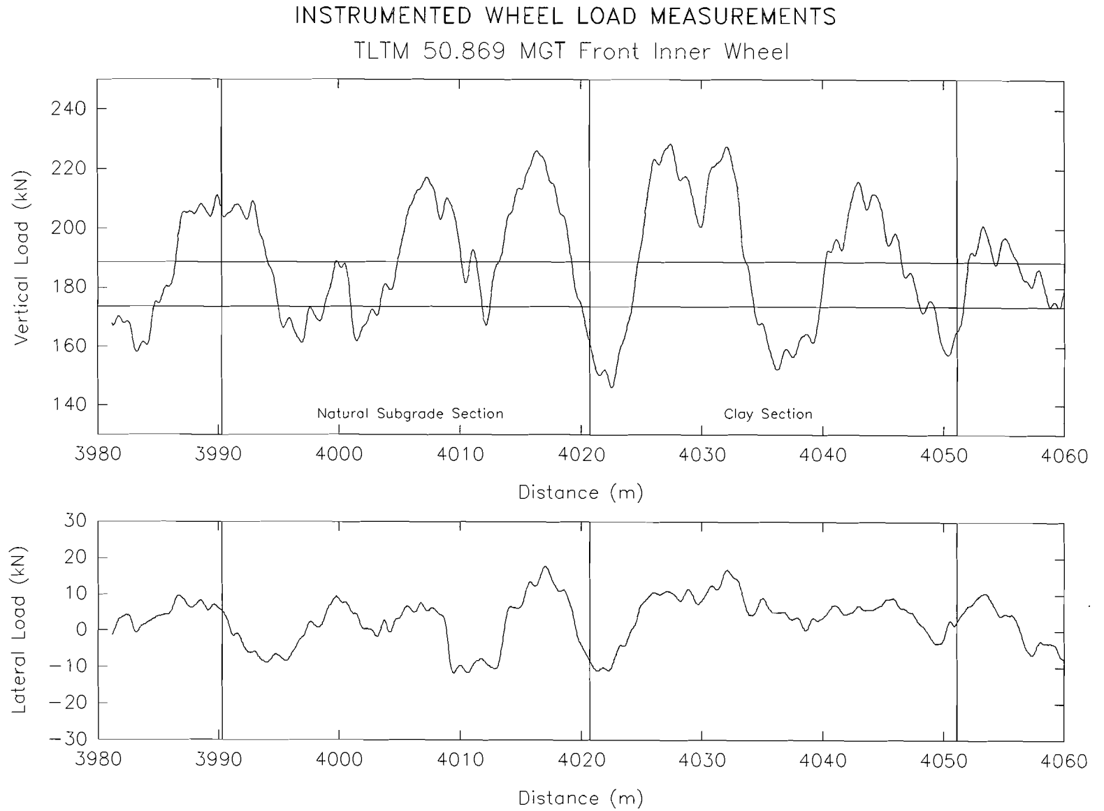
Figure 110: Wheel Load Measurements Front Inner Wheel
