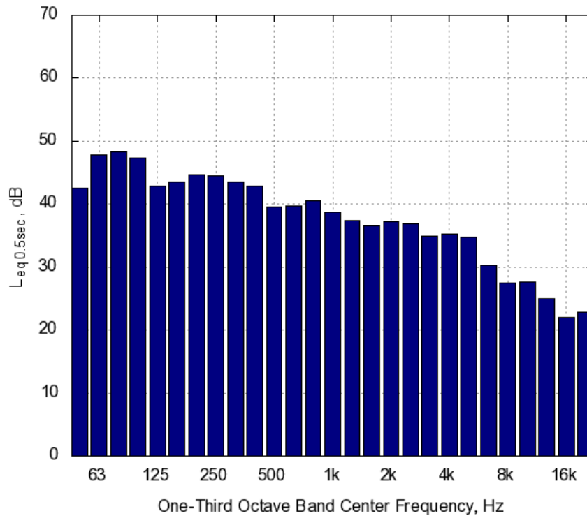
Figure A-72. Honda Civic Hybrid One-Third Octave Band Levels for 6 mph Constant Speed Passby at 12 ft Microphone
