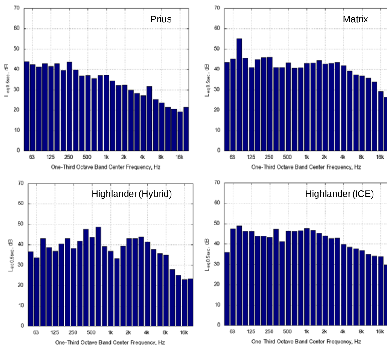
Figure 12. Sample One-Third Octave Band Spectra for 6 mph Constant Speed Passby at 12-ft Microphone Location
