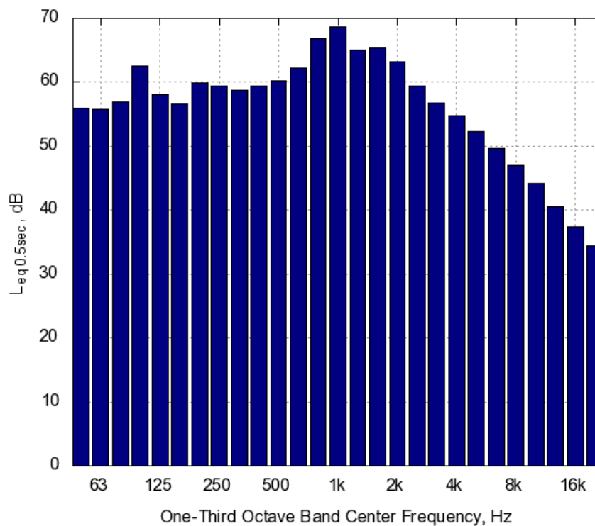
Figure A-61. Prius One-Third Octave Band Levels for 40 mph Constant Speed Passby at 12 ft Microphone
