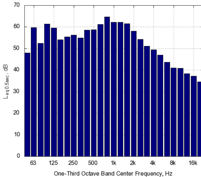
Figure A-91. Toyota Highlander Hybrid One-Third Octave Band Levels for 30 mph Constant Speed Passby at 12 ft Microphone
