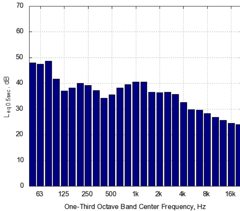
Figure A-96. Toyota Highlander ICE One-Third Octave Band Levels for Idle at 12 ft Microphone
