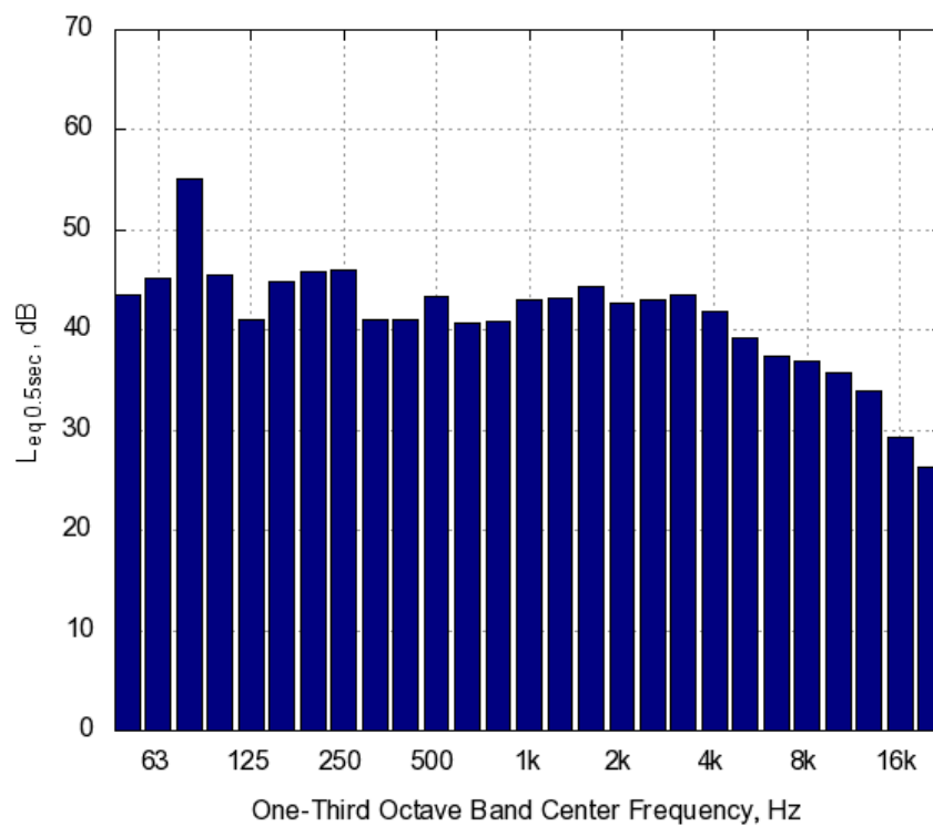
Figure A-62. Matrix One-Third Octave Band Levels for Idle at 12 ft Microphone
