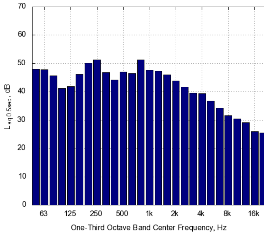
Figure A-78. Honda Civic Hybrid One-Third Octave Band Levels for Deceleration Passby at 12 ft Microphone
