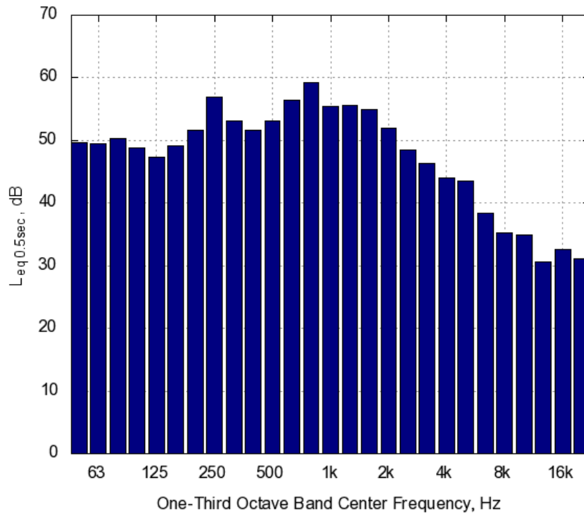
Figure A-90. Toyota Highlander Hybrid One-Third Octave Band Levels for 20 mph Constant Speed Passby at 12 ft Microphone
