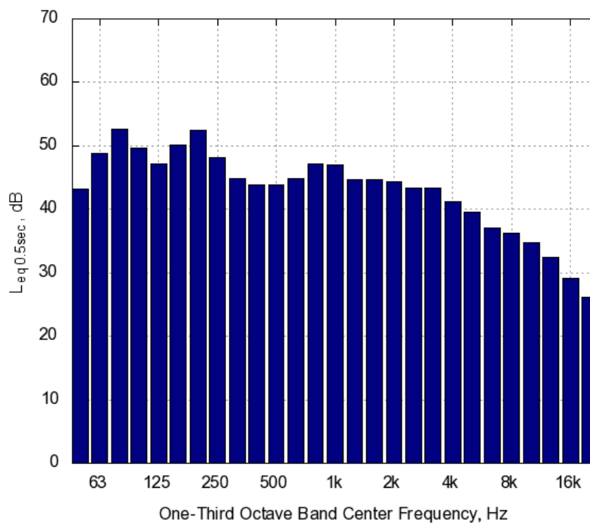
Figure A-64. Matrix One-Third Octave Band Levels for 10 mph Constant Speed Passby at 12 ft Microphone
