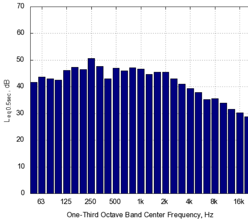
Figure A-81. Honda Civic ICE One-Third Octave Band Levels for 10 mph Constant Speed Passby at 12 ft Microphone
