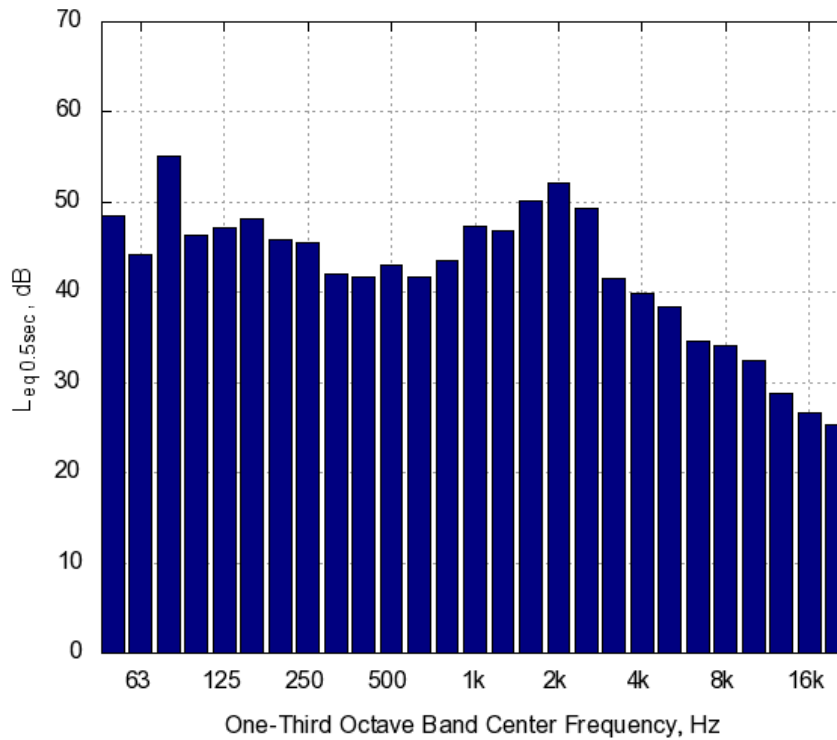
Figure A-85. Honda Civic ICE One-Third Octave Band Levels for Reverse 5 mph Constant Speed Passby at 12 ft Microphone
