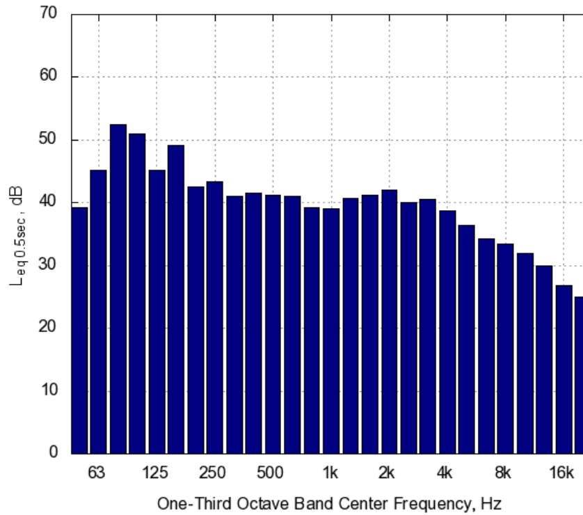
Figure A-68. Matrix One-Third Octave Band Levels for Reverse 5 mph Constant Speed Passby at 12 ft Microphone
