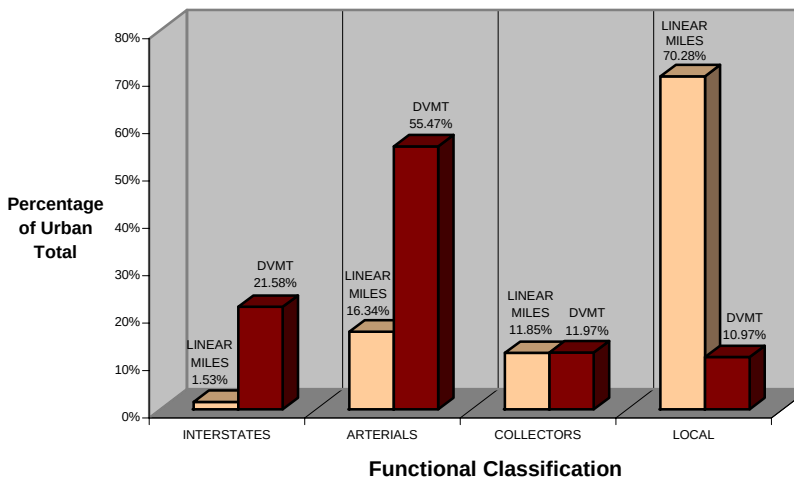
MILEAGE AND TRAVEL BY FUNCTIONAL CLASSIFICATION AS A PERCENTAGE OF TOTAL URBAN SYSTEM
