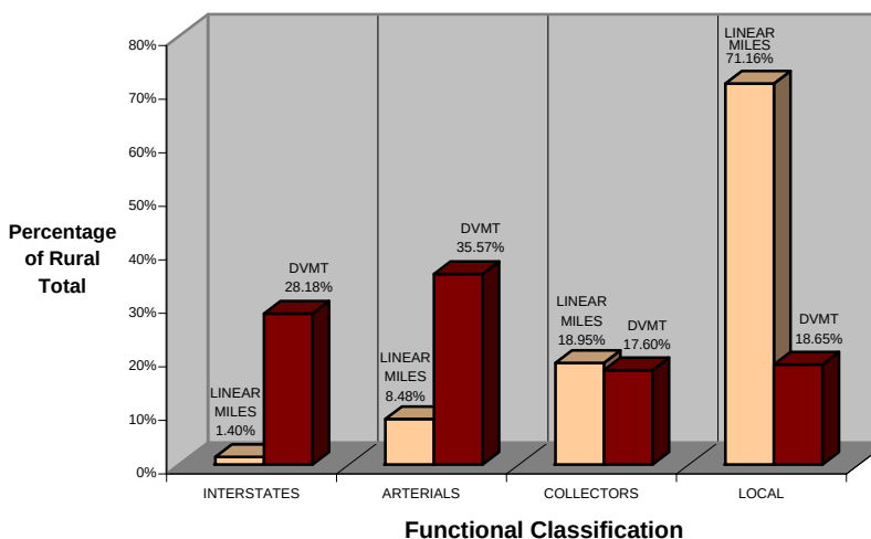
MILEAGE AND TRAVEL BY FUNCTIONAL CLASSIFICATION AS A PERCENTAGE OF TOTAL RURAL SYSTEM
