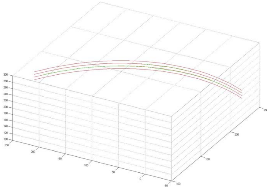
Figure 2-7 The calculated ellipses and surface deviation lines are presented as a 3-D model in Matlab.
