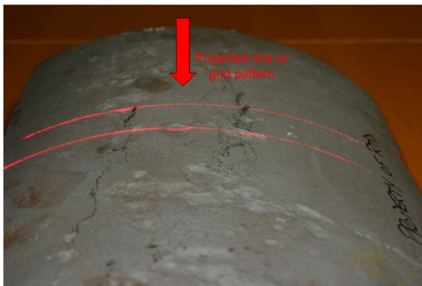
Figure 2-1 Two lines projected onto a corroded pipe section and viewed at a different angle. The distortion of the lines as they pass over corroded regions is clear.
