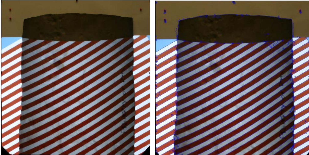
Figure 2-13 Illumination by pattern of thick lines (left), with the extracted lines shown in blue (right).
