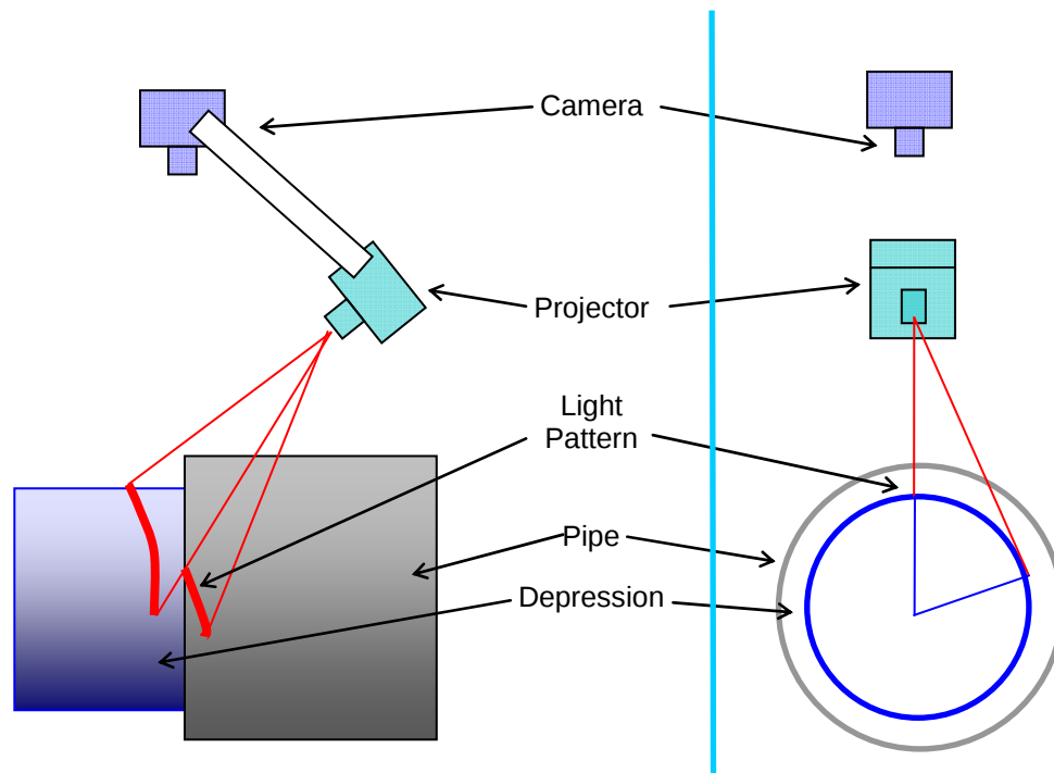
Figure 2-15 Schematic drawing of the Phase II prototype system.
