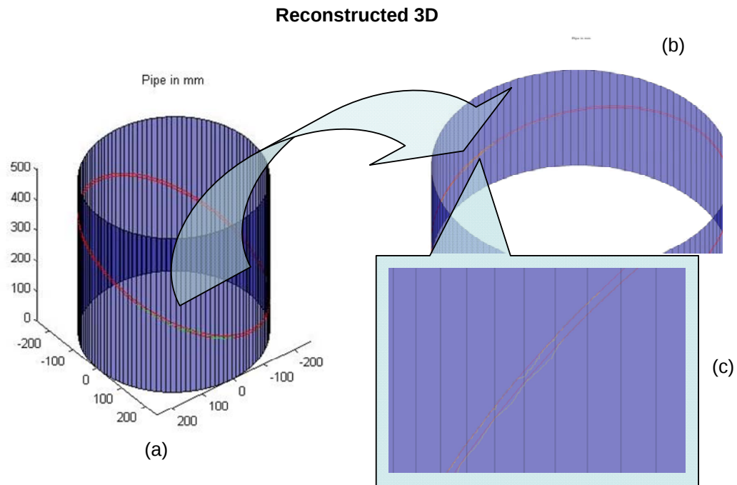
Figure 2-6 Calculated position of the ellipses (red line) at the idealized pipe (blue cylinder): (a) common view, (b) enlarged part on cylinder, and (c) further enlarged part of the surface.
