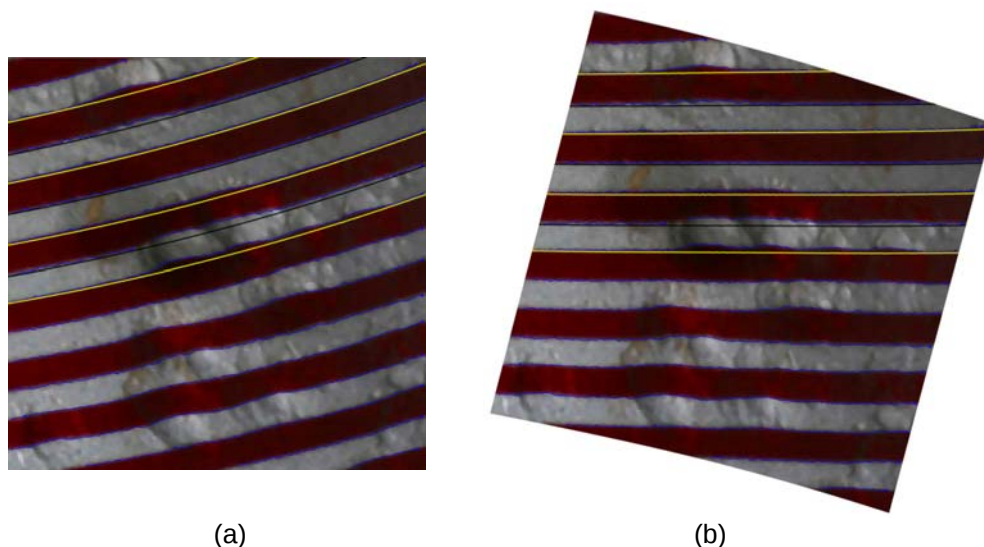
Figure 2-4 Fitting ellipses to the line allows the general shape of the pipe and depth information to be extracted: (a) We determined ellipses that fit to the surface (yellow lines); then we could unwrap the surface (b) in such a way that the yellow lines become straight. The depression depth (blue line) can then be clearly seen as a deviation from the surface (yellow line).
