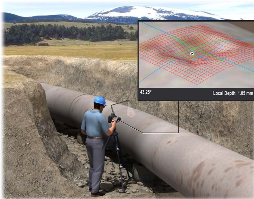
Figure 1-1 A pipeline inspector will be able to capture an image of the illuminated damaged region with a conventional camera. Signal processing will yield the full 2-D depth profile with mm accuracy.
