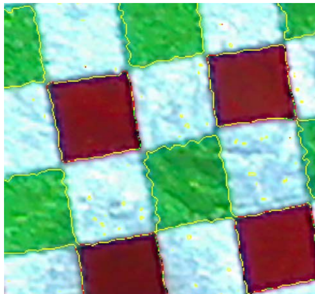
Figure 2-12 Result of the checkerboard pattern processing. The yellow lines are the extracted shape.
