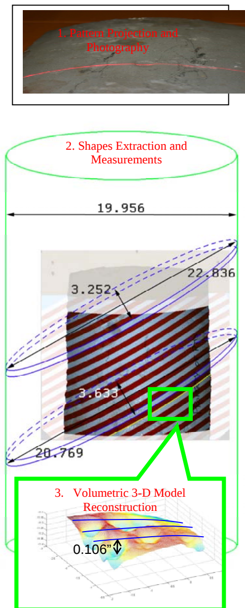
Figure 2-2 (1) Line projected across corrosion pit at its center. On the undistorted surface the line has the shape of an ellipse; (2) example of the extraction of the pipe shape and dimensions from a projected line pattern; (3) extracted 3-D model of the surface provides quantitative damage assessment.
