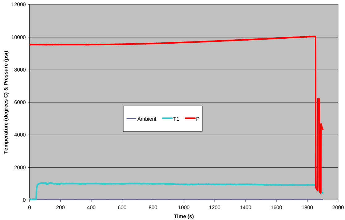
Figure 27 – Surface temperature and internal pressure measurements on Quantum during 30 minute localized fire test.
