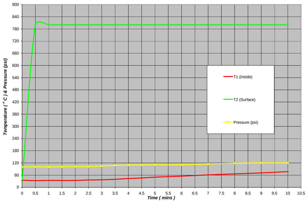
Figure 8 – Change in tank pressure and internal temperature during exposure to 800°C surface temperature
