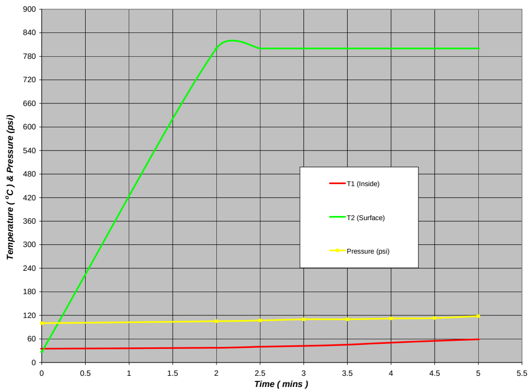
Figure 18 – Pressure and temperature rise inside tank during 5 minute localized fire test.
