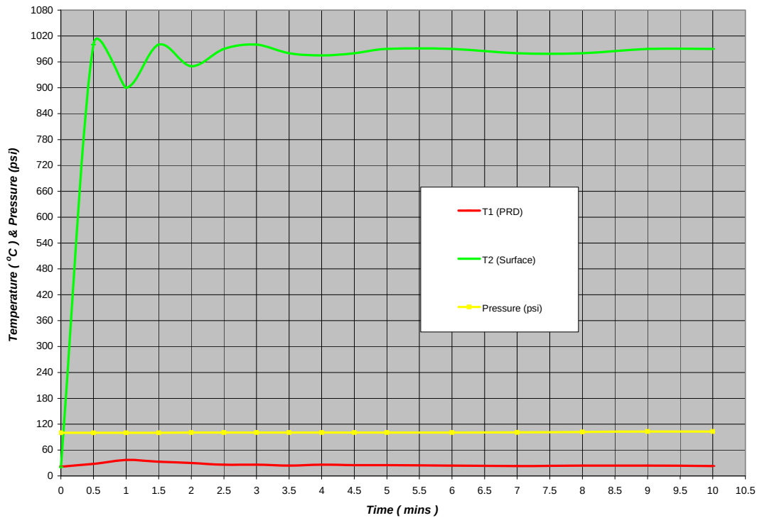
Figure 24 – Pressure and temperature change within the Quantum tank during localized fire at temperatures in excess of 950°C.
