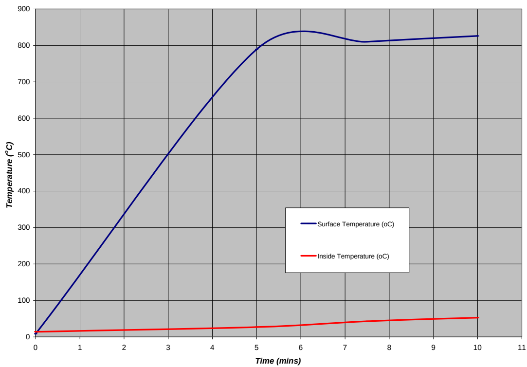
Figure 15 – Comparison of internal tank and external blanket temperatures on Flexible Min-K during localized fire test.
