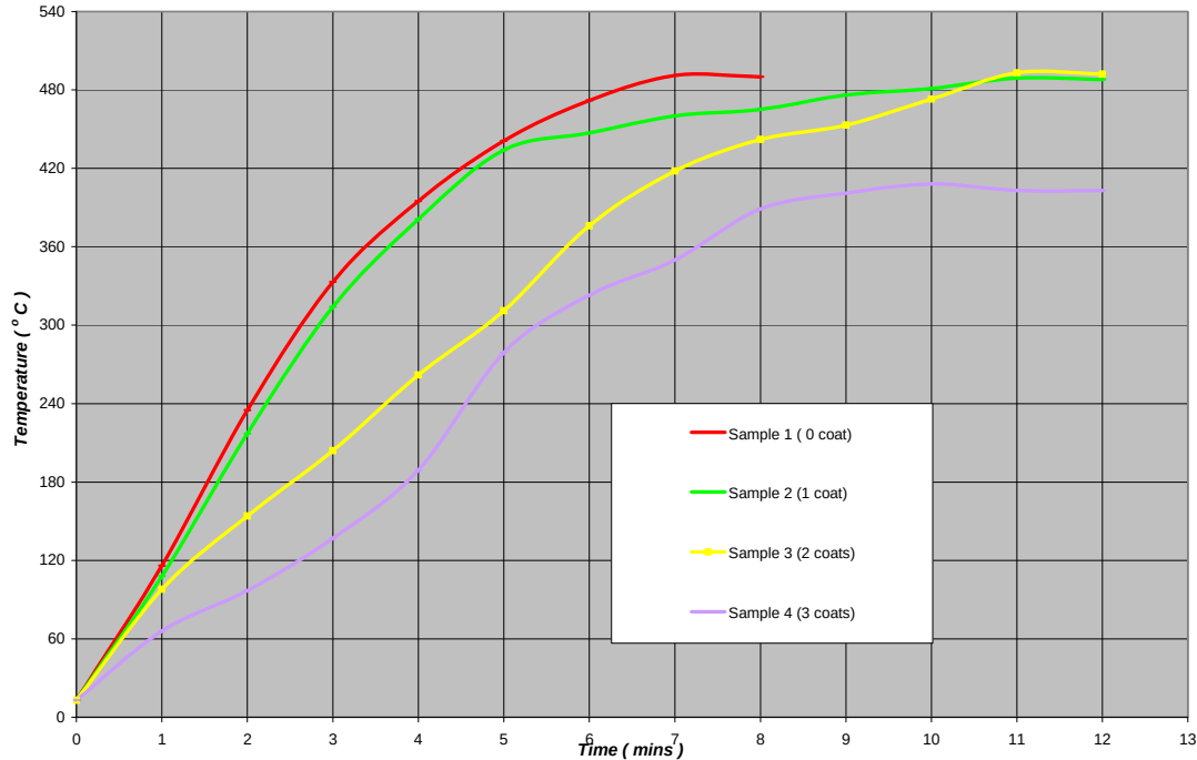
Figure 3 – Illustrates effect of paint coating on temperature rise on internal surface of steel pipe section when heated on external surface.
