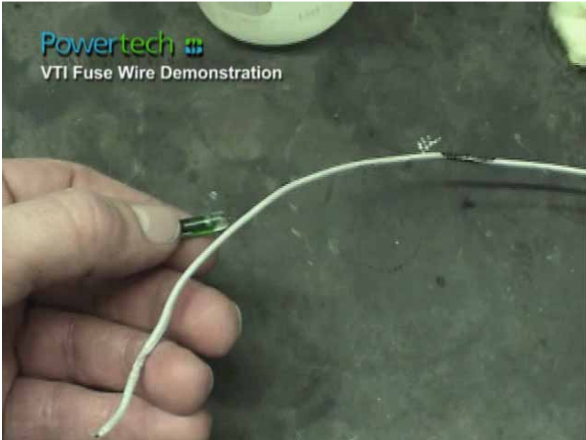
Figure 19 – Fuse wire and glass bulb used in VTI TPRD
