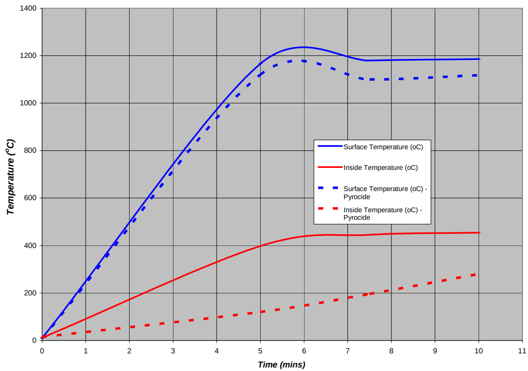
Figure 5 – Comparison of temperature performance of PyroCide II coated tank vs uncoated tank
