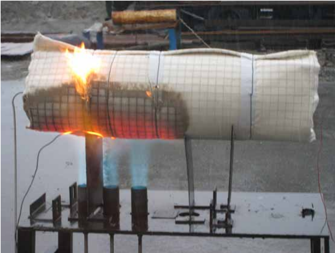
Figure 14 – Localized fire test of tank wrapped in Flexible Min-K blanket.
