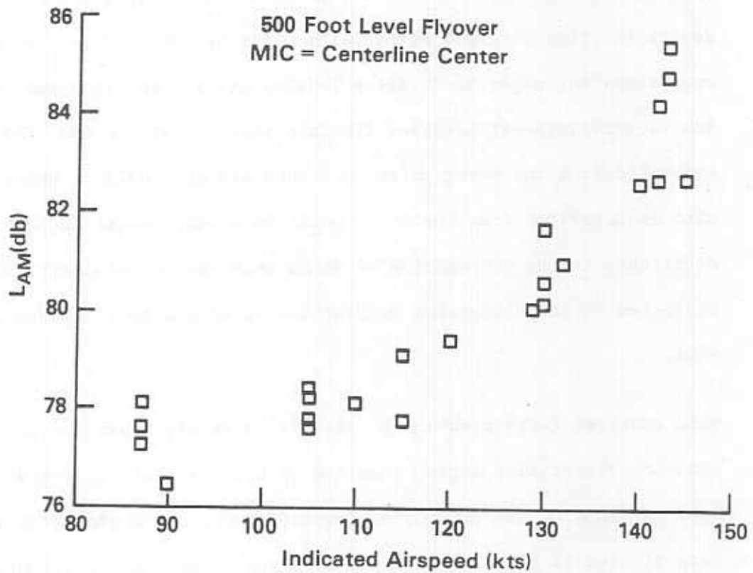
Figure 9.5 Helicopter Noise Measurement Data (June 24, 1980 Ref. Table A.3-2.1)
