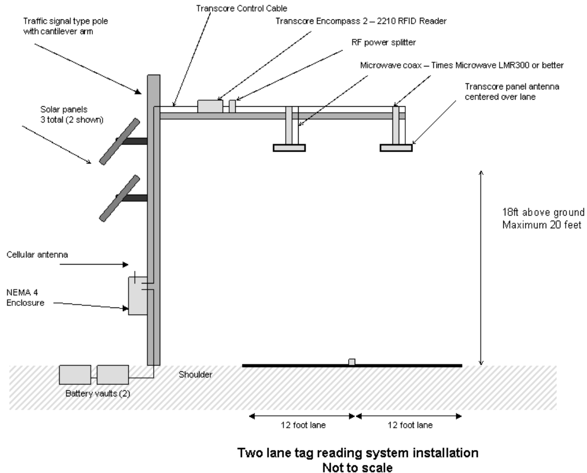
Figure 8. Sample RFID reader station.
