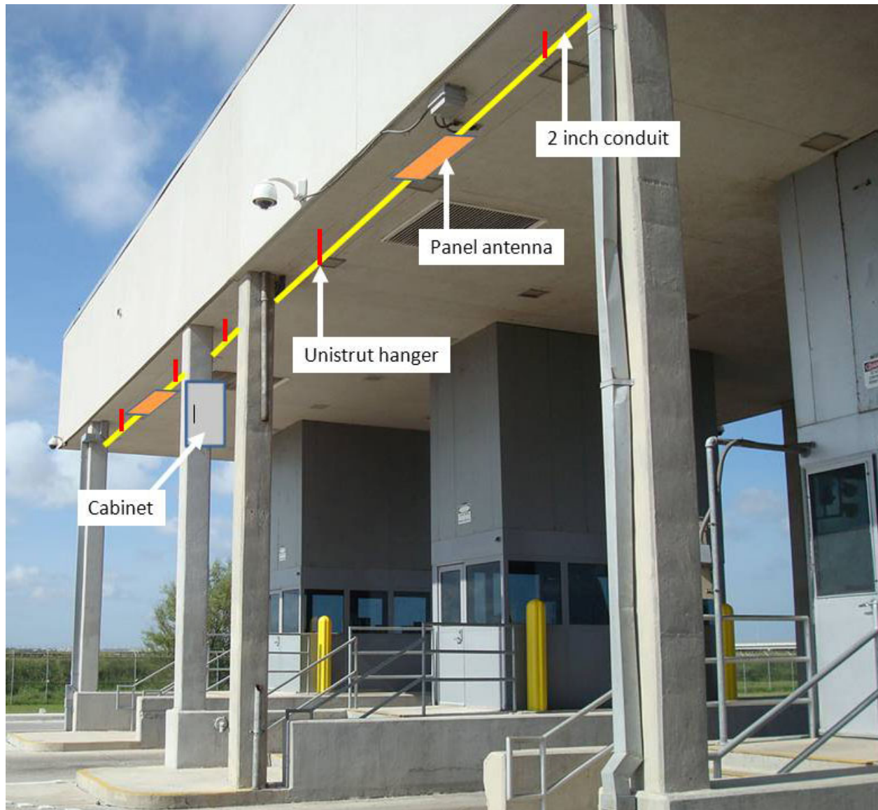
Exhibit 2. Installation Visualization
