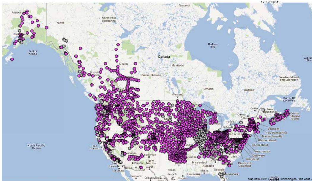
Figure 3.1 Clarus Observations
