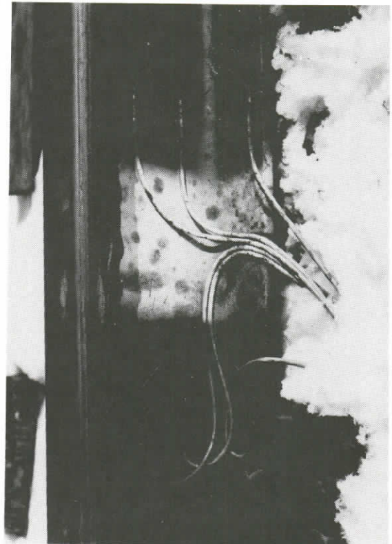
43. DETAIL OF STRAIN GAGE PATTERN AS INSTALLED
