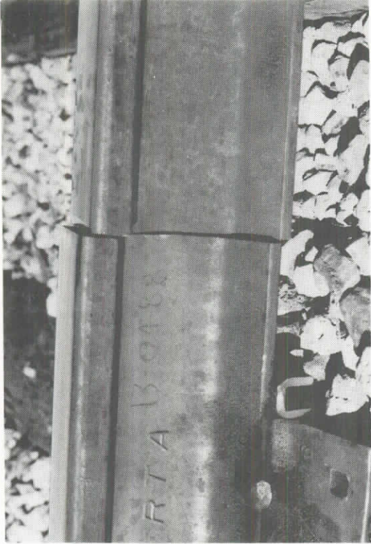
204. DETAIL OF RAIL BREAK
