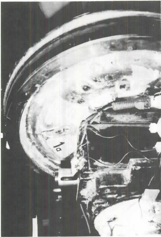
152. ORIENTATION OF STRAIN GAGES - RIGHT VIEW
