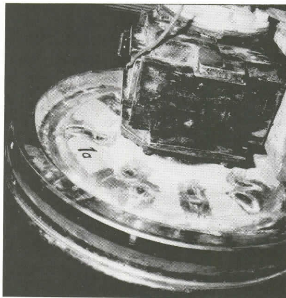
151. ORIENTATION OF STRAIN GAGES - LEFT VIEW
