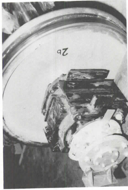
72. INSTRUMENTED WHEELSET 11 WITH JOURNAL BOX REINSTALLED
