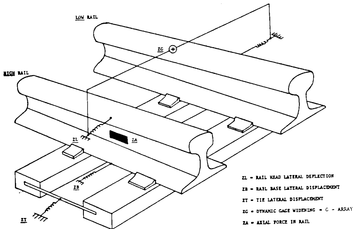
FIGURE 3-24. SCHEMATIC OF DISPLACEMENT TRANSDUCER ARRAYS
