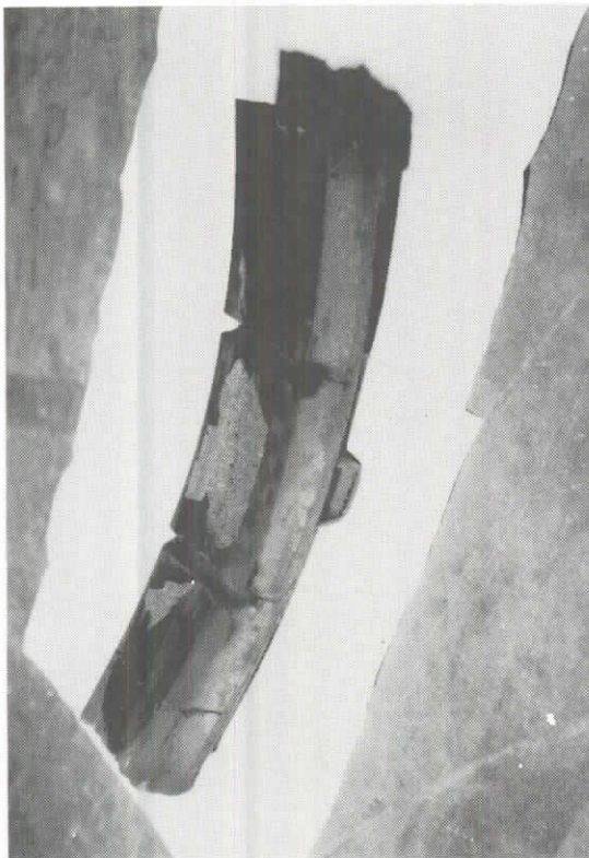
120. HEAT DAMAGED BRAKE SHOE OF AXLE 10 RIGHT WHEEL
