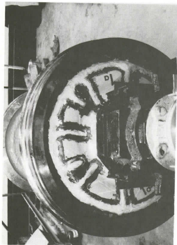
165. PROTECTIVE COATING APPLIED TO GAGES AND WIRING
