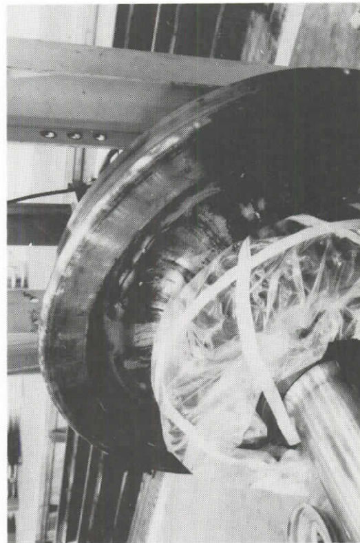
162. CALIBRATING REPAIRED WHEELSET ALSO SHOWS AXLE GEARING
