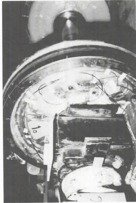
155. WIRING FOR STRAIN GAGES AXLE 10 RIGHT WHEEL
