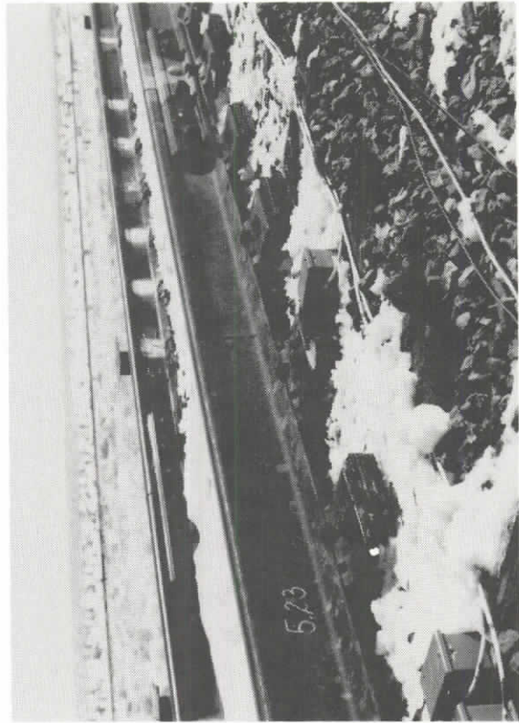
16. SECTION 5.23 - SHOWING 2" SHIMS USED ON LOW RAIL TO REDUCE NOMINAL SUPERELEVATION TO 1"
