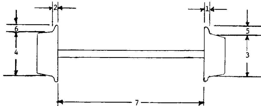
WHEELSET DIMENSIONS (1) (INCHES)
