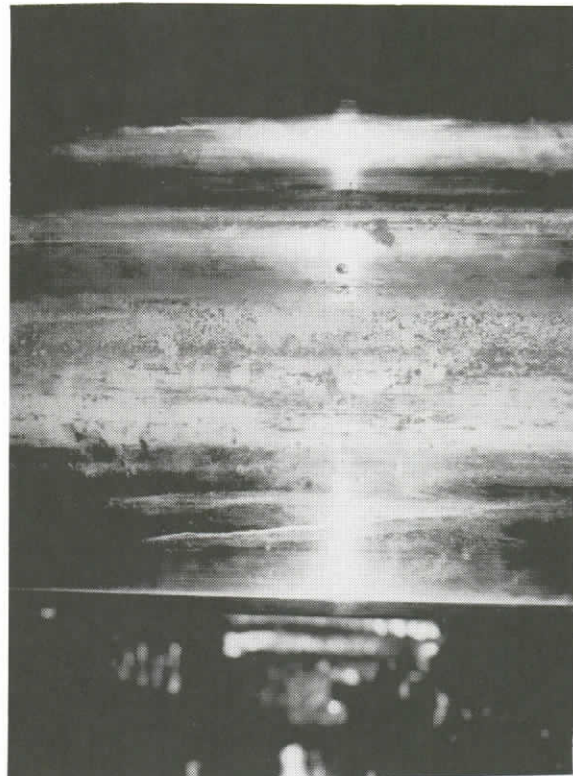
126. SCARRING OF WHEEL TREAD SURFACE
