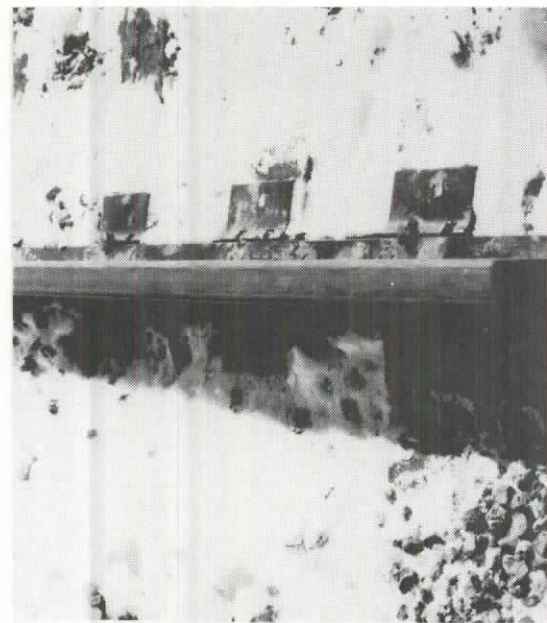
6. SPIKING PATTERN FOR "SOFT" TRACK SECTION 3
