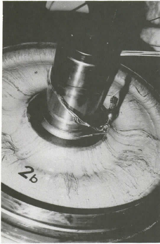
180. DAMAGED WIRING DUE TO OVERHEATED THRUST BEARING
