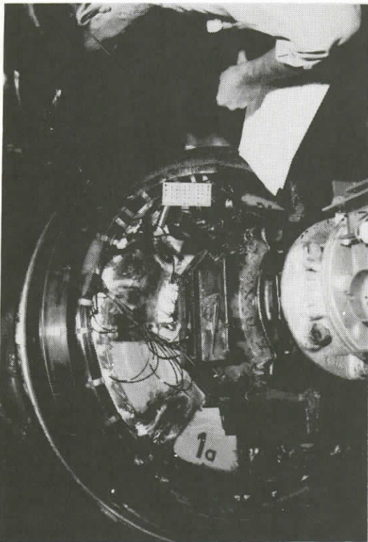
156. PREPARING NEW LEADS FOR JUNCTION BOARD
