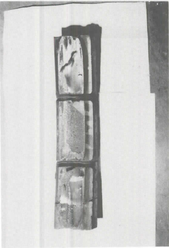
121. HEAT DAMAGED BRAKE SHOE OF AXLE 11 RIGHT WHEEL
