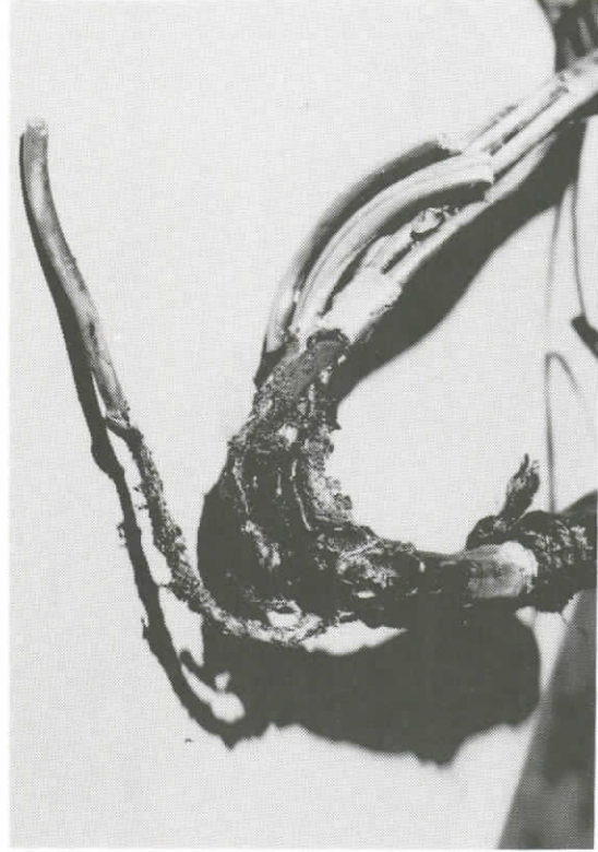
182. DETAIL OF DAMAGED WIRING AFTER REMOVAL
