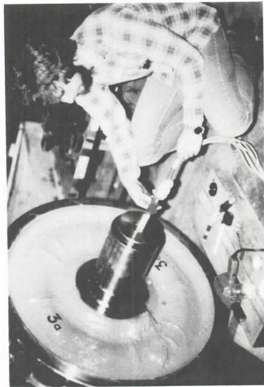
71. INSTRUMENTED WHEELSET 12 SLIP RING PREPARATION
