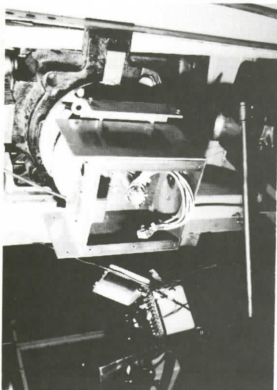
164. CALIBRATING REPAIRED WHEELSET SHOWING SLIP RING ASSEMBLY
