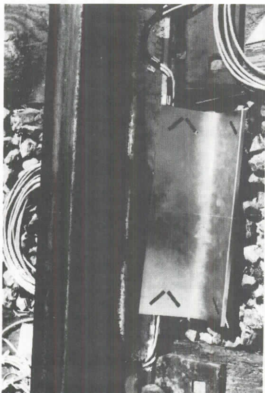
45. STRAIN GAGE TEMPLATE
