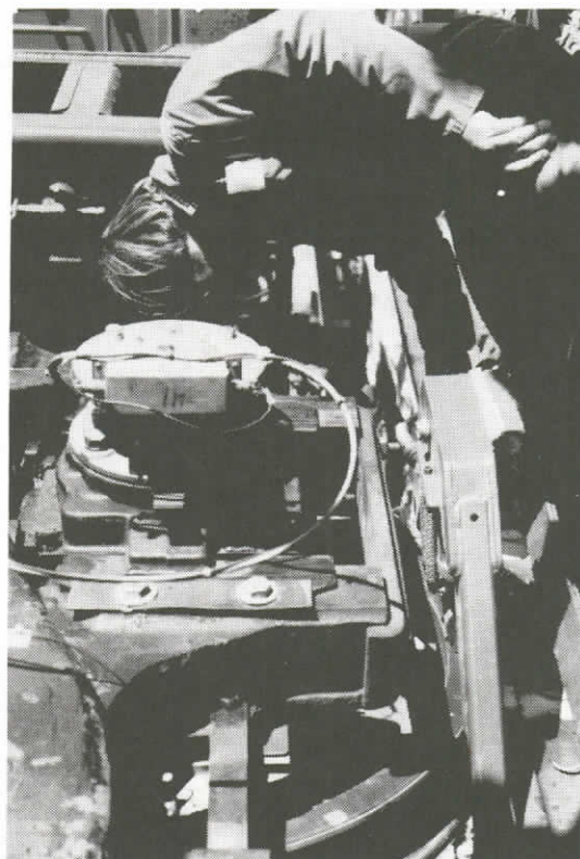
100. DETAIL OF WHEELSET/WAYSIDE JOINT CALIBRATION JACK
