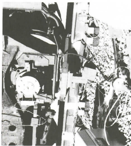
99. CALIBRATION JACK FORCES WHEELSET AGAINST OUTER RAIL TO OBTAIN SIMULTANEOUS WHEELSET AND WAYSIDE LATERAL FORCE MEASUREMENTS
