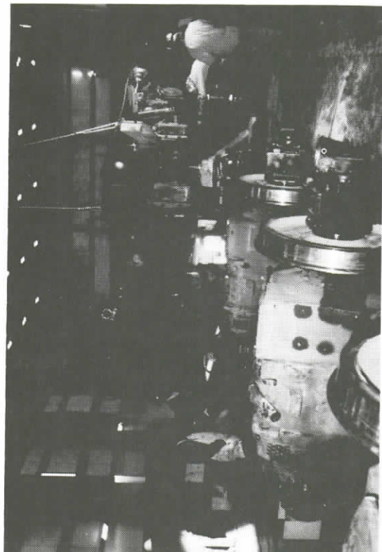
75. POSITIONING SDP-40F TRUCK FRAME PRIOR TO REASSEMBLY
