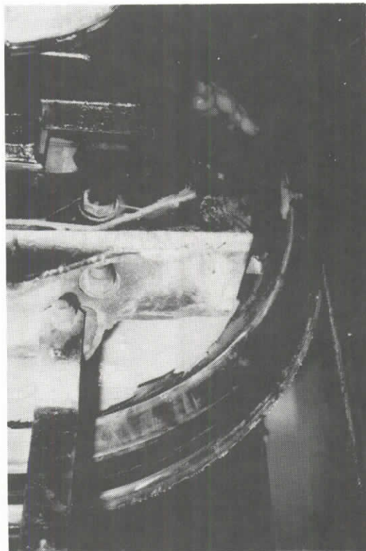
122. OVERHEATED WHEEL CAUSED BY ENGAGED HAND BRAKE
