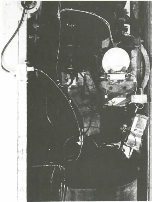
85. VIDEO CAMERA USED TO RECORD AXLE 10 WHEEL CLIMB - ALSO SHOWN: LOCATION OF ALD TRANSDUCER
