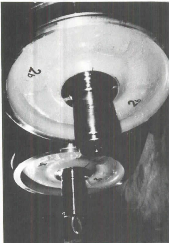
69. ASEA/SJ INSTRUMENTED WHEELSETS 11 AND 12 LEFT SIDE
