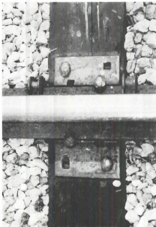
5. NORMAL SPIKING PATTERN FOR "STIFF" TRACK
