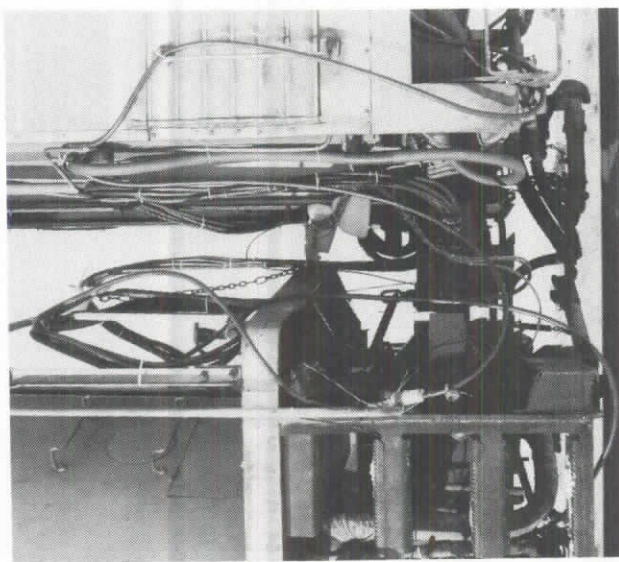
89. SDP-40F AND BAGGAGE CAR INSTRUMENTED COUPLERS AND CABLING OF INSTRUMENTATION
