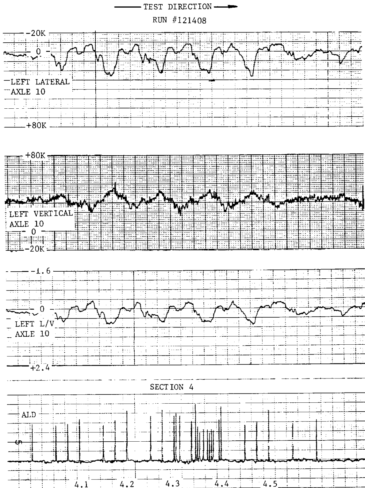
FIGURE 6-9. SDP-40F RESPONSE IN SECTION 4 AT 65 MPH - "A" CONSIST - LEFT LATERAL, LEFT VERTICAL, AND L/V - AXLE 10
