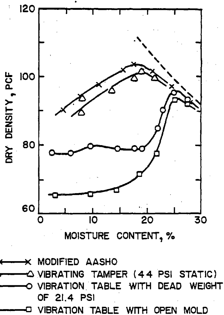
Figure 5.5. Density-Moisture Content Variation of Silt for Various Methods (Ref. 171)
