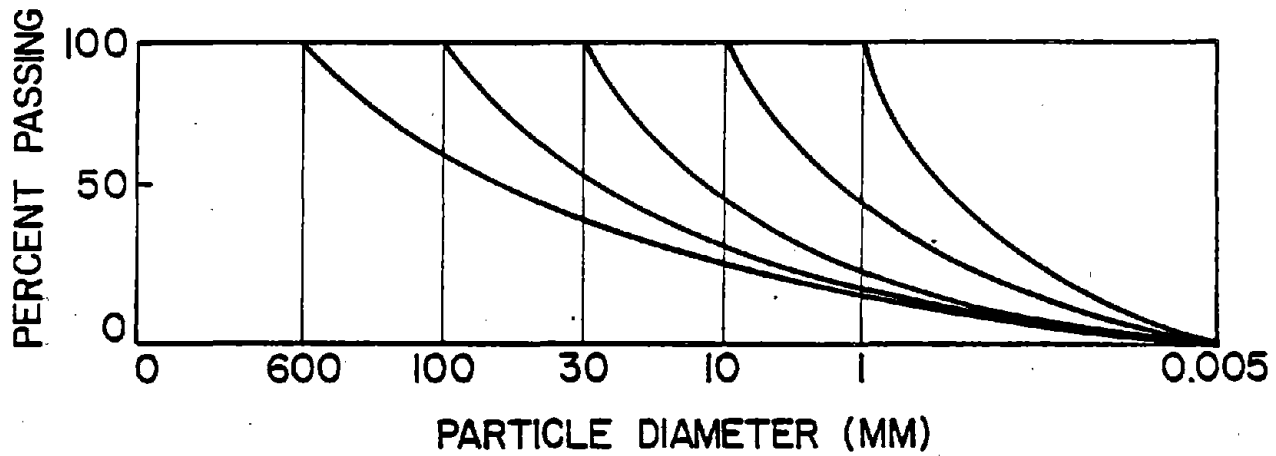
Figure 4.8. Gradation Curves by the Scalping Method (Ref. 83)
