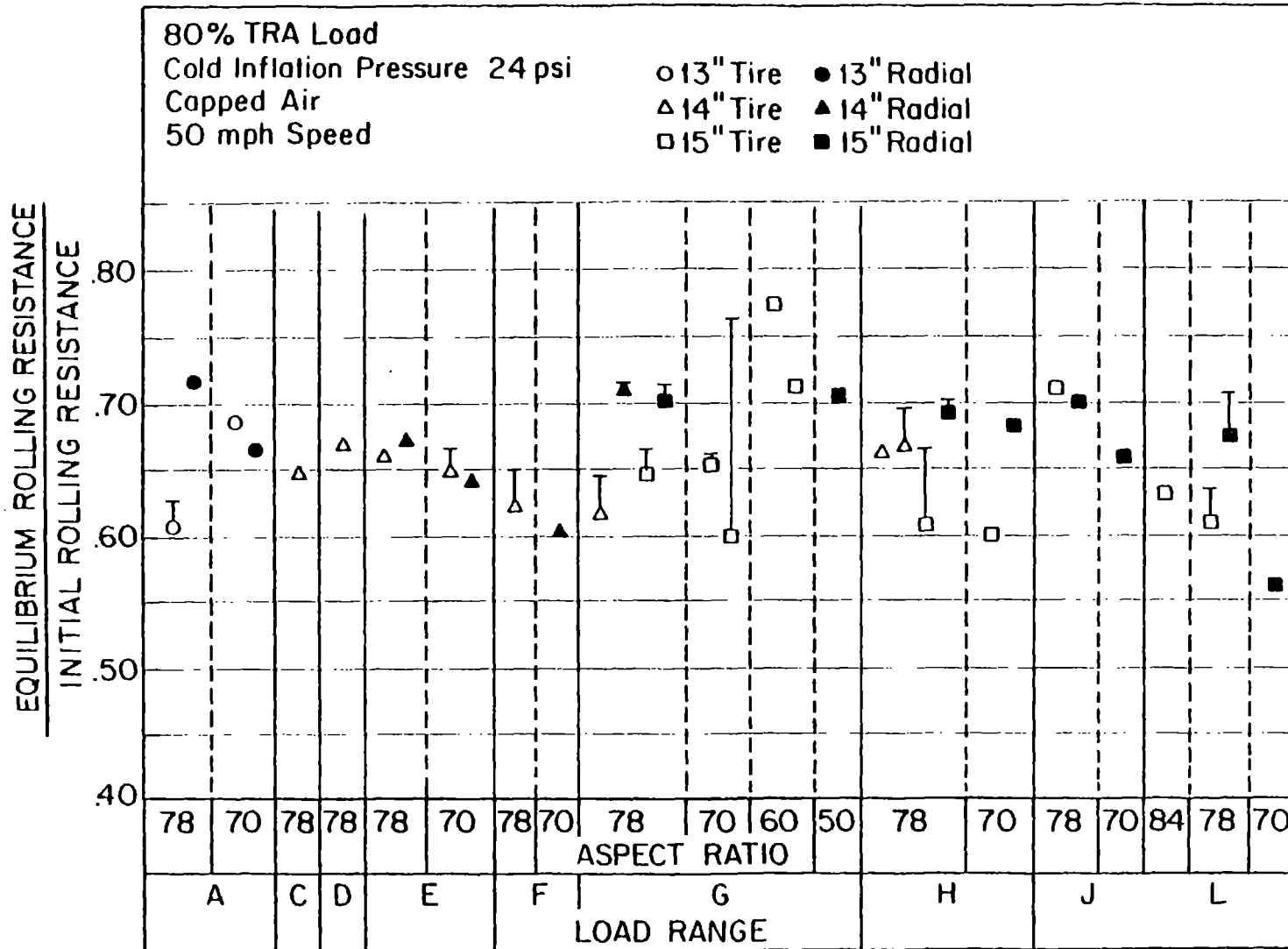
FIGURE 19. RATIO OF EQUILIBRIUM ROLLING RESISTANCE TO INITIAL ROLLING RESISTANCE FOR A SELECTION OF PASSENGER CAR TIRES
