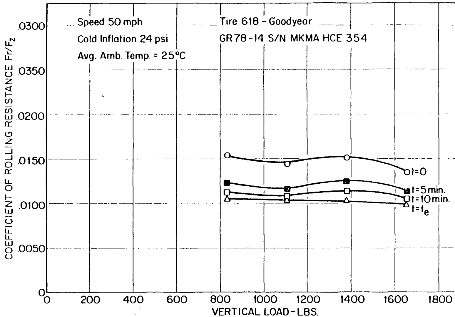
FIGURE 10. COEFFICIENT OF ROLLING RESISTANCE VS. VERTICAL LOAD FOR GR78-14 RADIAL TIRE
