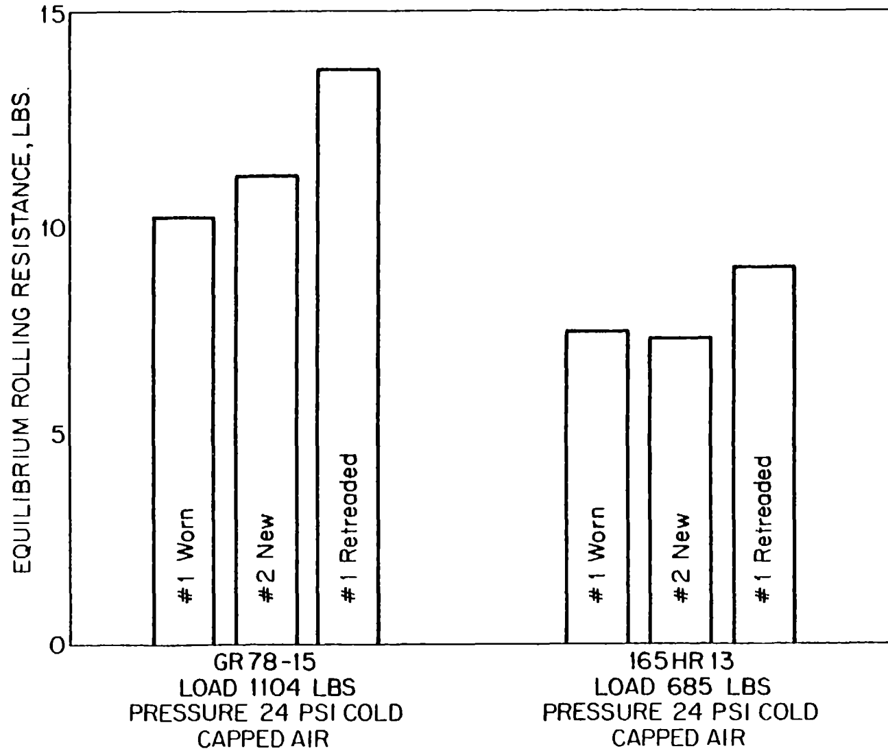
FIGURE 21. EQUILIBRIUM ROLLING RESISTANCE VALUES FOR NEW, WORN, AND RETREADED TIRES OF THE SAME TYPE
