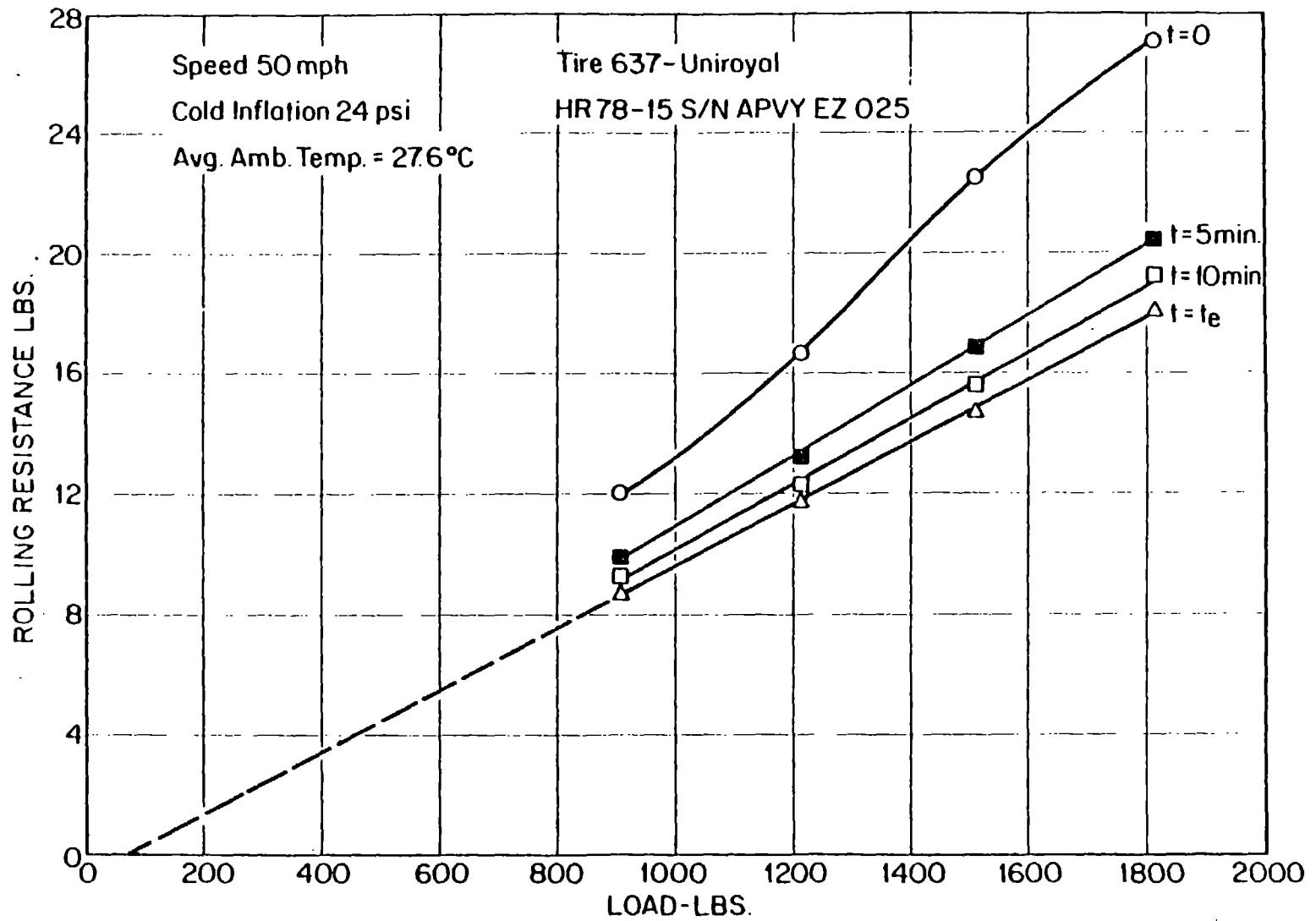
FIGURE 7. ROLLING RESISTANCE VS. VERTICAL LOAD FOR HR78-15 RADIAL TIRE
