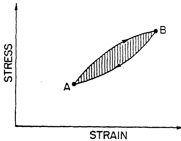
FIGURE 1. A TYPICAL STRESS STRAIN CURVE ILLUSTRATING LOSS
