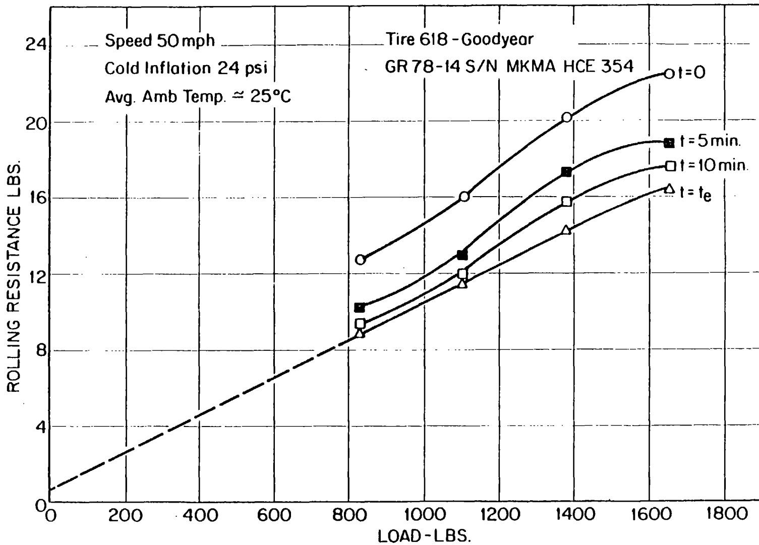
FIGURE 6. ROLLING RESISTANCE VS. VERTICAL LOAD FOR GR78-14 RADIAL TIRE
