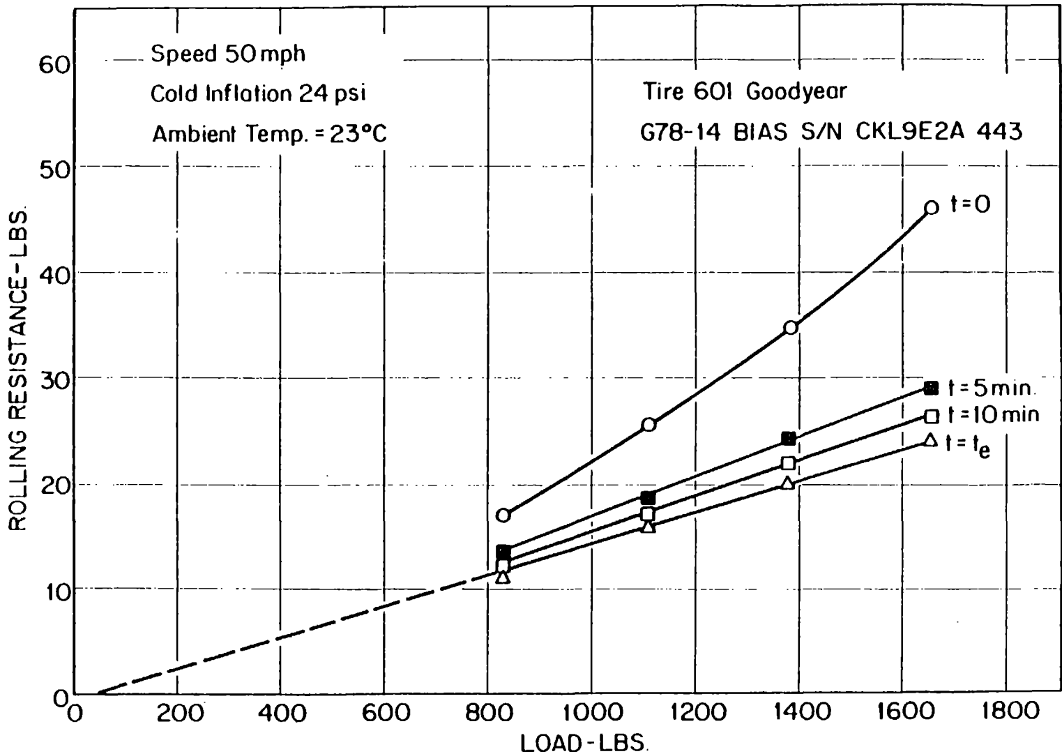
FIGURE 4. ROLLING RESISTANCE VS. VERTICAL LOAD FOR G78-14 BIAS TIRE
