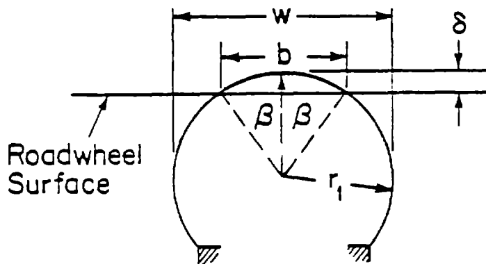
FIGURE A-6. TYPICAL TIRE CROSS-SECTIONAL GEOMETRY
