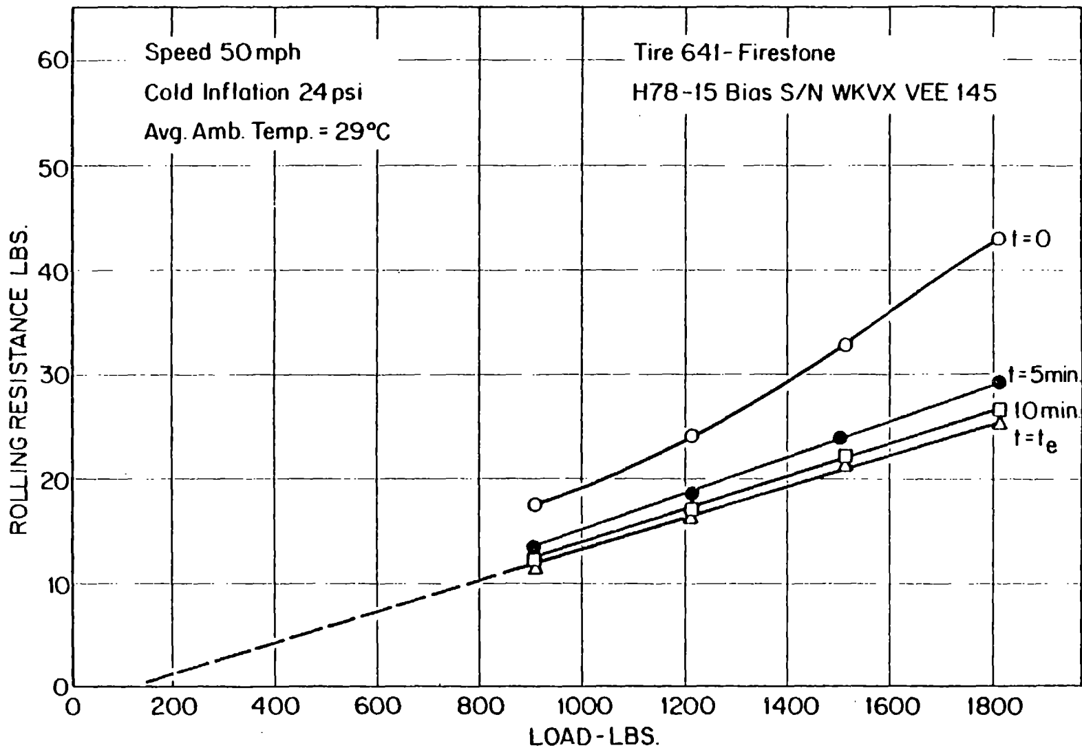
FIGURE 5. ROLLING RESISTANCE VS. VERTICAL LOAD FOR H78-15 BIAS TIRE
