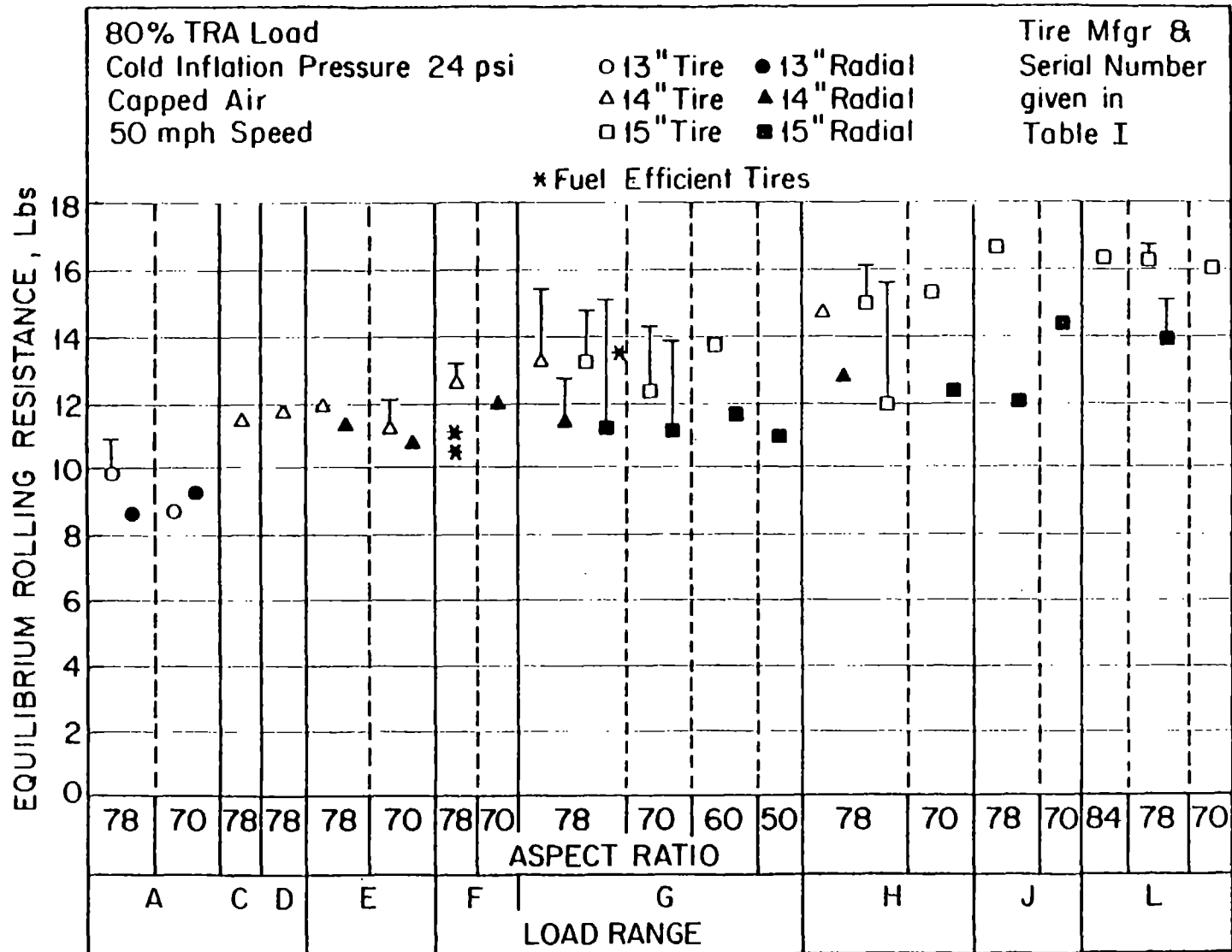
FIGURE 17. ROLLING RESISTANCE VS. TIRE LOAD RATING FOR A TYPICAL SELECTION OF PASSENGER CAR TIRES
