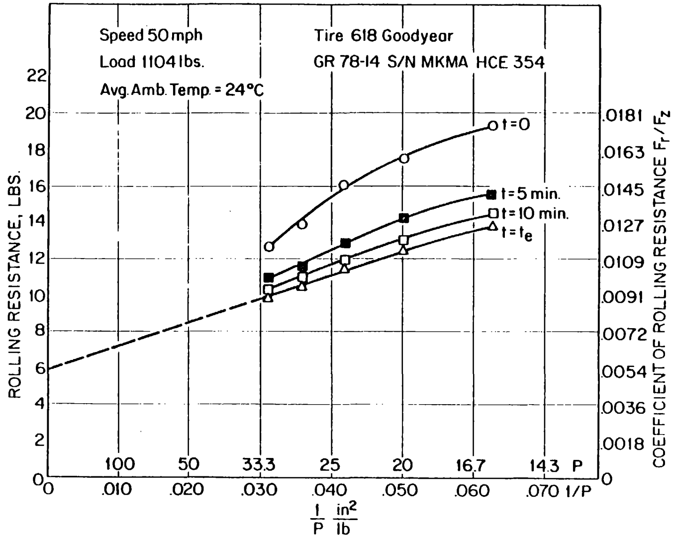
FIGURE 14. ROLLING RESISTANCE AND COEFFICIENT OF ROLLING RESISTANCE VS. RECIPROCAL OF INFLATION PRESSURE FOR GR78-14 RADIAL TIRE
