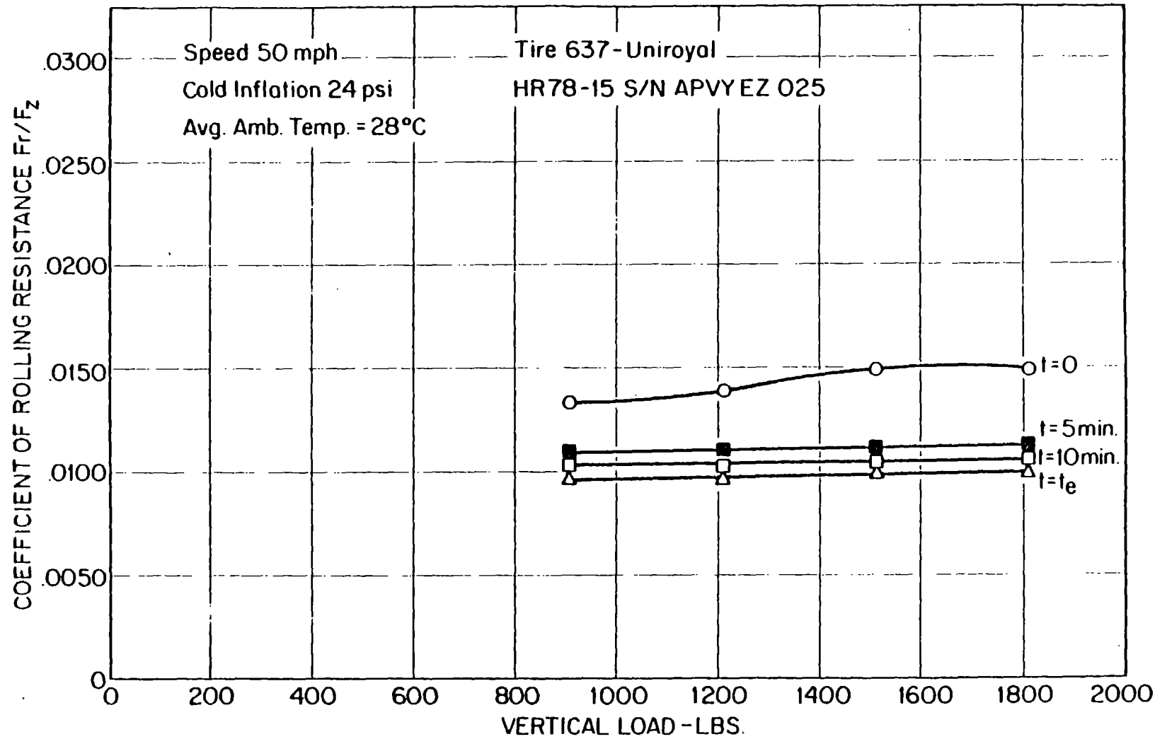
FIGURE 11. COEFFICIENT OF ROLLING RESISTANCE VS. VERTICAL LOAD FOR HR78-15 RADIAL TIRE
