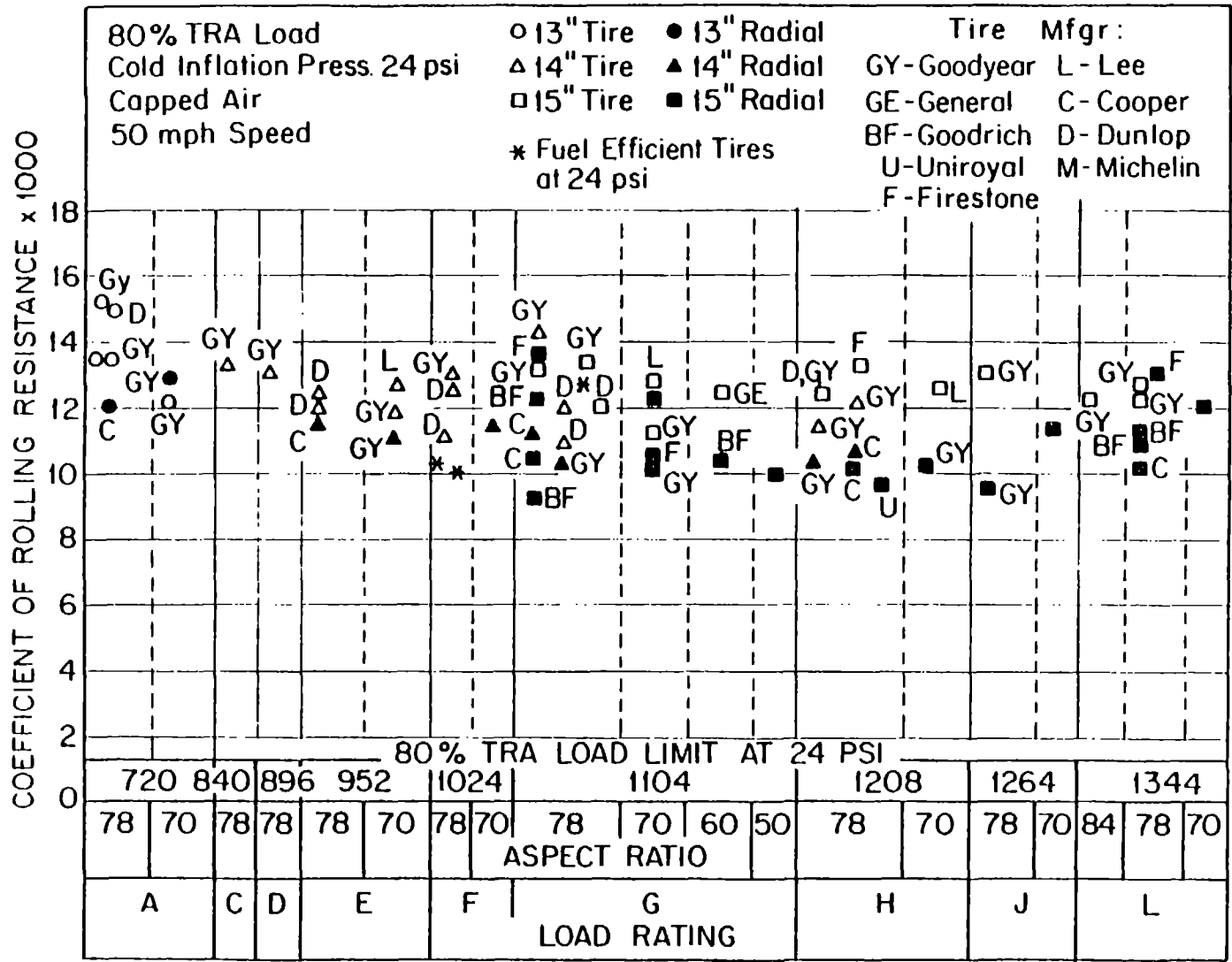
FIGURE 18. COEFFICIENT OF ROLLING RESISTANCE VS. TIRE LOAD RATING FOR A SELECTION OF PASSENGER CAR TIRES
