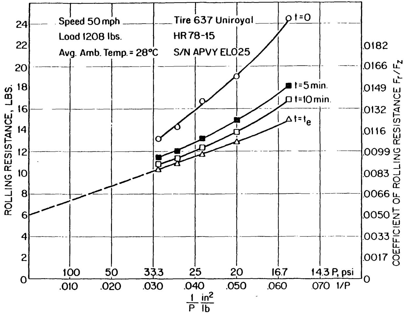
FIGURE 15. ROLLING RESISTANCE AND COEFFICIENT OF ROLLING RESISTANCE VS. RECIPROCAL OF INFLATION PRESSURE FOR HR78-15 RADIAL TIRE
