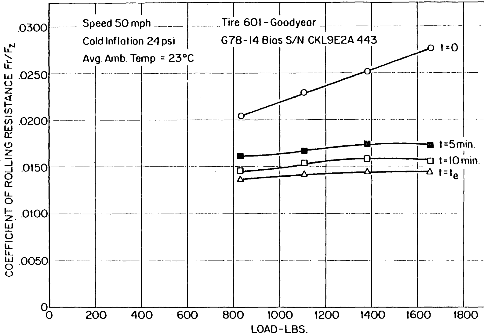
FIGURE 8. COEFFICIENT OF ROLLING RESISTANCE VS. VERTICAL LOAD FOR G78-14 BIAS TIRE
