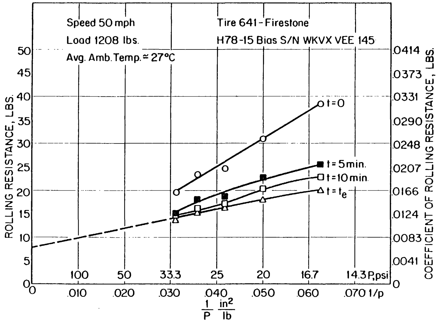
FIGURE 13. ROLLING RESISTANCE AND COEFFICIENT OF ROLLING RESISTANCE VS. RECIPROCAL OF INFLATION PRESSURE FOR H78-15 BIAS TIRE
