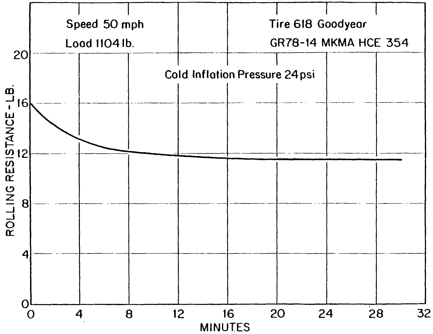
FIGURE 3. TYPICAL ROLLING RESISTANCE VS. TIME VARIATION
