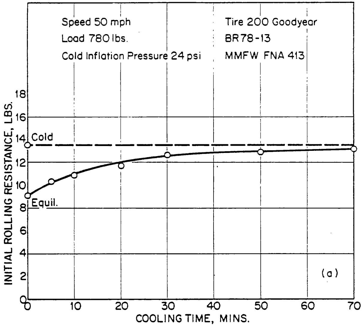
FIGURE 20. ROLLING RESISTANCE VS. COOLING TIME
