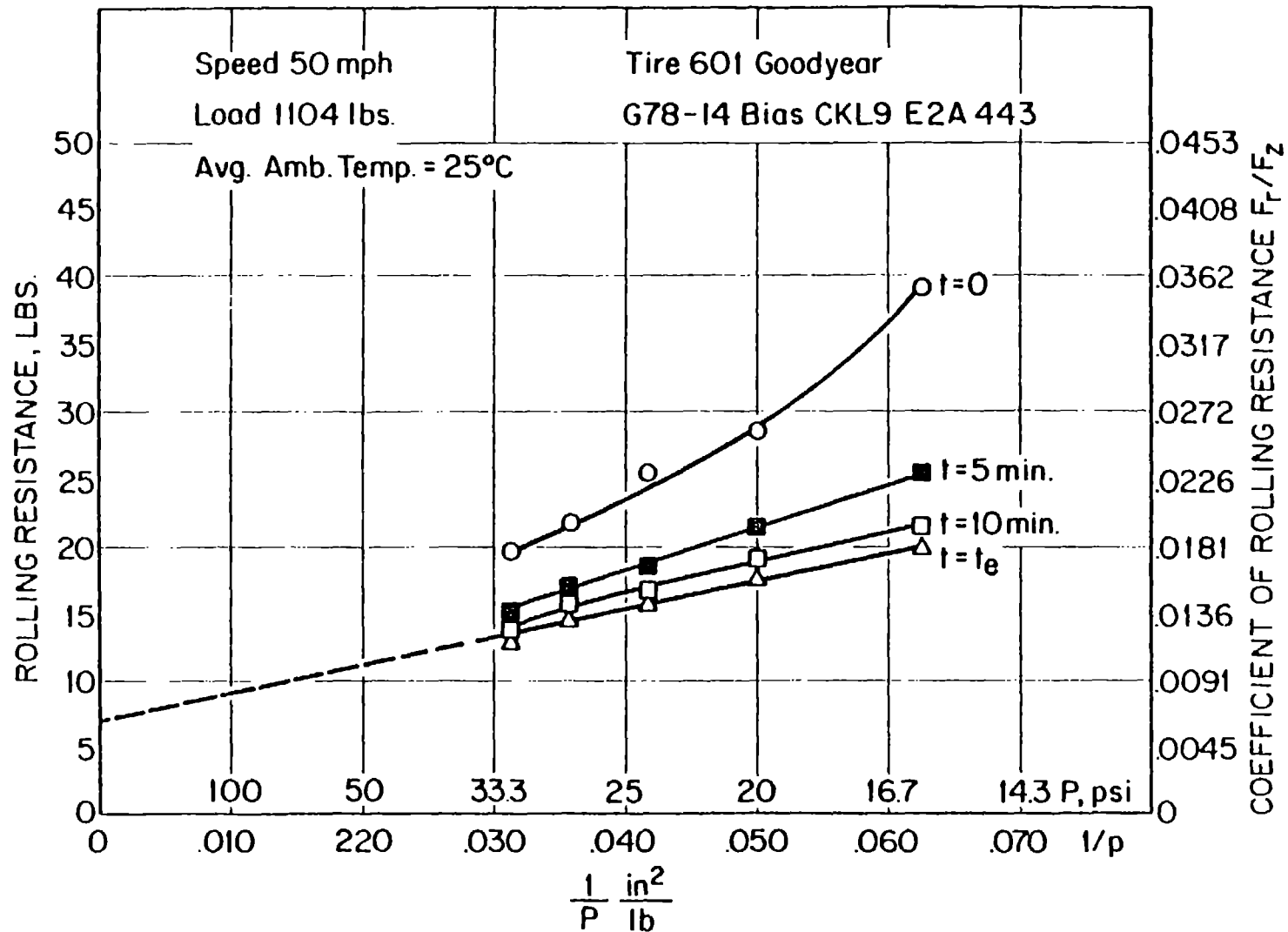
FIGURE 12. ROLLING RESISTANCE AND COEFFICIENT OF ROLLING RESISTANCE VS. RECIPROCAL OF INFLATION PRESSURE FOR G78-14 BIAS TIRE
