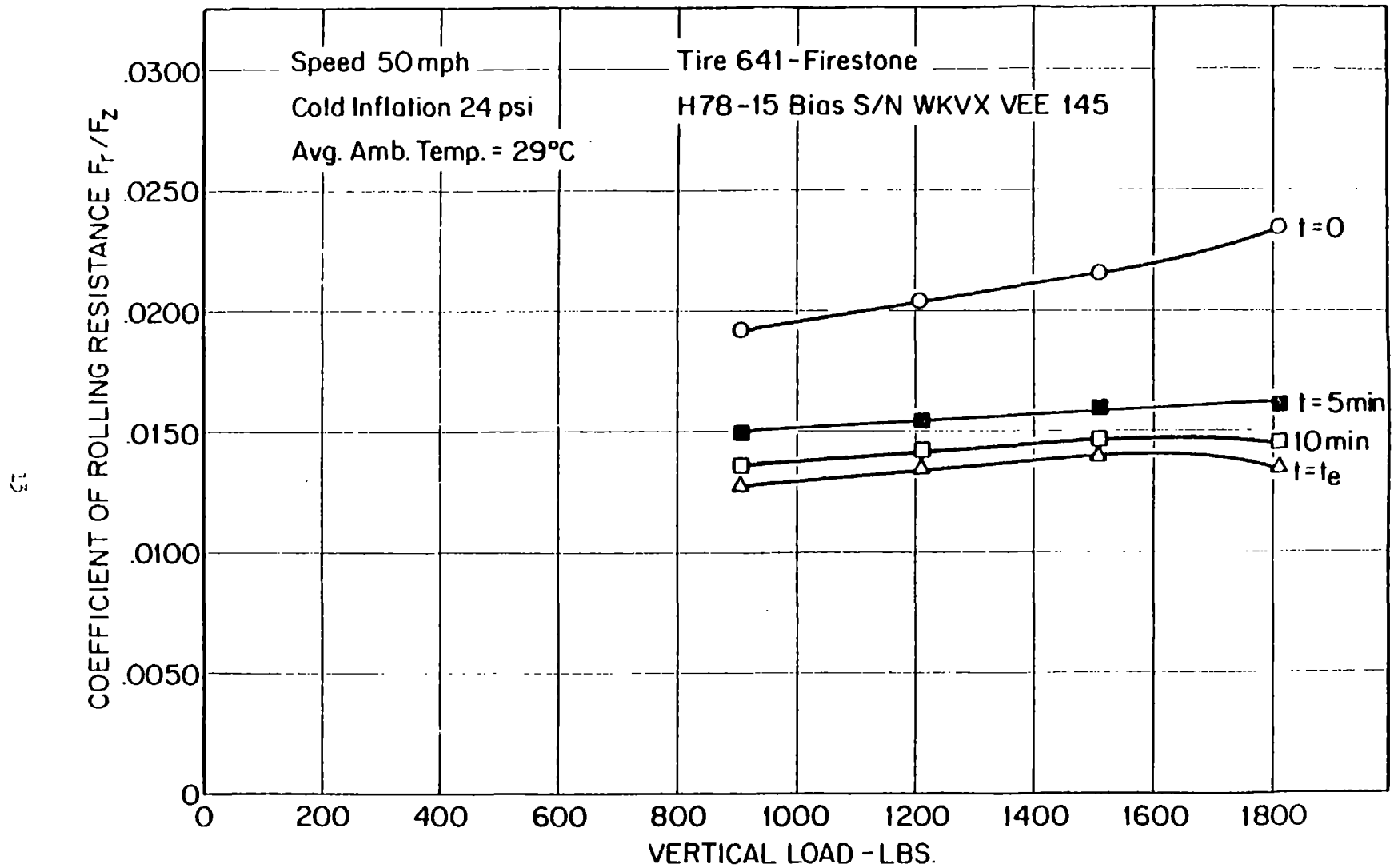
FIGURE 9. COEFFICIENT OF ROLLING RESISTANCE VS. VERTICAL LOAD FOR H78-15 BIAS TIRE
