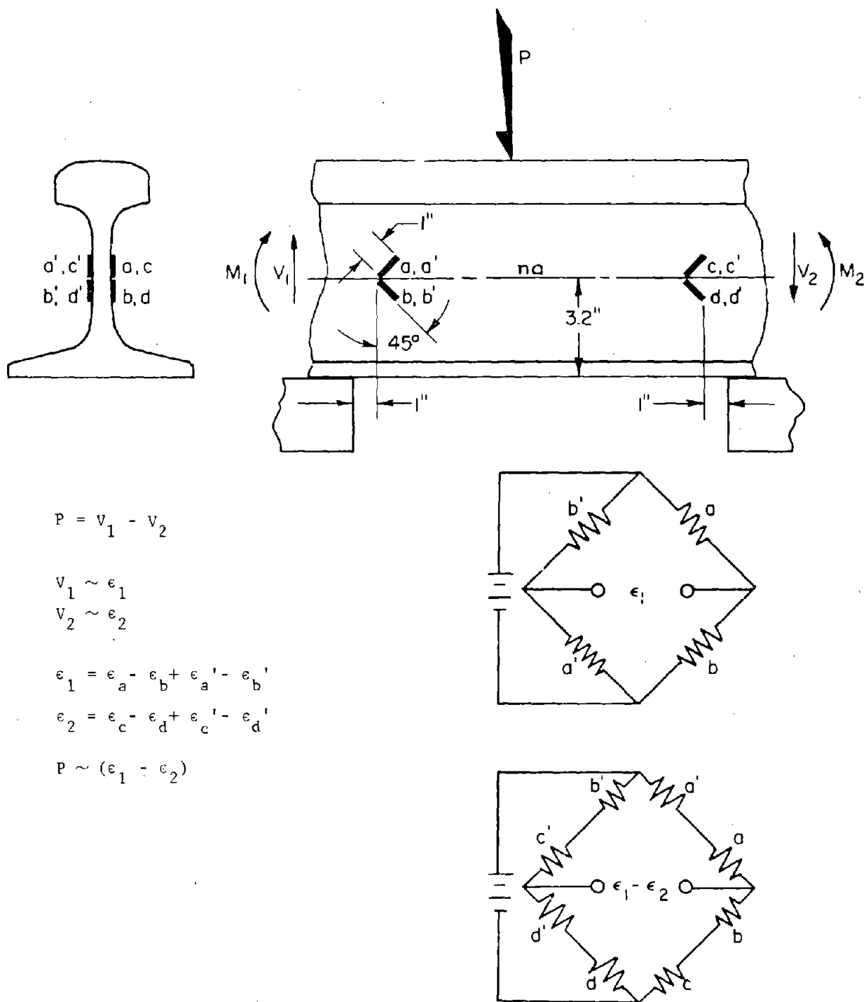
FIGURE 6-3. WHEEL/RAIL VERTICAL LOAD CIRCUITS USING RAIL SHEAR STRESS TO MEASURE LOAD ON 132 LB RAIL
