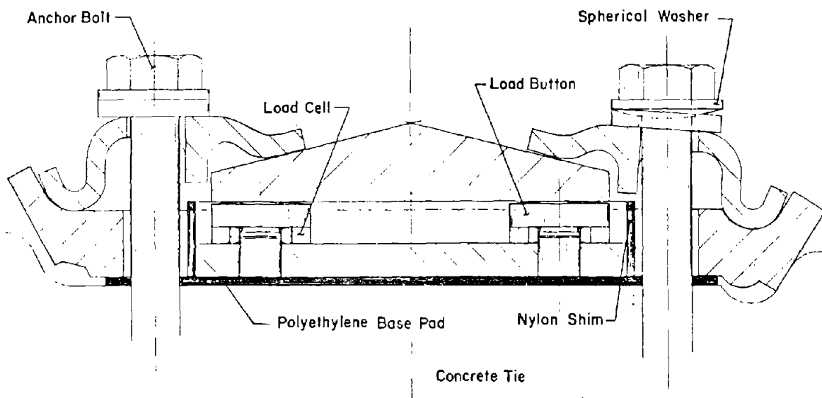
FIGURE 6-5. TIE PLATE LOAD CELL DESIGN RECOMMENDED FOR FEC TIE
