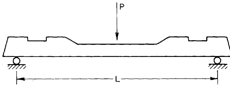
FIGURE 6-10a. LOADING CONFIGURATION TO GENERATE AVERAGE EI VALUE FOR ENTIRE SPAN L = 86 \text{ in.}
