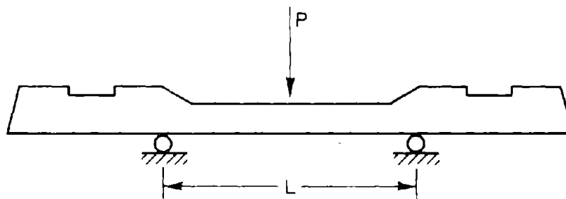
FIGURE 6-10b. LOADING CONFIGURATION TO GENERATE EI VALUE FOR CENTER SECTION L = 36 \text{ in.}
