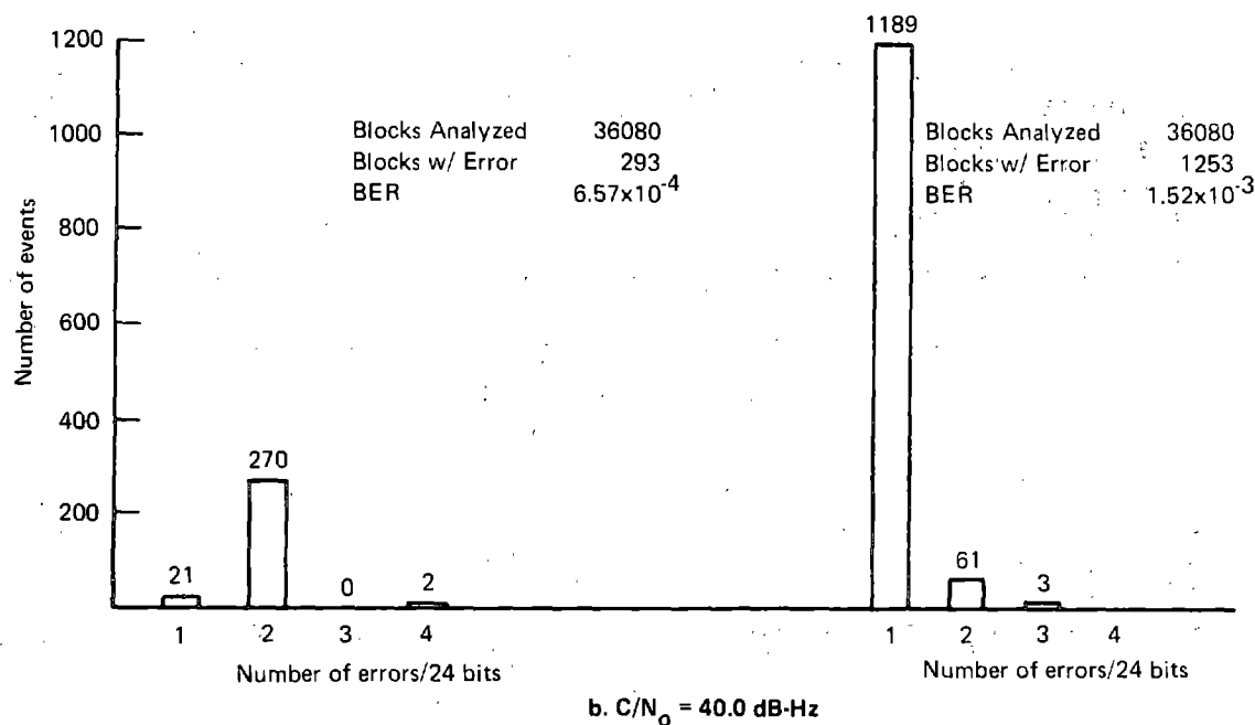
Figure 5-19.—Type I Block Error Histograms
