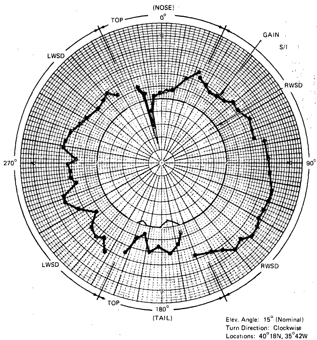
Figure 6-2.—Gain and S/I, Slot Dipole Antennas, March 25, 1975
