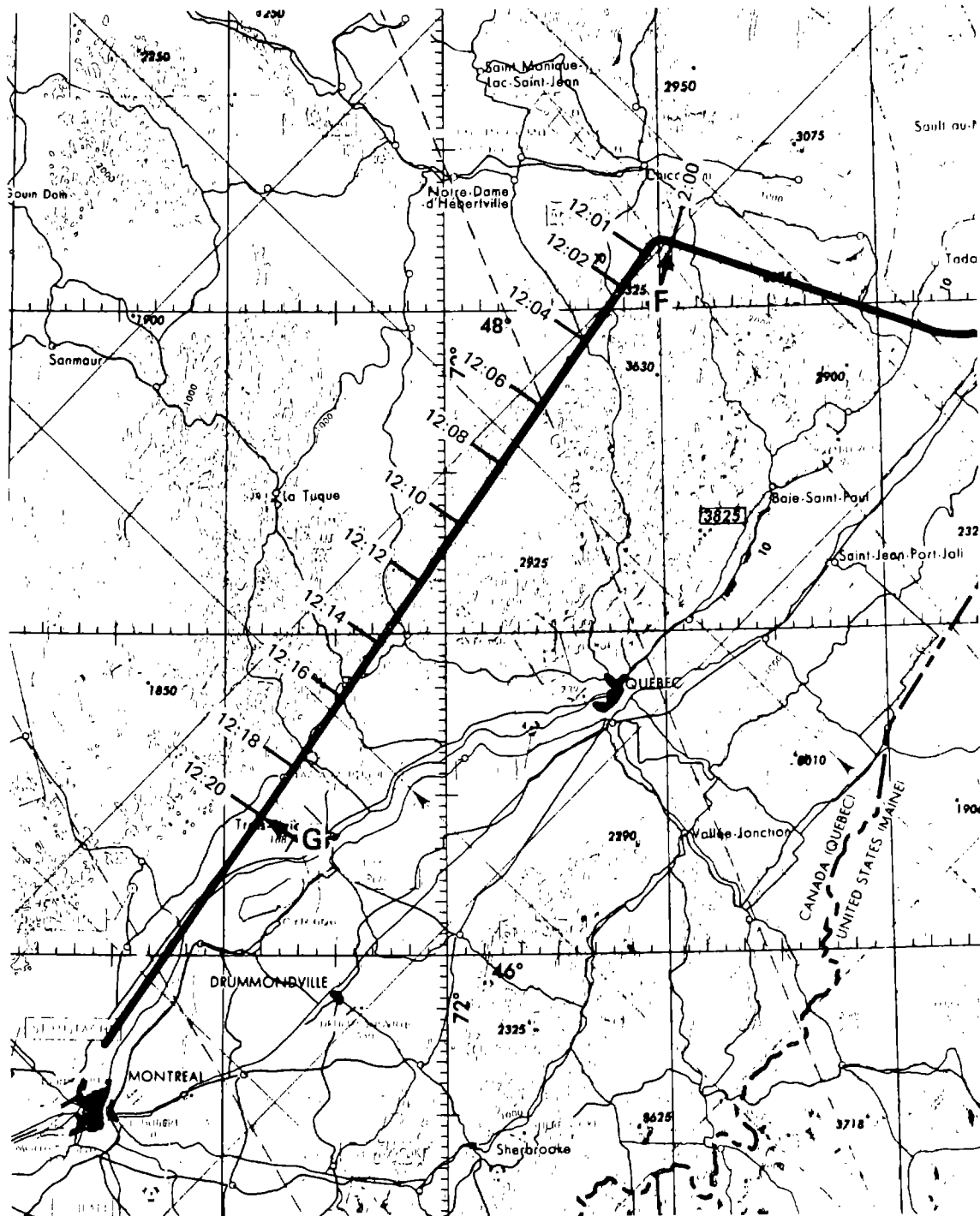
Figure 4-20.—Specular Point Overlay Leg FG February 20, 1975
