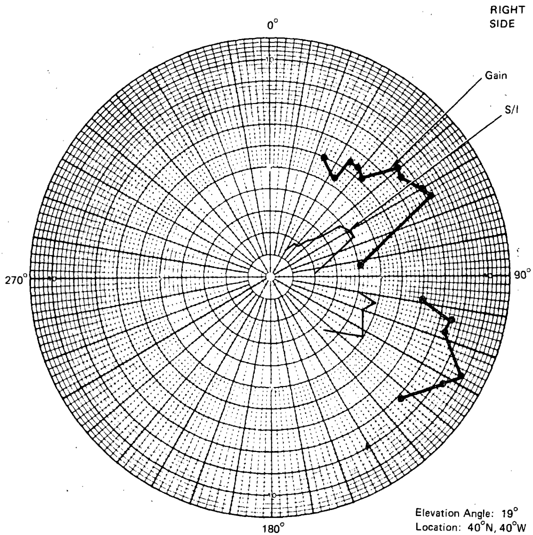
Figure 6-9.—Gain and S/I, Phased Array, November 21, 1974
