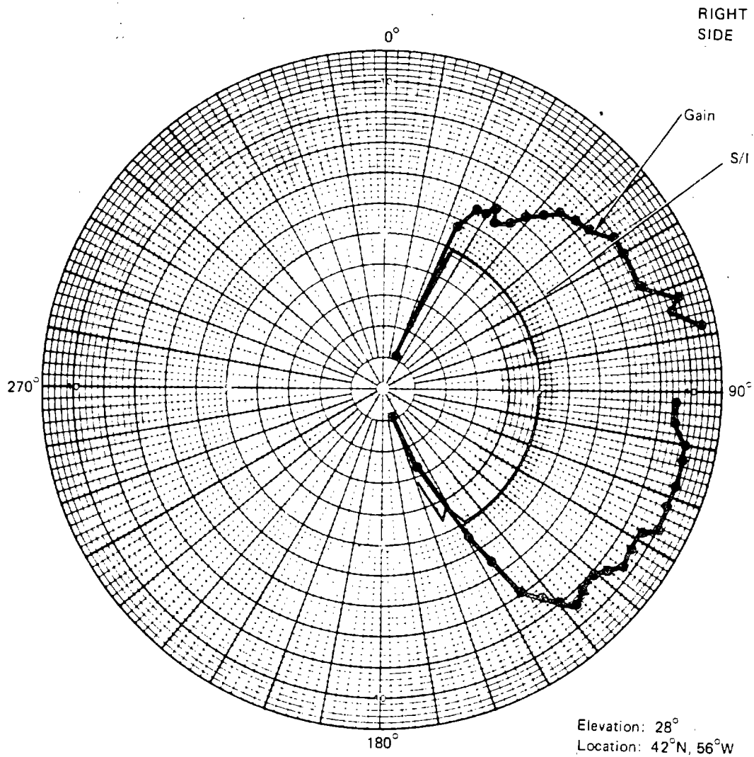
Figure 6-8.—Gain and S/I, Phased Array, September 24, 1974
