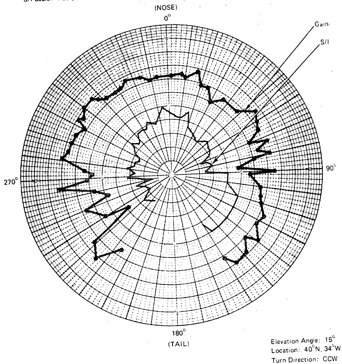
Figure 6-11.—Gain and S/I, Crossed Slot, April 1, 1975
