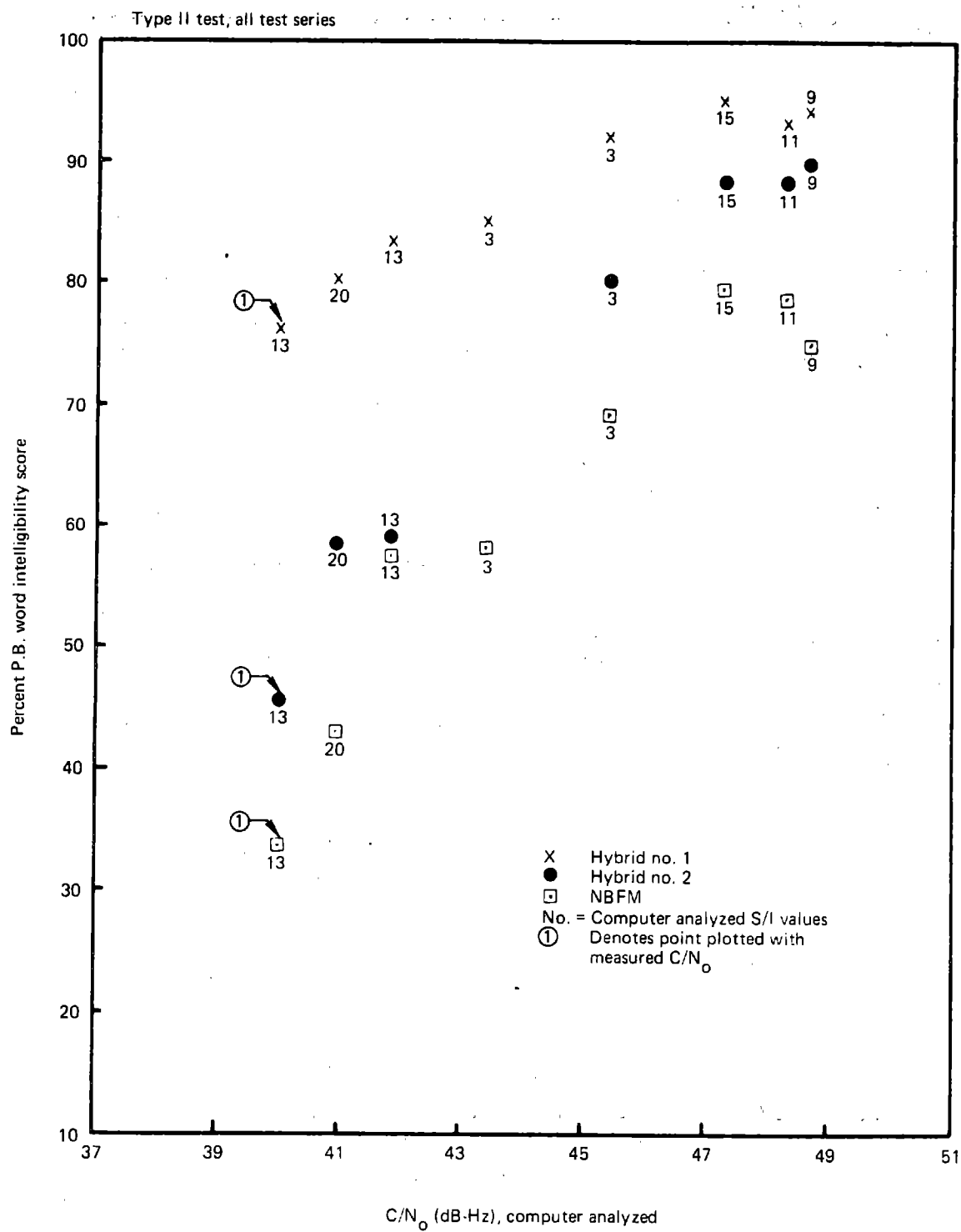
Figure 5-6.—Voice Modem Intelligibility Score, Voice Only Mode
