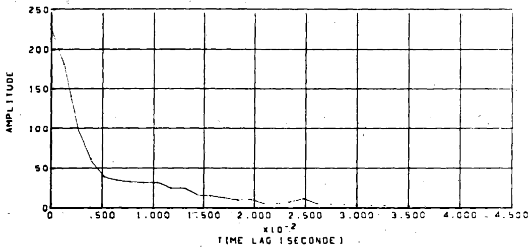
Figure 4-10(b).—Spectra and Autocorrelation Parameters—Vertical Polarization, In-plane Geometry
