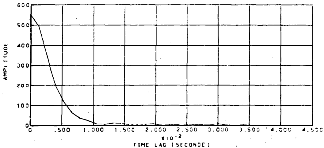
Figure 4-8(b).—Spectra and Autocorrelation Parameters—Horizontal Polarization, 45° Heading
