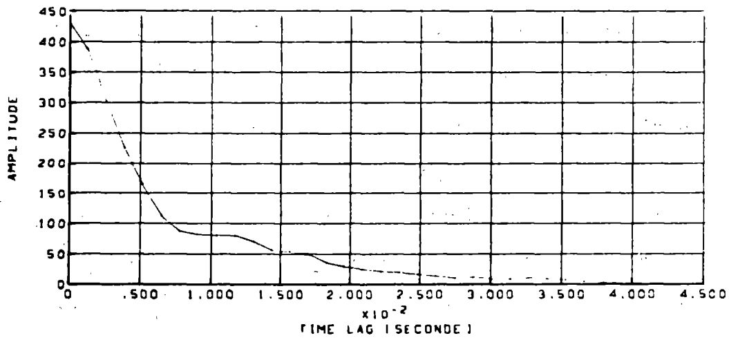
Figure 4-7(b).—Spectra and Autocorrelation Parameters—Horizontal Polarization, In-plane Geometry
