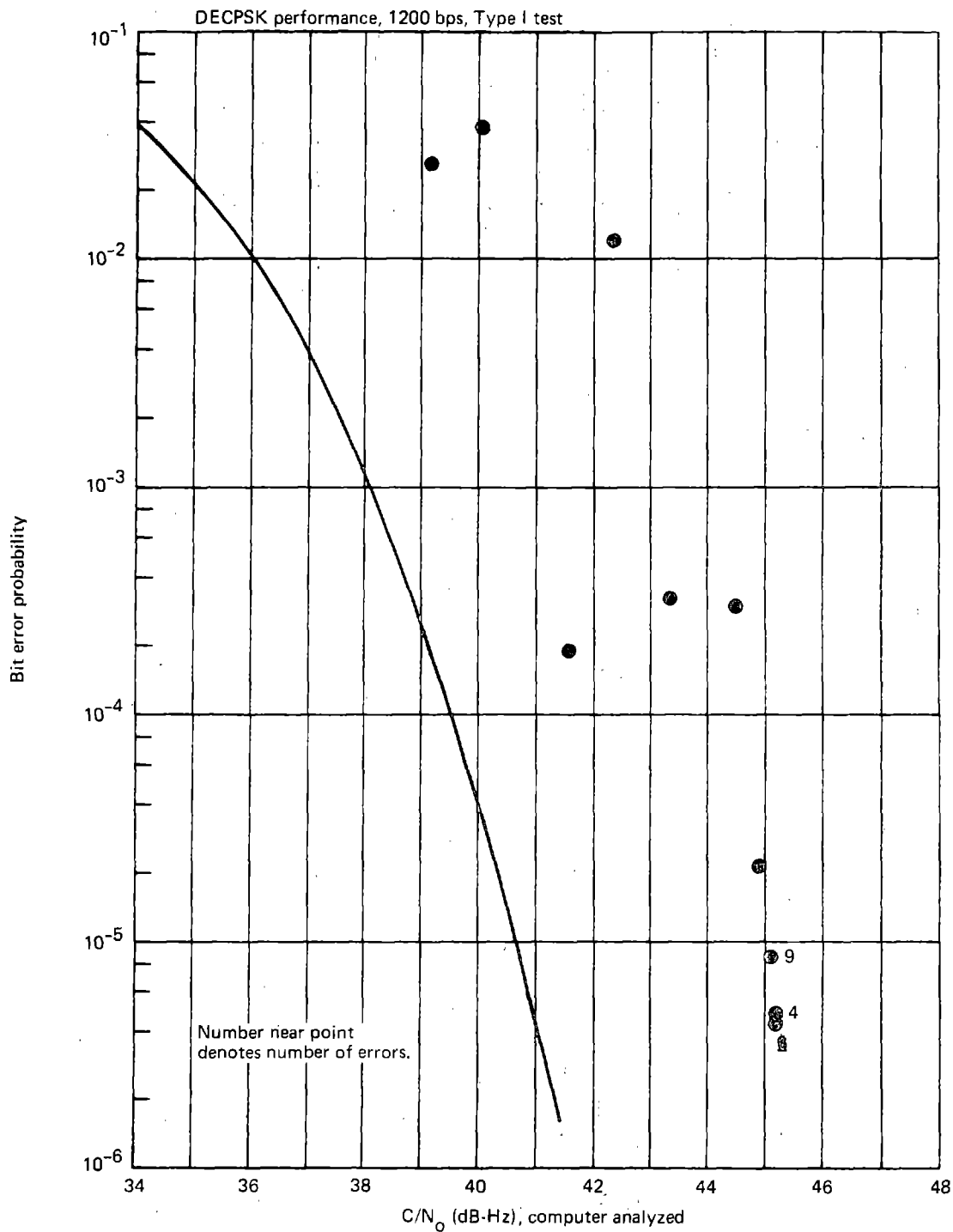
Figure 5-13.—BER Performance, Hybrid Number 2 Demodulator, Hybrid Mode
