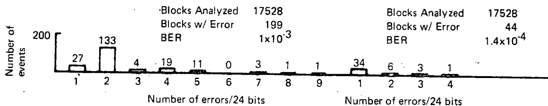
Figure 5-20.—Type II Block Error Histograms
