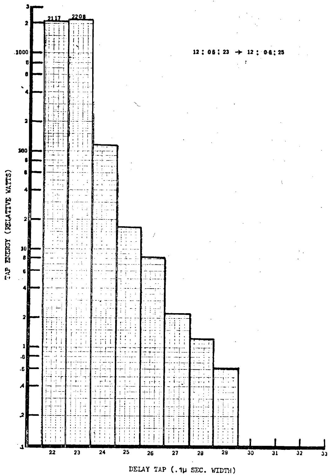
Figure 4-32.—O'Hare Delay Spectra (12:06:24 GMT)
