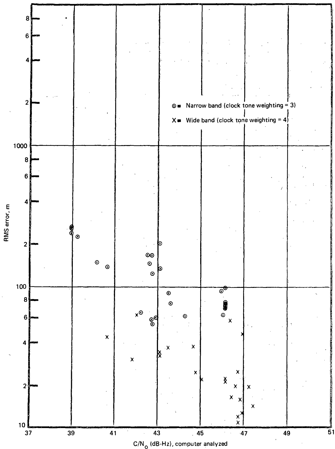
Figure 5-21.—RMS Error Performance, TSC Ranging Modem
