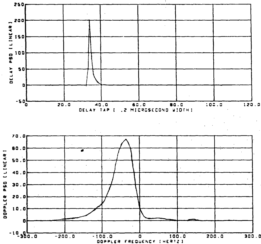
Figure 4-26(b).—CONUS Scatter Channel Parameters—February 19, 1975, Vertical Polarization
