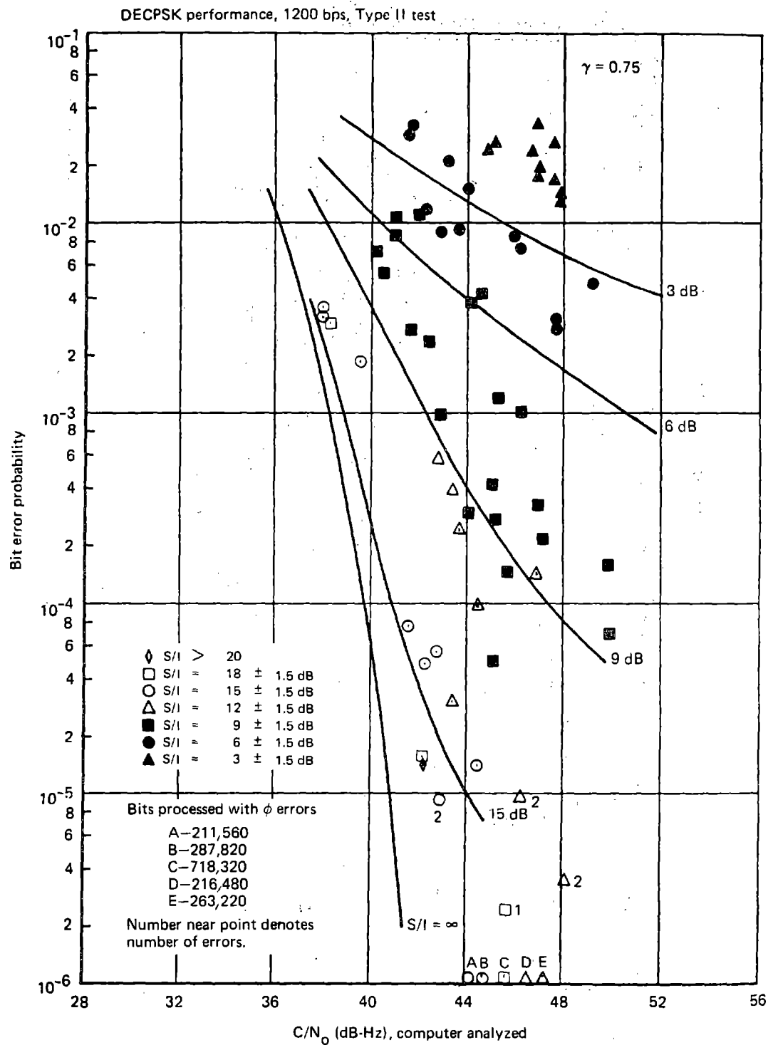
Figure 5-17.—BER Performance, CPSK Demodulator
