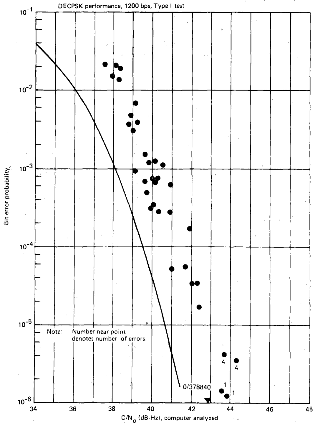
Figure 5-7.--BER Performance, NASA DECPSK Demodulator
