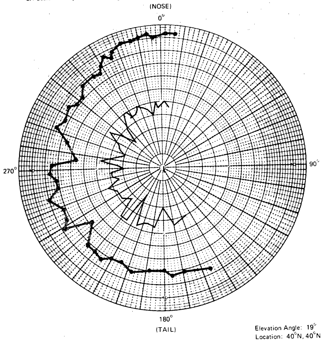
Figure 6-10.—Gain and S/I, Patch Antenna, November 21, 1974
