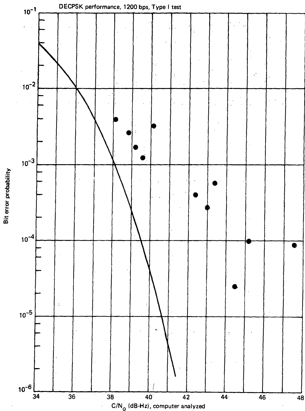
Figure 5-12.—BER Performance, Hybrid Number 1 Demodulator, Hybrid Mode
