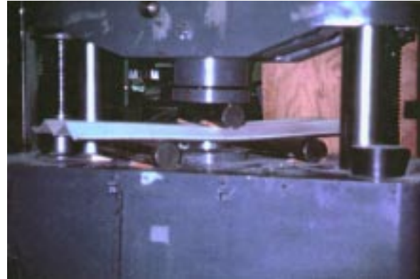
Figure 11. Testing of commercial FRP beam W-configuration.
