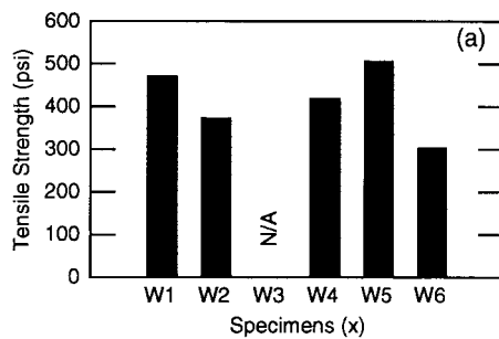
a. Tensile strengths of x specimens.
