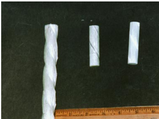
Figure 65. Preparation of the notched bar impact test specimen from the FRP rebar sample.
