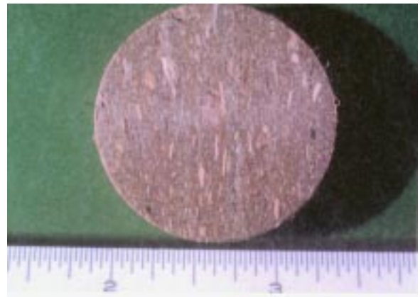
Figure 40. Section of the improved RPC specimens free of any wood chip inclusions.
