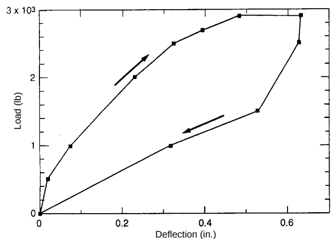
Figure 12. Test results of commercial FRP beam of W-configuration.
