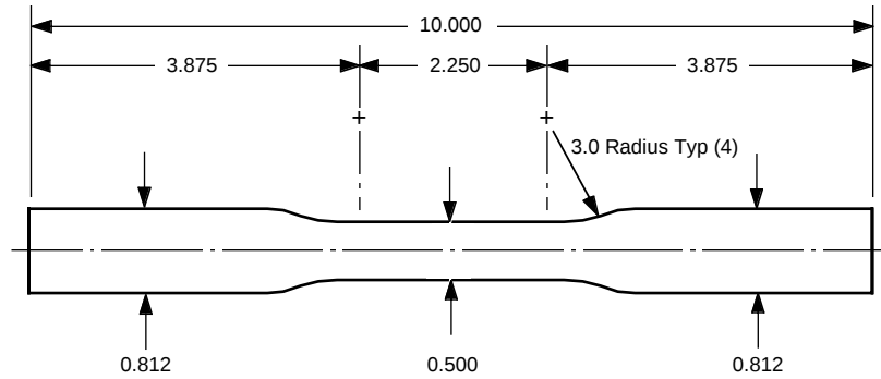
Figure 16. Dimensions of the coupon test specimens.
