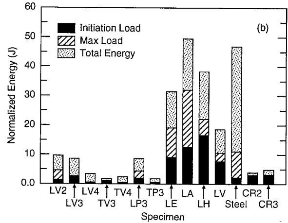
b. Comparison of normalized energy for the W-beam composites with other composites.
