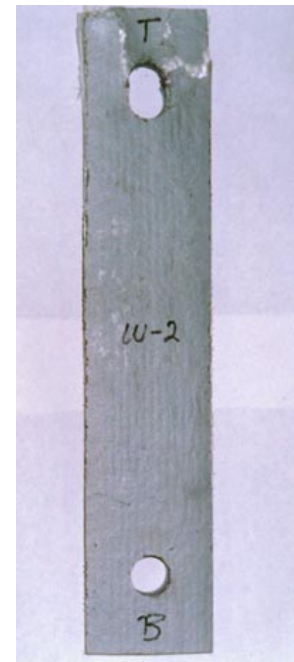
Figure 25. Failed specimen from the bolt pull-out test.
