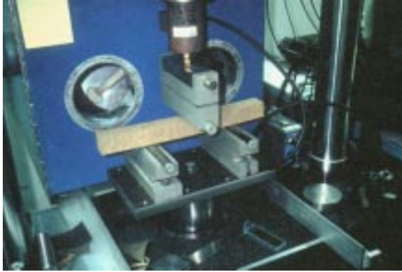
Figure 52. Flexural testing of the RPC.
