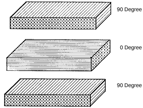
Figure 4. Schematic representation of a fiber composite lamina.
