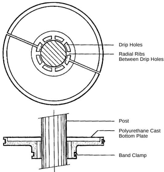
Figure 76. Details of the bottom end-cap.
