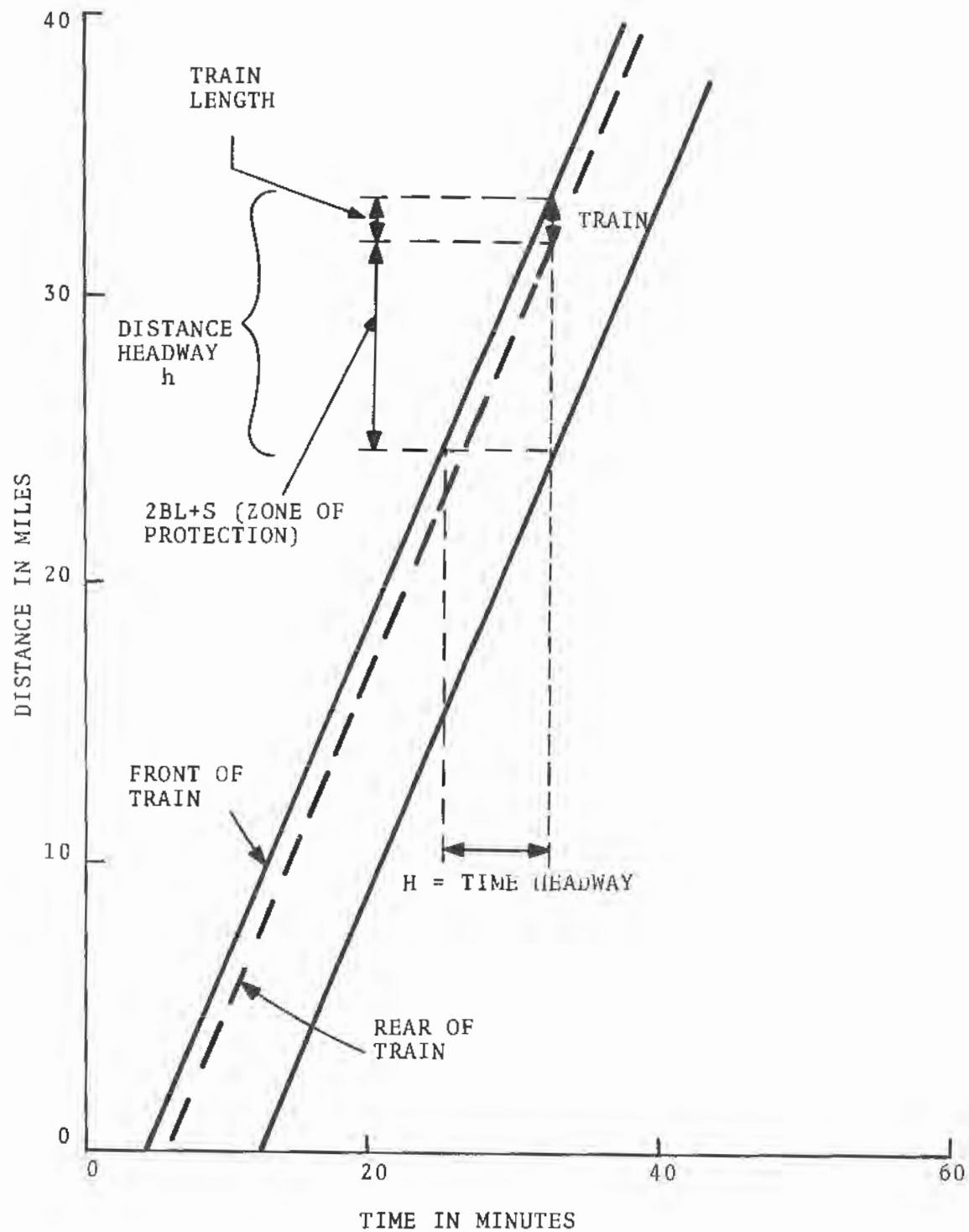
Figure 5-2. Simplified Train Graph I
