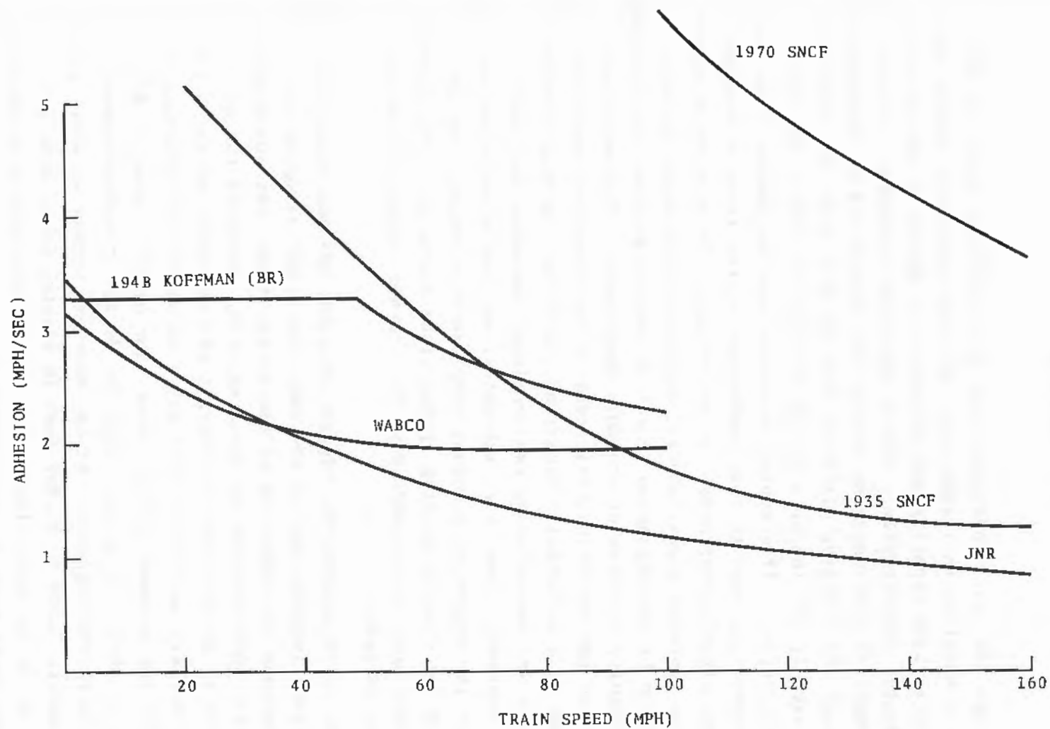
Figure A-1. Wheel-to-Rail Adhesion ~ Worst-Case Values
