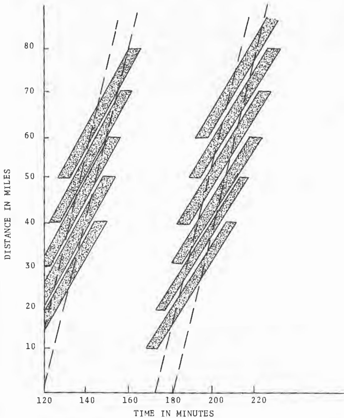
Figure 5-11. Case VIIb - Passing Tracks and Running Meets - Occupancy of the Passing Tracks (Dashed Lines Indicate HSPT's on Running Track - Crossovers Located at 10-Mile Intervals)
