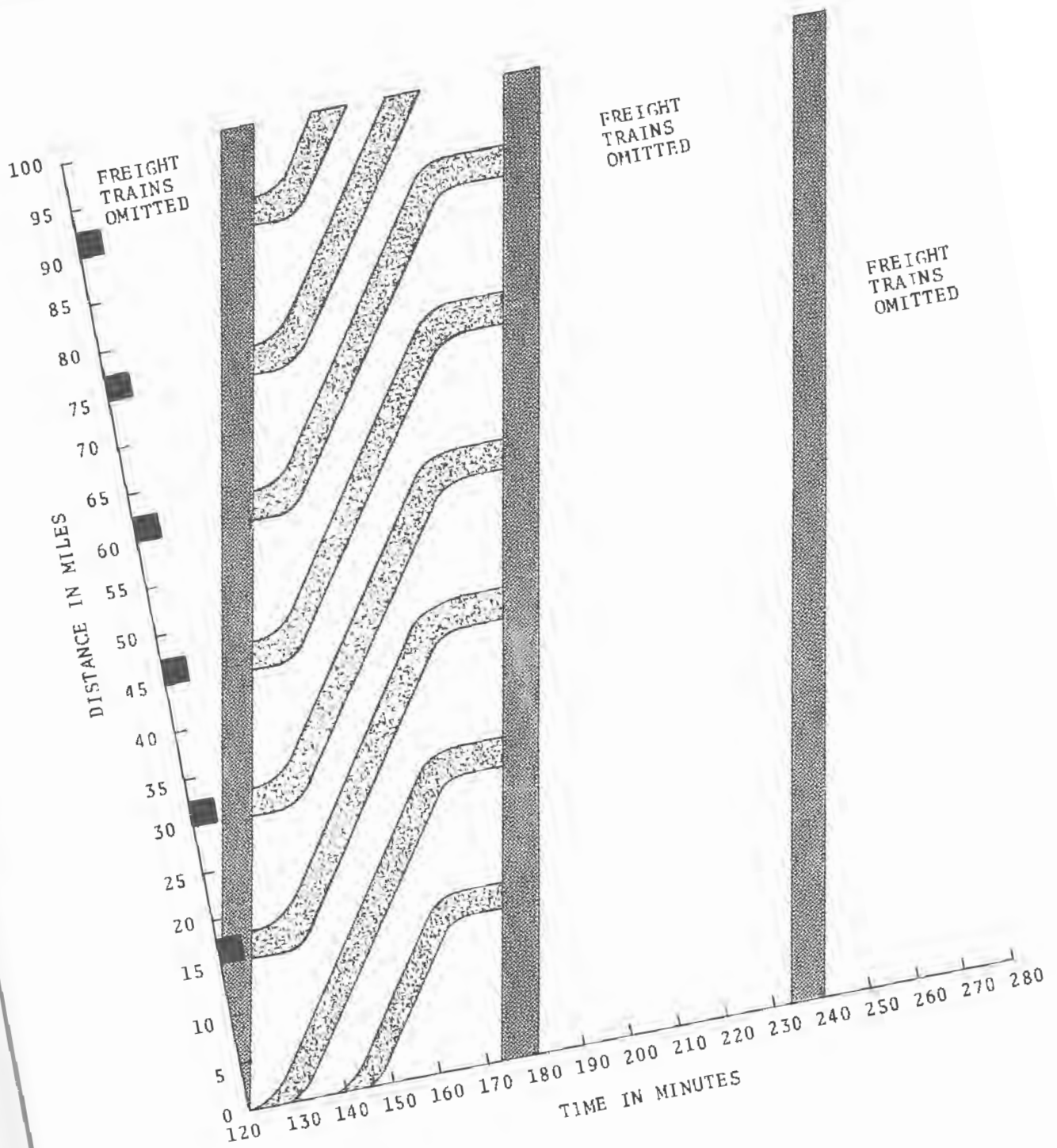
Figure 5-6. Train Graph III - 150 MPH HSPT's, 50 MPH Freight Train
