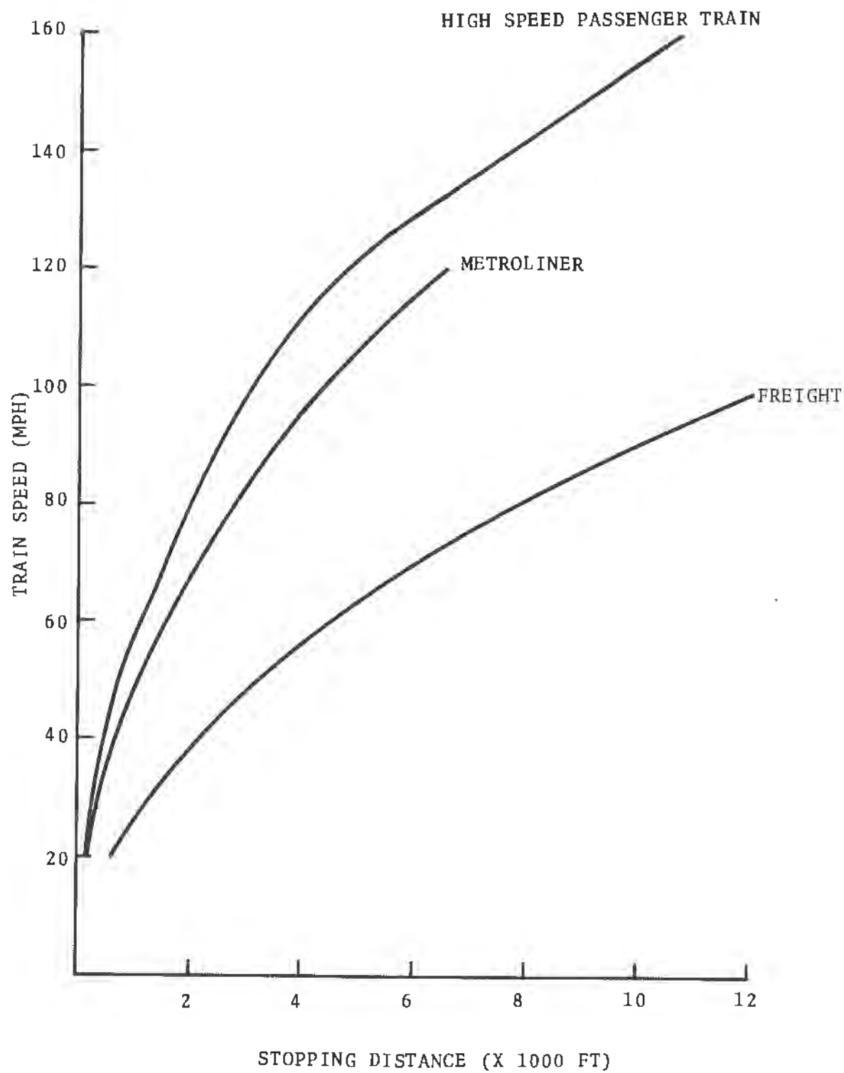
Figure 2-5. Stopping Distances, +1% Grade
