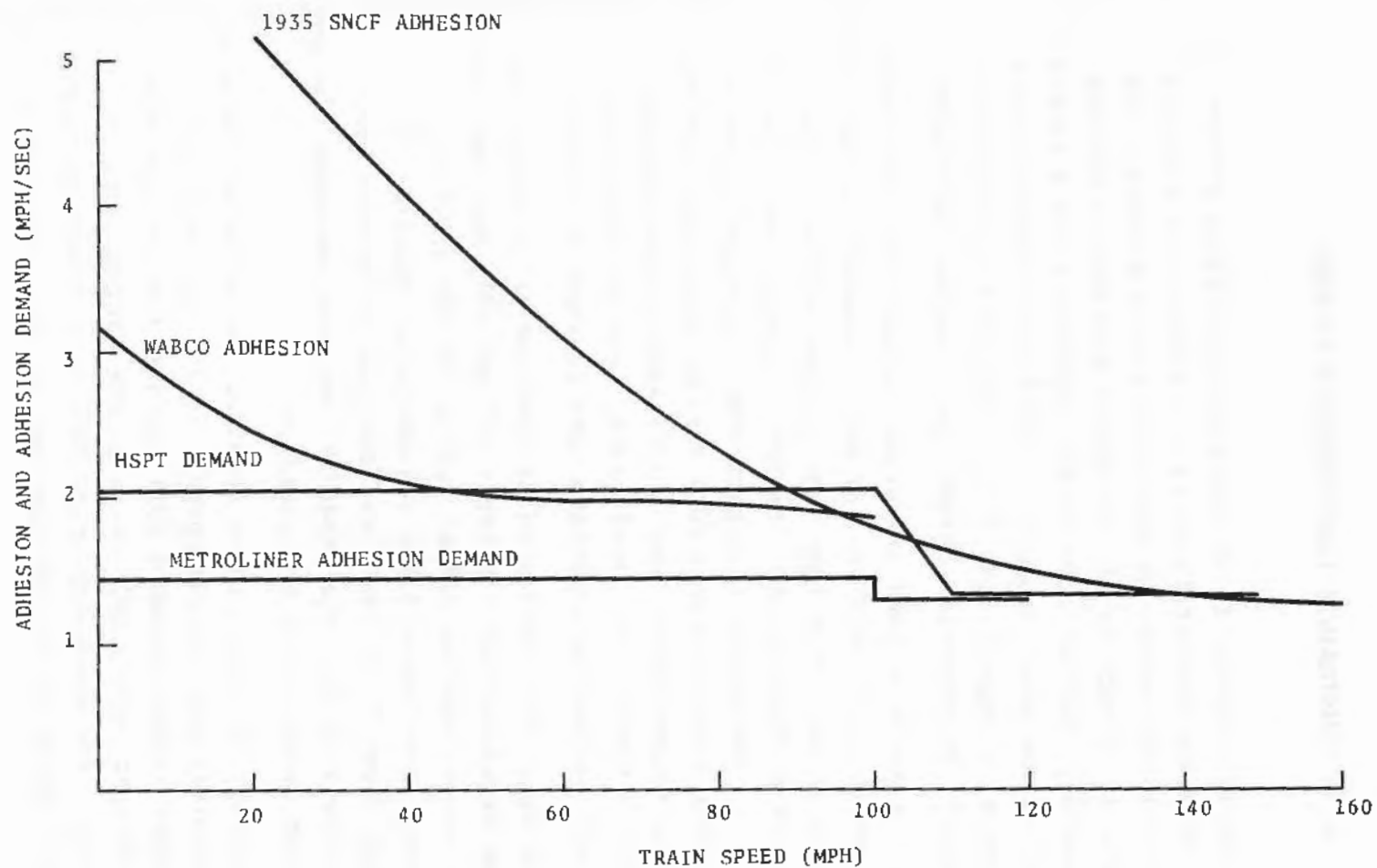
Figure A-4. Worst-Case Adhesion and Adhesion Demand Assumed for Metroliner and Hypothetical HSPT
